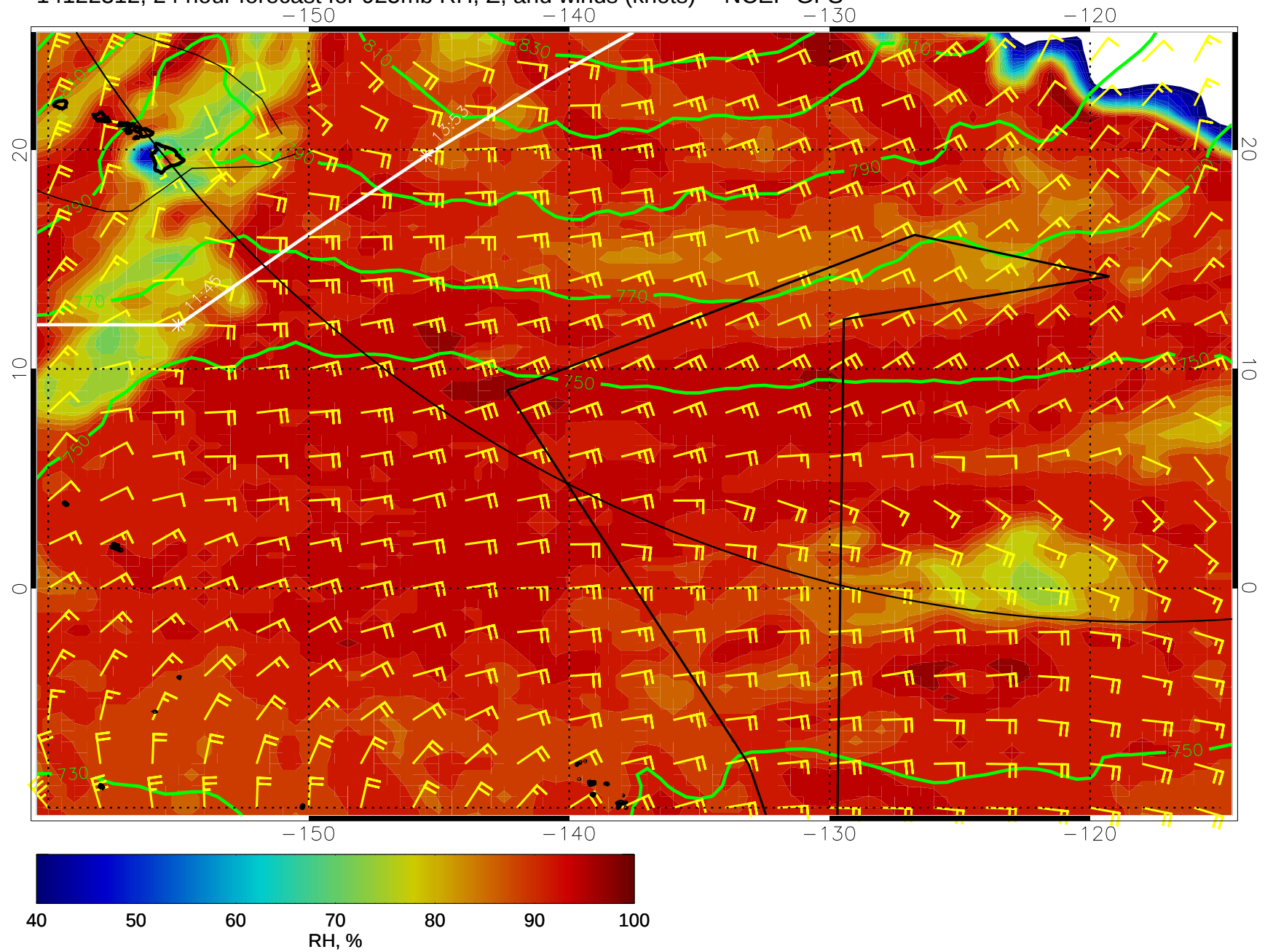
14122312, 24 hour forecast for 925mb RH, Z, and winds (knots) -- NCEP GFS
