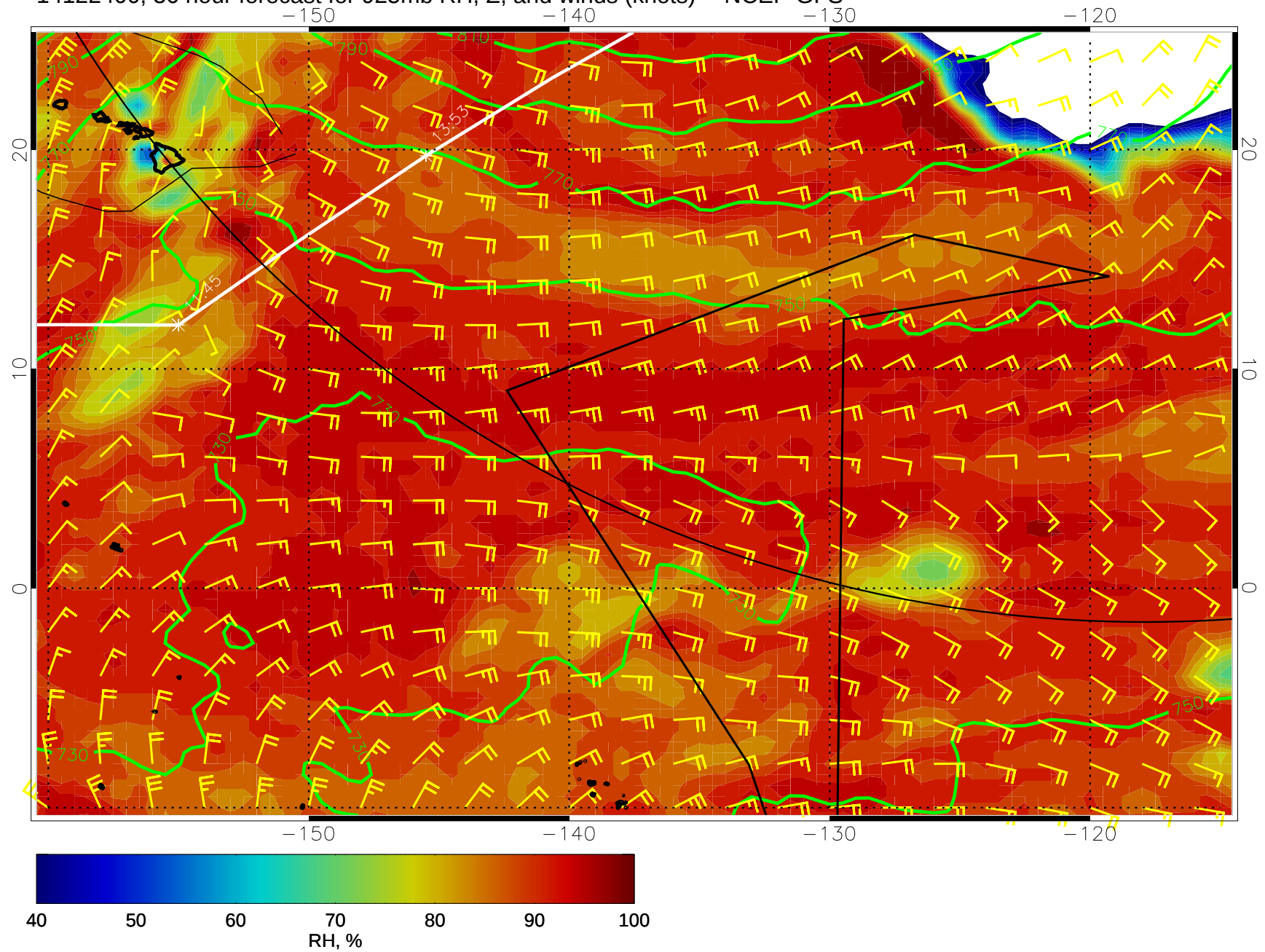
14122400, 36 hour forecast for 925mb RH, Z, and winds (knots) -- NCEP GFS
