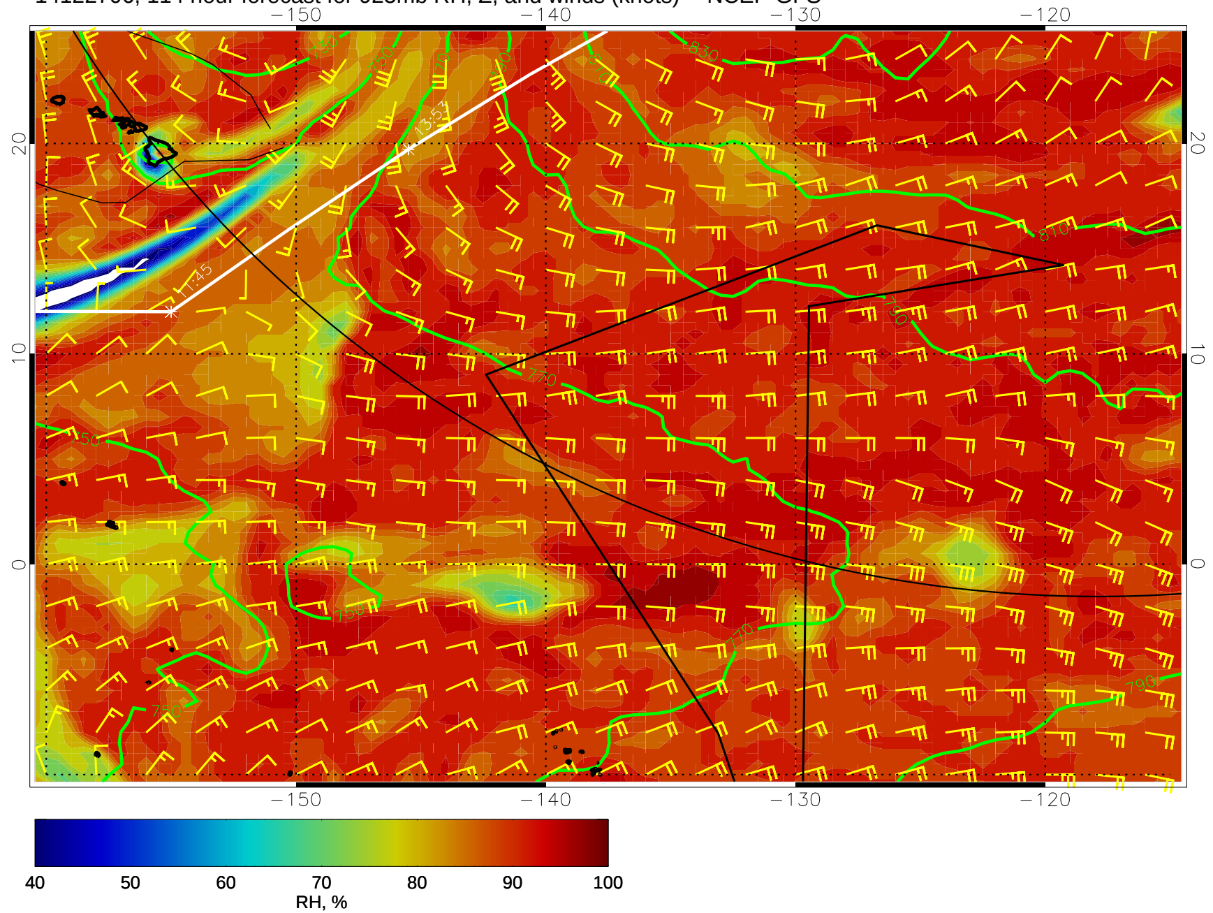
14122706, 114 hour forecast for 925mb RH, Z, and winds (knots) -- NCEP GFS
