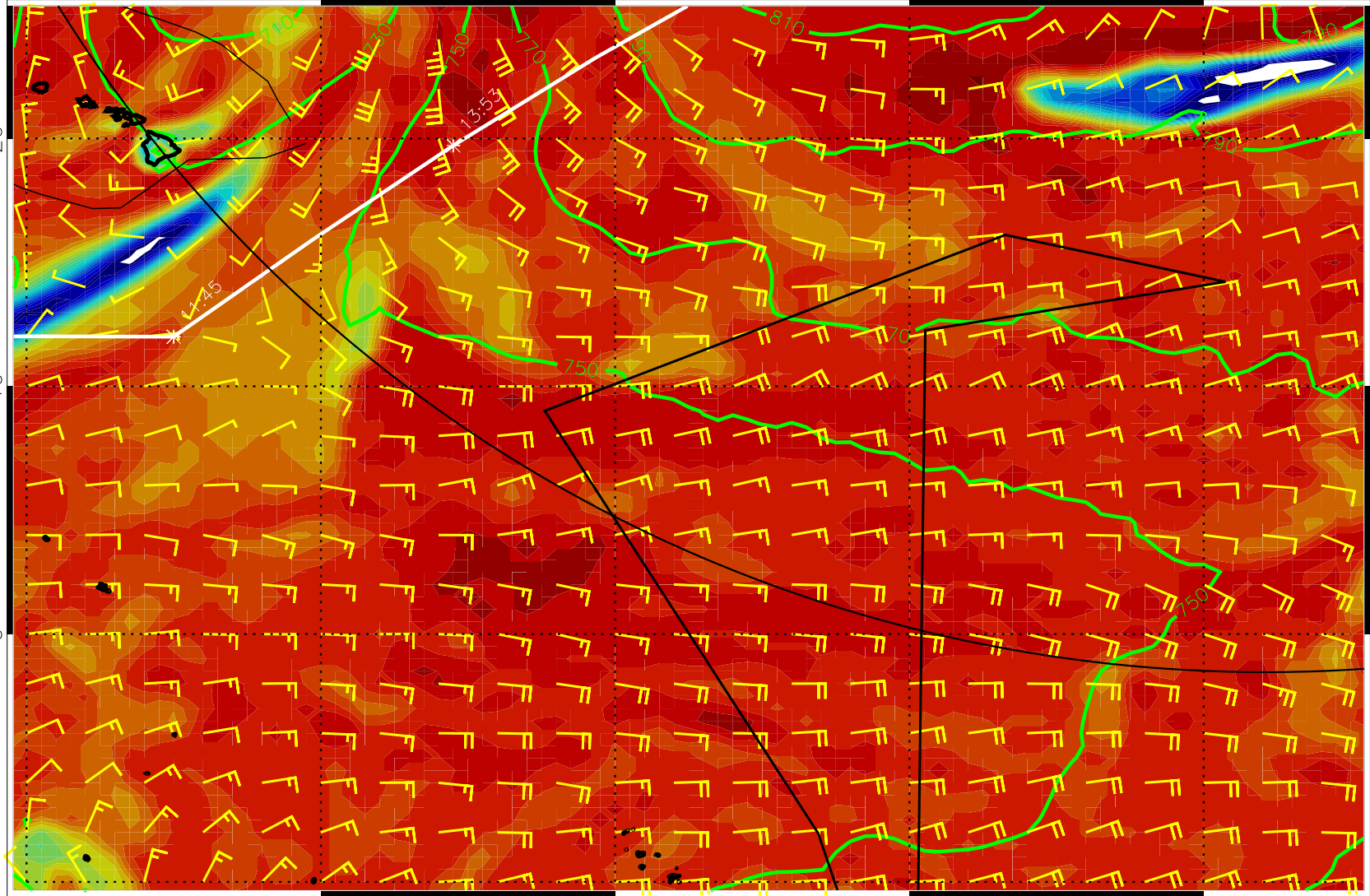
East for elements A, B, and C (km/s) \rightarrow 150 \rightarrow 140 \rightarrow 130 \rightarrow 120
