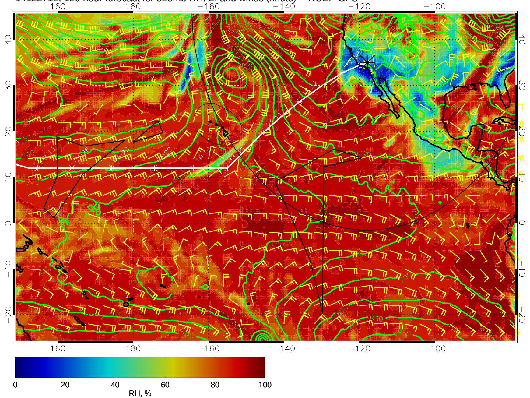
14122712, 120 hour forecast for 925mb RH, Z, and winds (knots) -- NCEP GFS
