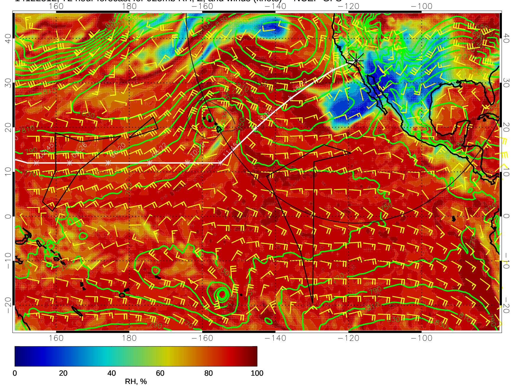
14122512, 72 hour forecast for 925mb RH, Z, and winds (knots) -- NCEP GFS
