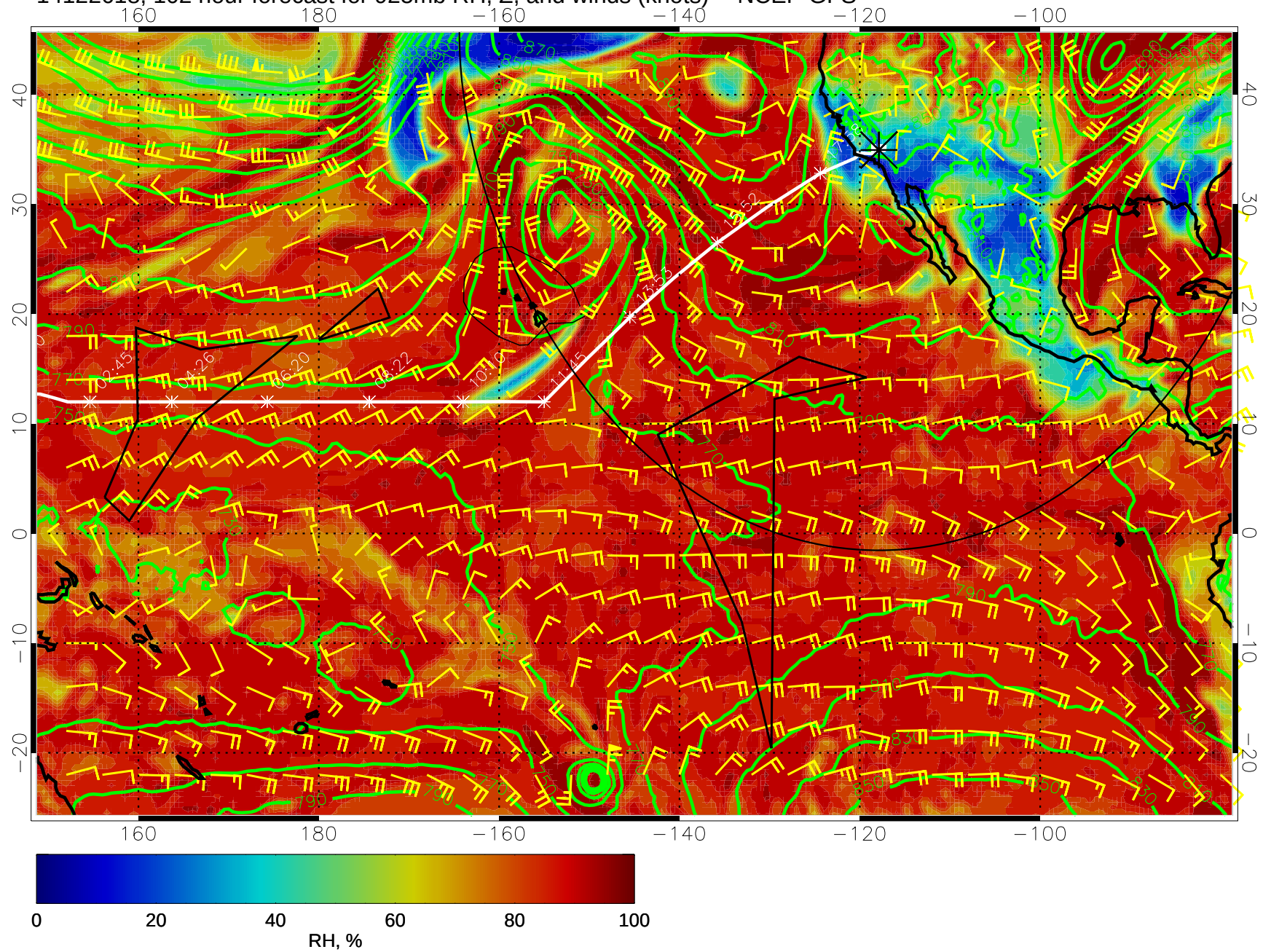
14122618, 102 hour forecast for 925mb RH, Z, and winds (knots) -- NCEP GFS
