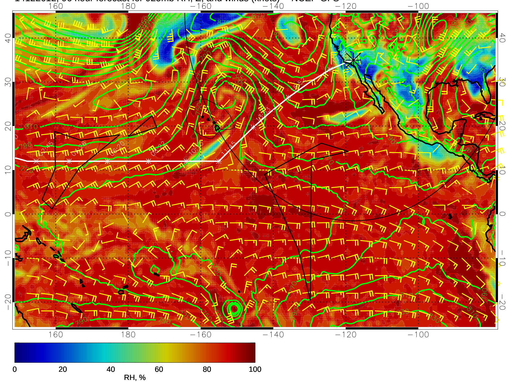
14122612, 96 hour forecast for 925mb RH, Z, and winds (knots) -- NCEP GFS
