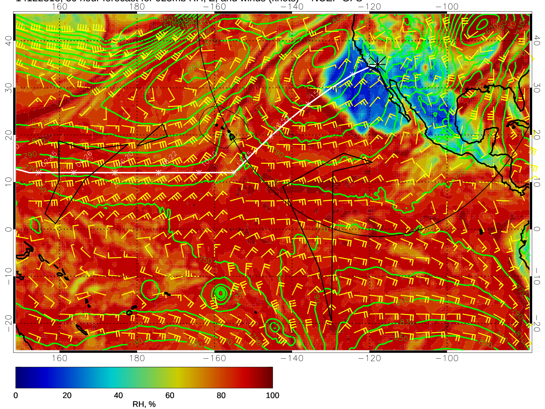
14122318, 30 hour forecast for 925mb RH, Z, and winds (knots) -- NCEP GFS
