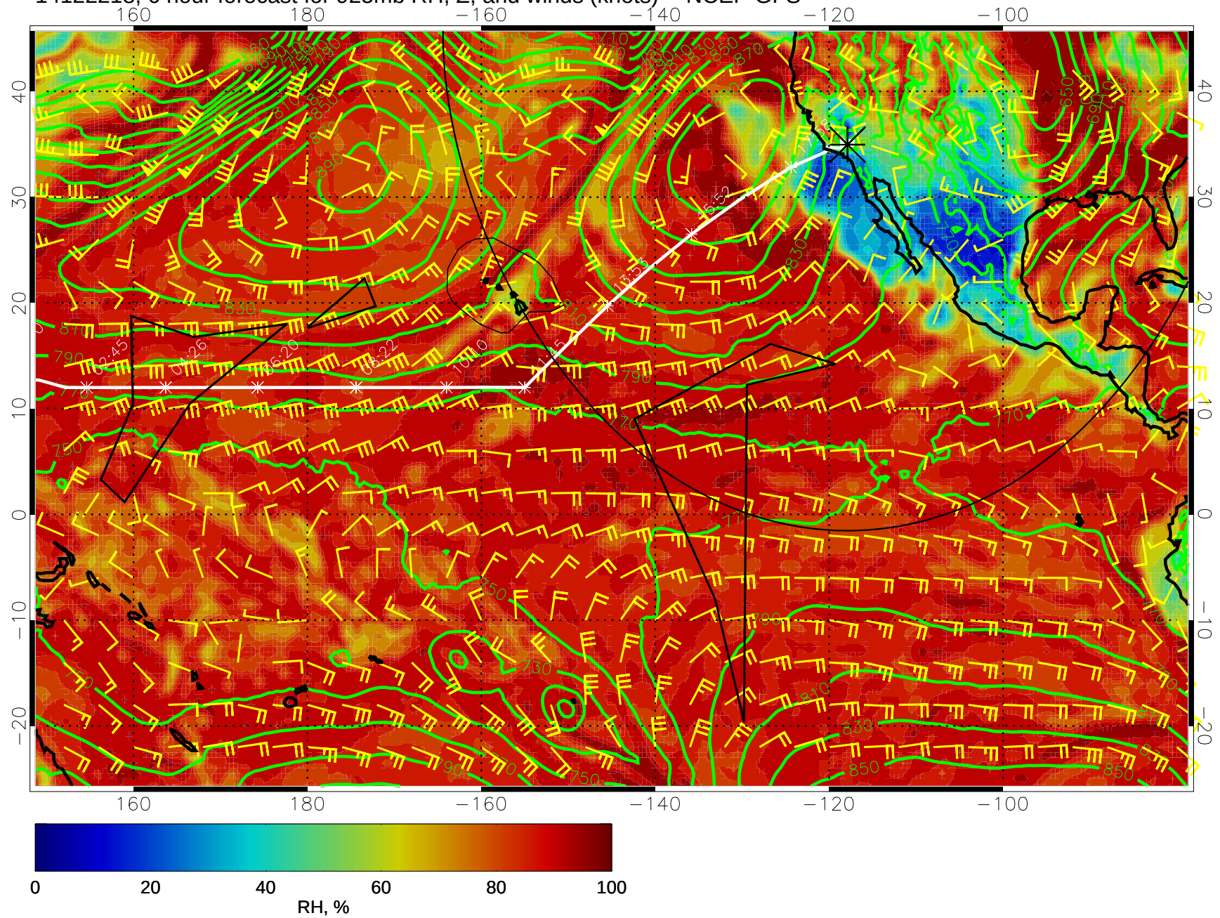
14122218, 6 hour forecast for 925mb RH, Z, and winds (knots) -- NCEP GFS
