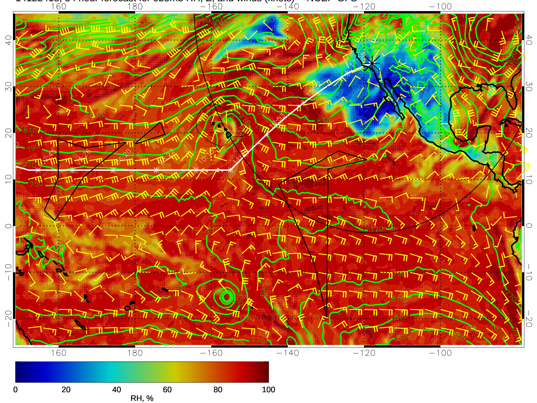
14122418, 54 hour forecast for 925mb RH, Z, and winds (knots) -- NCEP GFS
