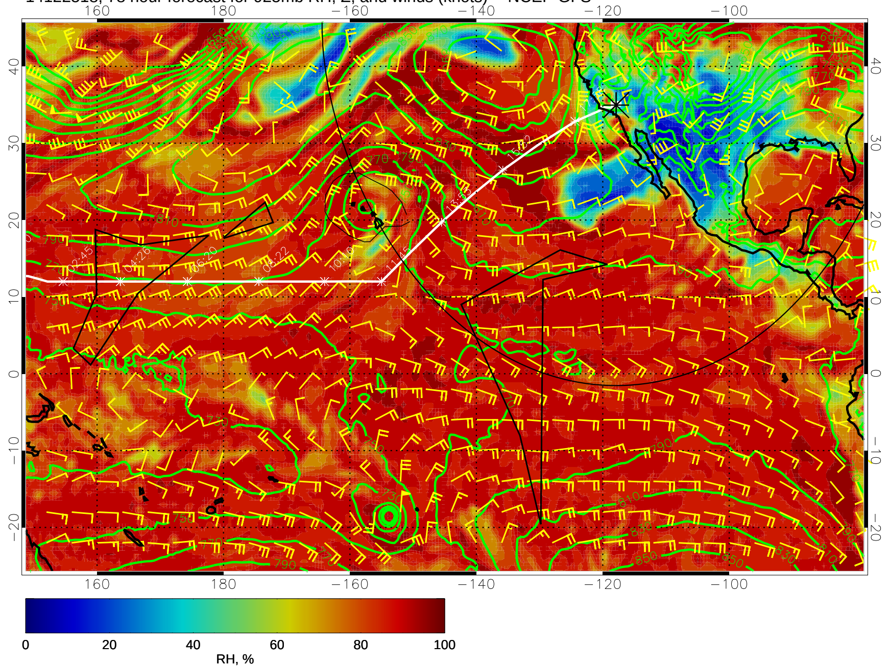
14122518, 78 hour forecast for 925mb RH, Z, and winds (knots) -- NCEP GFS
