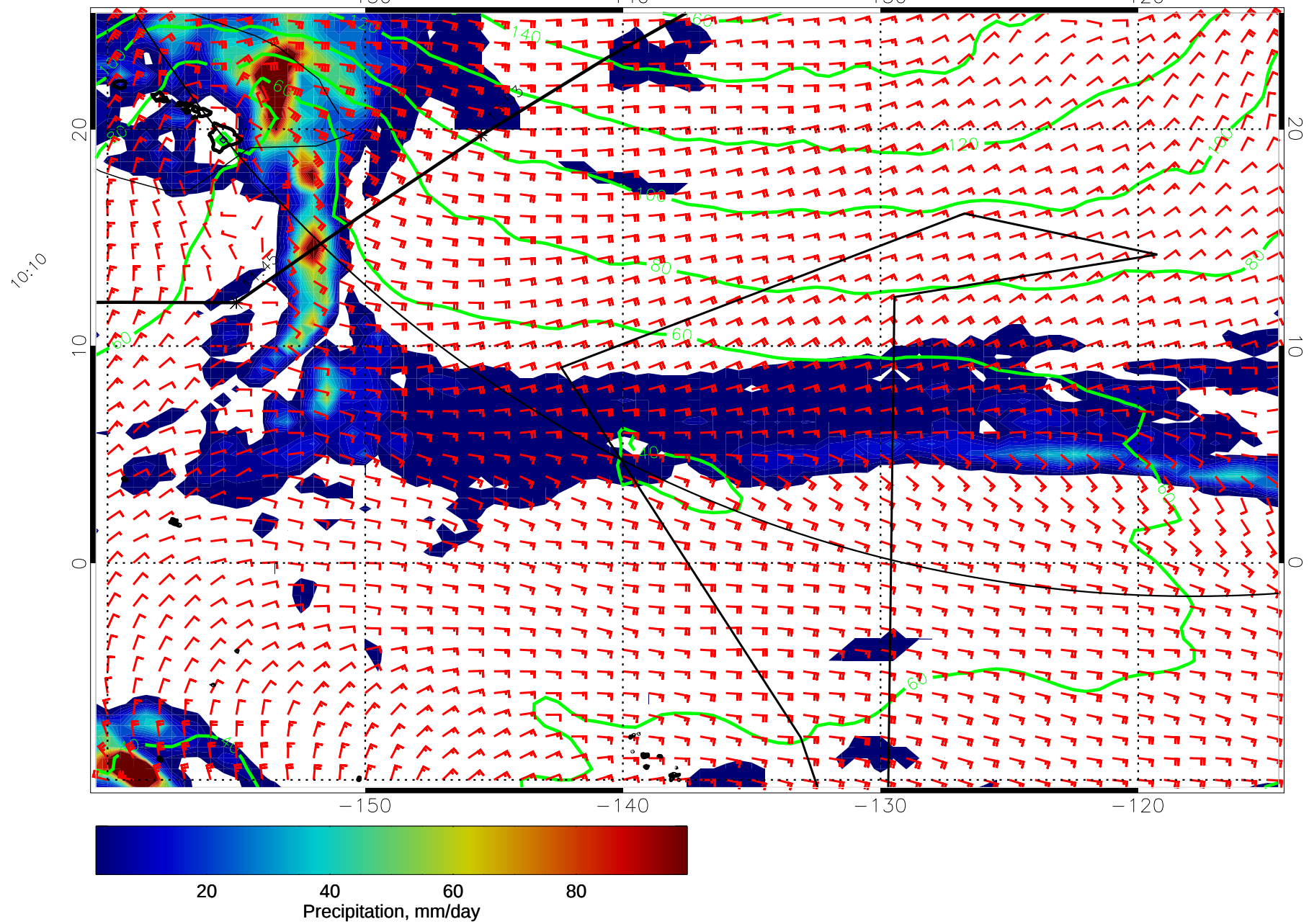
14122412, 48 hour forecast for precip, 1000mb Z, and winds (knots) -- NCEP GFS
