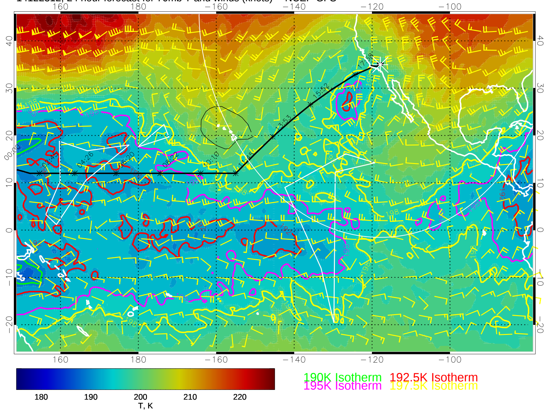
14122312, 24 hour forecast for 70mb T and winds (knots) -- NCEP GFS
