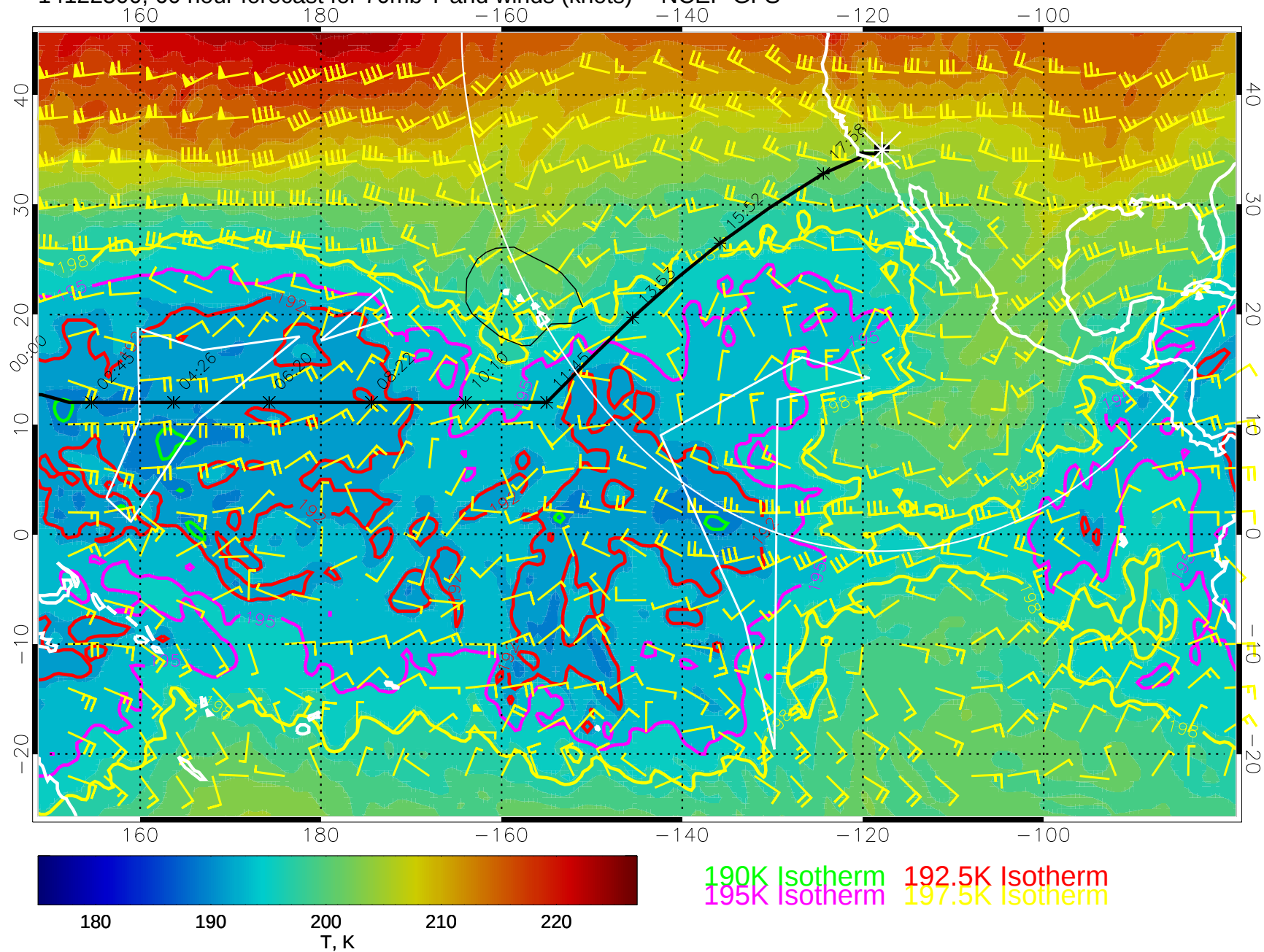
14122500, 60 hour forecast for 70mb T and winds (knots) -- NCEP GFS
