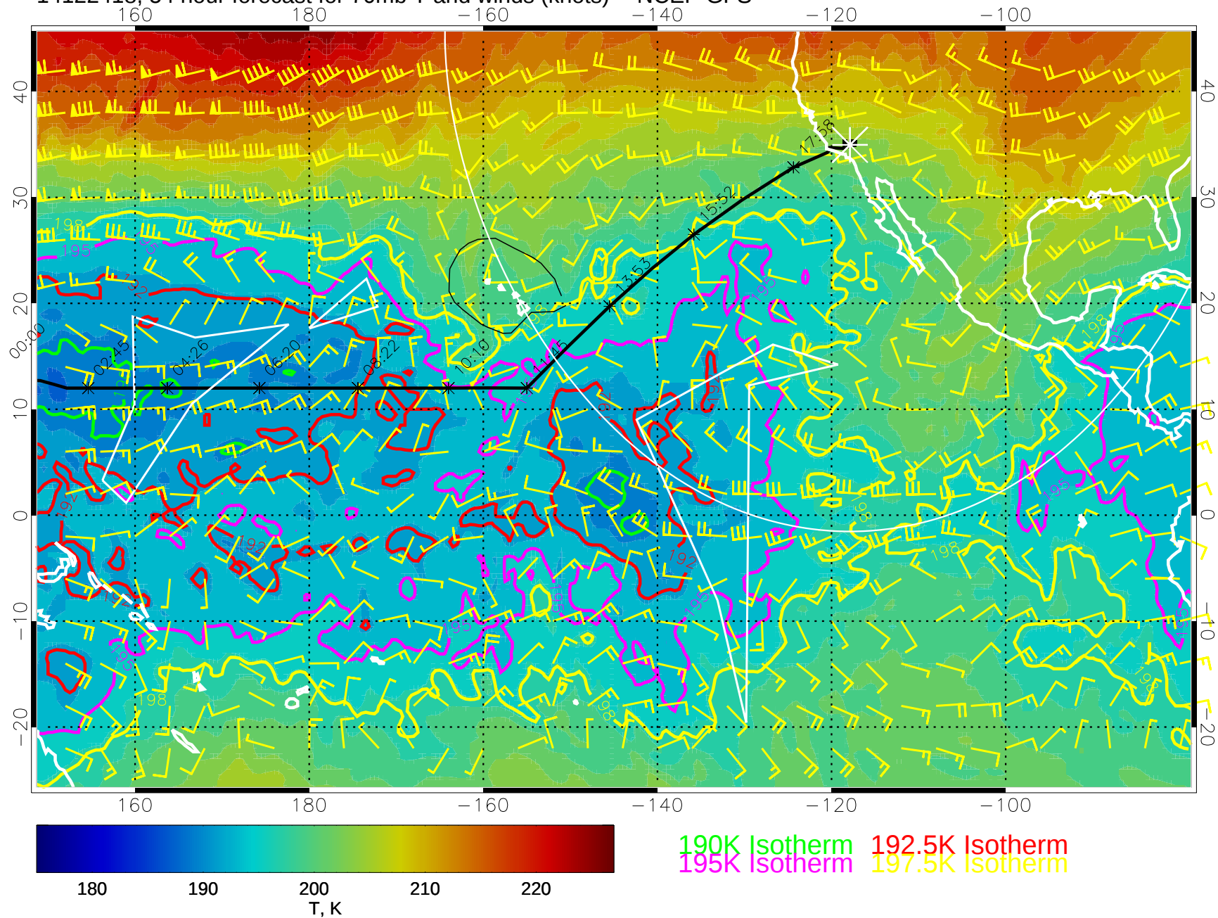
14122418, 54 hour forecast for 70mb T and winds (knots) -- NCEP GFS
