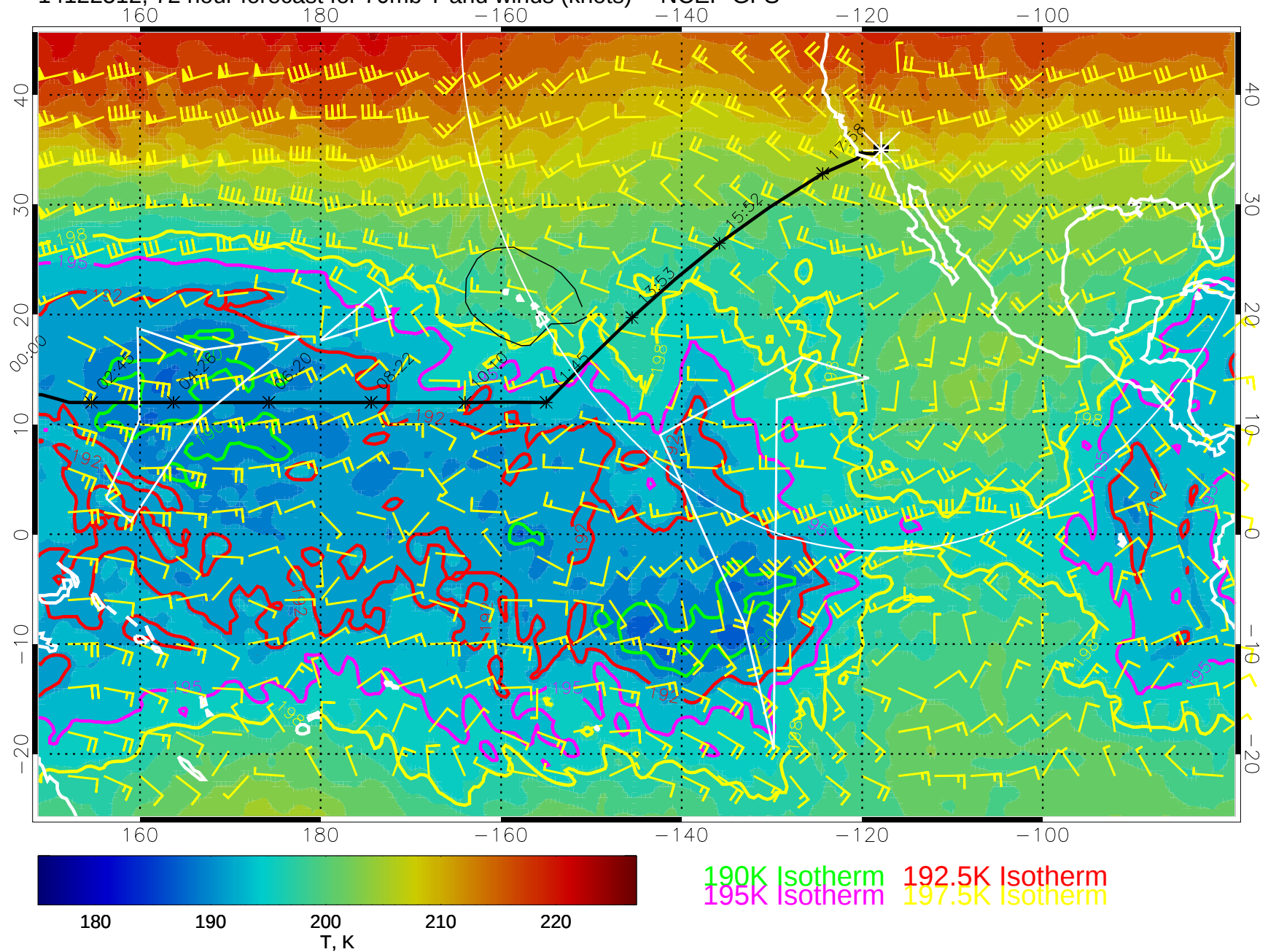
14122512, 72 hour forecast for 70mb T and winds (knots) -- NCEP GFS
