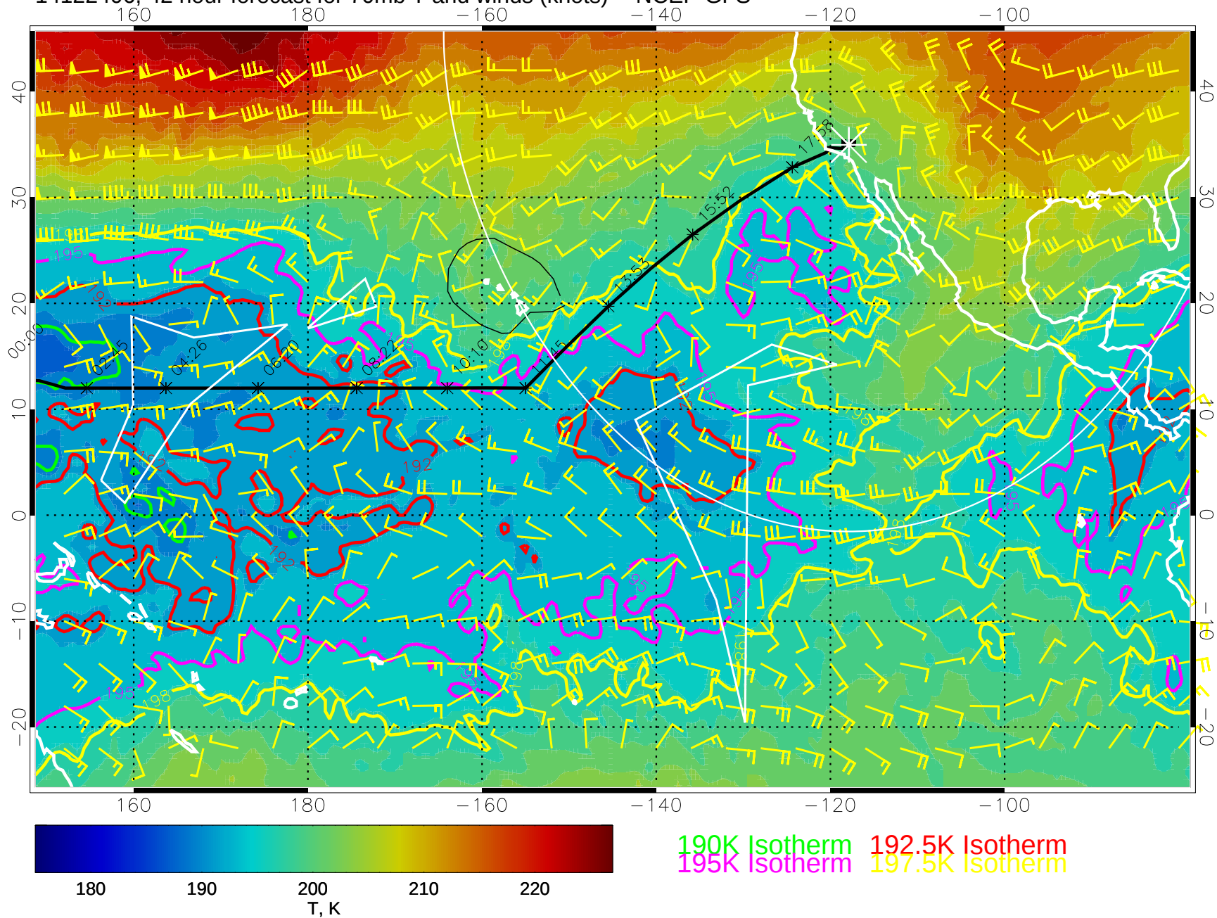
14122406, 42 hour forecast for 70mb T and winds (knots) -- NCEP GFS
