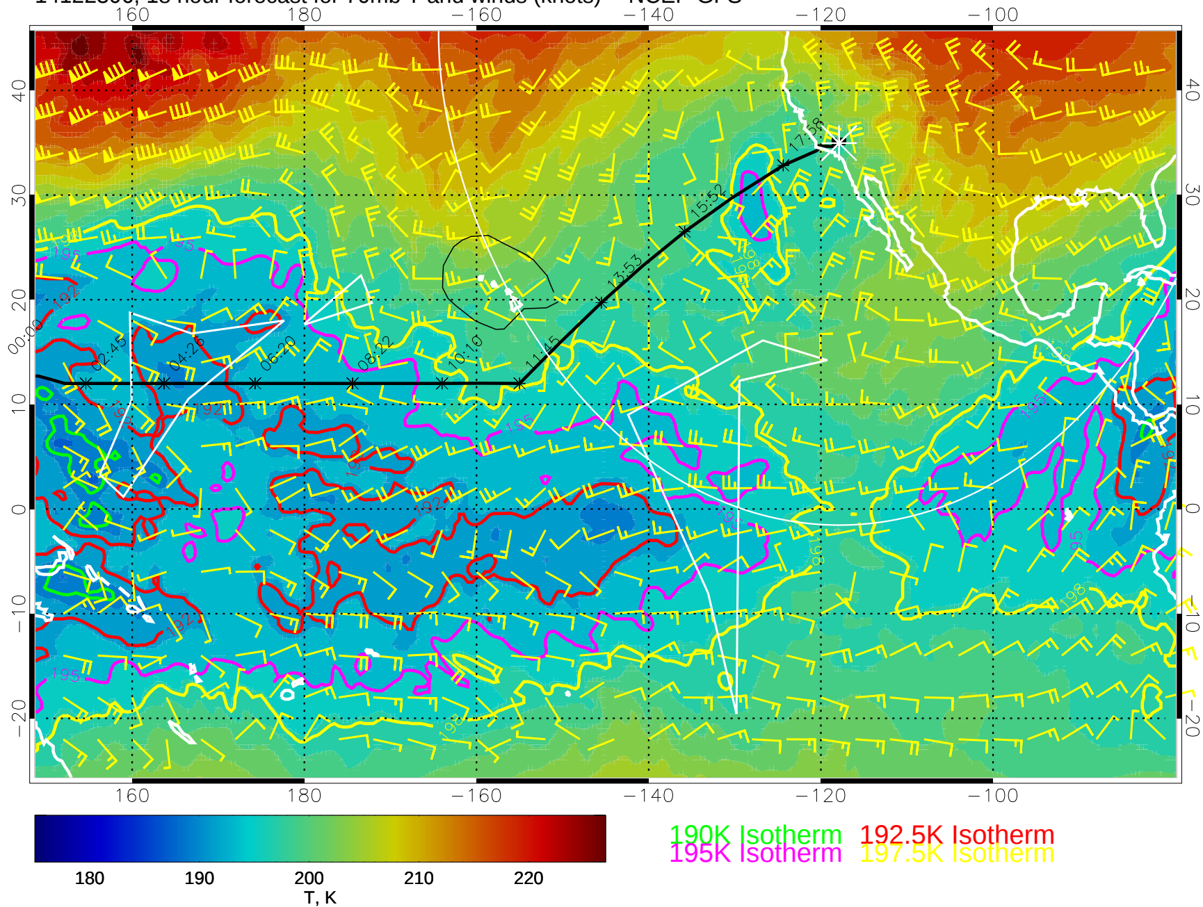
14122306, 18 hour forecast for 70mb T and winds (knots) -- NCEP GFS
