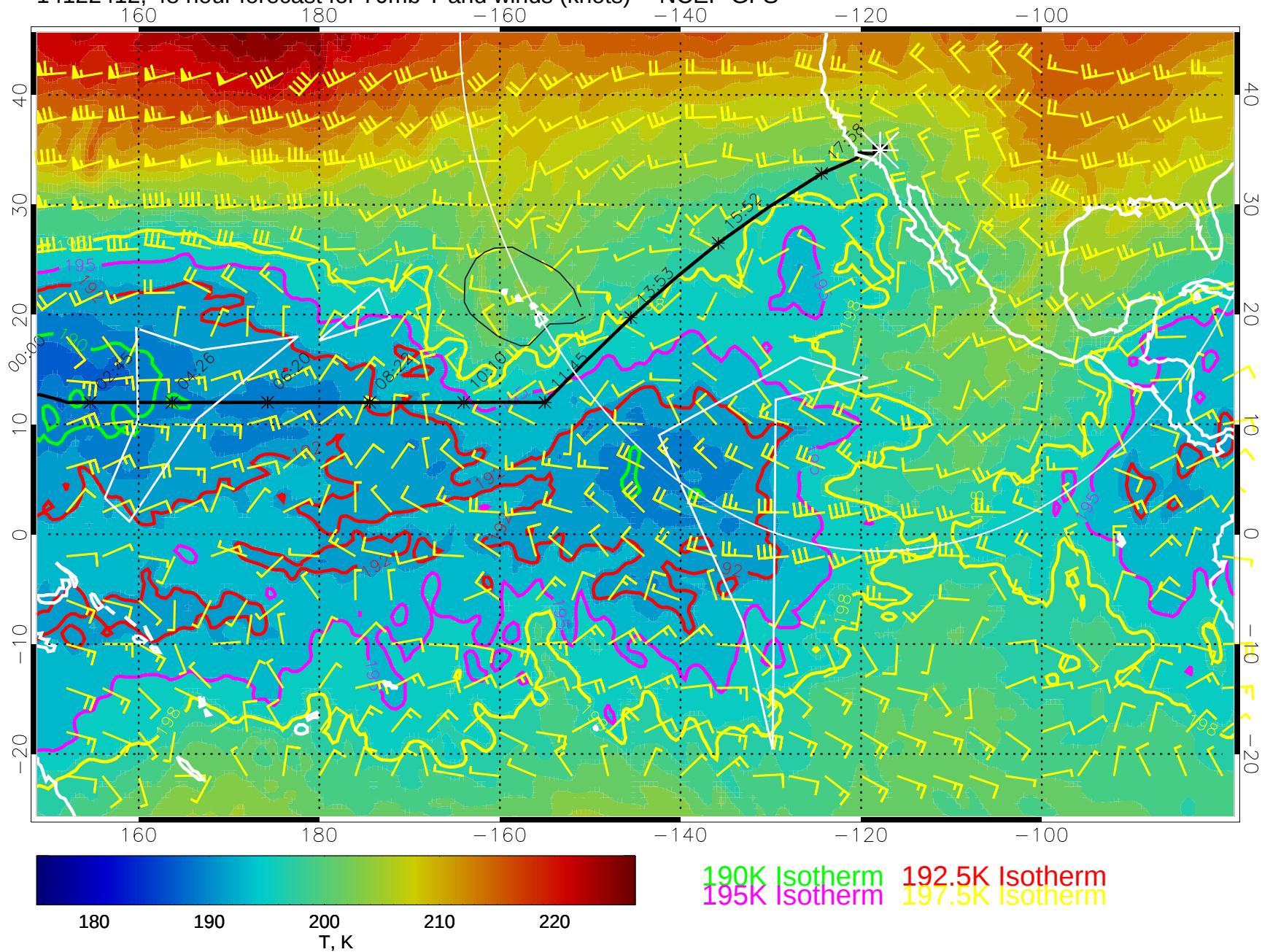
14122412, 48 hour forecast for 70mb T and winds (knots) -- NCEP GFS
