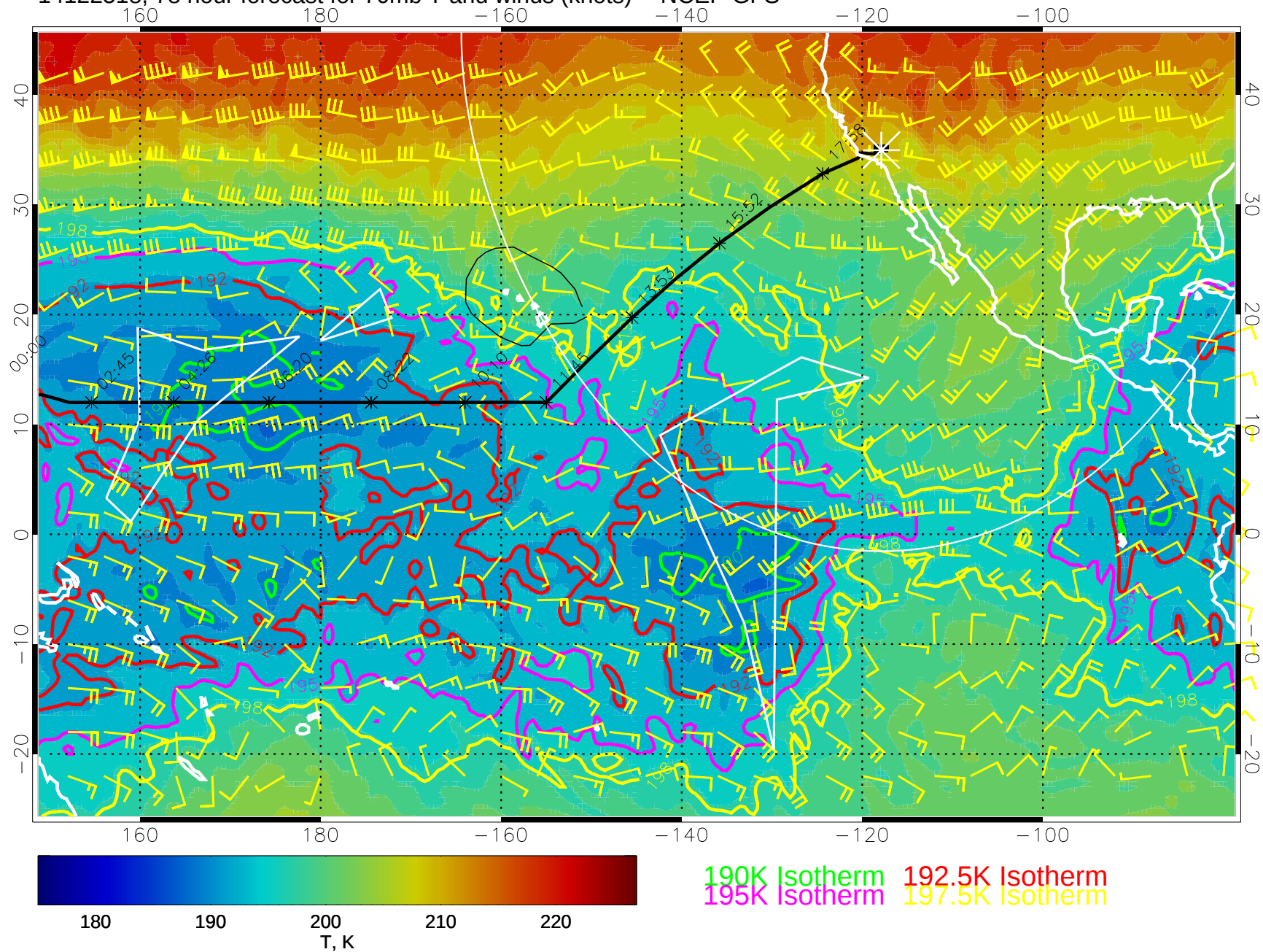
14122518, 78 hour forecast for 70mb T and winds (knots) -- NCEP GFS
