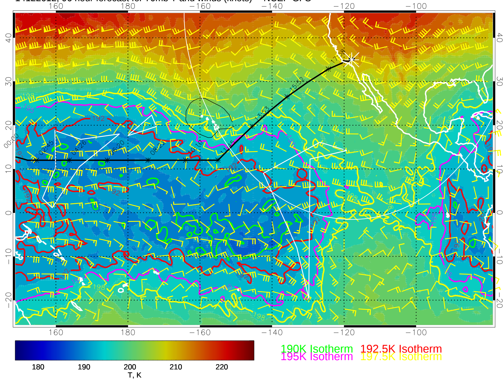
14122612, 96 hour forecast for 70mb T and winds (knots) -- NCEP GFS
