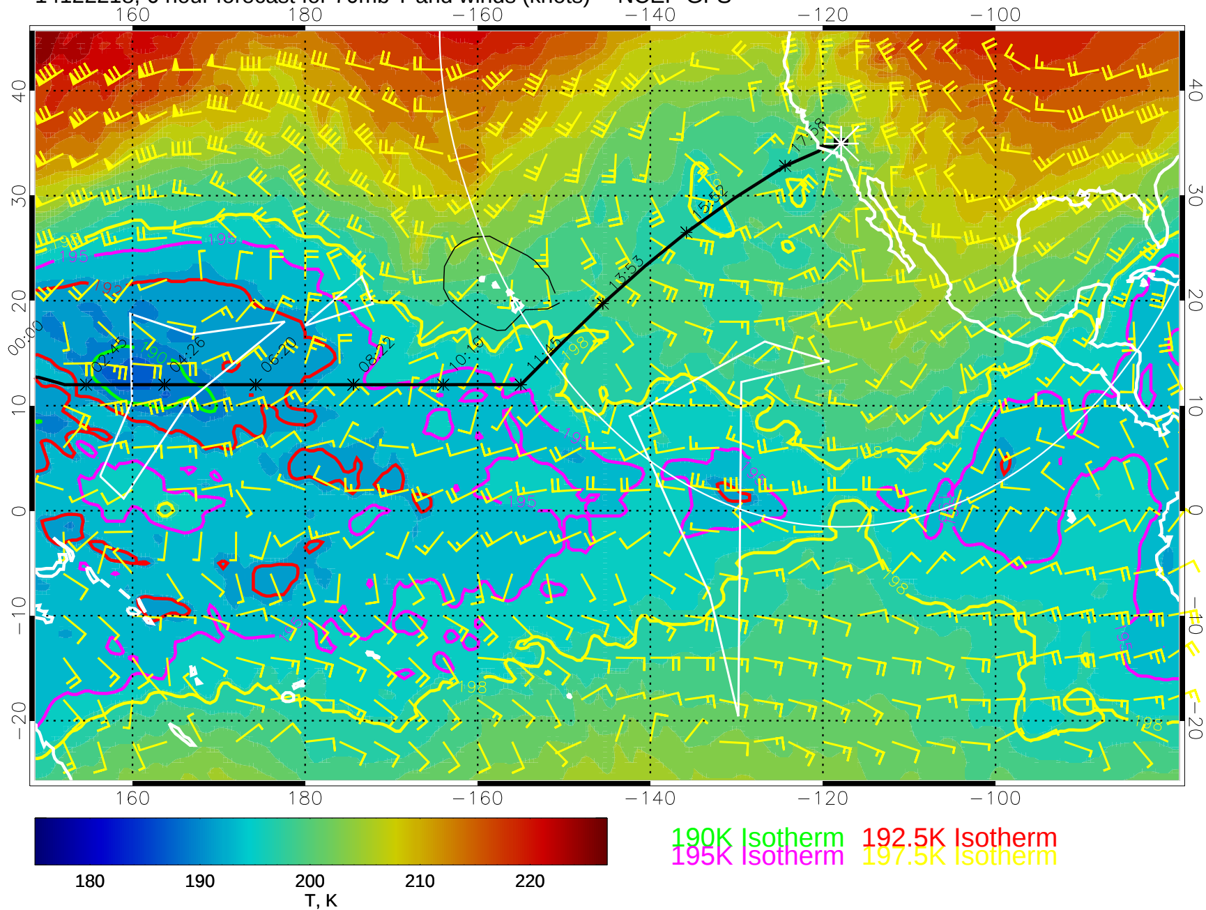
14122218, 6 hour forecast for 70mb T and winds (knots) -- NCEP GFS
