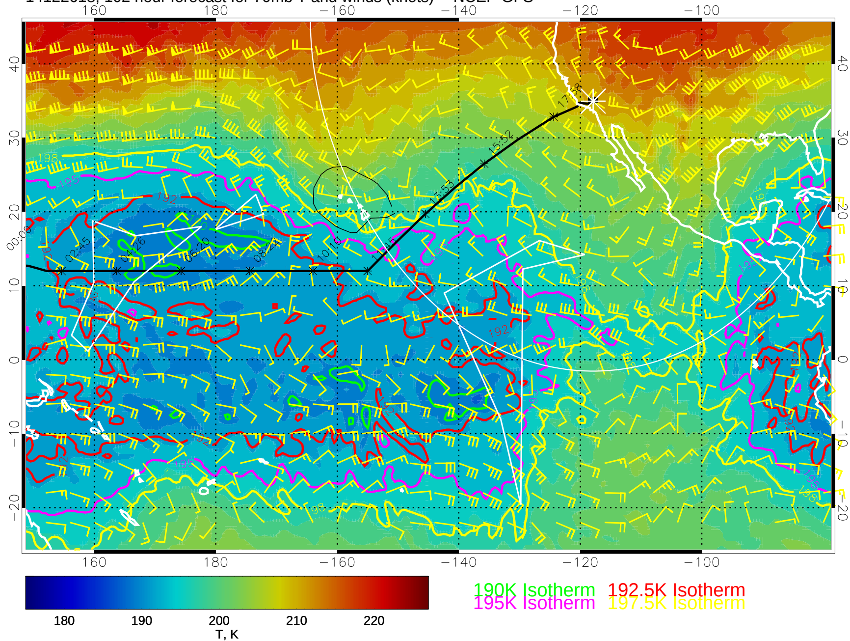
14122618, 102 hour forecast for 70mb T and winds (knots) -- NCEP GFS
