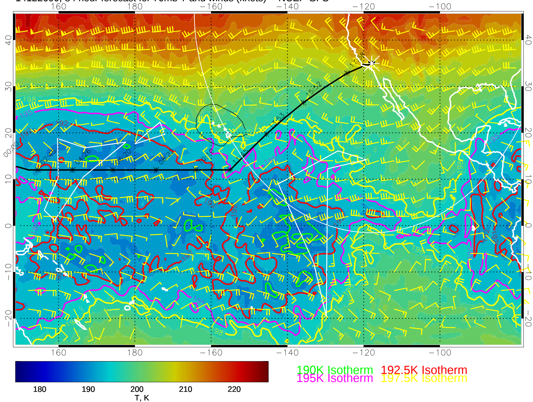
14122600, 84 hour forecast for 70mb T and winds (knots) -- NCEP GFS
