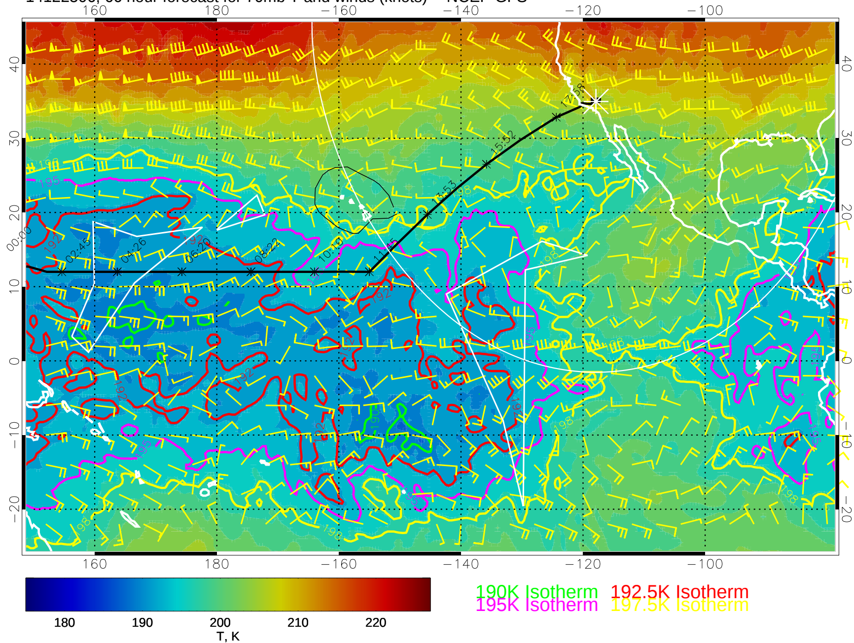
14122506, 66 hour forecast for 70mb T and winds (knots) -- NCEP GFS
