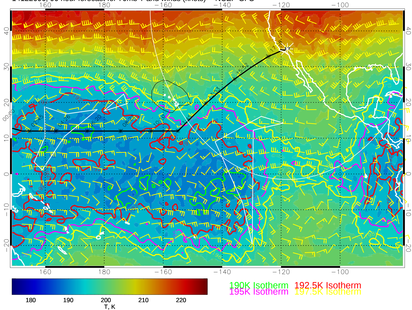
14122606, 90 hour forecast for 70mb T and winds (knots) -- NCEP GFS
