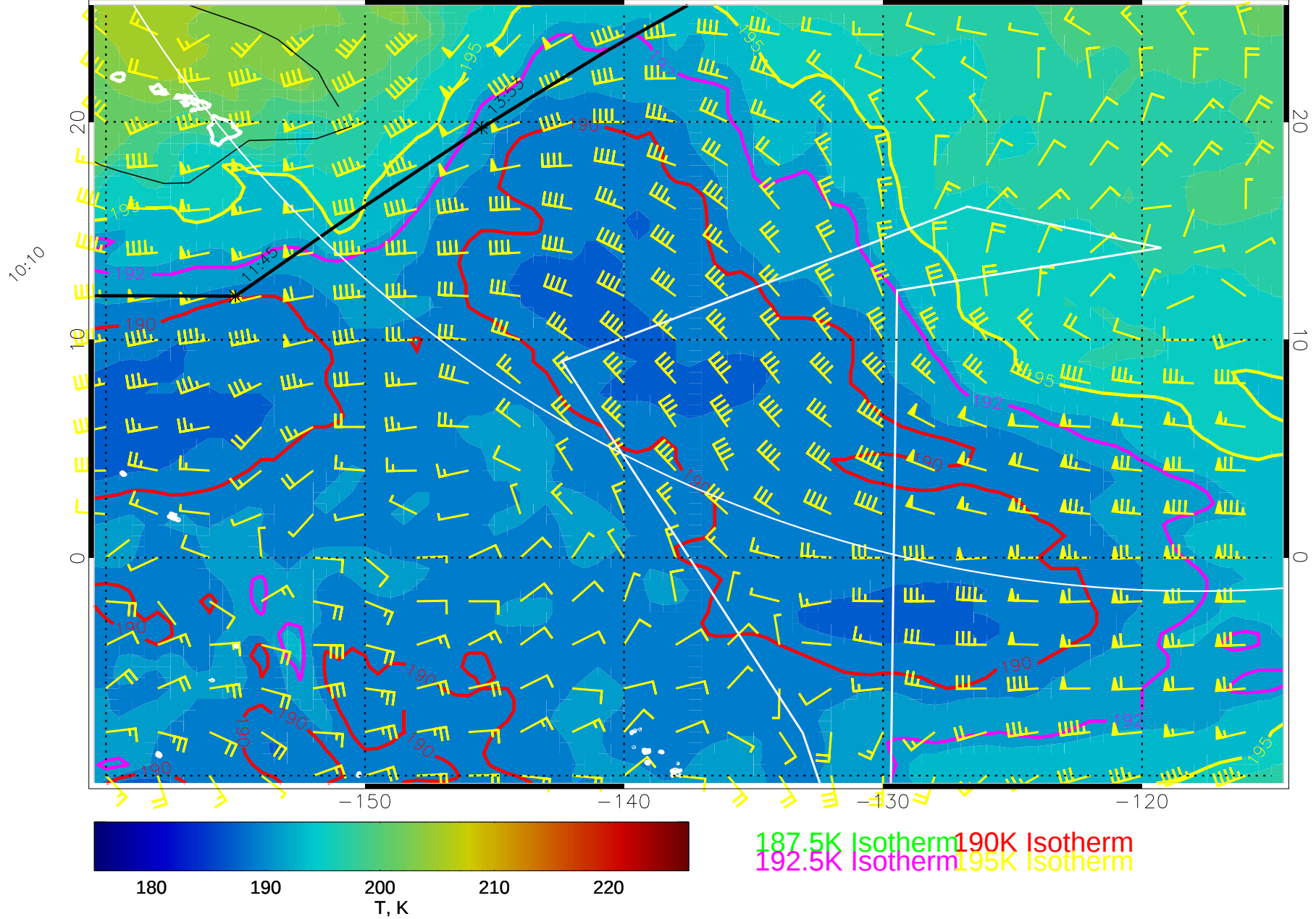
14122418, 54 hour forecast for 100mb T and winds (knots) -- NCEP GFS
