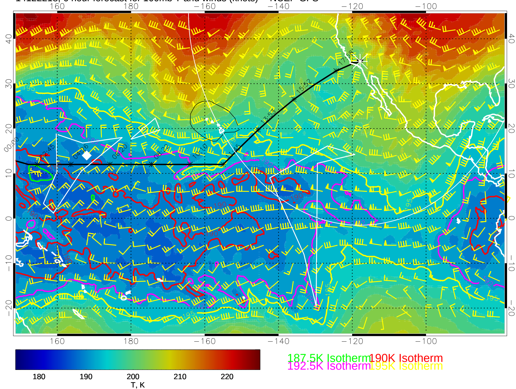
14122218, 6 hour forecast for 100mb T and winds (knots) -- NCEP GFS
