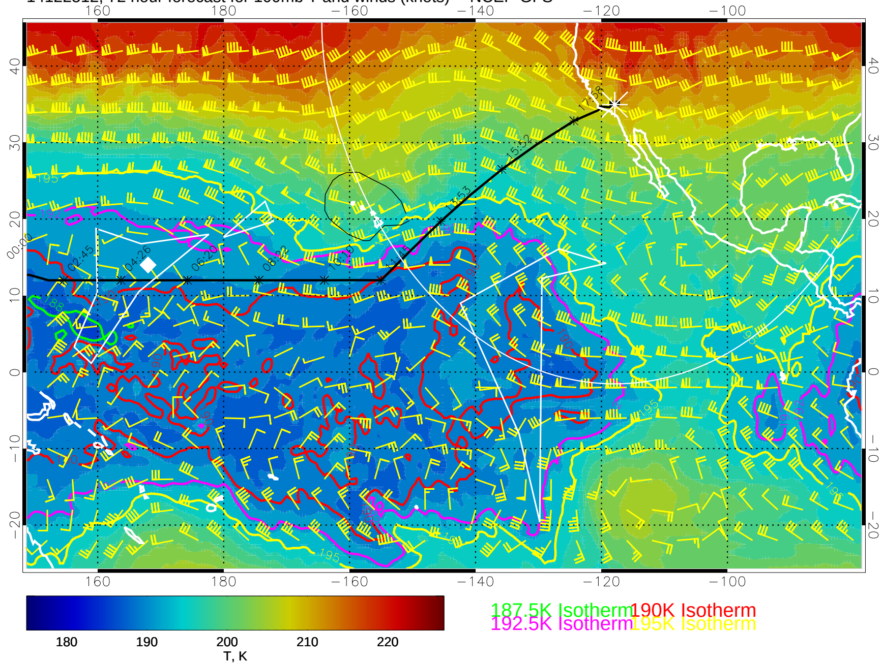
14122512, 72 hour forecast for 100mb T and winds (knots) -- NCEP GFS
