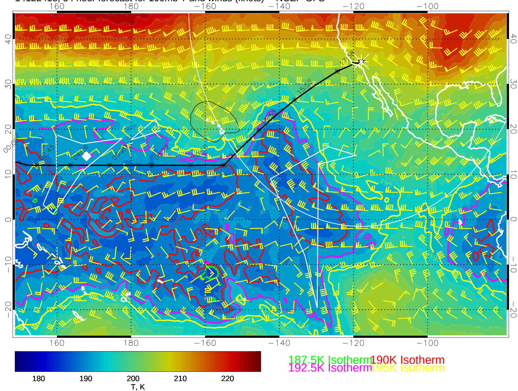
14122418, 54 hour forecast for 100mb T and winds (knots) -- NCEP GFS
