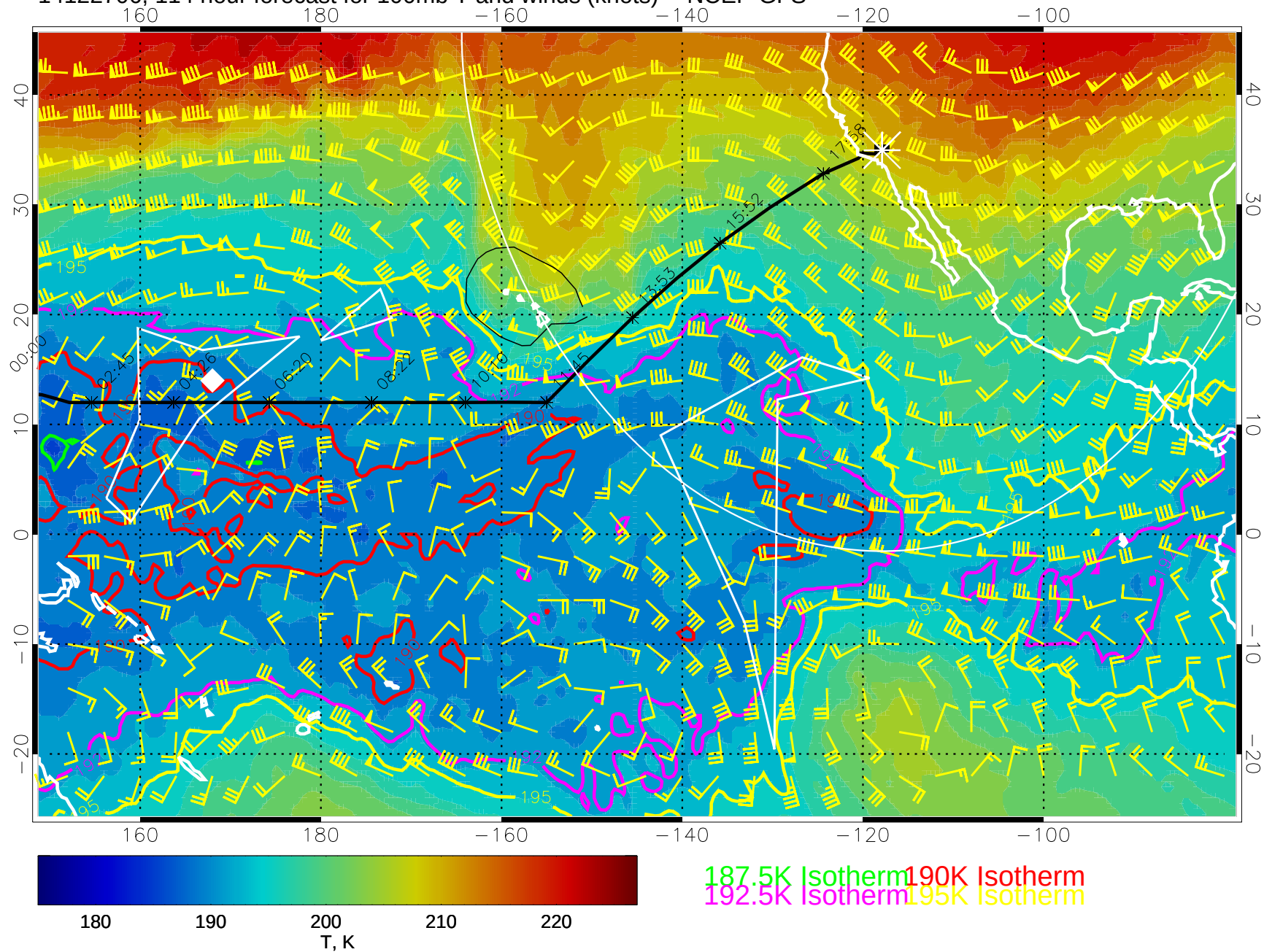
14122706, 114 hour forecast for 100mb T and winds (knots) -- NCEP GFS
