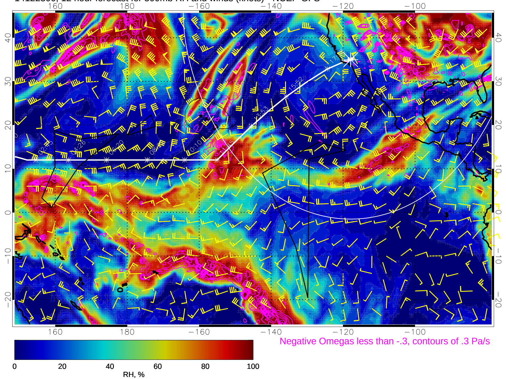
14122300, 12 hour forecast for 500mb RH and winds (knots) - NCEP GFS
