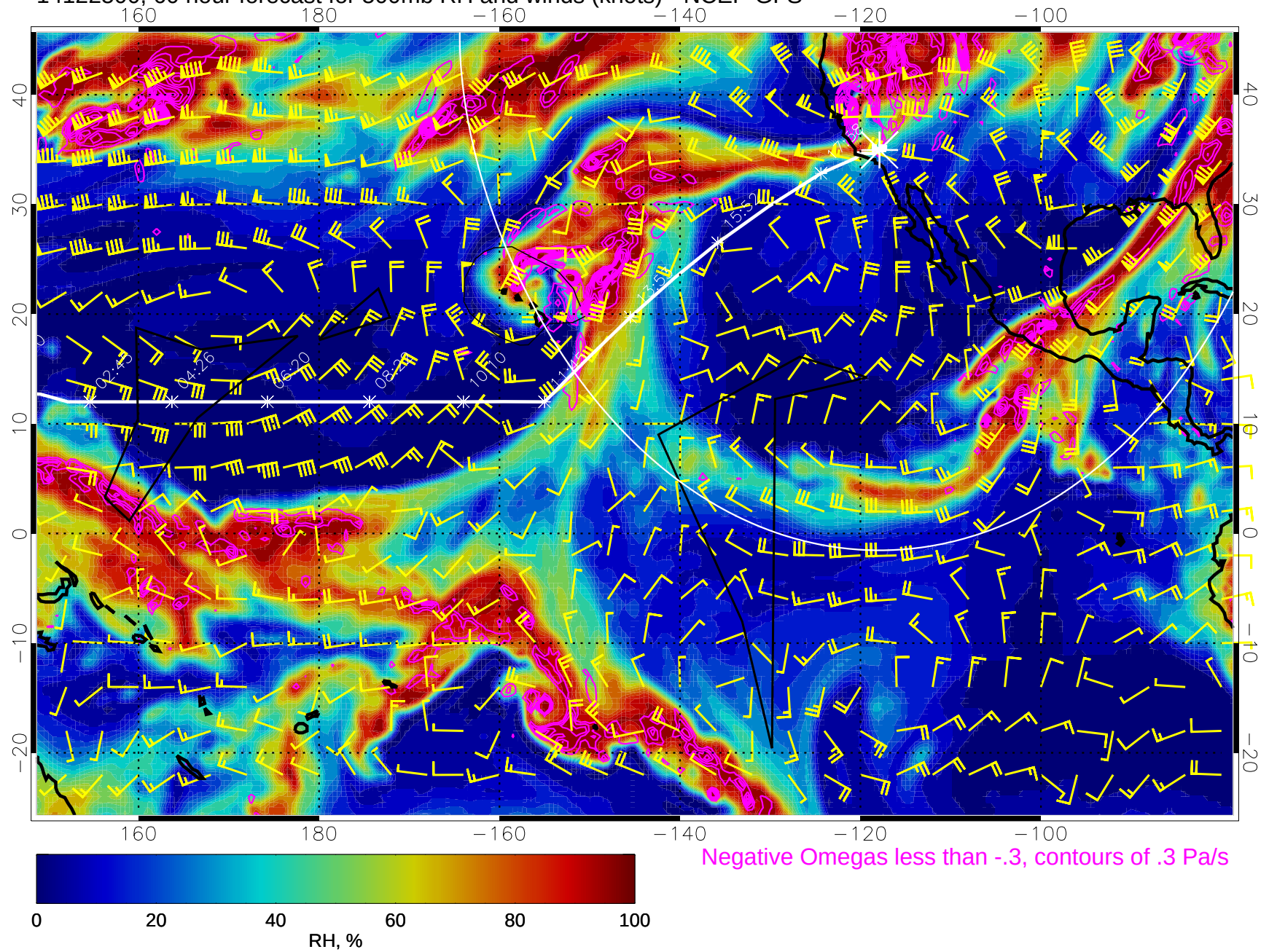
14122500, 60 hour forecast for 500mb RH and winds (knots) - NCEP GFS
