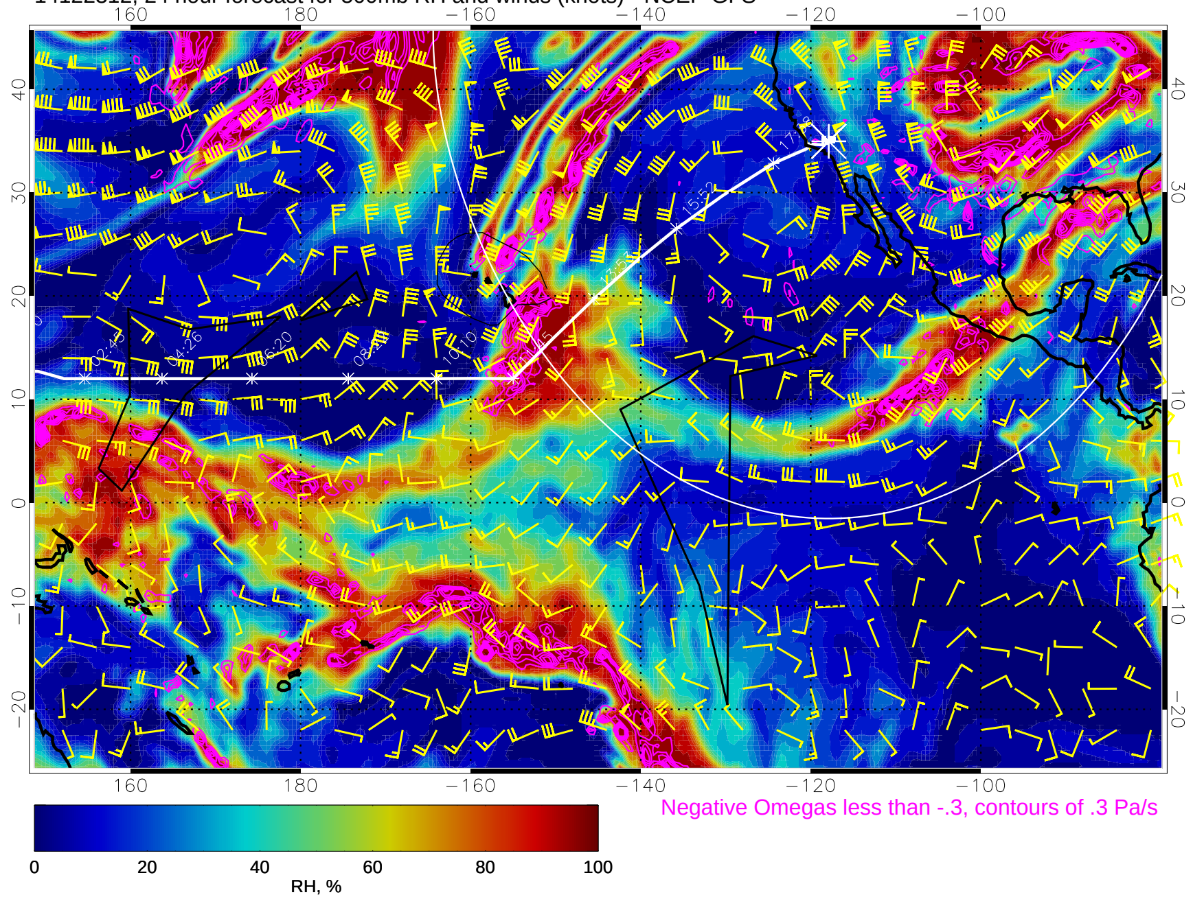
14122312, 24 hour forecast for 500mb RH and winds (knots) - NCEP GFS
