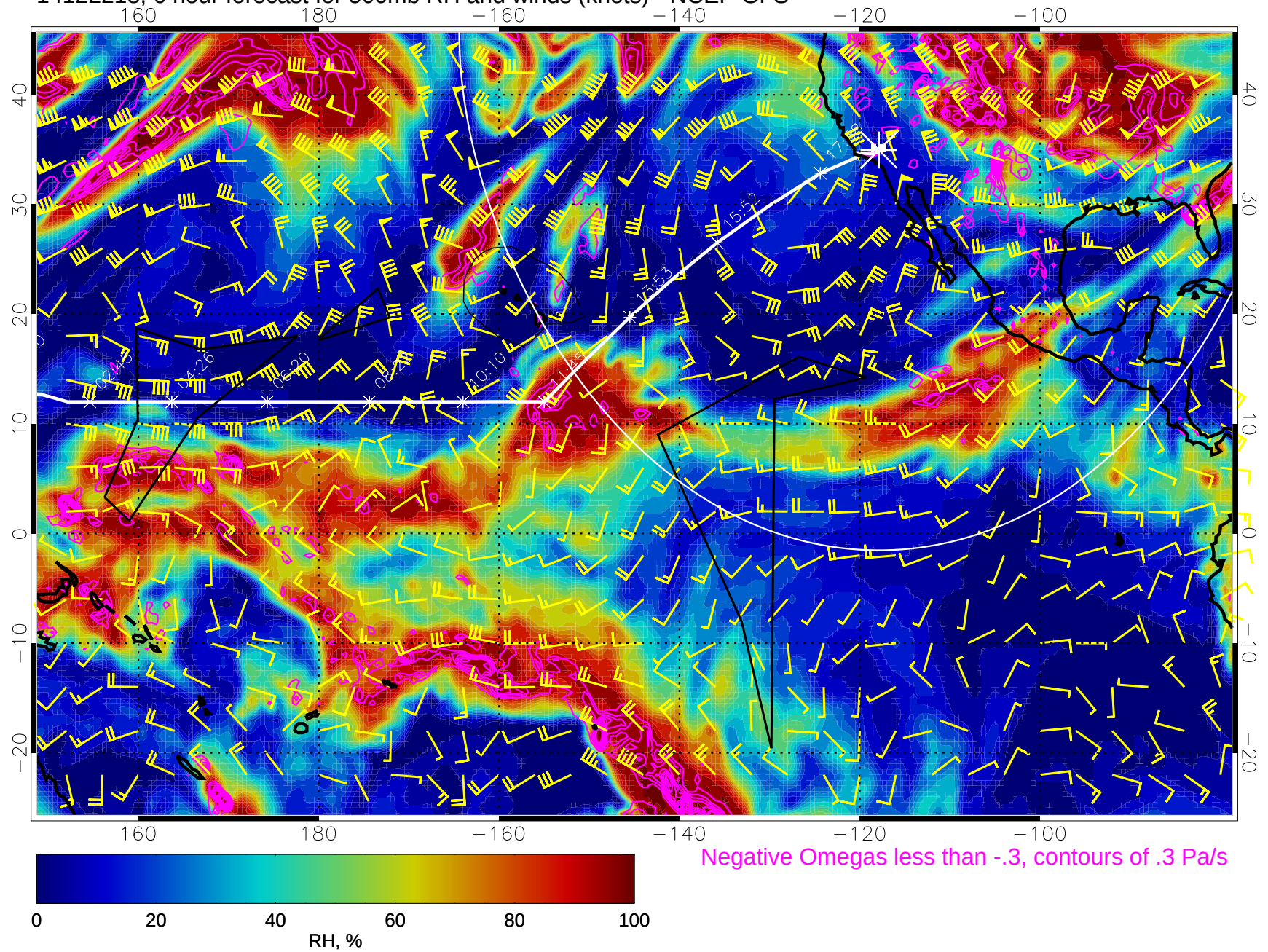
14122218, 6 hour forecast for 500mb RH and winds (knots) - NCEP GFS
