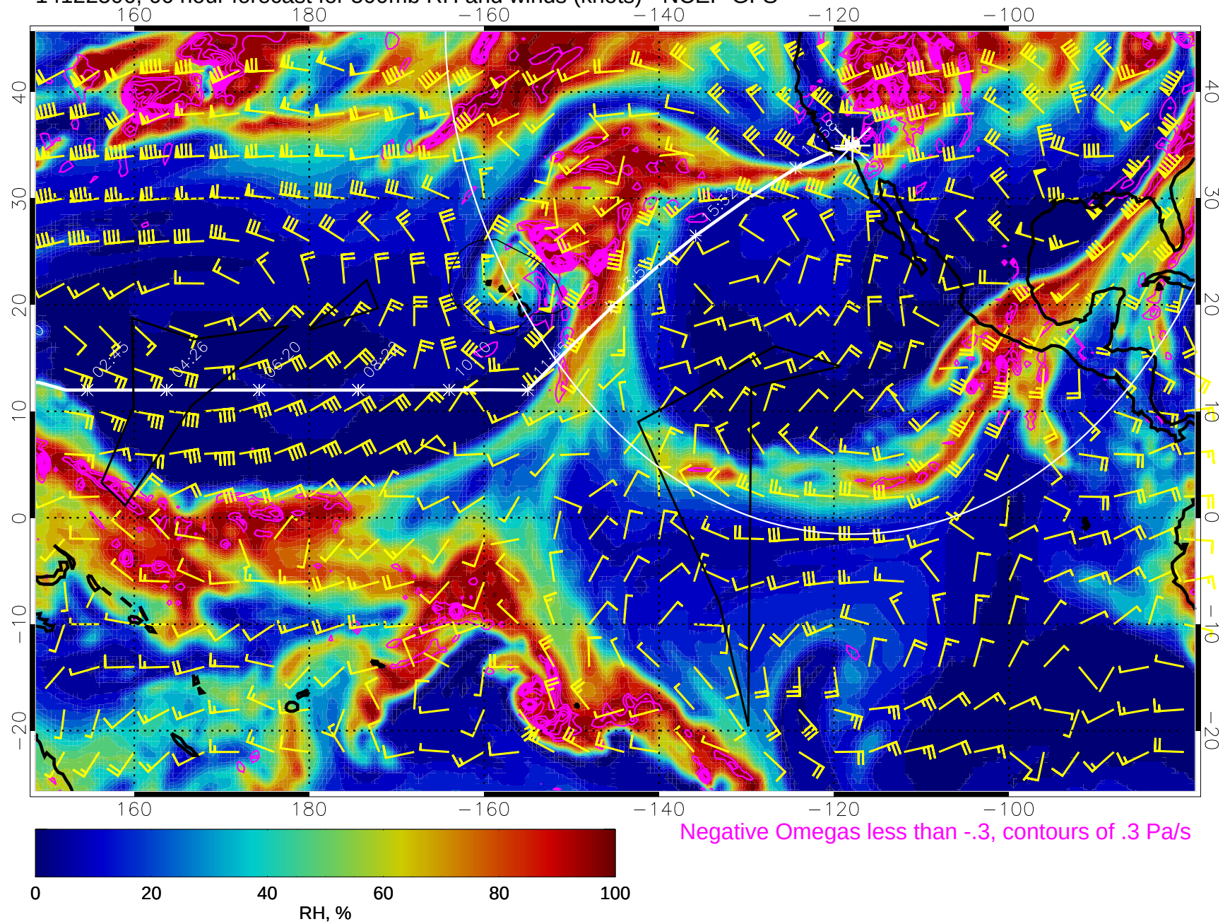
14122506, 66 hour forecast for 500mb RH and winds (knots) - NCEP GFS
