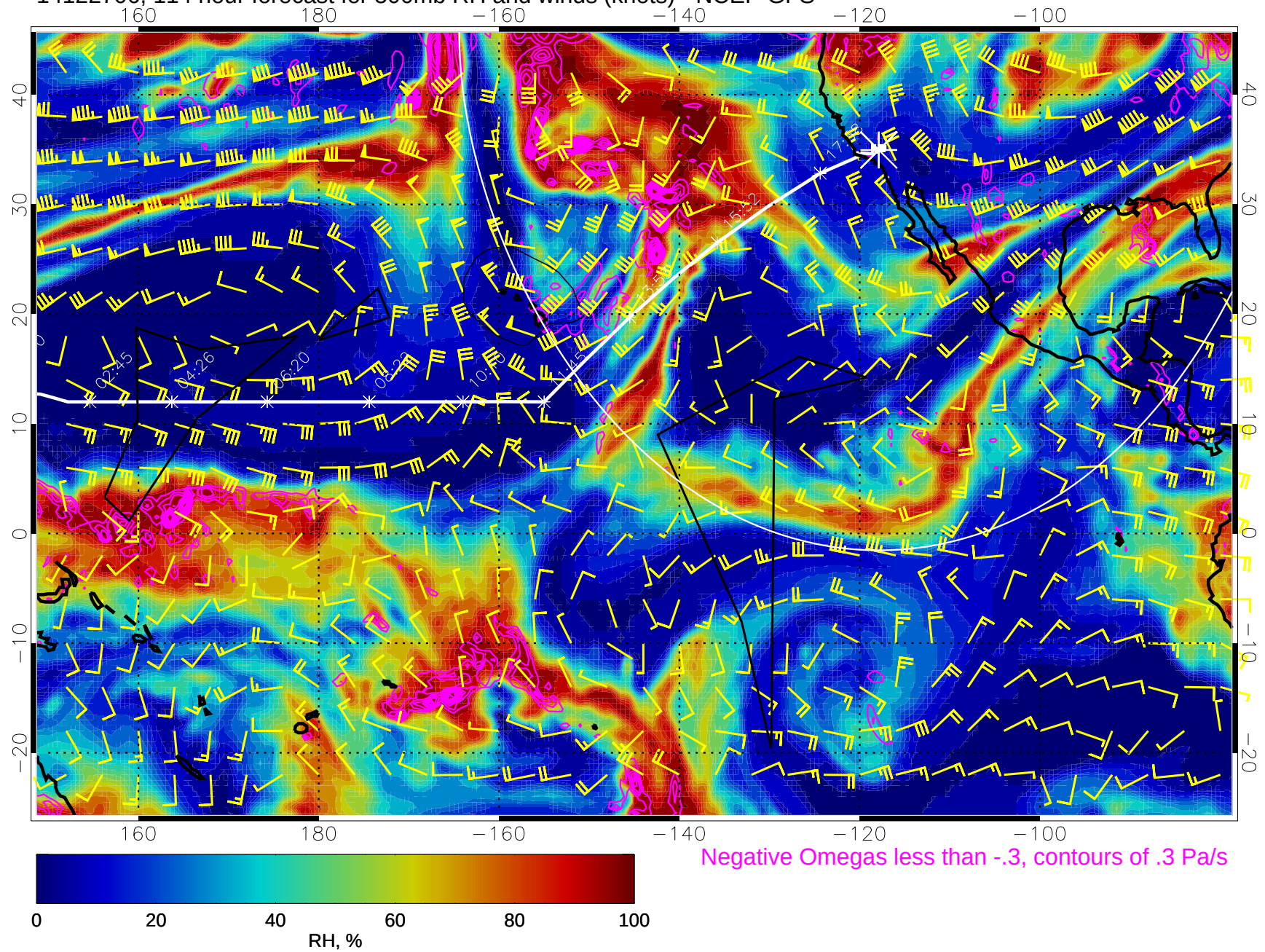
14122706, 114 hour forecast for 500mb RH and winds (knots) - NCEP GFS
