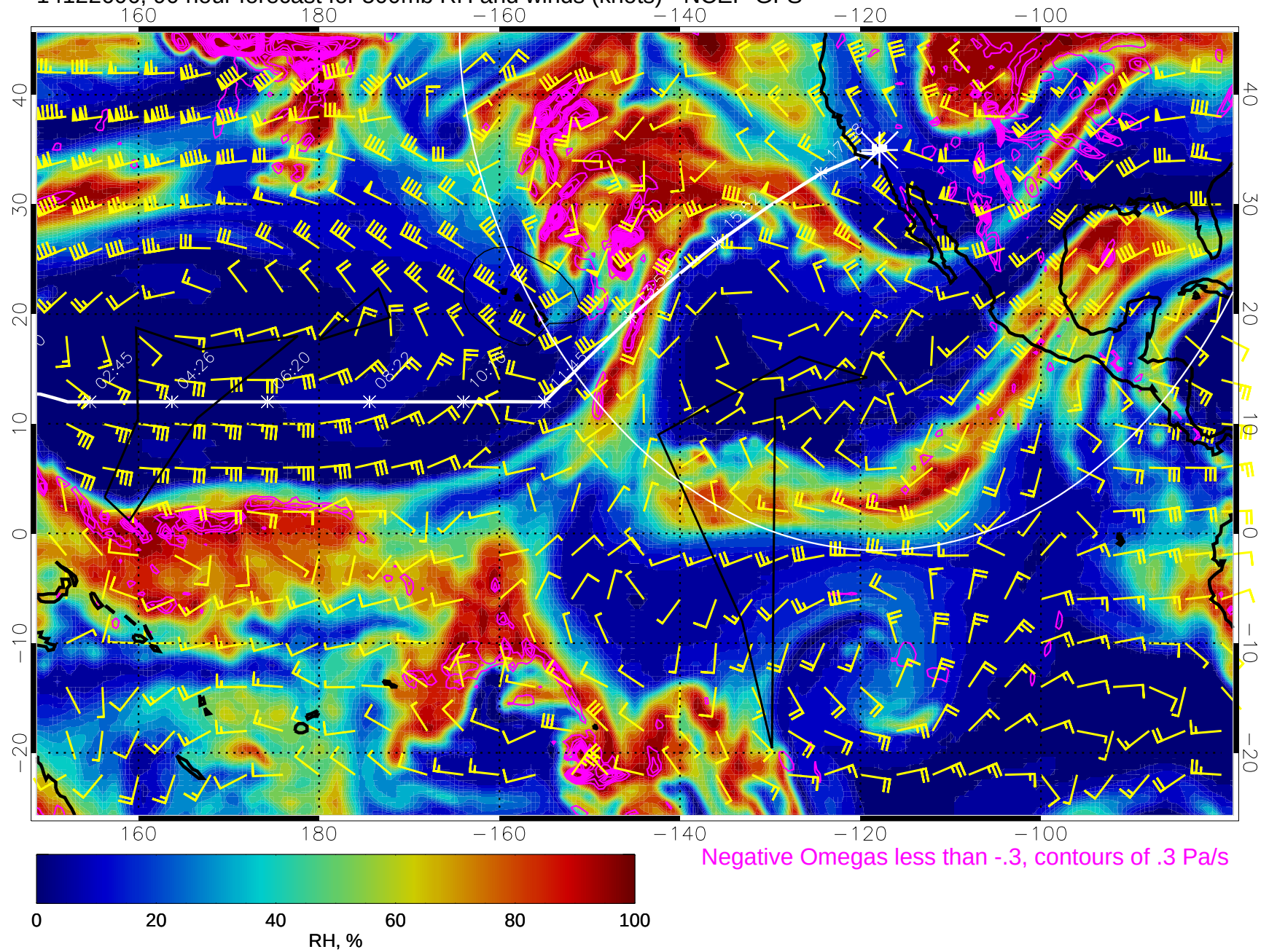
14122606, 90 hour forecast for 500mb RH and winds (knots) - NCEP GFS
