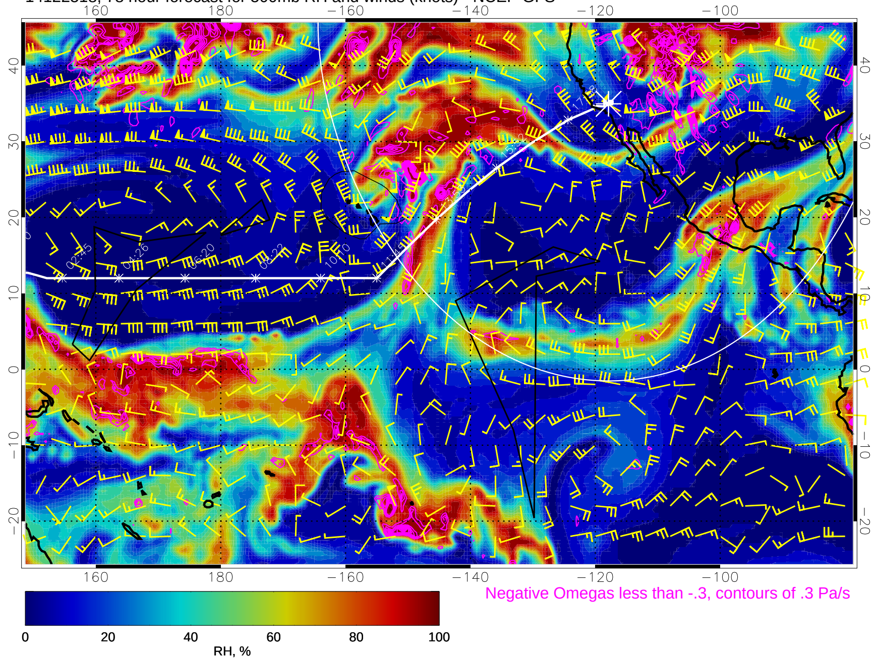
14122518, 78 hour forecast for 500mb RH and winds (knots) - NCEP GFS
