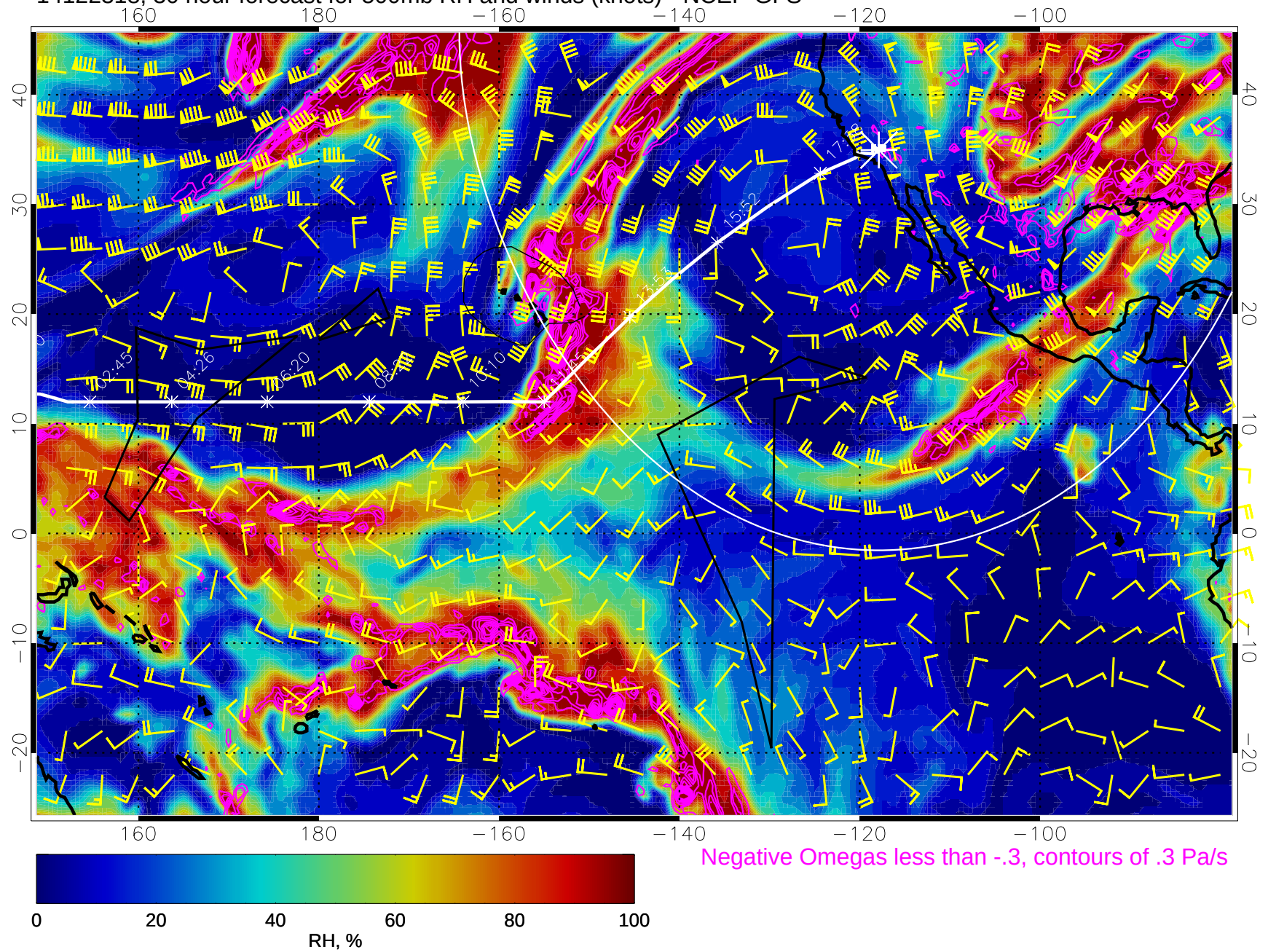
14122318, 30 hour forecast for 500mb RH and winds (knots) - NCEP GFS
