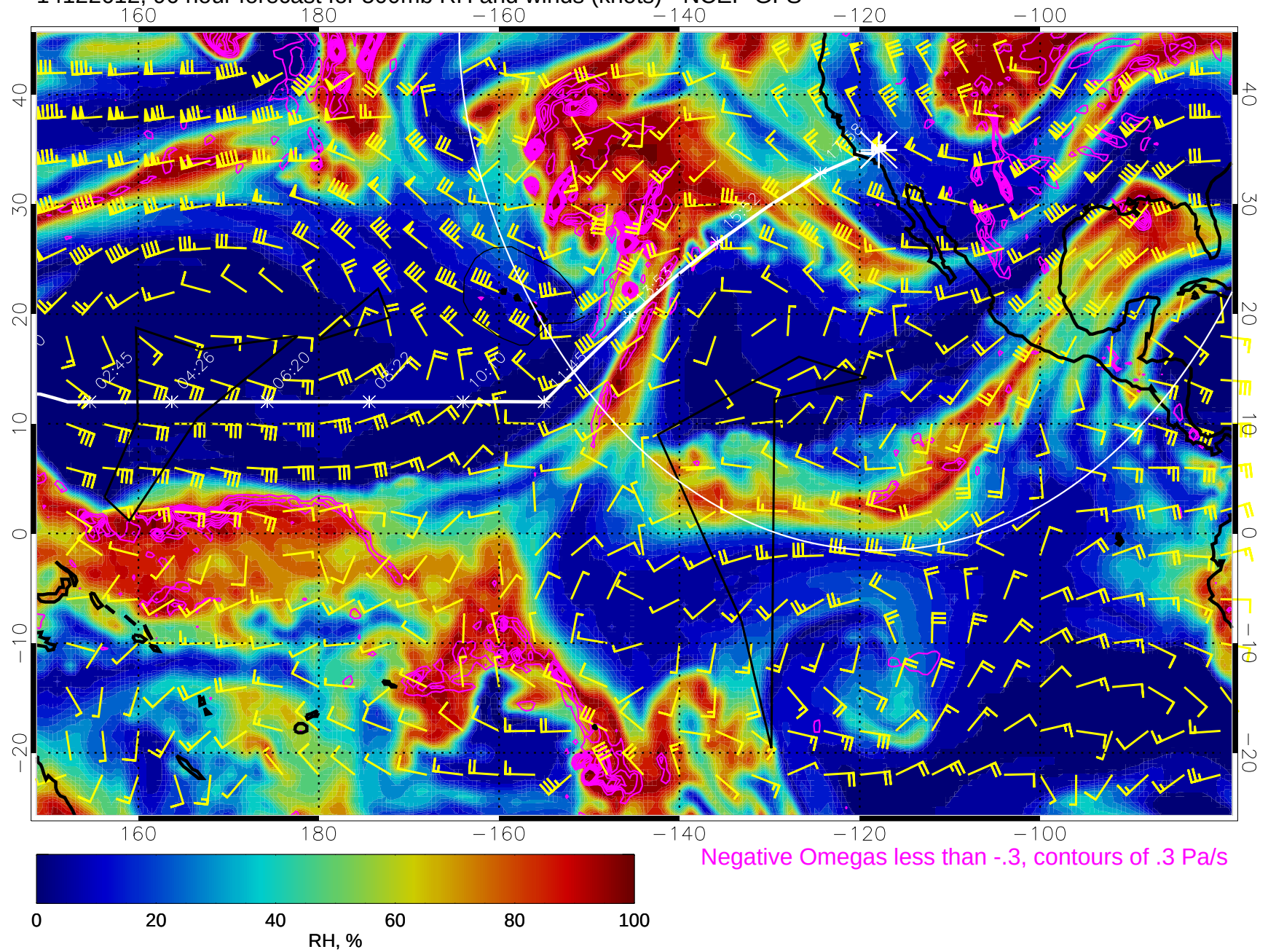
14122612, 96 hour forecast for 500mb RH and winds (knots) - NCEP GFS
