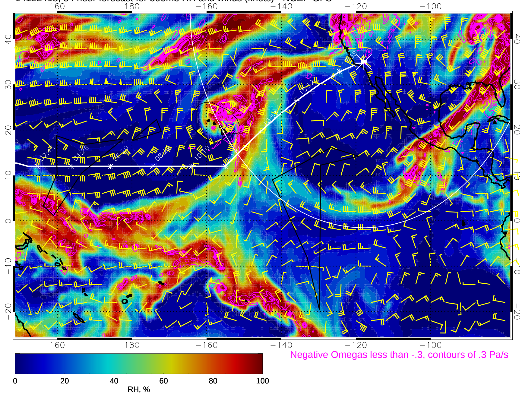
14122418, 54 hour forecast for 500mb RH and winds (knots) - NCEP GFS
