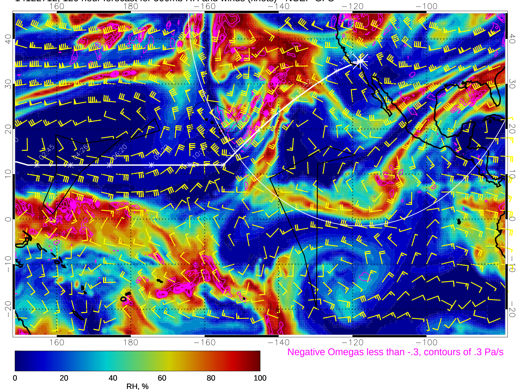
14122712, 120 hour forecast for 500mb RH and winds (knots) - NCEP GFS
