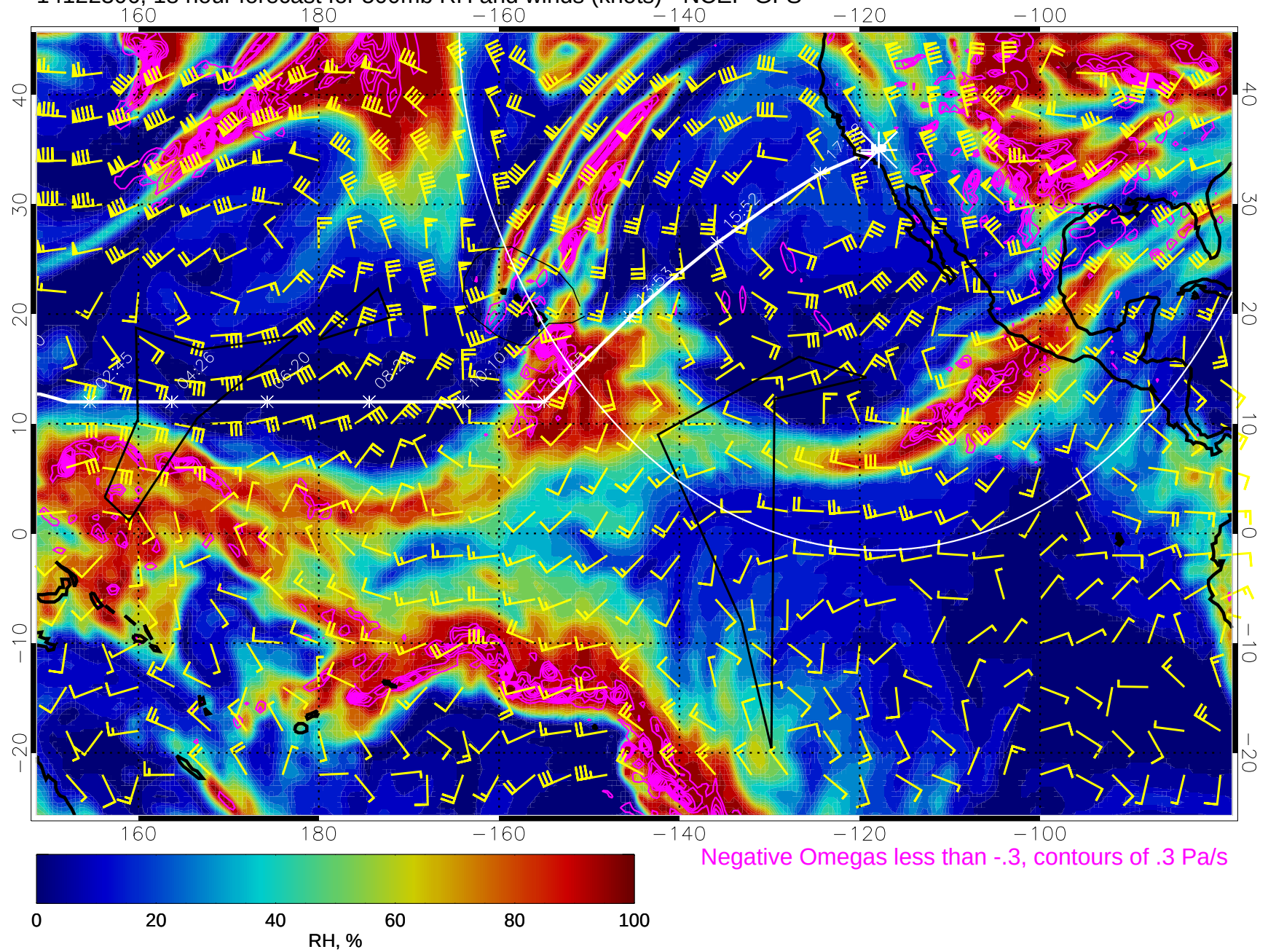
14122306, 18 hour forecast for 500mb RH and winds (knots) - NCEP GFS
