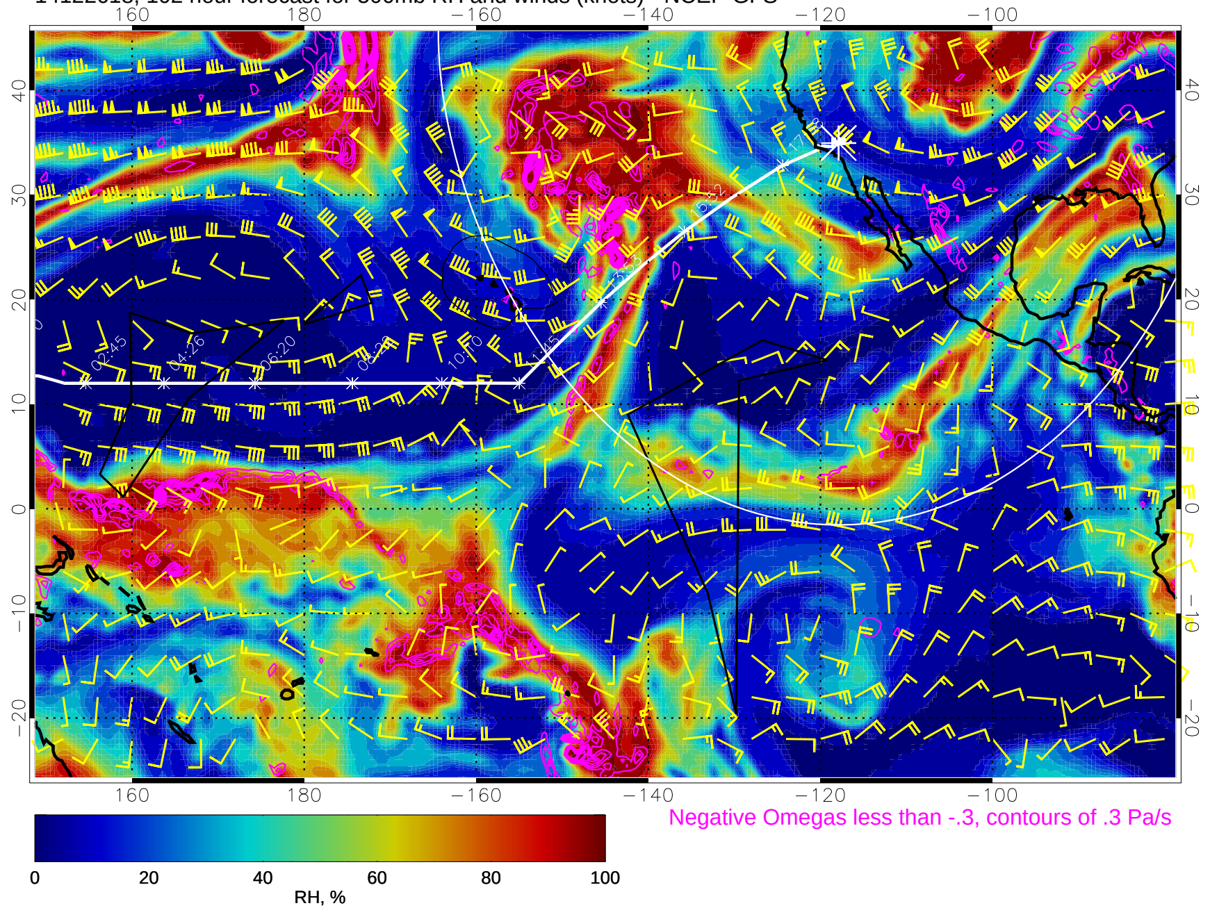
14122618, 102 hour forecast for 500mb RH and winds (knots) - NCEP GFS
