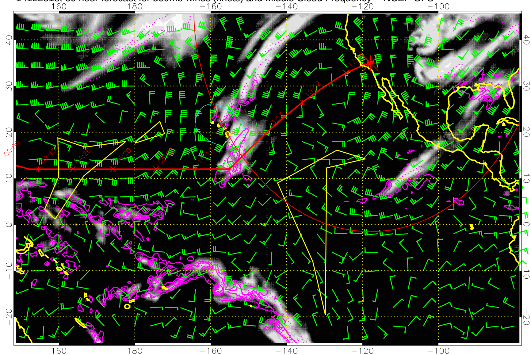
14122318, 30 hour forecast for 500mb winds (knots) and Middle Cloud Frequency -- NCEP GFS
