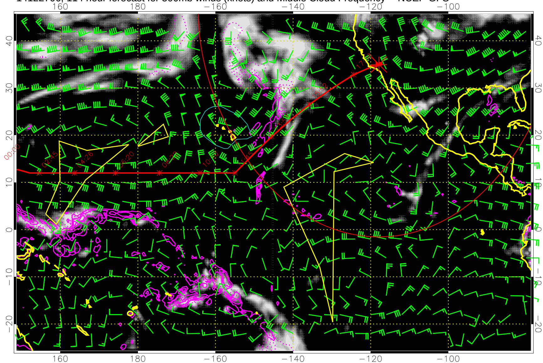
14122706, 114 hour forecast for 500mb winds (knots) and Middle Cloud Frequency -- NCEP GFS
