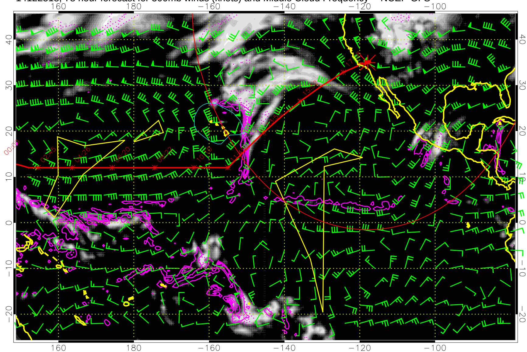
14122518, 78 hour forecast for 500mb winds (knots) and Middle Cloud Frequency -- NCEP GFS
