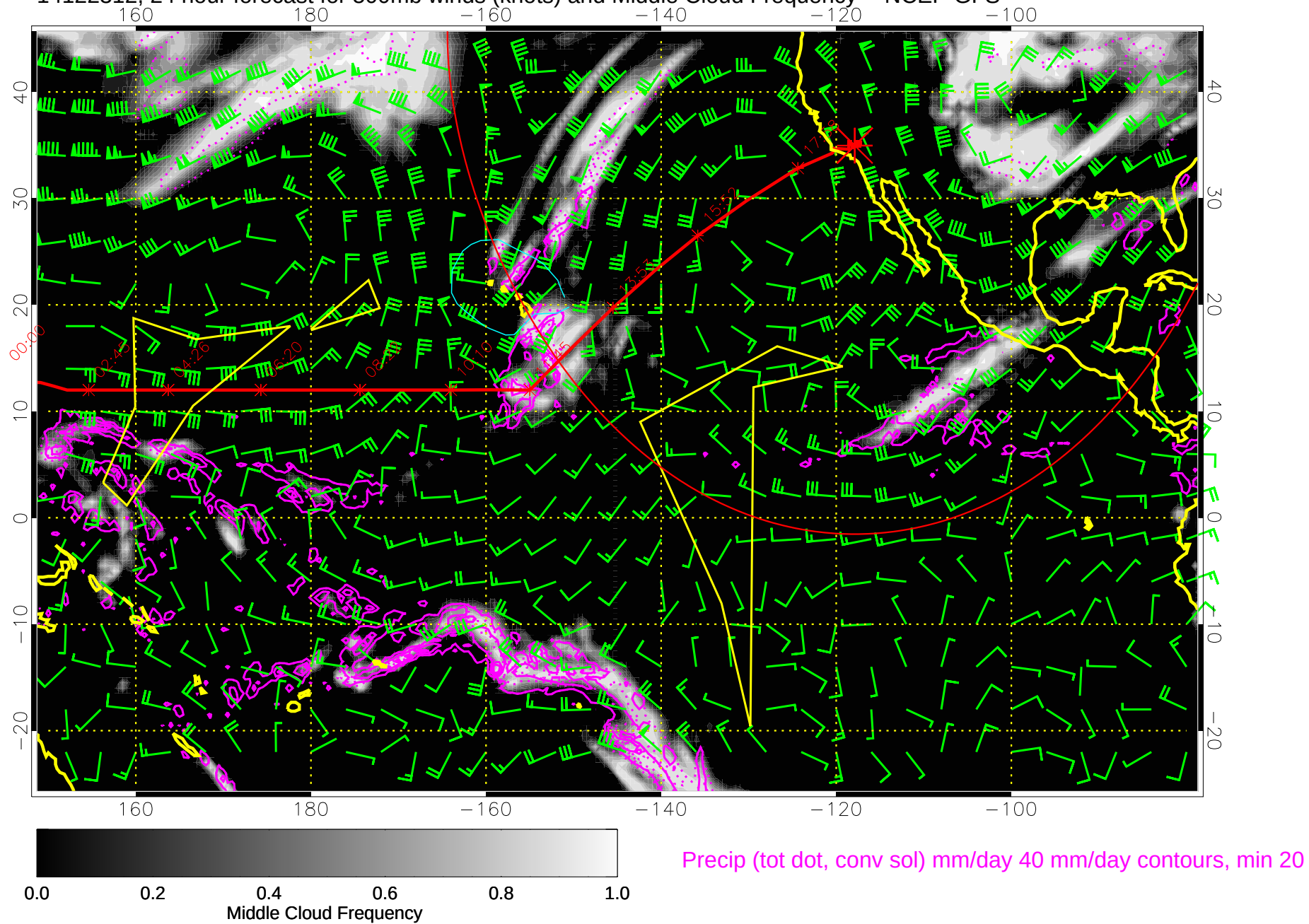
14122312, 24 hour forecast for 500mb winds (knots) and Middle Cloud Frequency -- NCEP GFS
