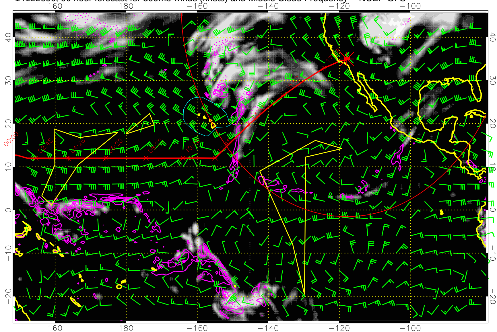
14122606, 90 hour forecast for 500mb winds (knots) and Middle Cloud Frequency -- NCEP GFS
