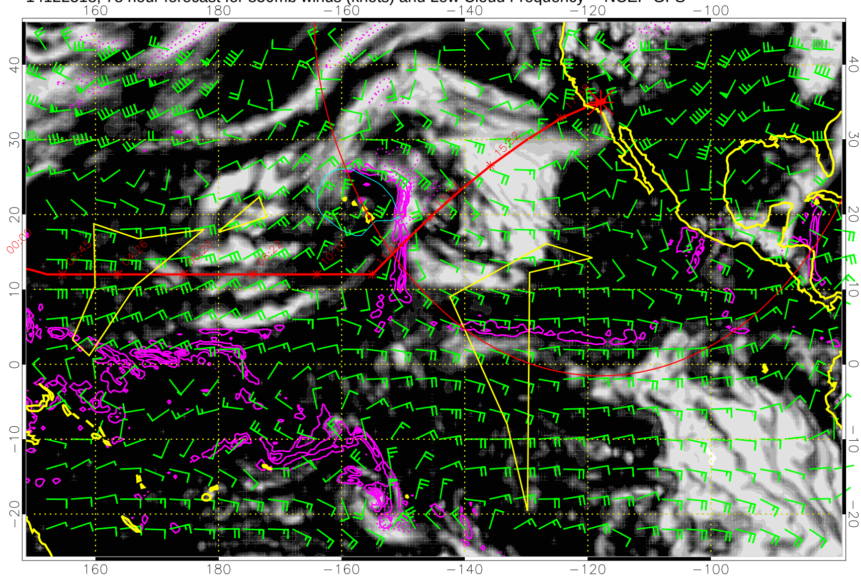
14122518, 78 hour forecast for 850mb winds (knots) and Low Cloud Frequency -- NCEP GFS
