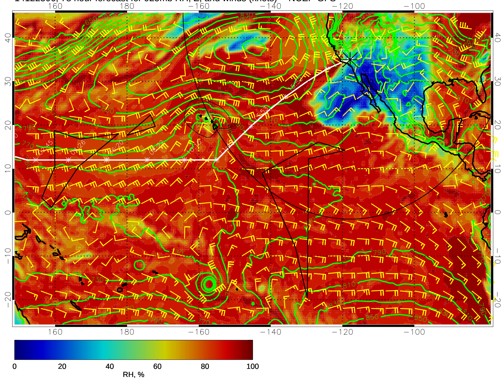
14122506, 78 hour forecast for 925mb RH, Z, and winds (knots) -- NCEP GFS
