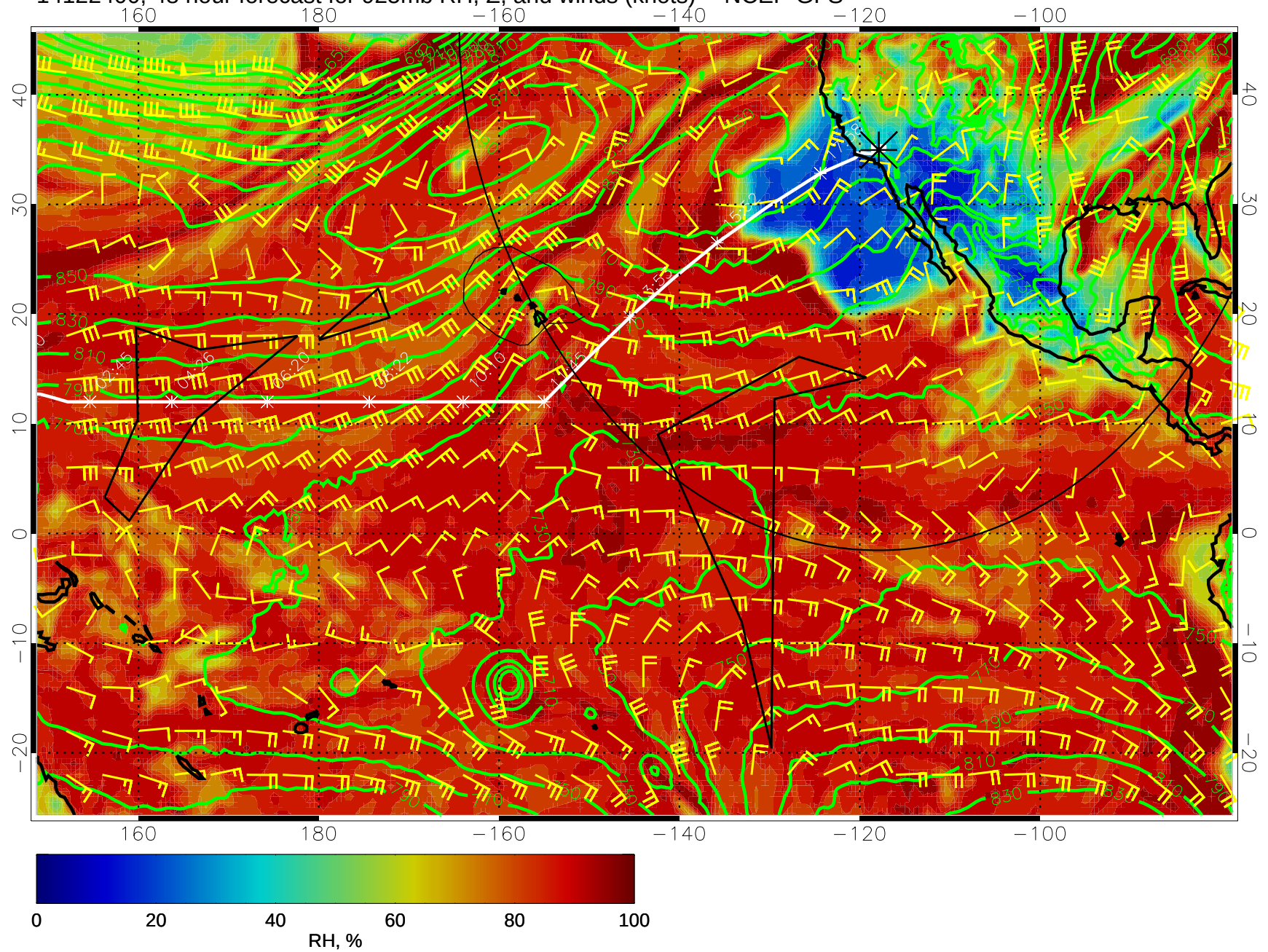
14122400, 48 hour forecast for 925mb RH, Z, and winds (knots) -- NCEP GFS
