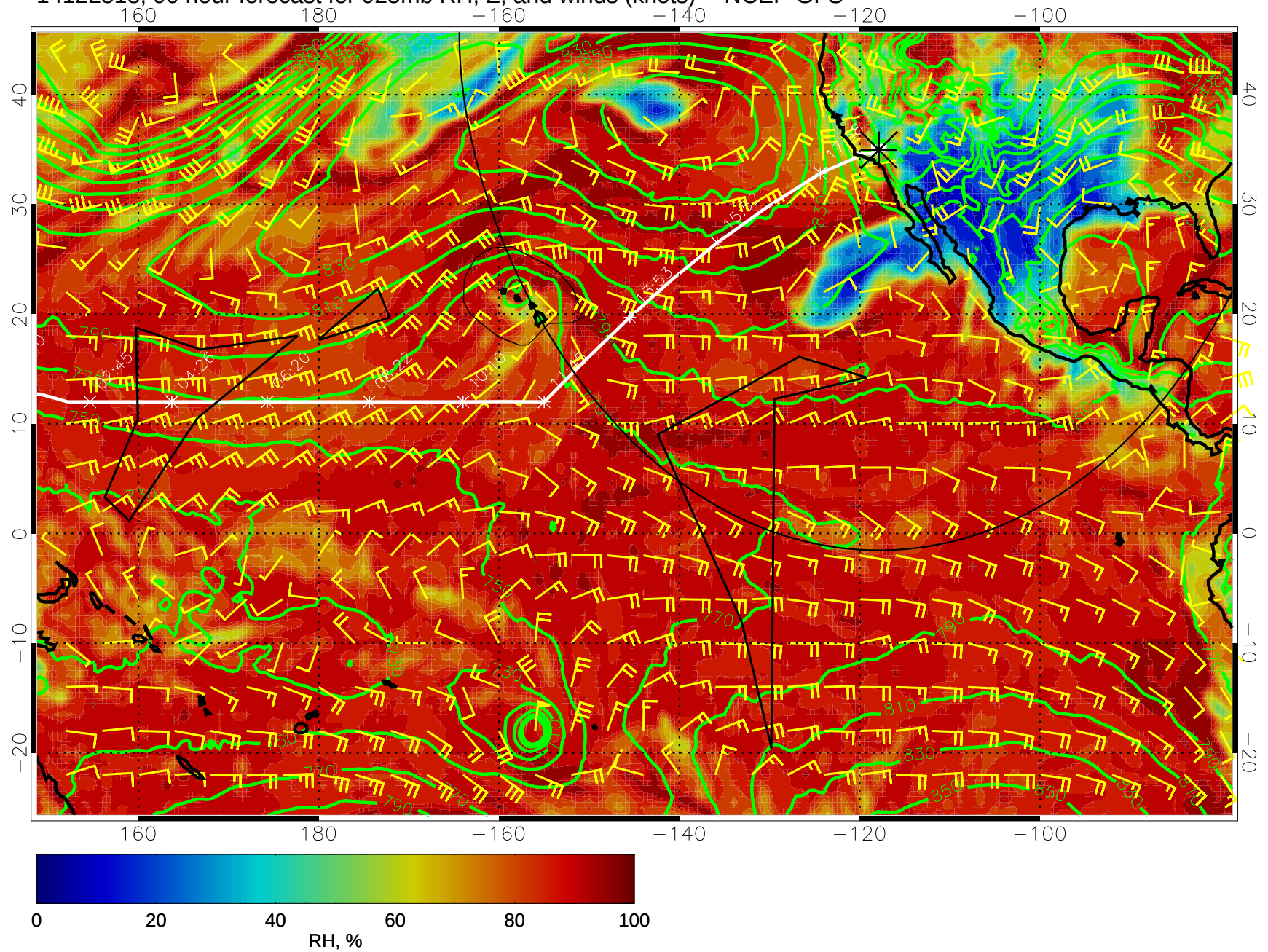
14122518, 90 hour forecast for 925mb RH, Z, and winds (knots) -- NCEP GFS
