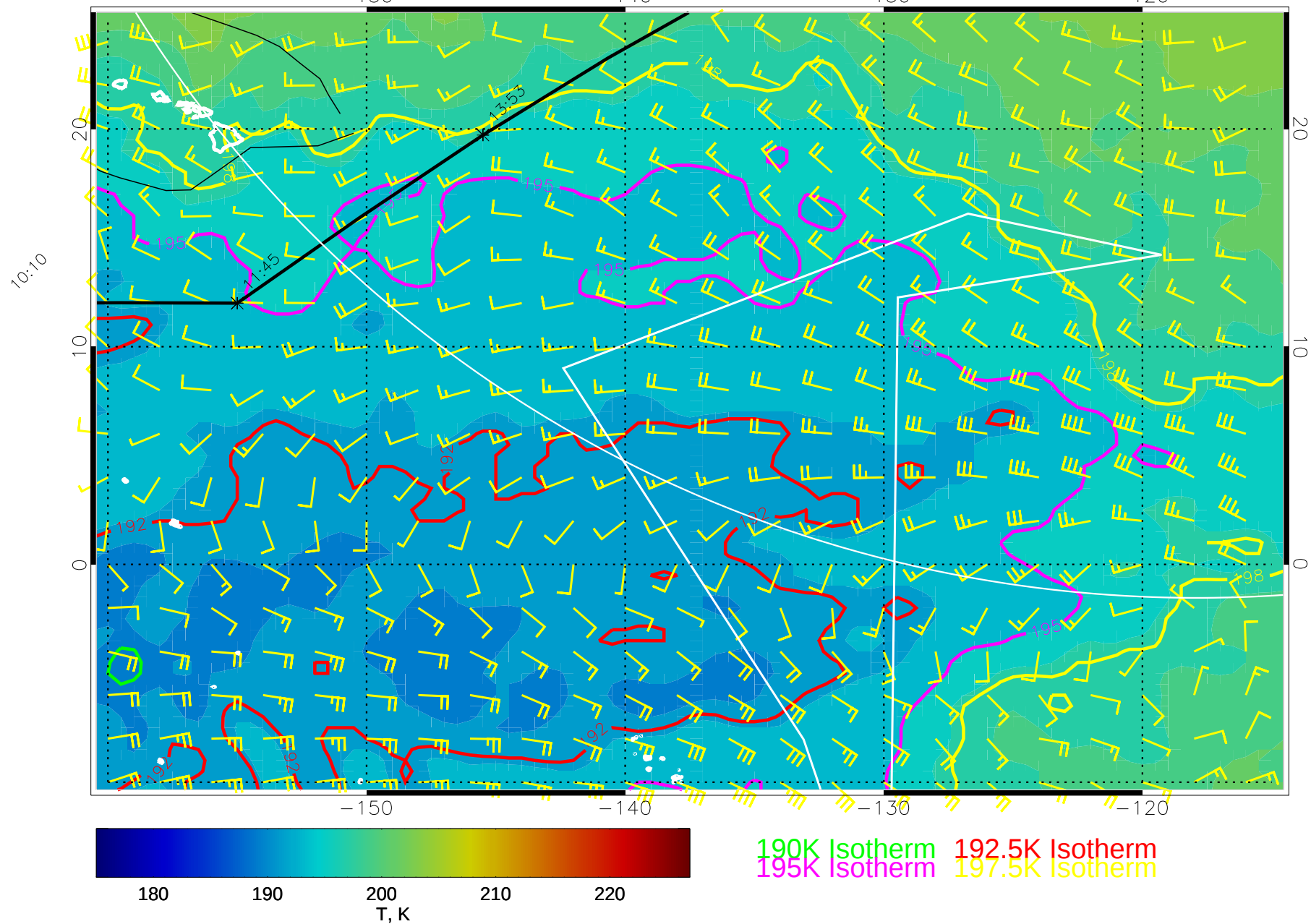
14122618, 114 hour forecast for 70mb T and winds (knots) -- NCEP GFS
