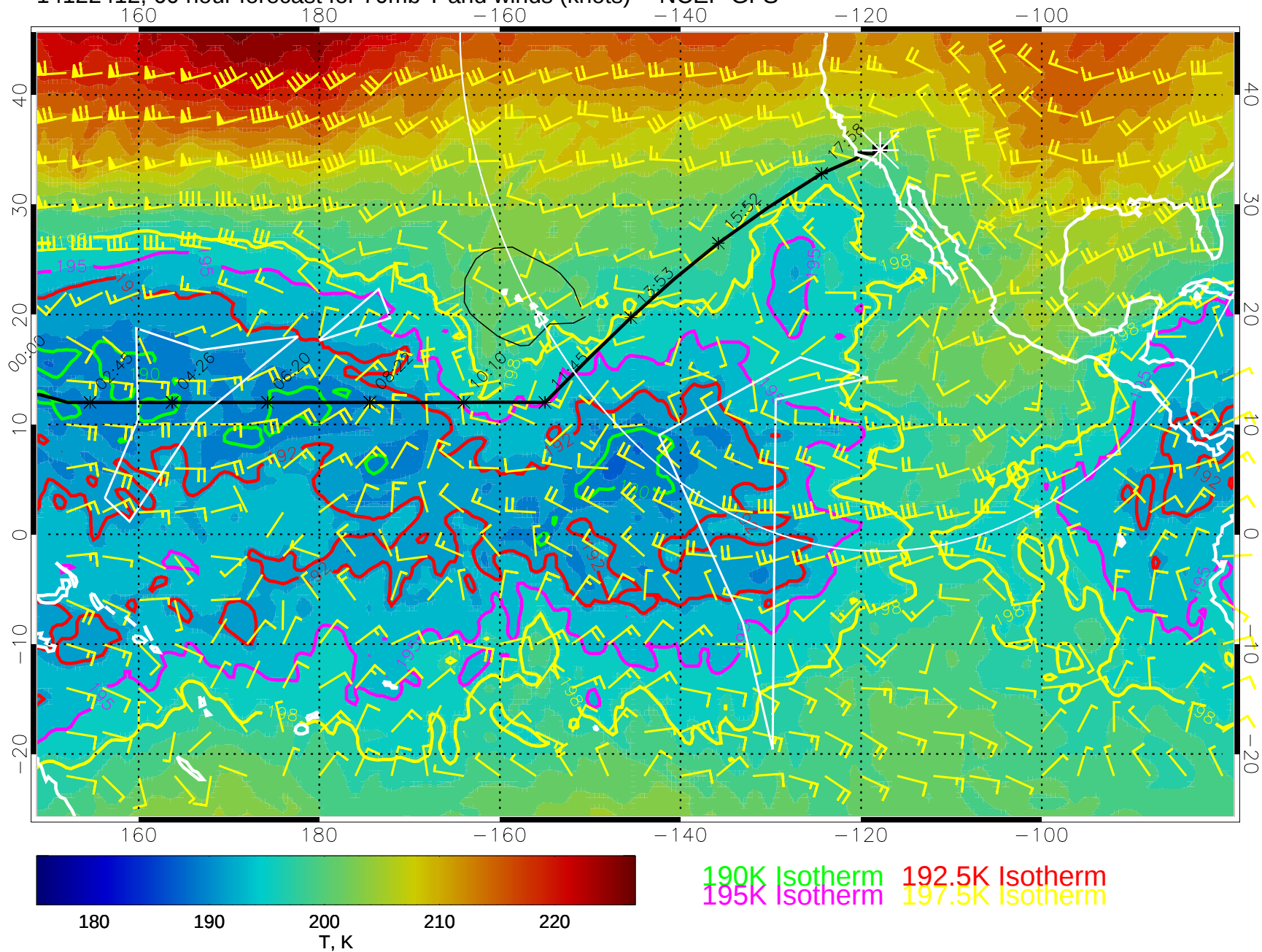
14122412, 60 hour forecast for 70mb T and winds (knots) -- NCEP GFS
