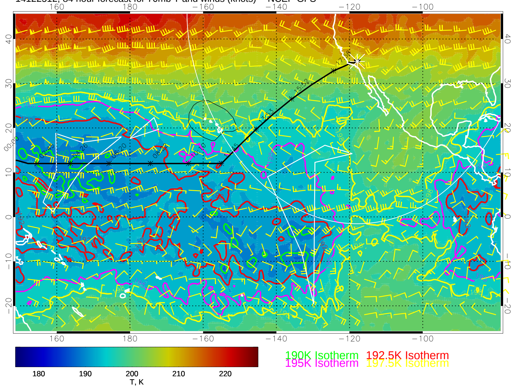
14122512, 84 hour forecast for 70mb T and winds (knots) -- NCEP GFS
