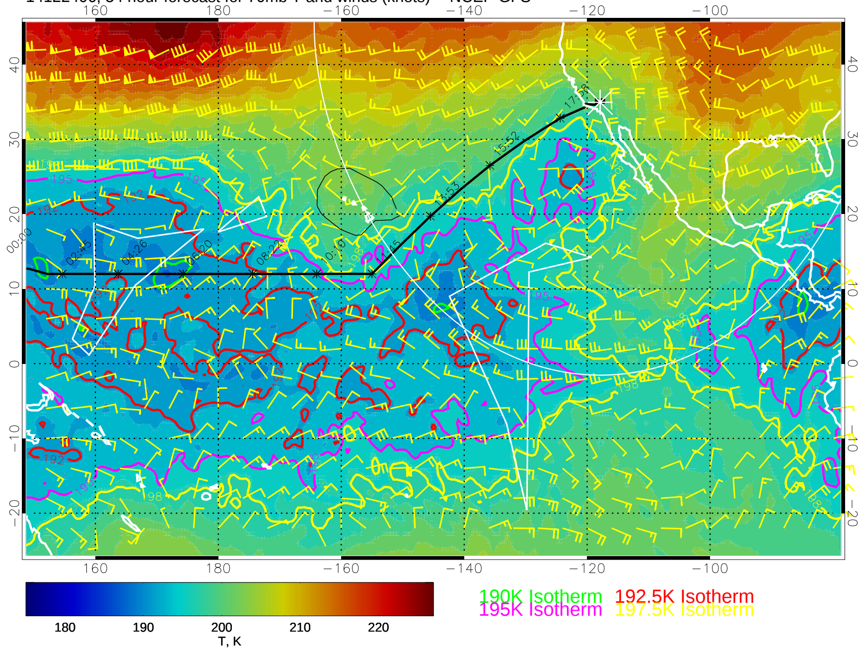
14122406, 54 hour forecast for 70mb T and winds (knots) -- NCEP GFS
