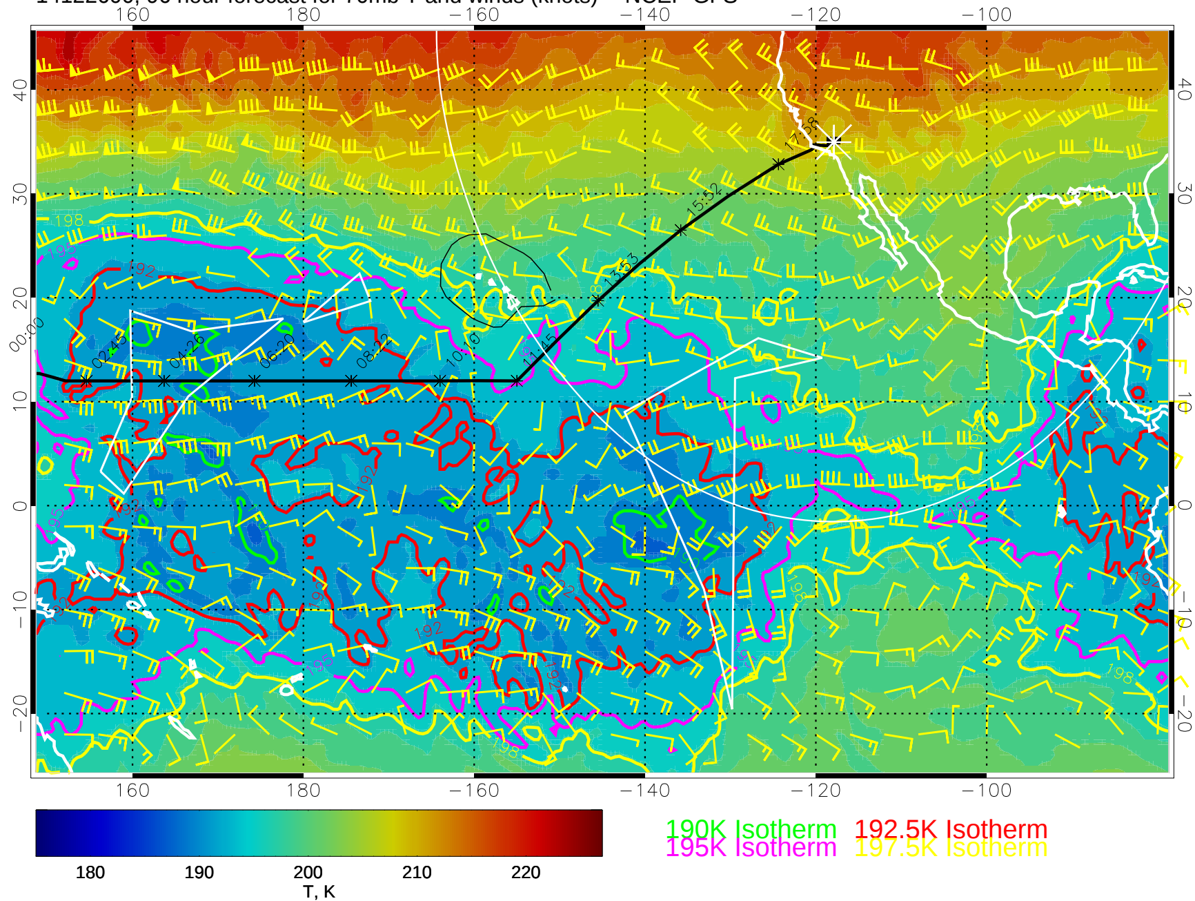
14122600, 96 hour forecast for 70mb T and winds (knots) -- NCEP GFS
