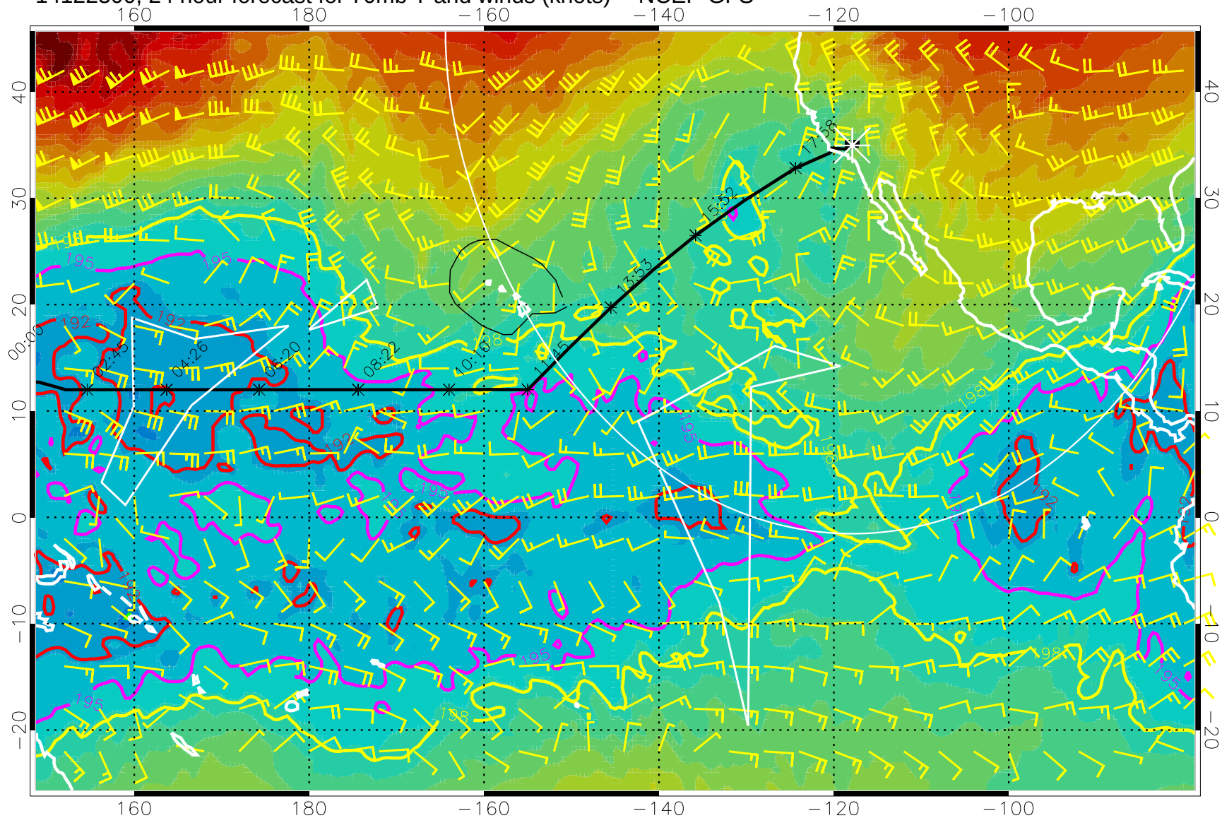
14122300, 24 hour forecast for 70mb T and winds (knots) -- NCEP GFS
