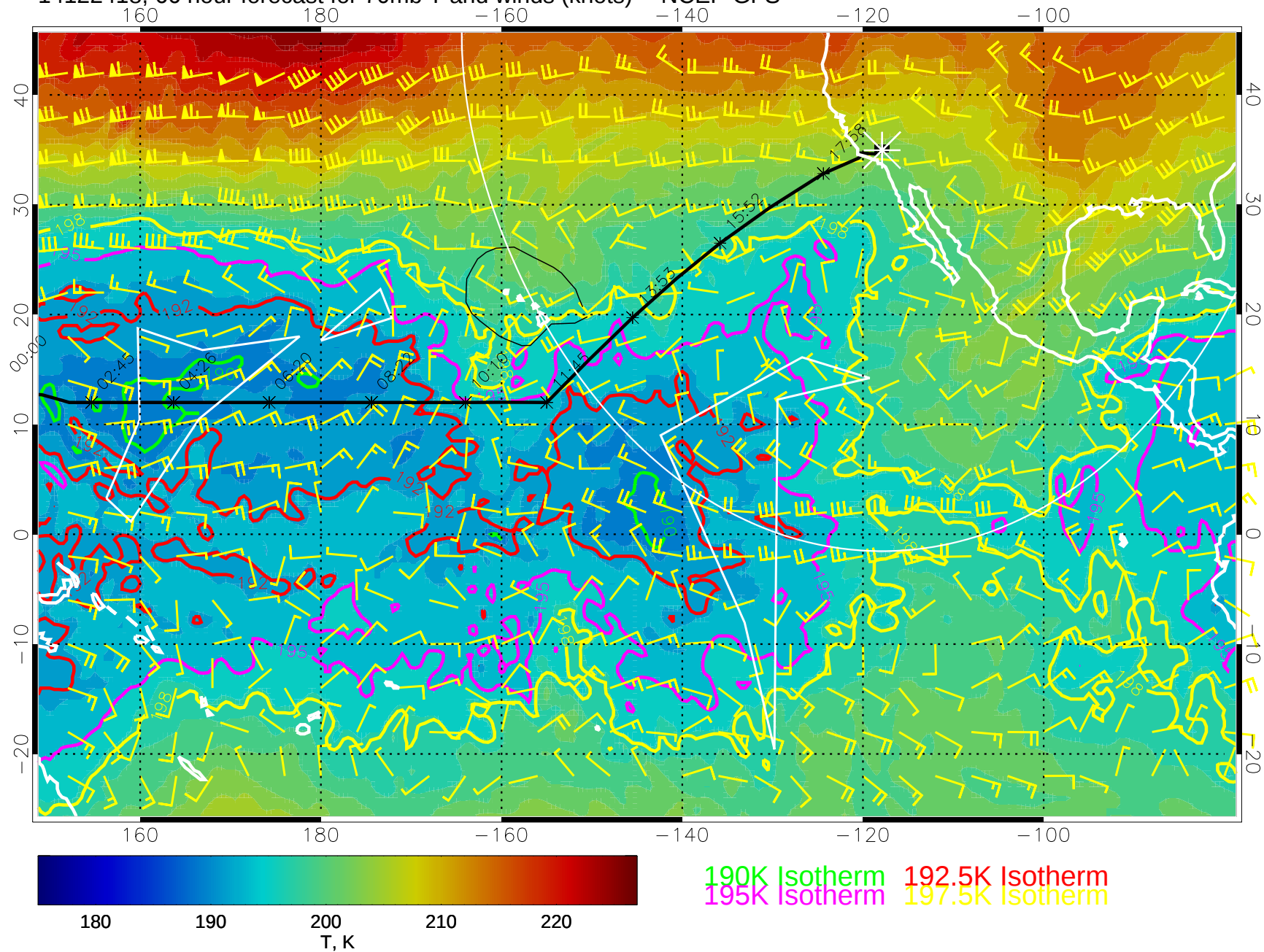
14122418, 66 hour forecast for 70mb T and winds (knots) -- NCEP GFS
