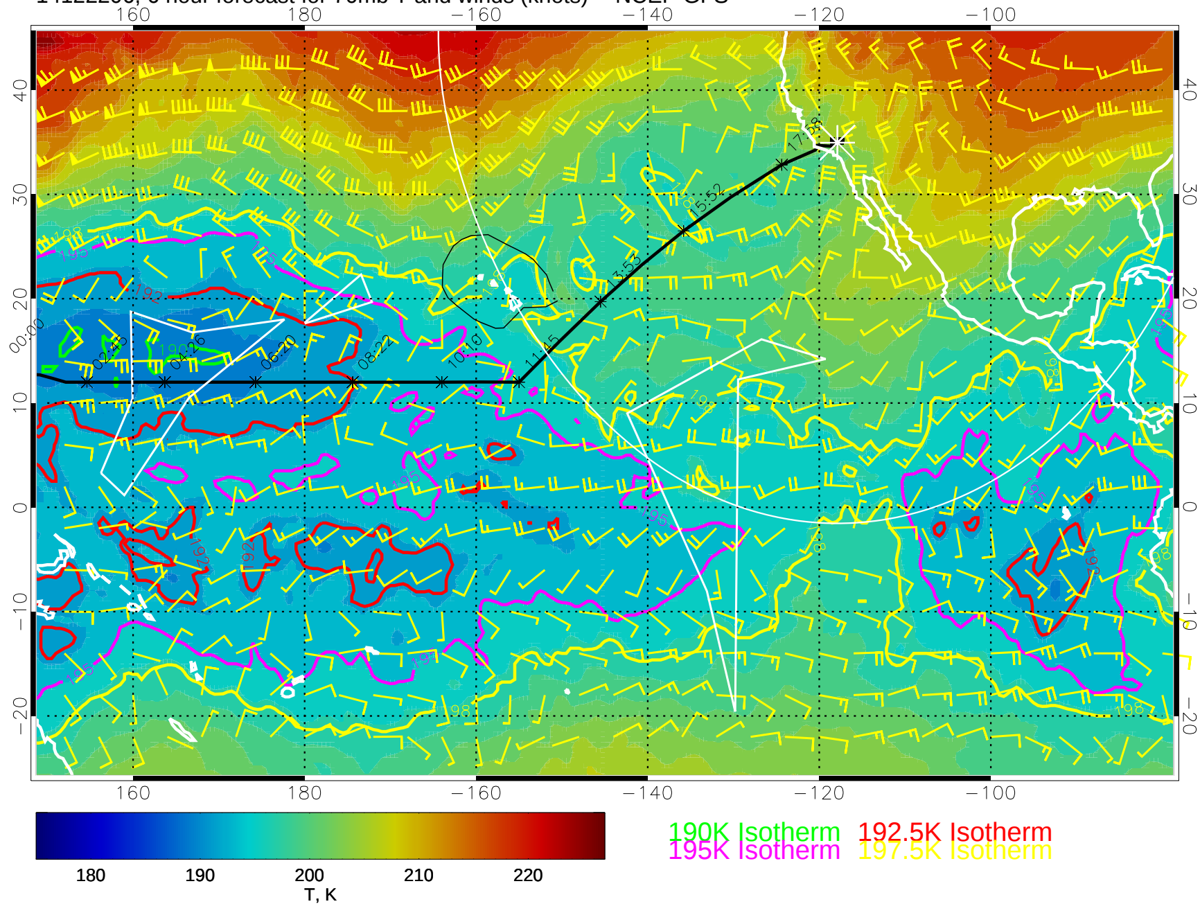
14122206, 6 hour forecast for 70mb T and winds (knots) -- NCEP GFS
