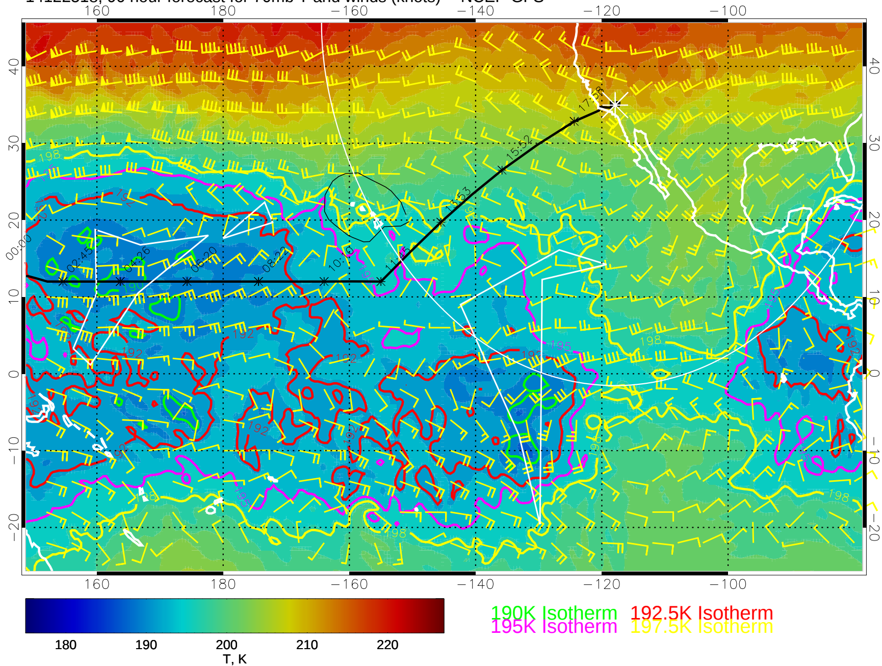
14122518, 90 hour forecast for 70mb T and winds (knots) -- NCEP GFS
