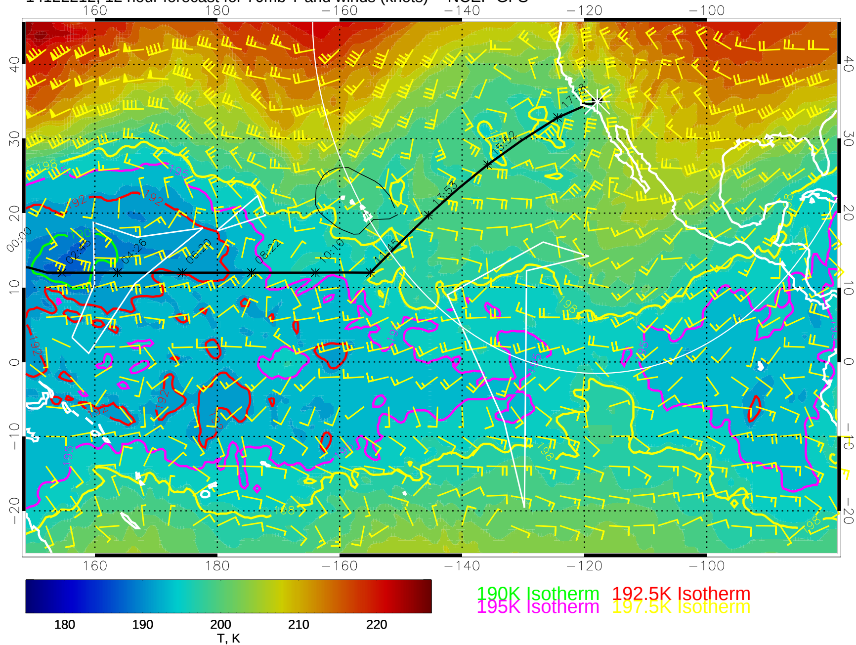
14122212, 12 hour forecast for 70mb T and winds (knots) -- NCEP GFS
