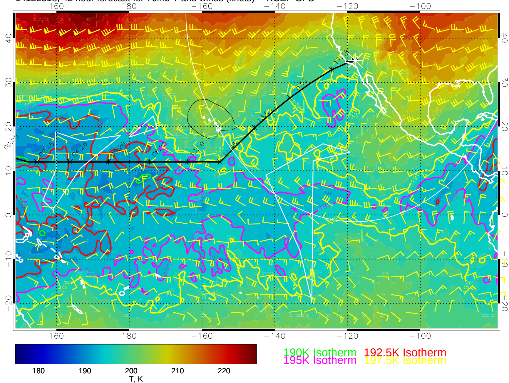
14122318, 42 hour forecast for 70mb T and winds (knots) -- NCEP GFS
