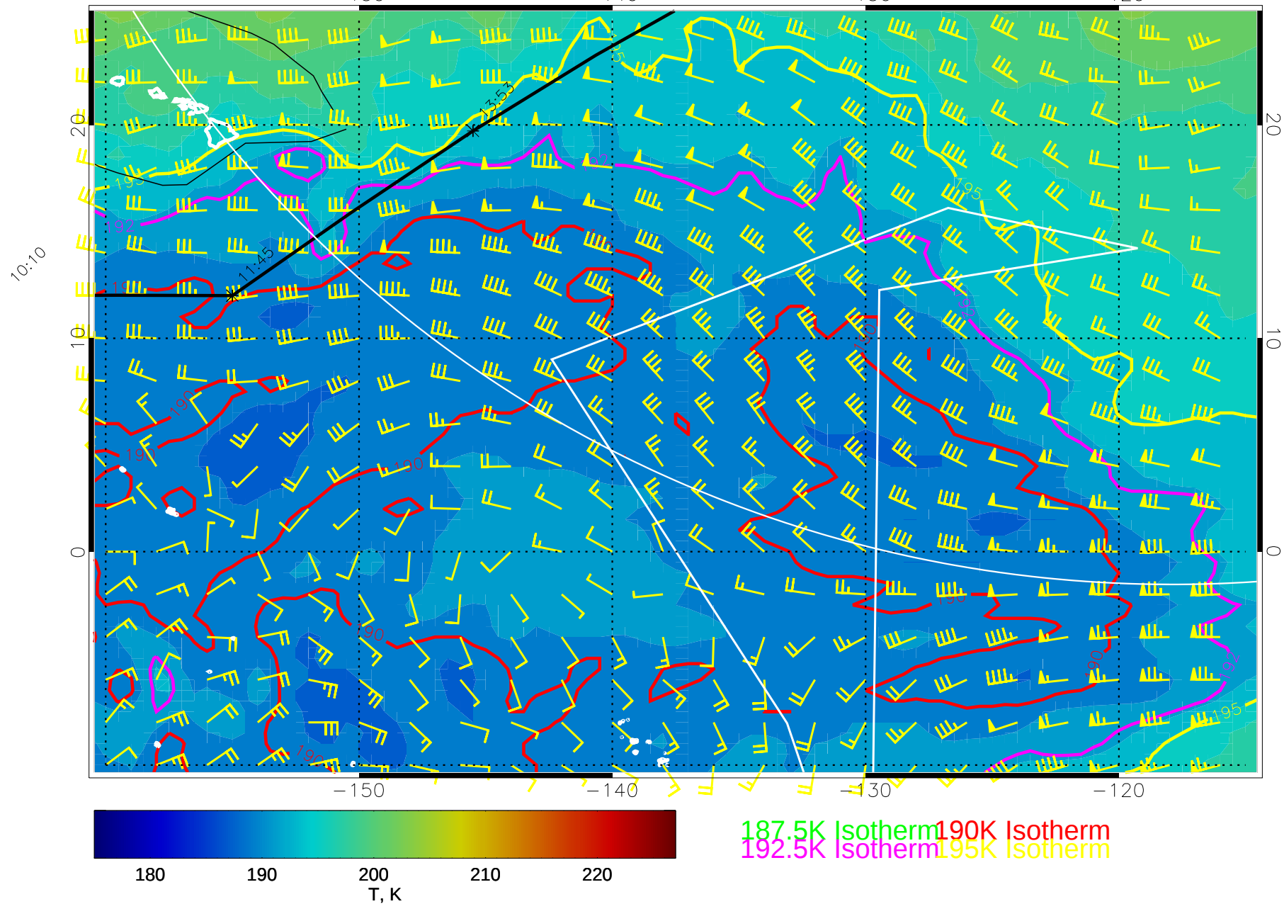
14122518, 90 hour forecast for 100mb T and winds (knots) -- NCEP GFS
