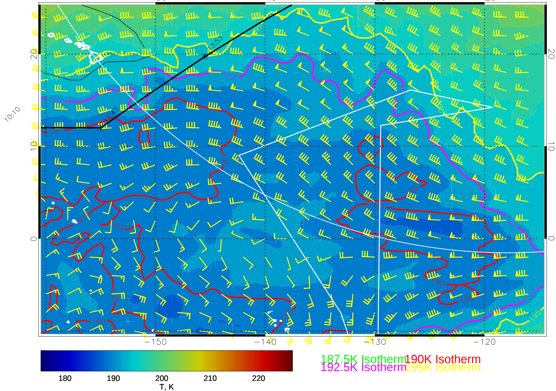
14122600, 96 hour forecast for 100mb T and winds (knots) -- NCEP GFS
