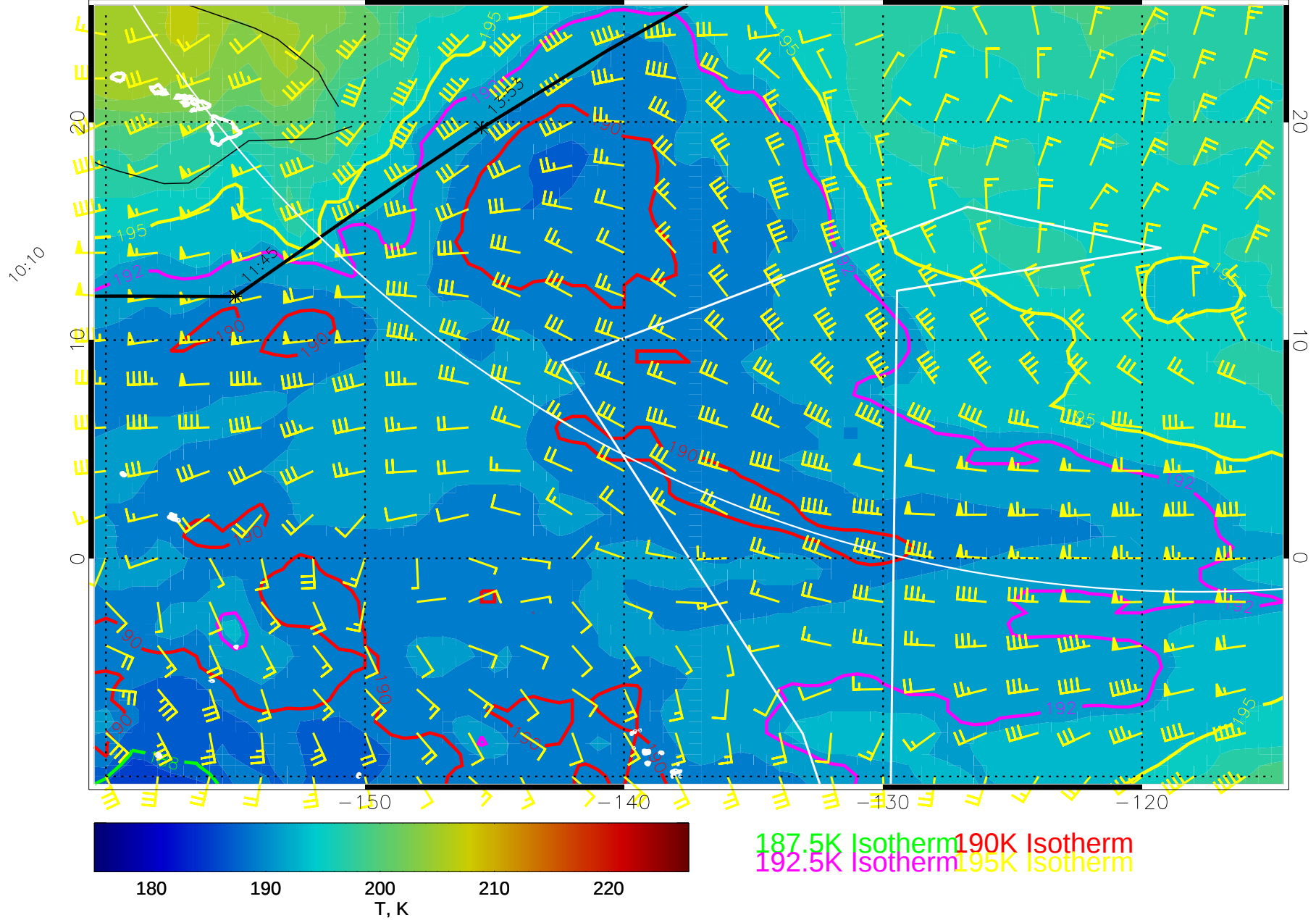
14122406, 54 hour forecast for 100mb T and winds (knots) -- NCEP GFS
