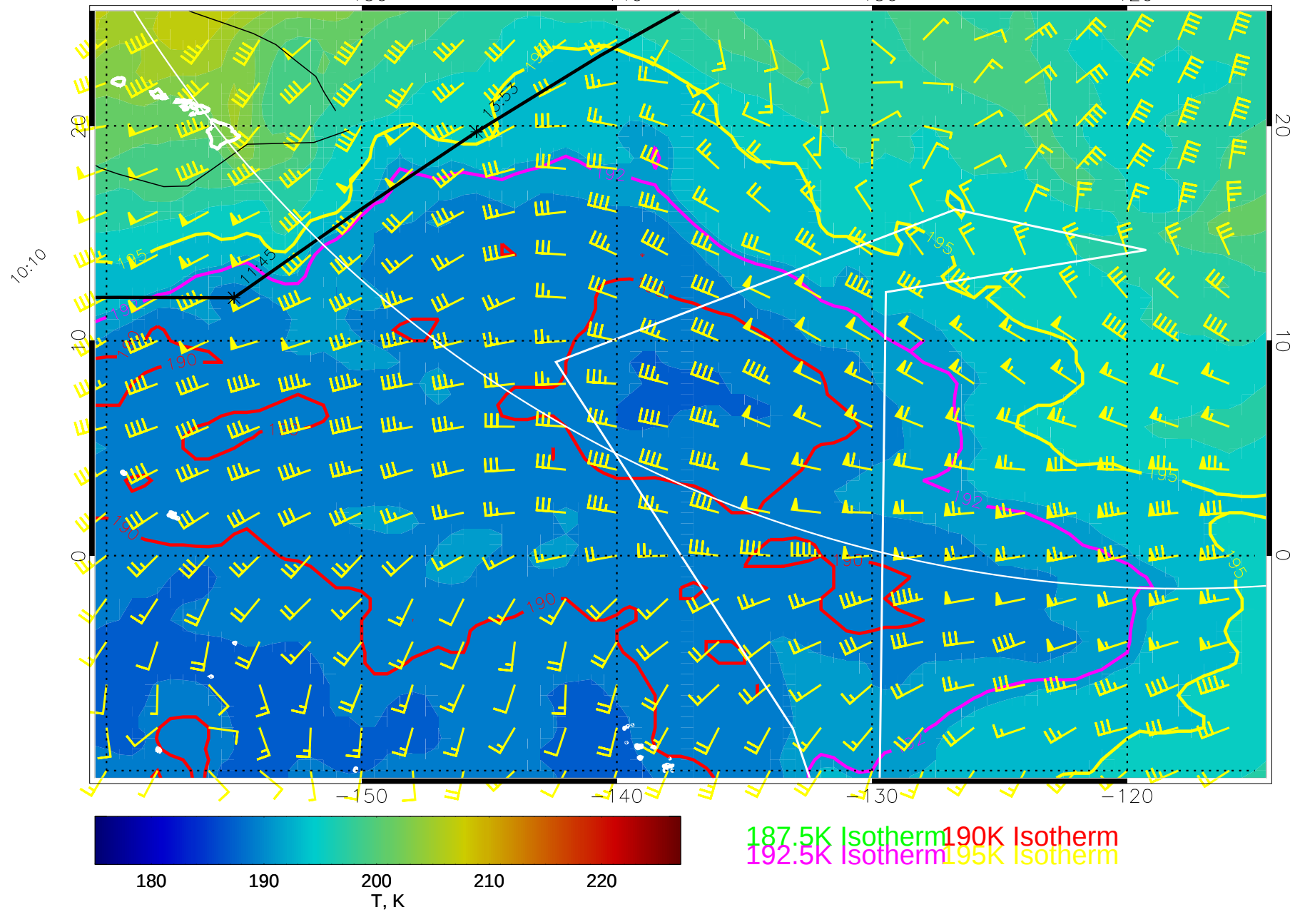
14122312, 36 hour forecast for 100mb T and winds (knots) -- NCEP GFS
