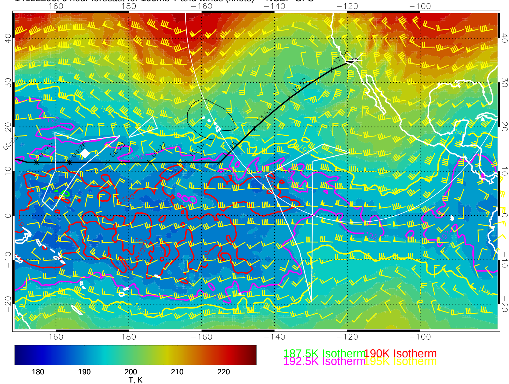
14122206, 6 hour forecast for 100mb T and winds (knots) -- NCEP GFS
