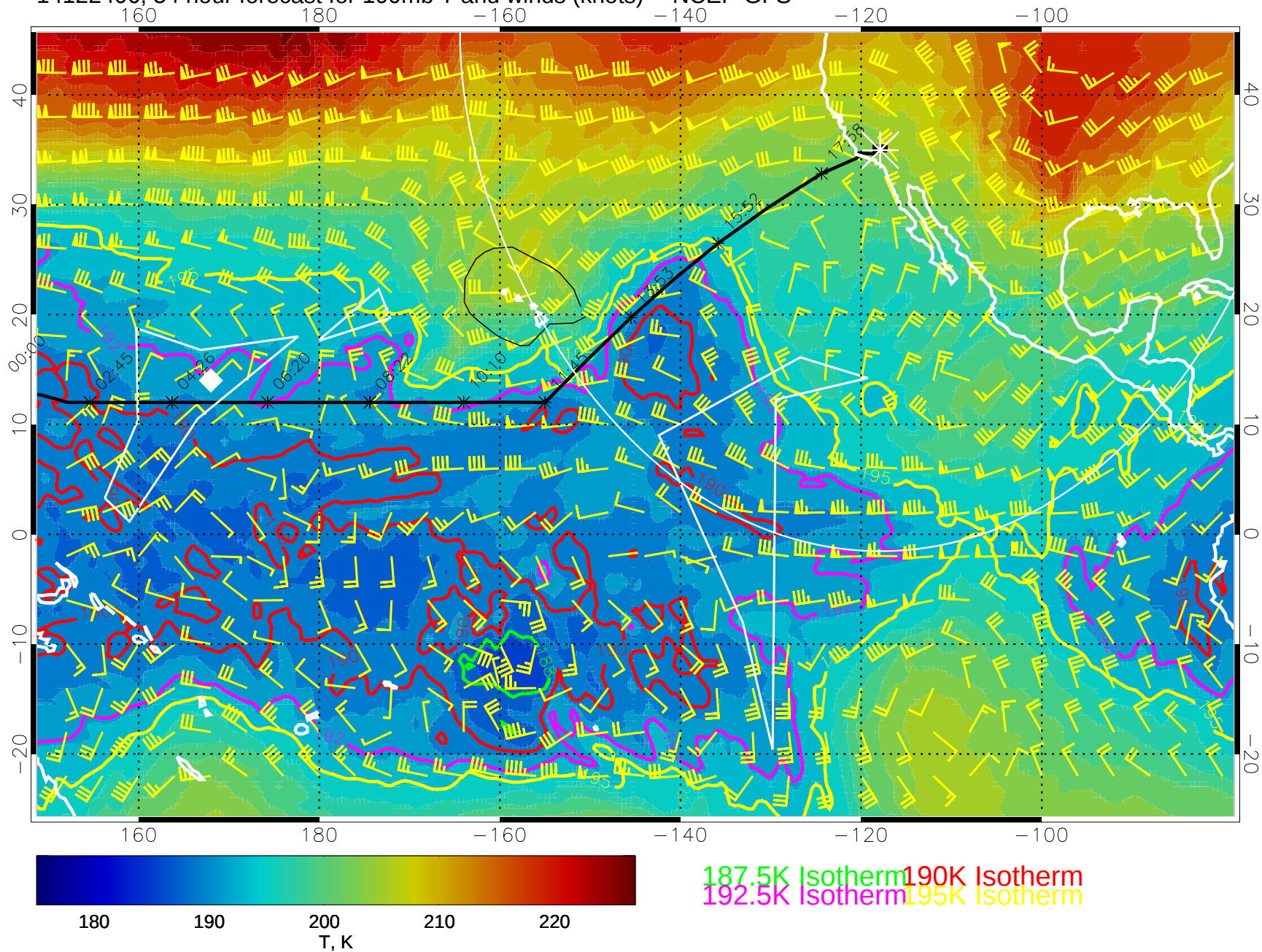
14122406, 54 hour forecast for 100mb T and winds (knots) -- NCEP GFS
