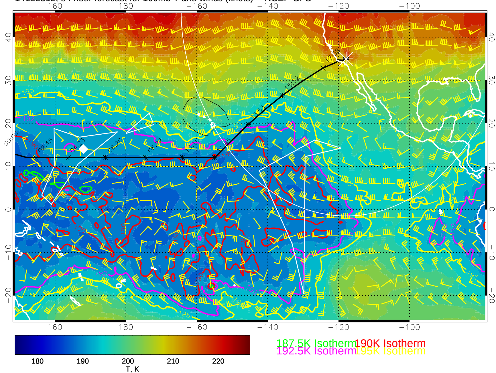
14122512, 84 hour forecast for 100mb T and winds (knots) -- NCEP GFS
