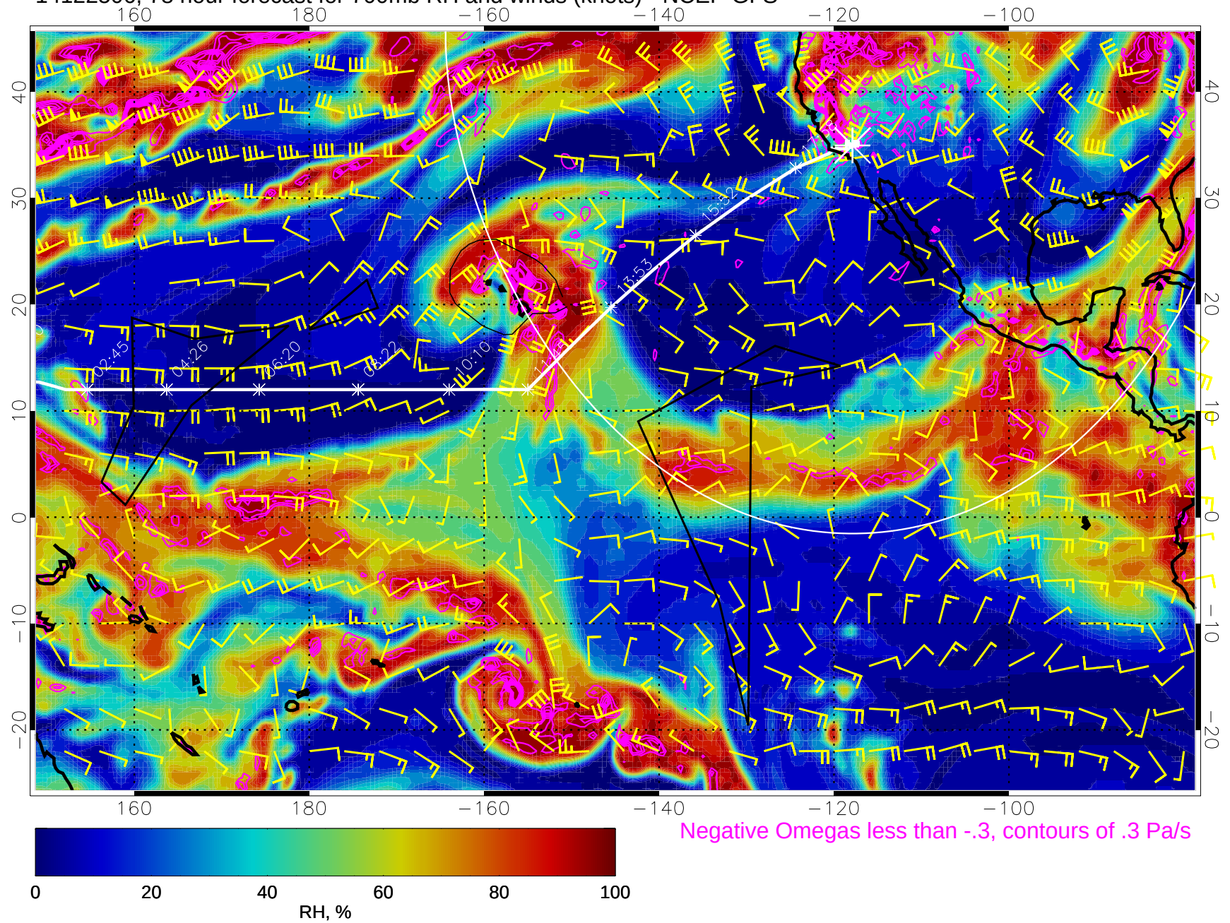
14122506, 78 hour forecast for 700mb RH and winds (knots) - NCEP GFS
