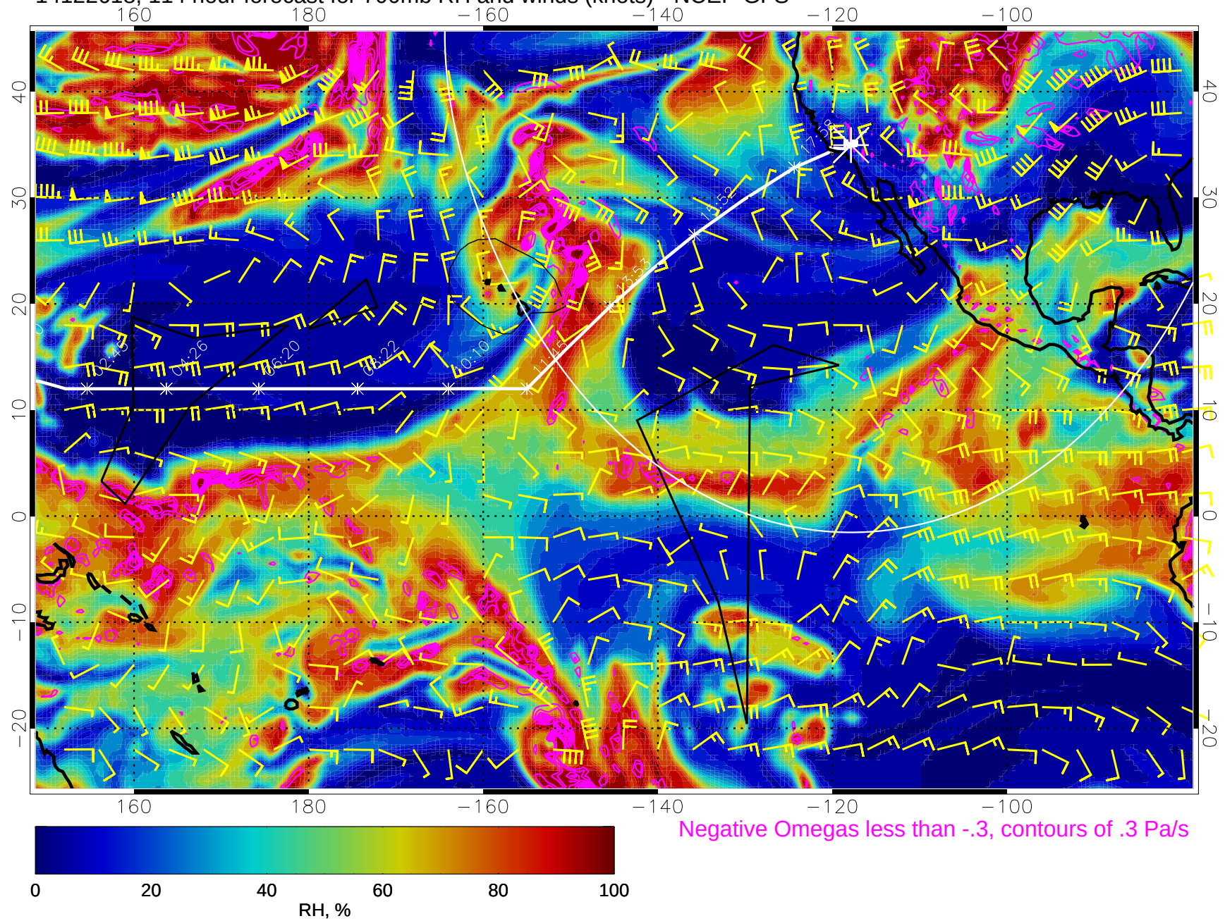
14122618, 114 hour forecast for 700mb RH and winds (knots) - NCEP GFS
