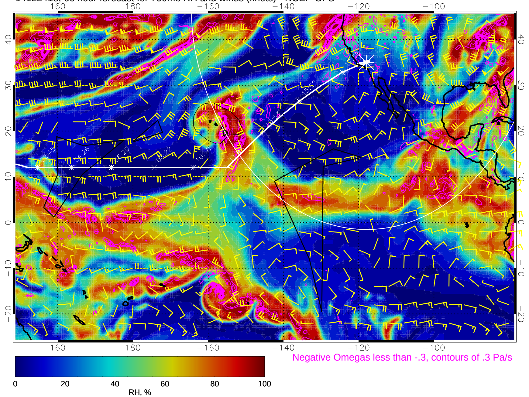
14122418, 66 hour forecast for 700mb RH and winds (knots) - NCEP GFS
