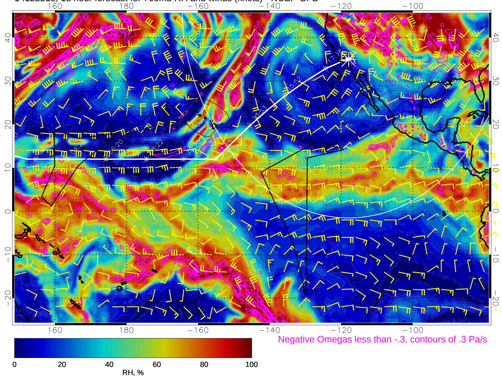
14122218, 18 hour forecast for 700mb RH and winds (knots) - NCEP GFS
