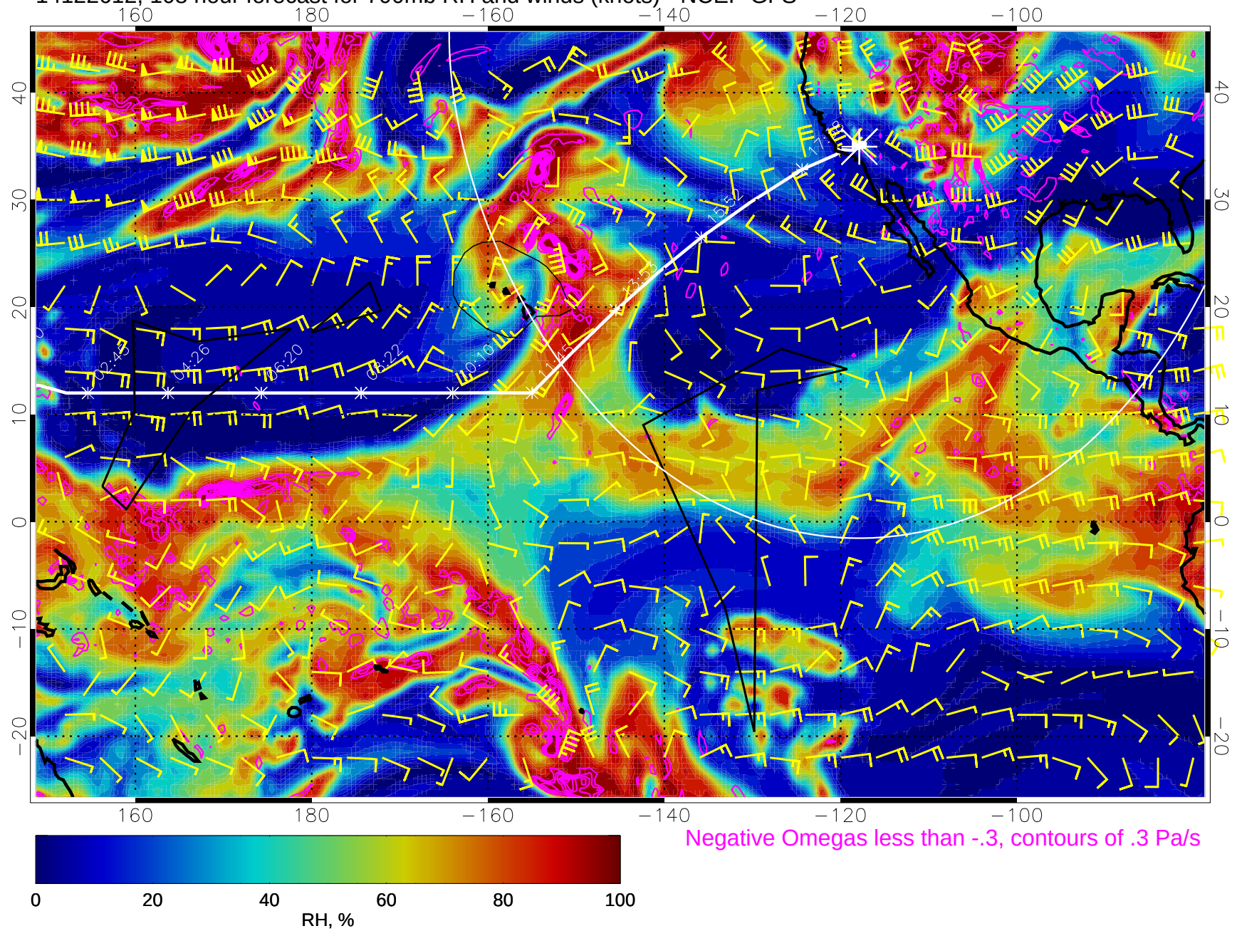
14122612, 108 hour forecast for 700mb RH and winds (knots) - NCEP GFS
