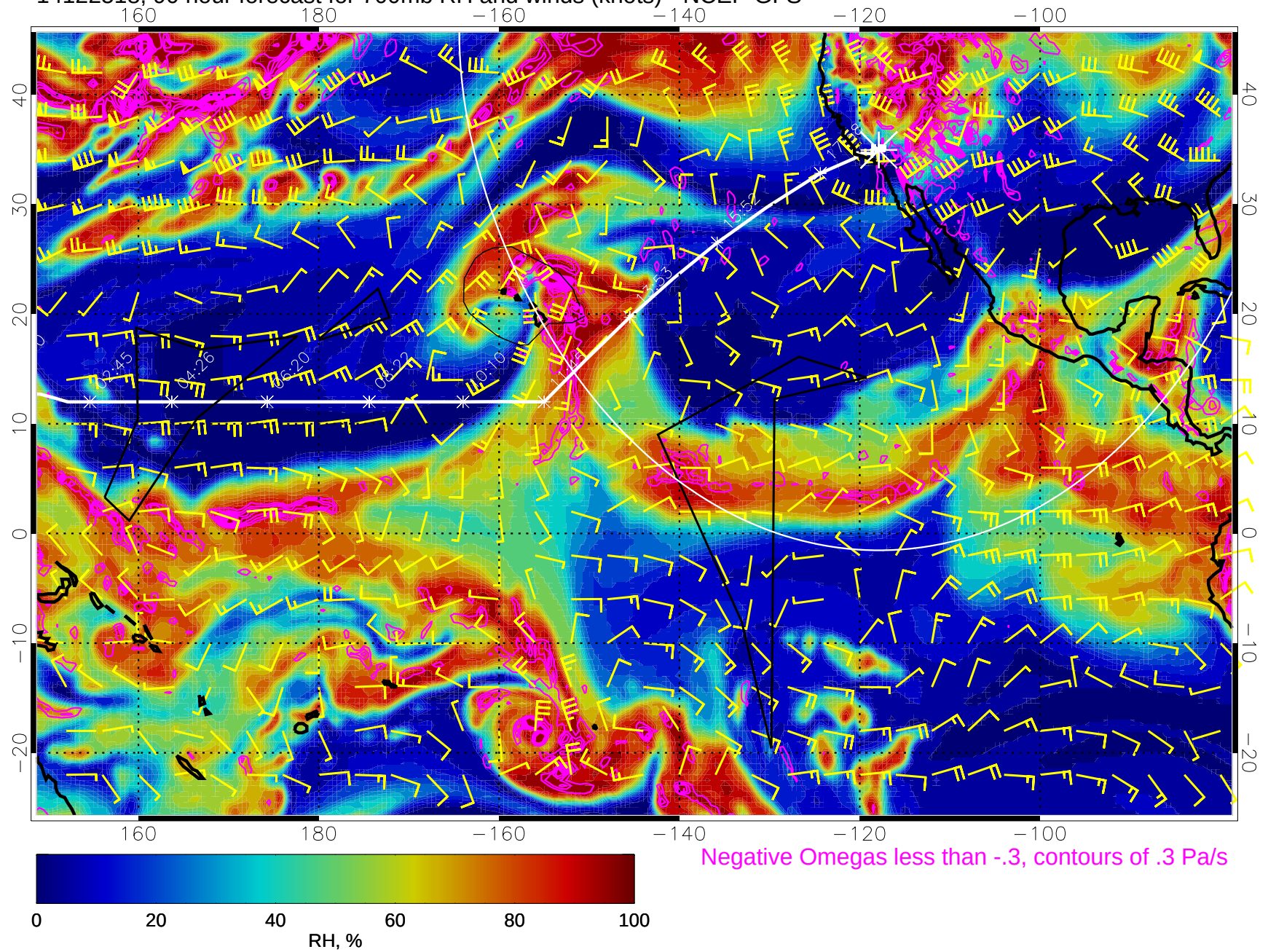
14122518, 90 hour forecast for 700mb RH and winds (knots) - NCEP GFS
