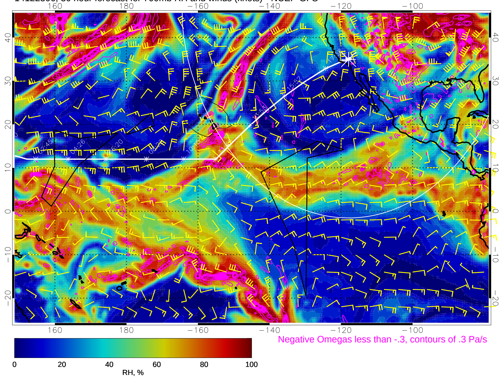
14122306, 30 hour forecast for 700mb RH and winds (knots) - NCEP GFS
