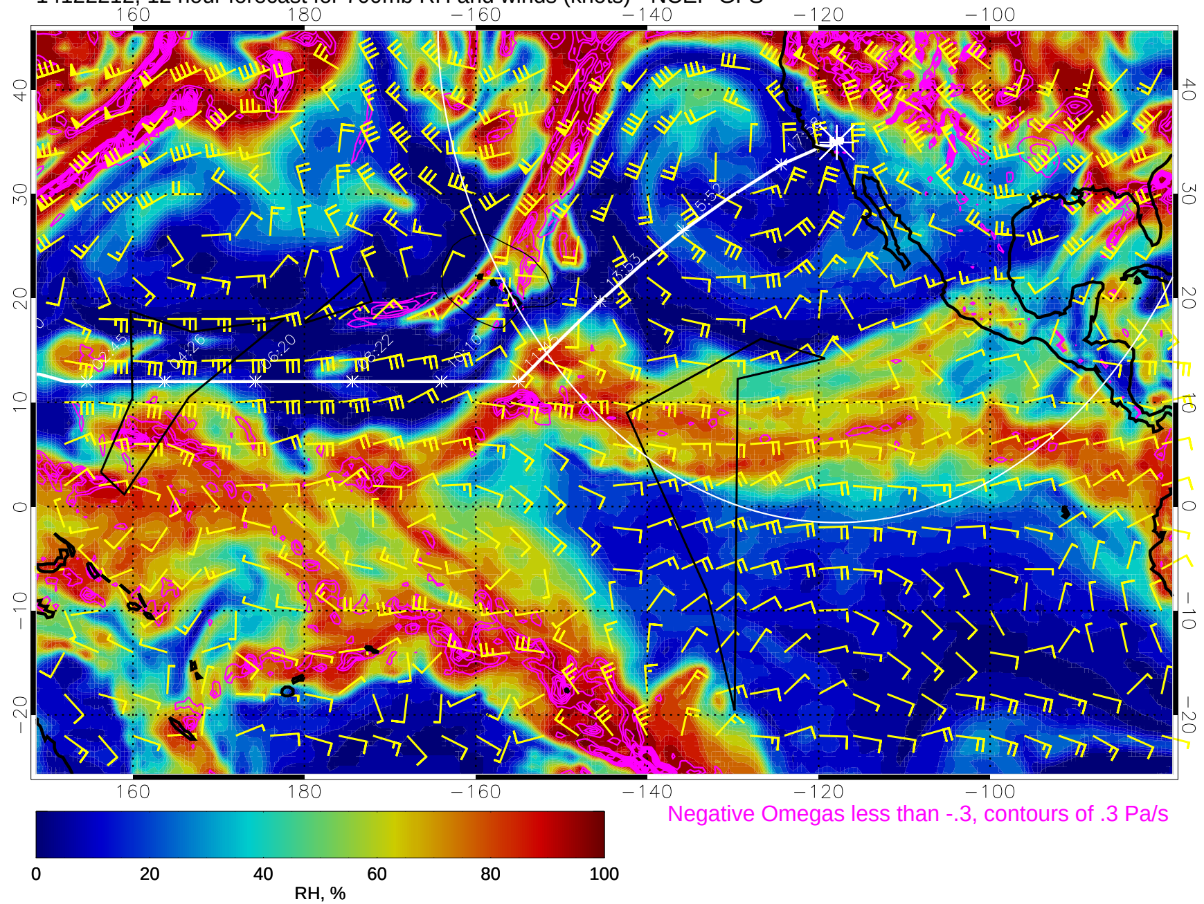
14122212, 12 hour forecast for 700mb RH and winds (knots) - NCEP GFS
