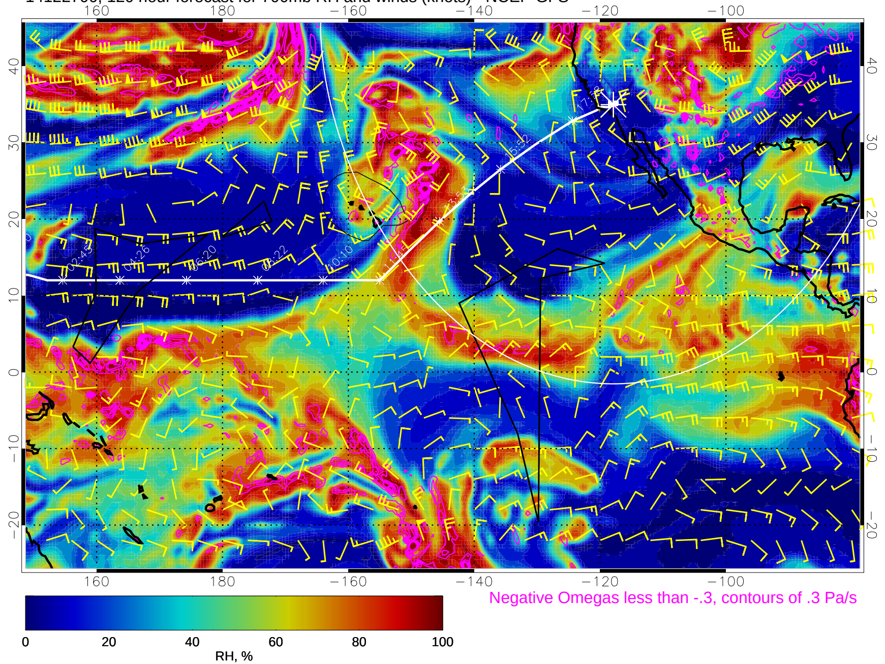
14122700, 120 hour forecast for 700mb RH and winds (knots) - NCEP GFS
