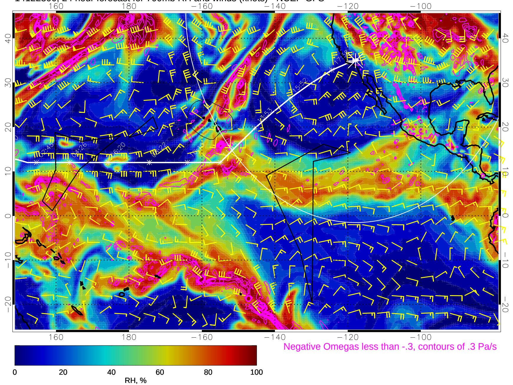
14122300, 24 hour forecast for 700mb RH and winds (knots) - NCEP GFS
