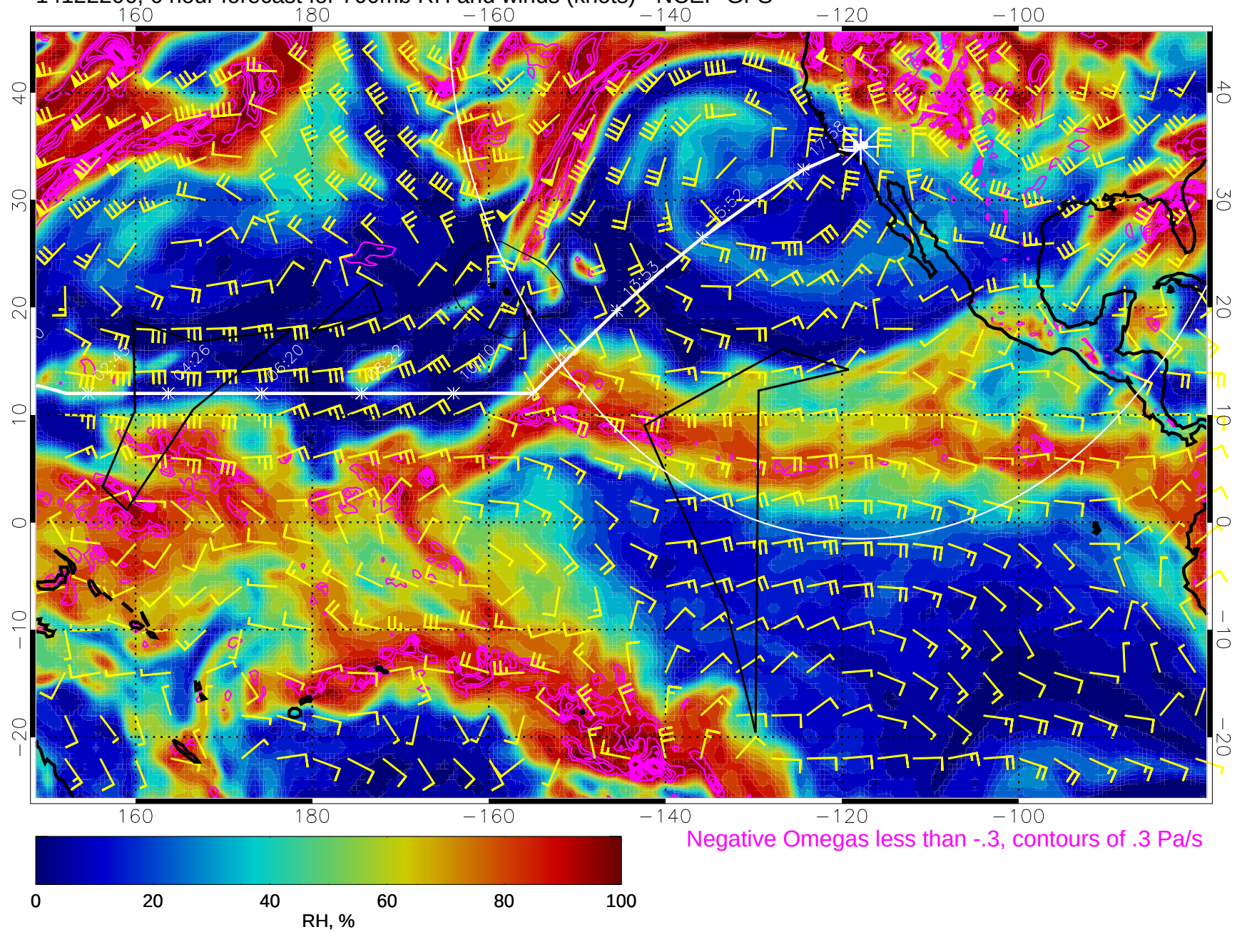
14122206, 6 hour forecast for 700mb RH and winds (knots) - NCEP GFS
