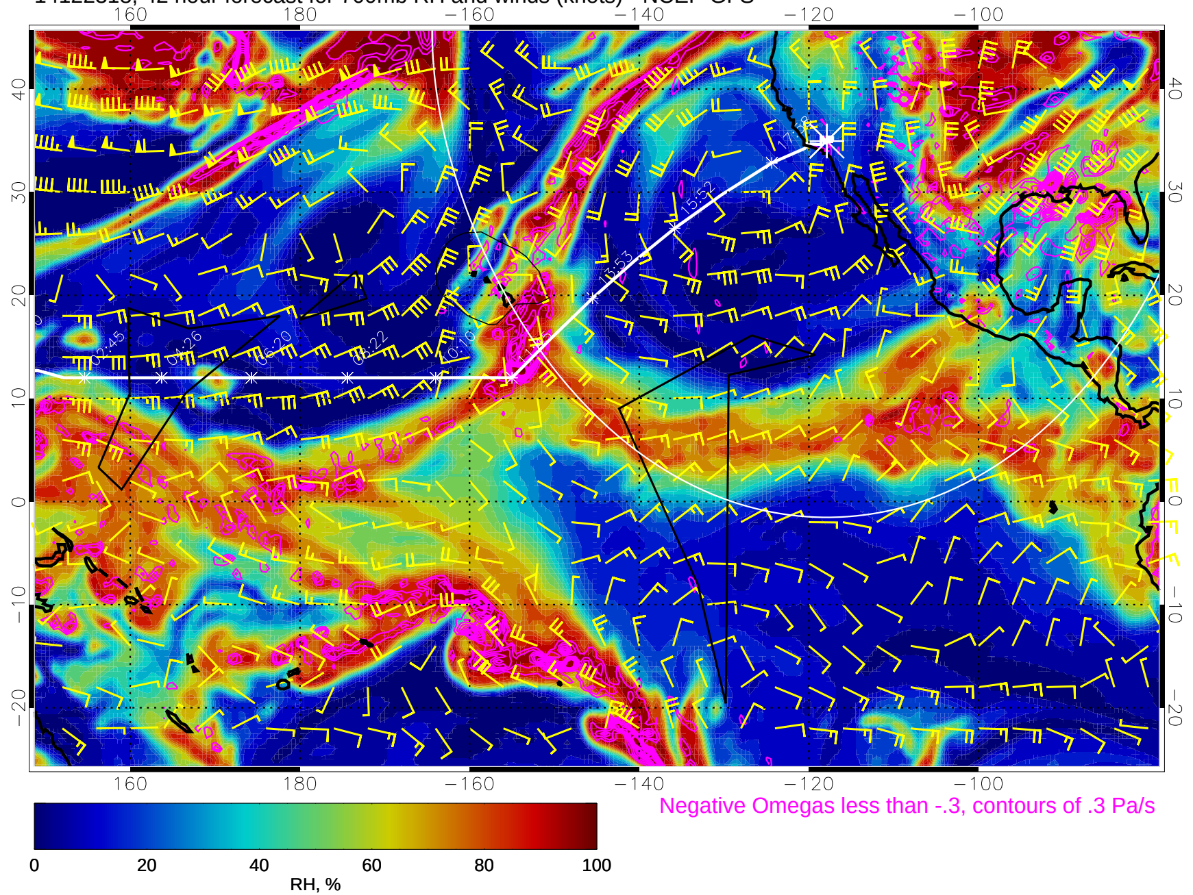
14122318, 42 hour forecast for 700mb RH and winds (knots) - NCEP GFS
