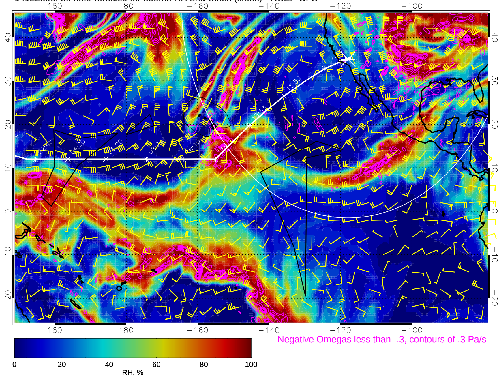
14122306, 30 hour forecast for 500mb RH and winds (knots) - NCEP GFS
