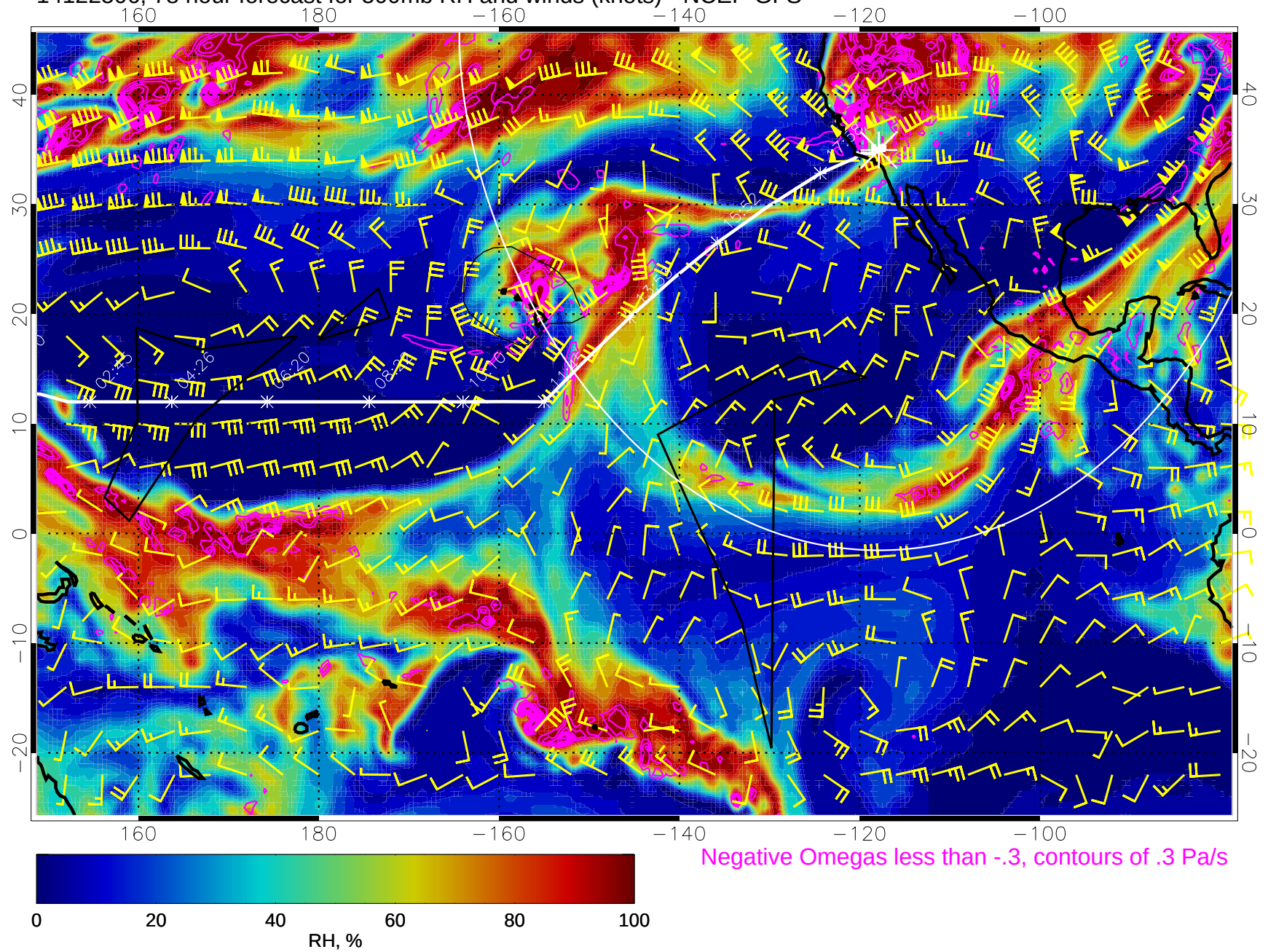
14122506, 78 hour forecast for 500mb RH and winds (knots) - NCEP GFS
