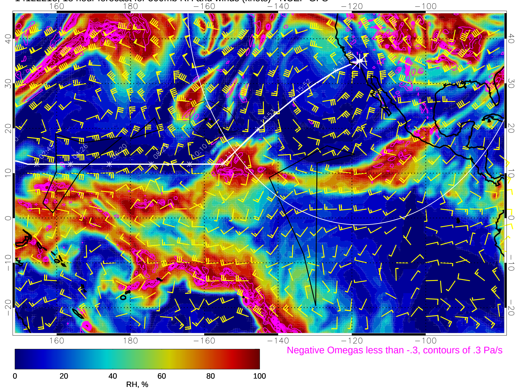
14122218, 18 hour forecast for 500mb RH and winds (knots) - NCEP GFS
