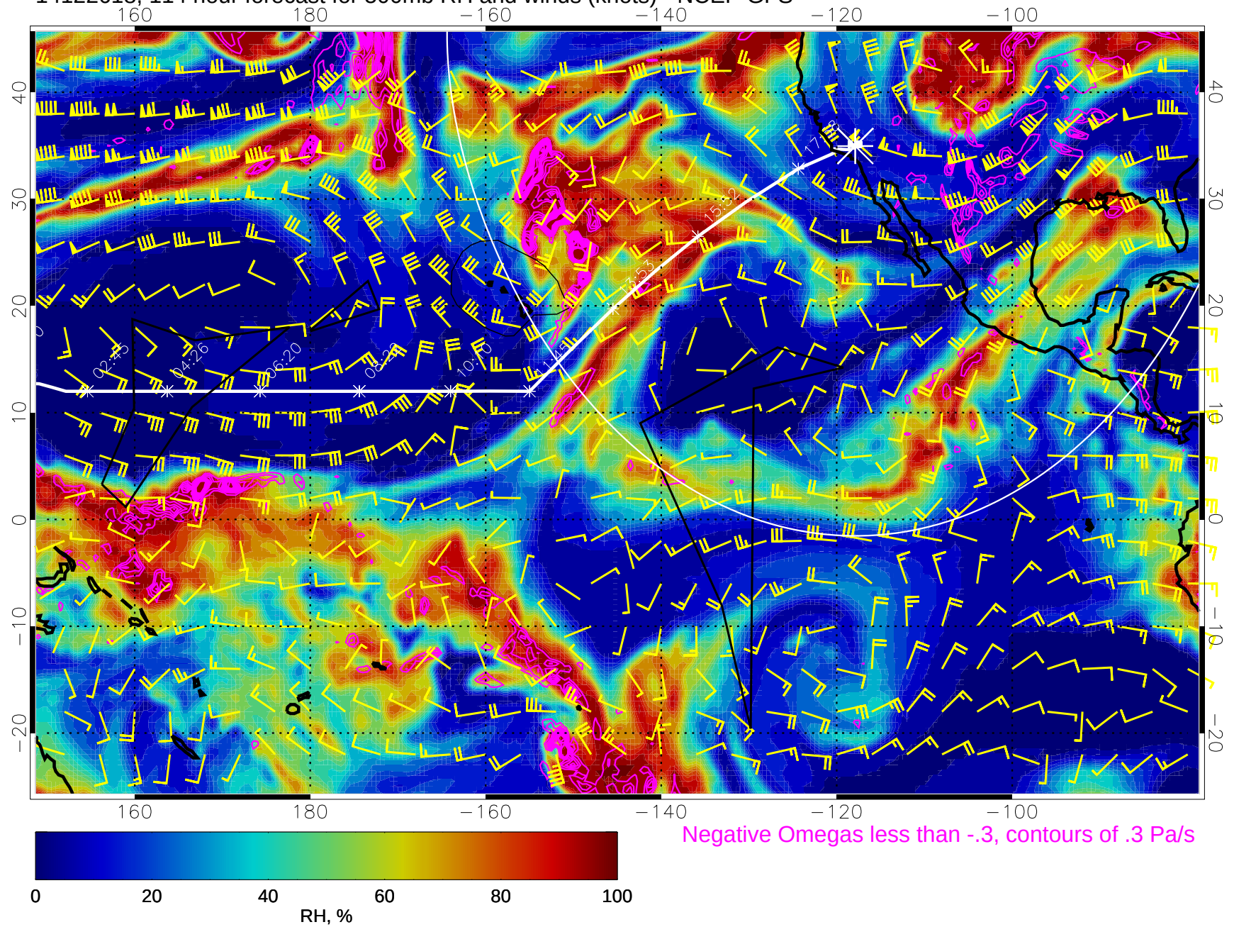
14122618, 114 hour forecast for 500mb RH and winds (knots) - NCEP GFS
