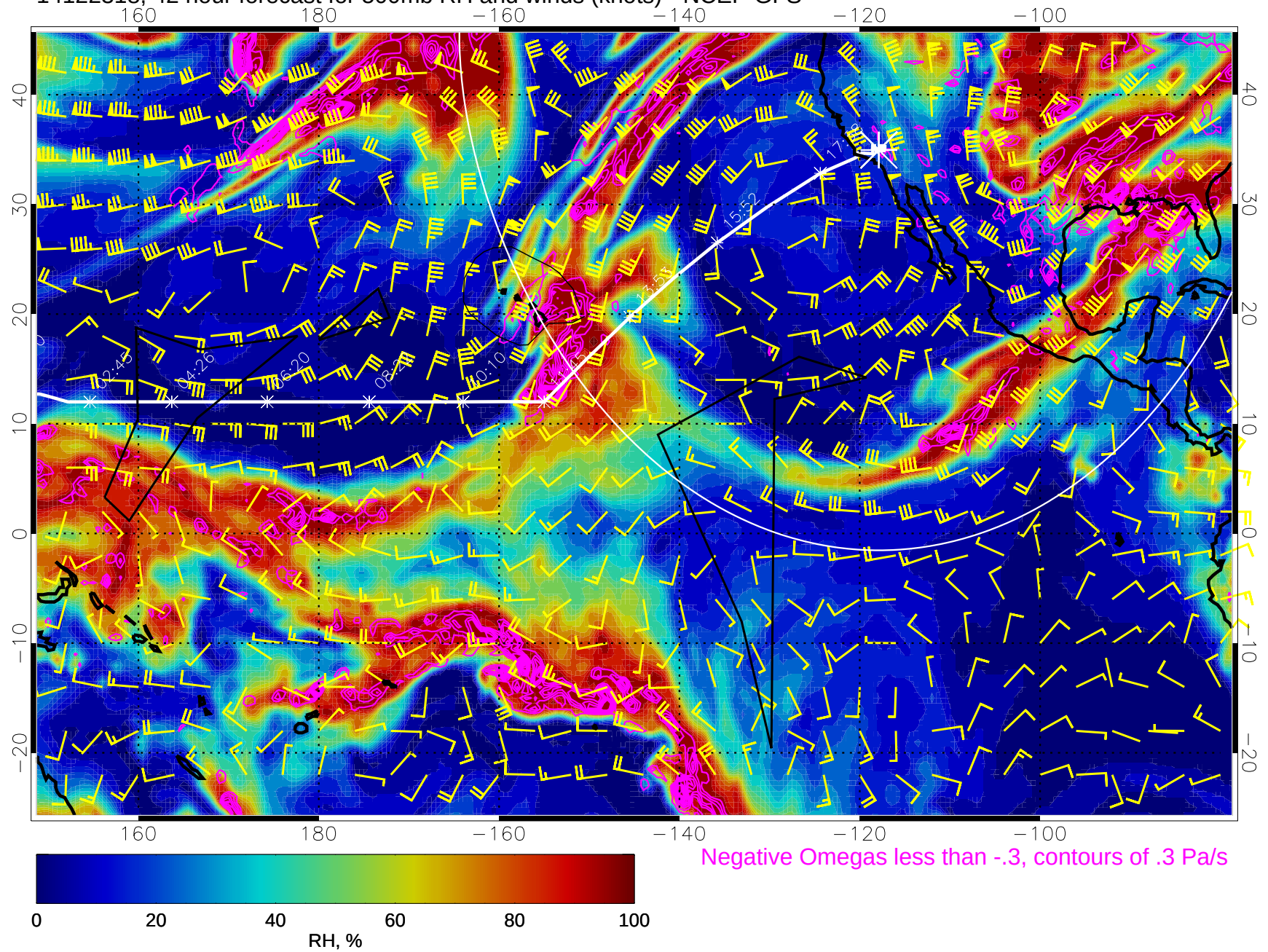
14122318, 42 hour forecast for 500mb RH and winds (knots) - NCEP GFS
