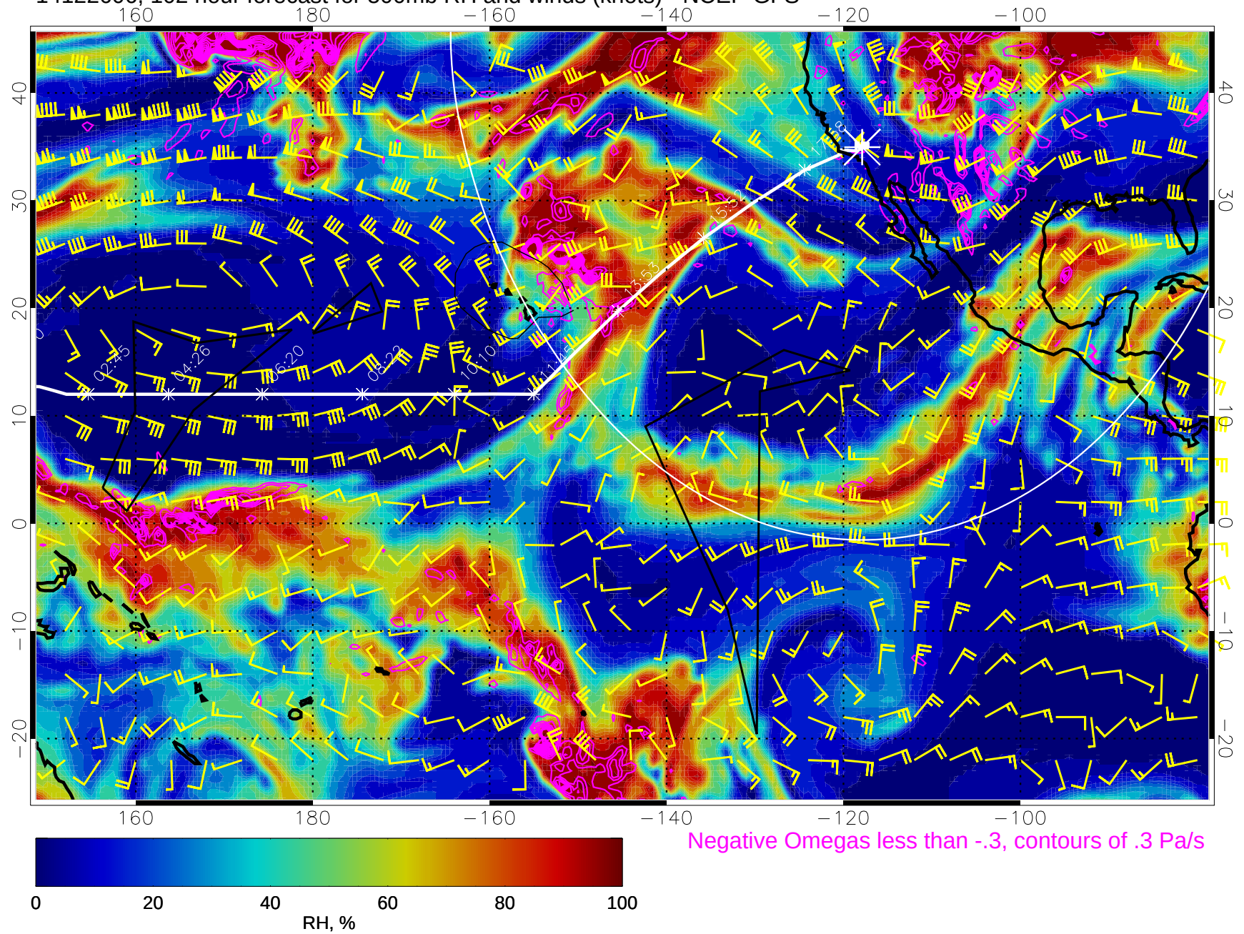
14122606, 102 hour forecast for 500mb RH and winds (knots) - NCEP GFS
