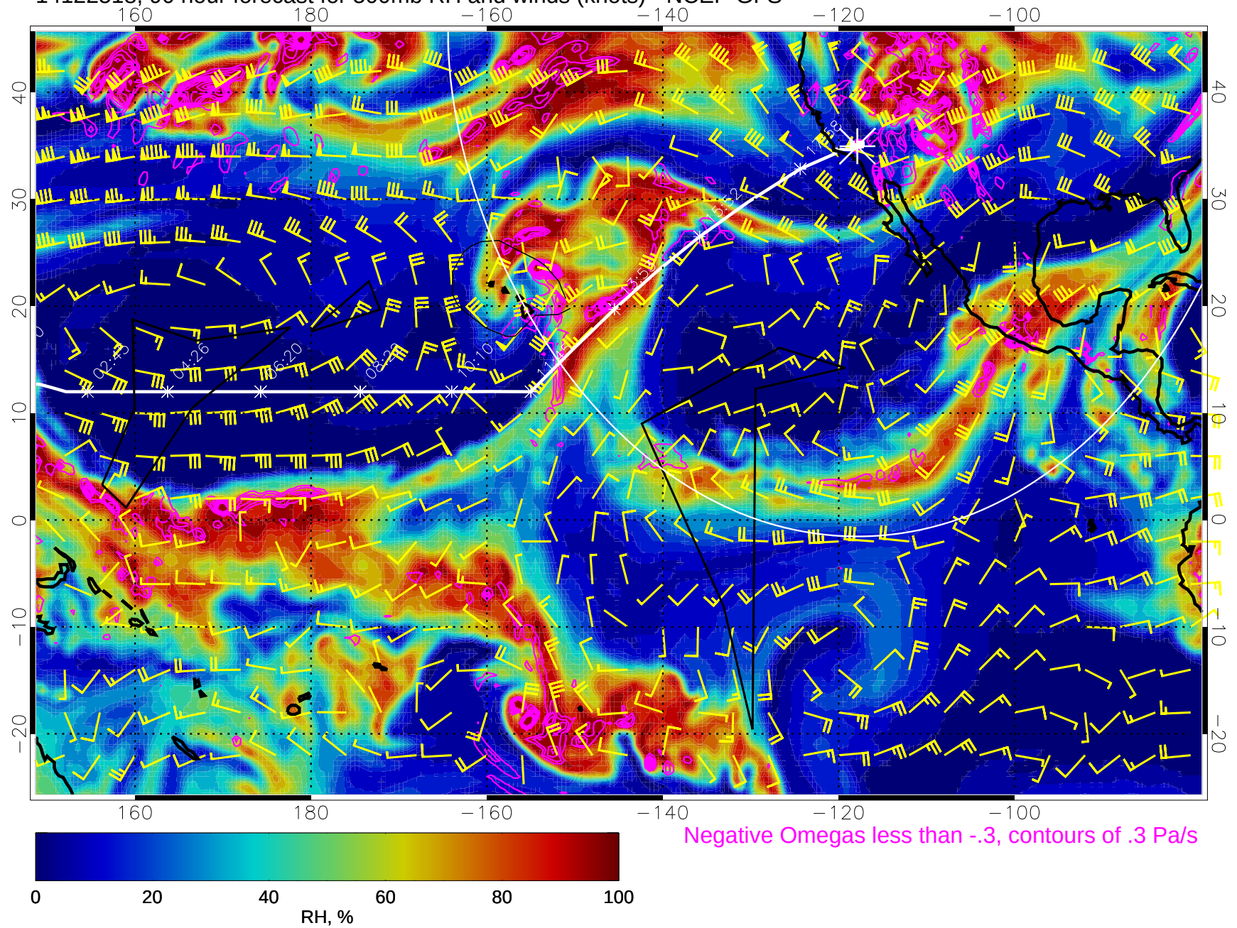
14122518, 90 hour forecast for 500mb RH and winds (knots) - NCEP GFS
