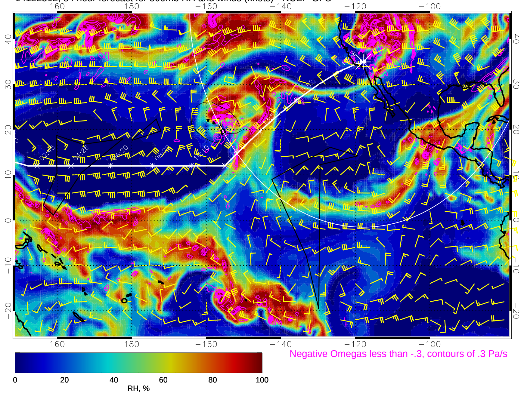
14122512, 84 hour forecast for 500mb RH and winds (knots) - NCEP GFS
