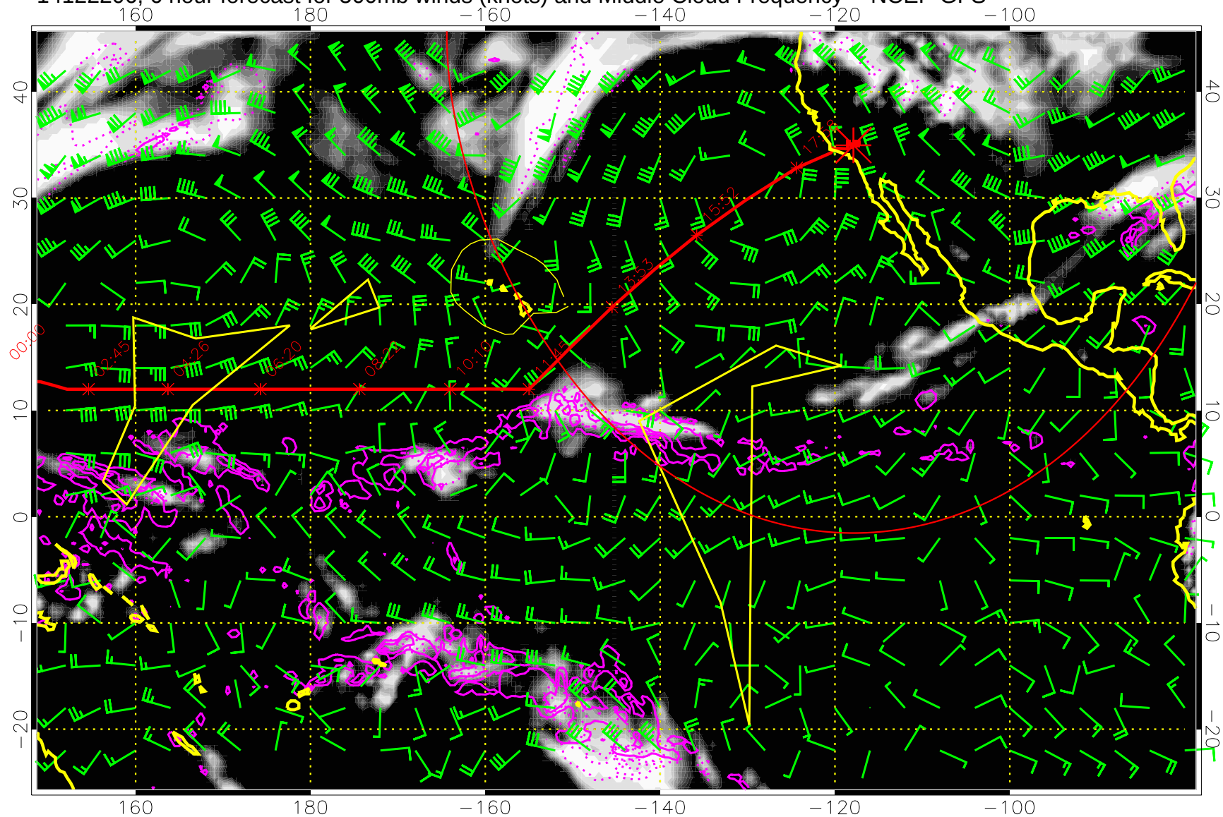
14122206, 6 hour forecast for 500mb winds (knots) and Middle Cloud Frequency -- NCEP GFS
