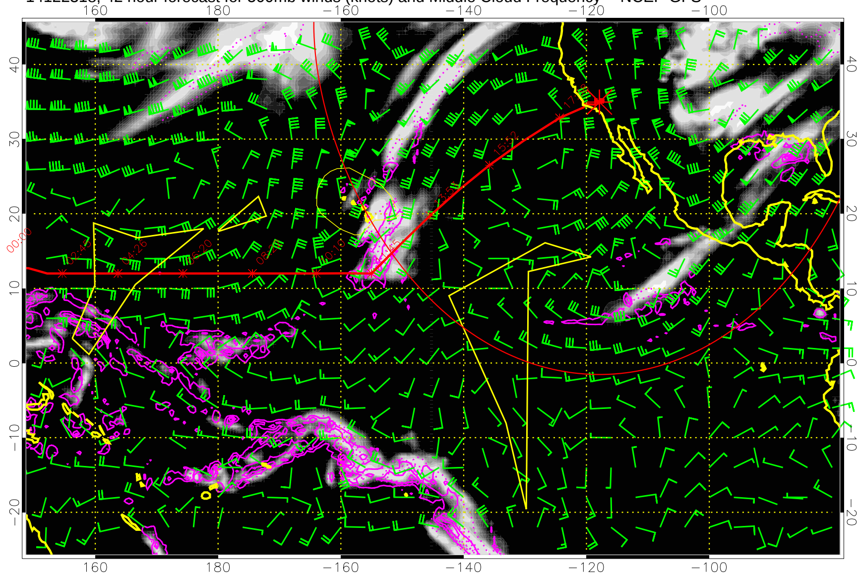
14122318, 42 hour forecast for 500mb winds (knots) and Middle Cloud Frequency -- NCEP GFS
