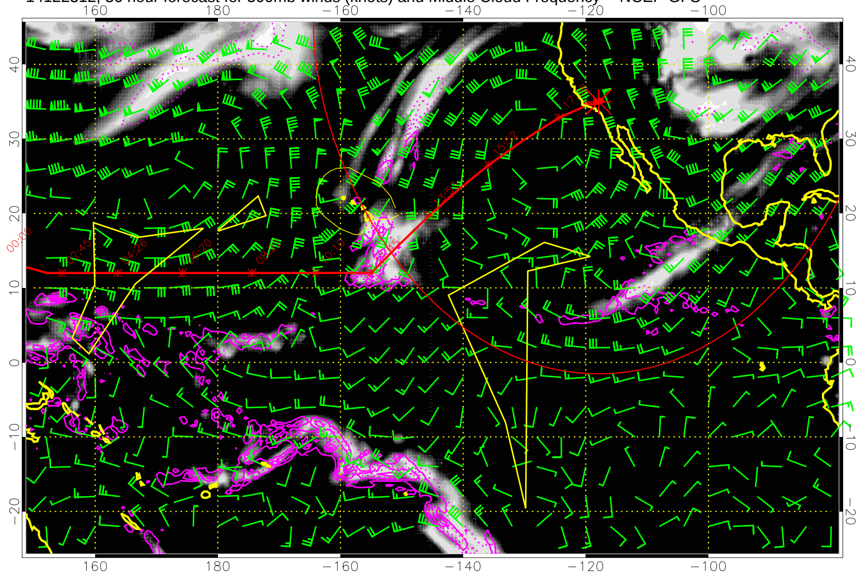
14122312, 36 hour forecast for 500mb winds (knots) and Middle Cloud Frequency -- NCEP GFS
