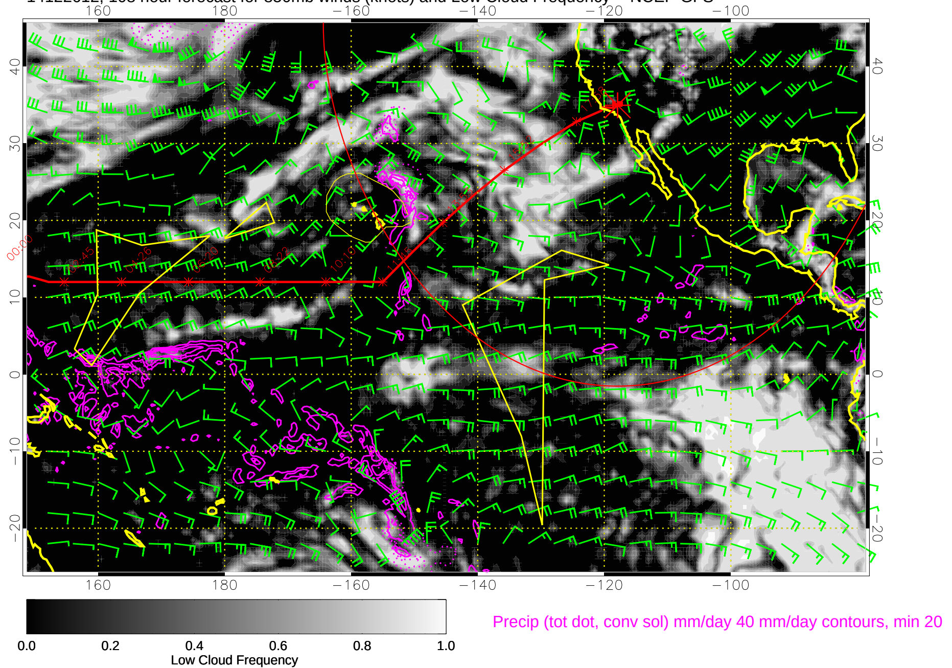
14122612, 108 hour forecast for 850mb winds (knots) and Low Cloud Frequency -- NCEP GFS
