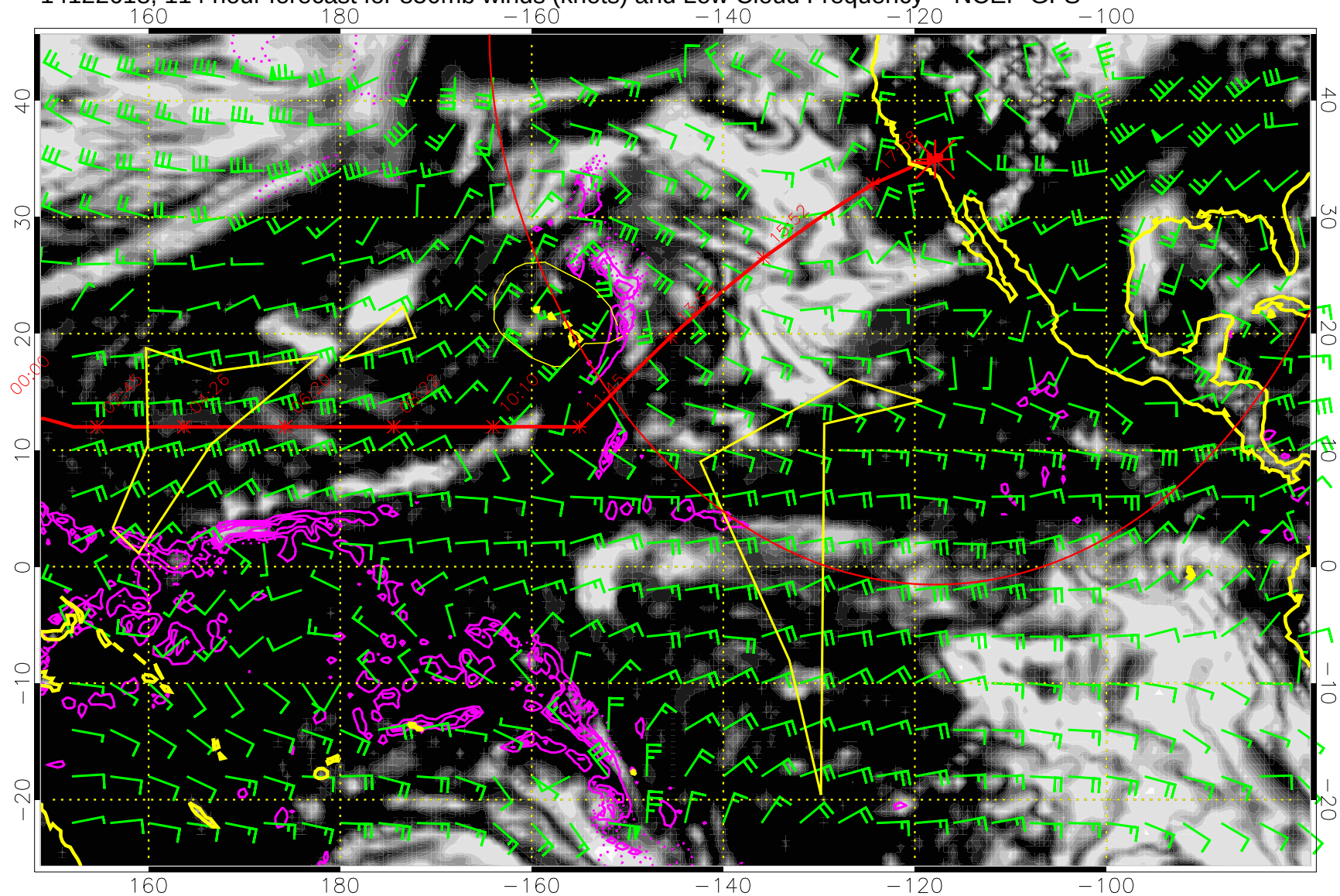
14122618, 114 hour forecast for 850mb winds (knots) and Low Cloud Frequency -- NCEP GFS
