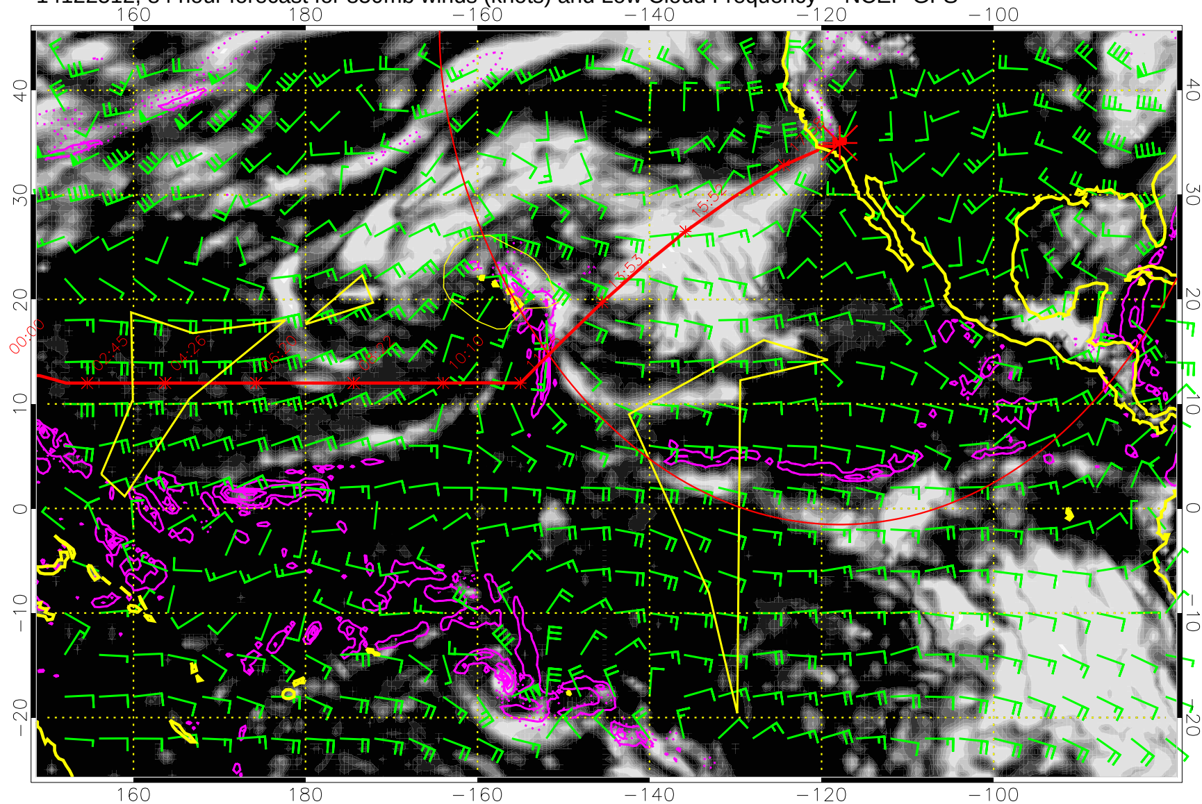
14122512, 84 hour forecast for 850mb winds (knots) and Low Cloud Frequency -- NCEP GFS
