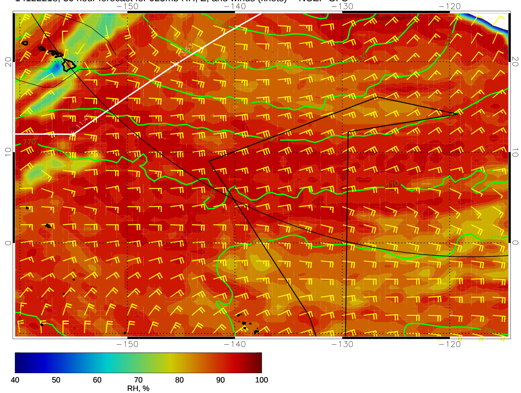
14122218, 30 hour forecast for 925mb RH, Z, and winds (knots) -- NCEP GFS
