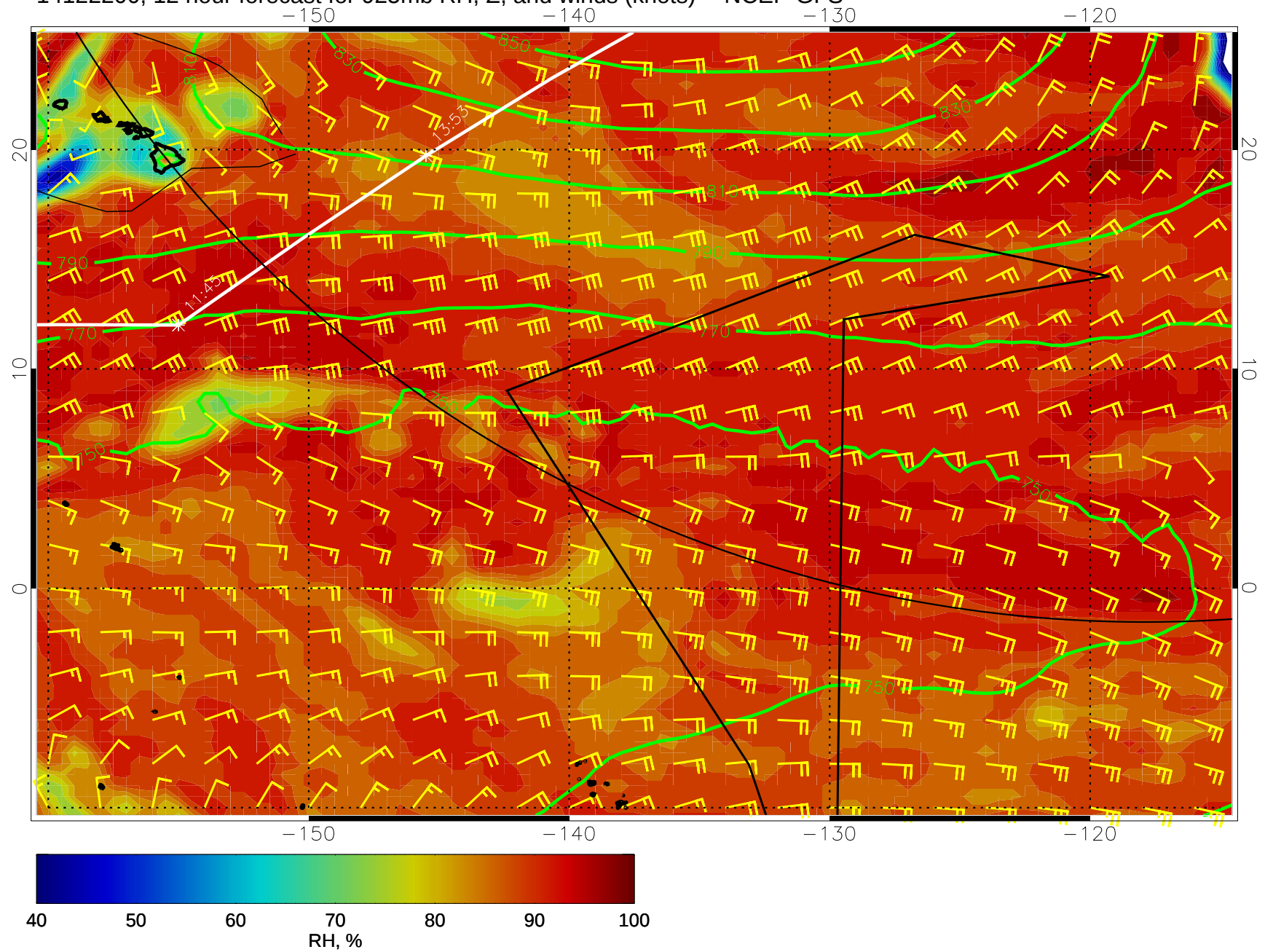
14122200, 12 hour forecast for 925mb RH, Z, and winds (knots) -- NCEP GFS
