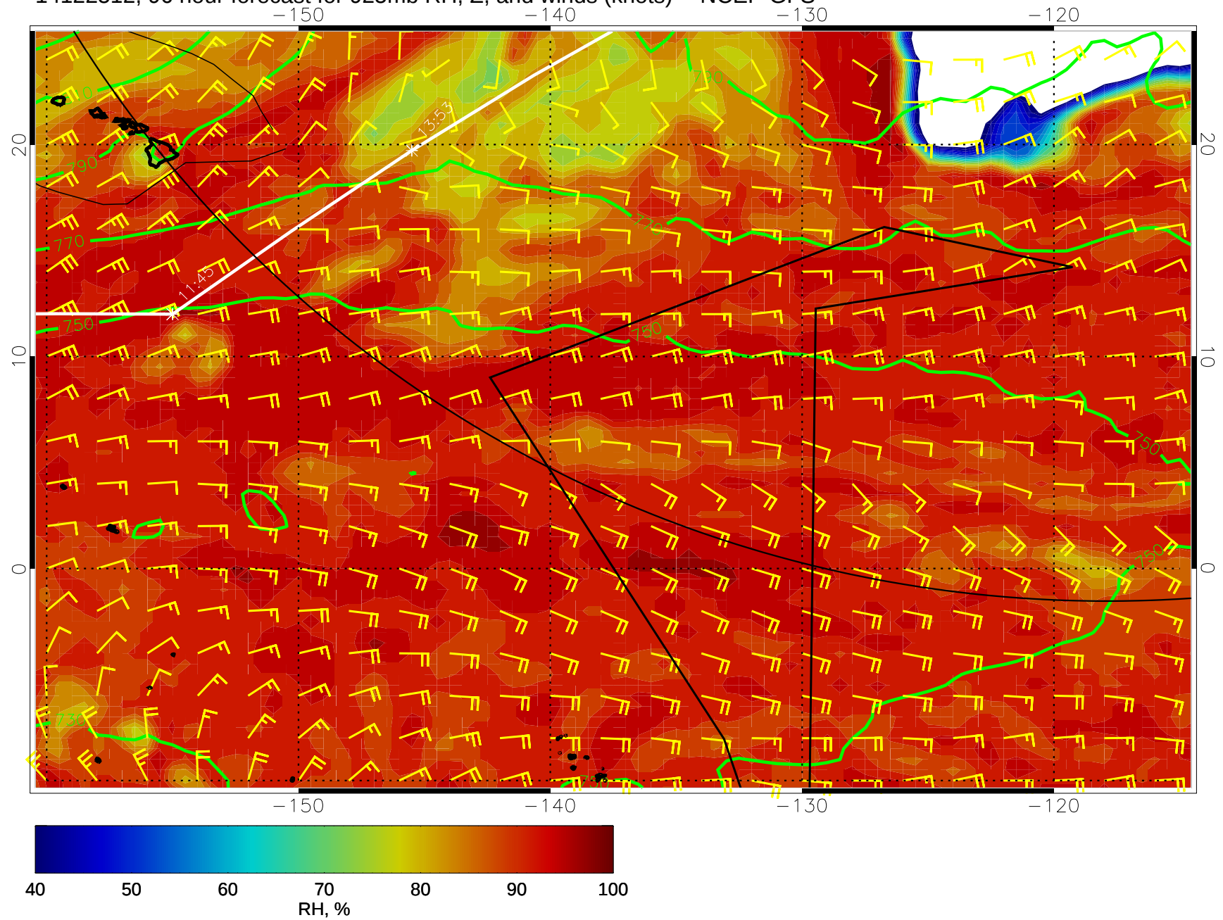
14122512, 96 hour forecast for 925mb RH, Z, and winds (knots) -- NCEP GFS
