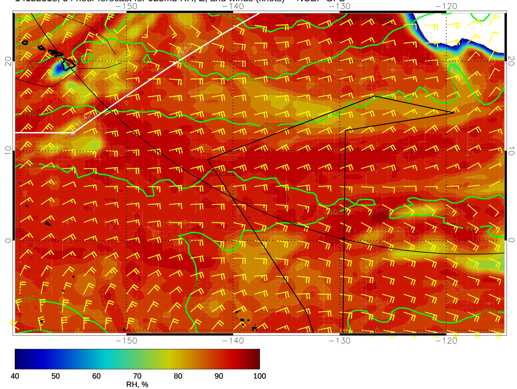
14122318, 54 hour forecast for 925mb RH, Z, and winds (knots) -- NCEP GFS
