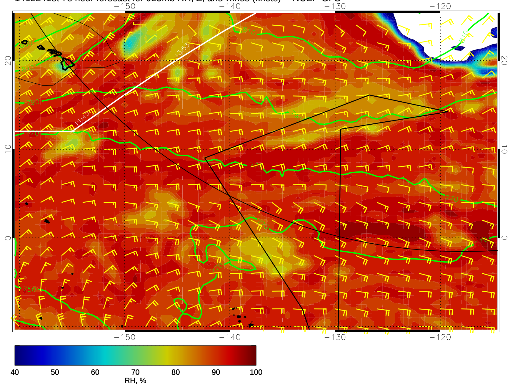
14122418, 78 hour forecast for 925mb RH, Z, and winds (knots) -- NCEP GFS
