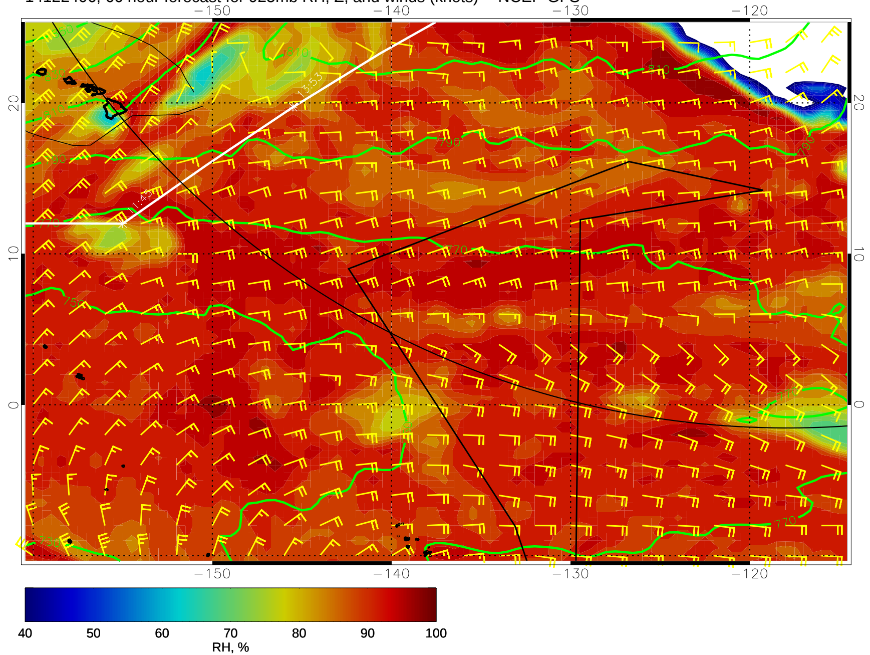
14122406, 66 hour forecast for 925mb RH, Z, and winds (knots) -- NCEP GFS
