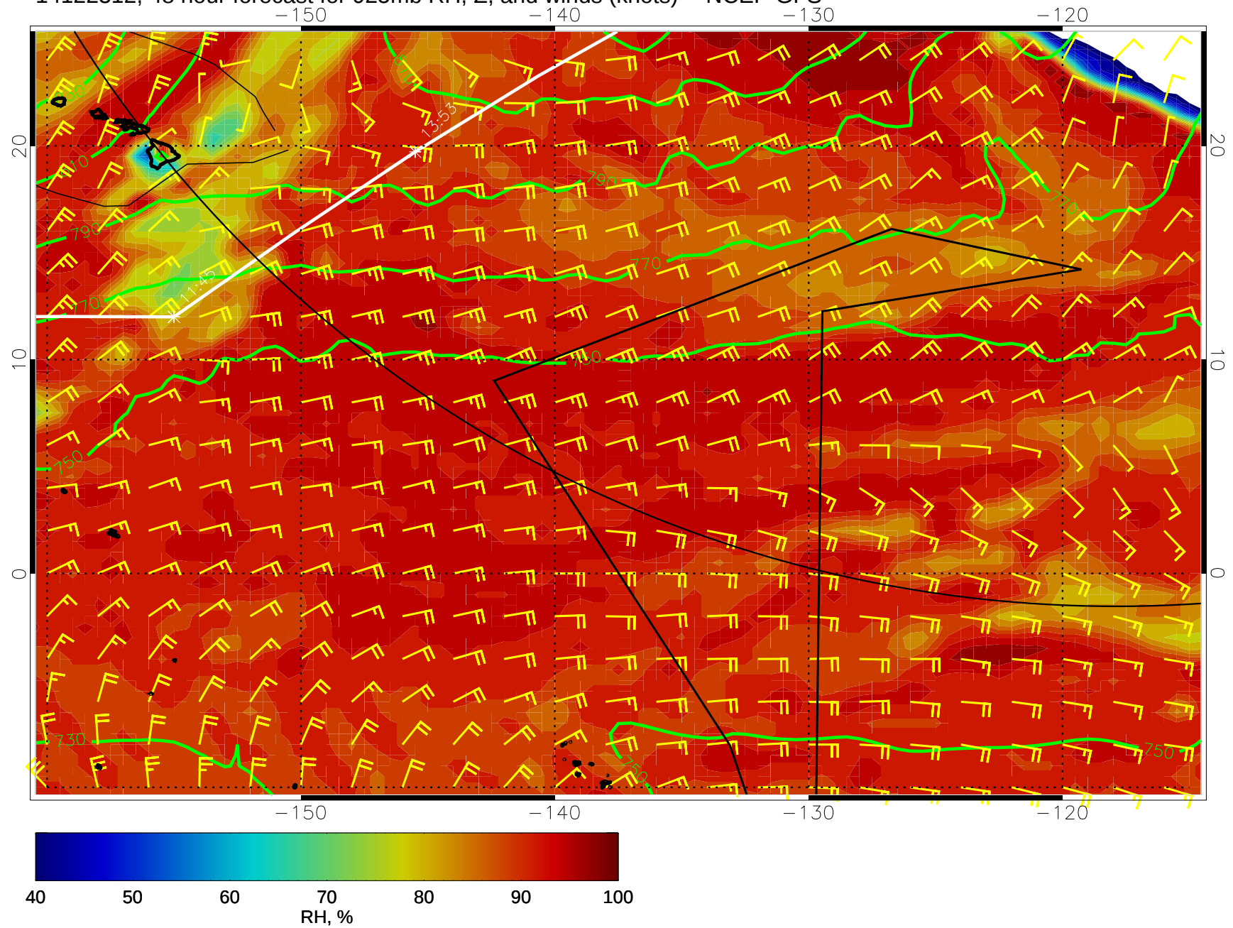
14122312, 48 hour forecast for 925mb RH, Z, and winds (knots) -- NCEP GFS
