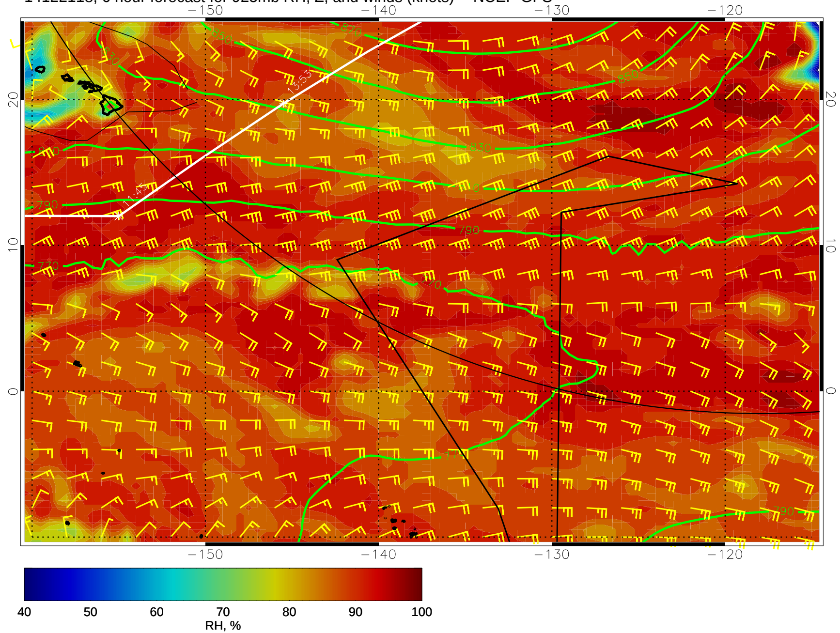
14122118, 6 hour forecast for 925mb RH, Z, and winds (knots) -- NCEP GFS
