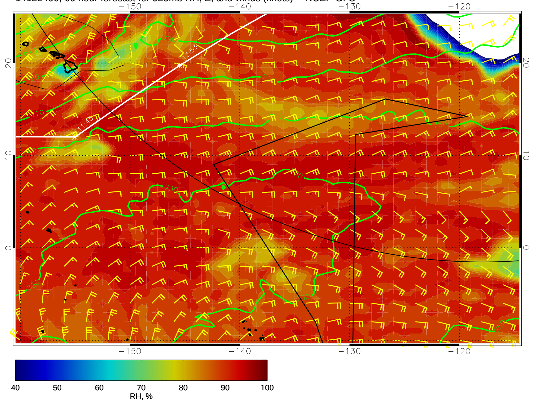
14122400, 60 hour forecast for 925mb RH, Z, and winds (knots) -- NCEP GFS
