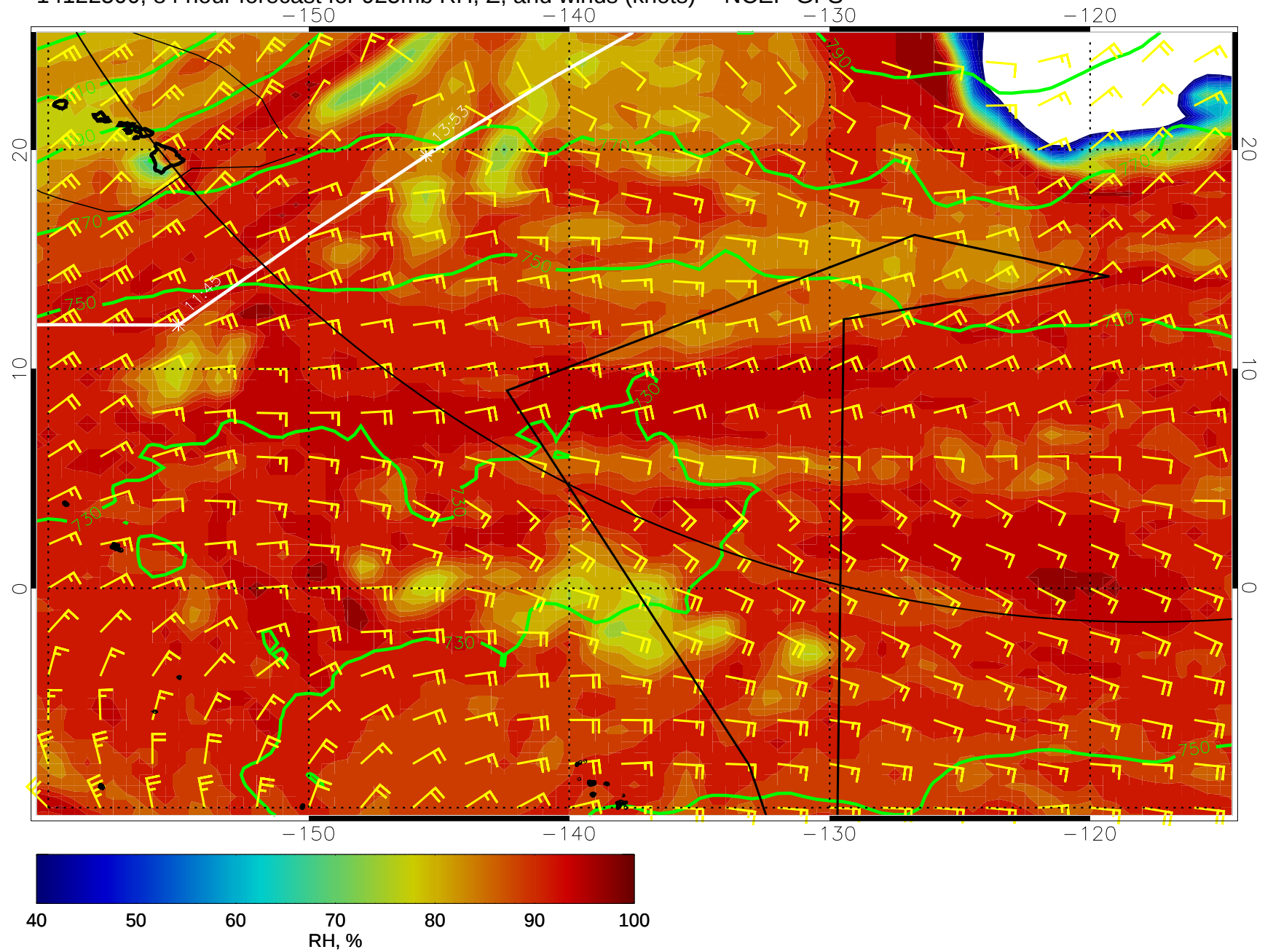
14122500, 84 hour forecast for 925mb RH, Z, and winds (knots) -- NCEP GFS
