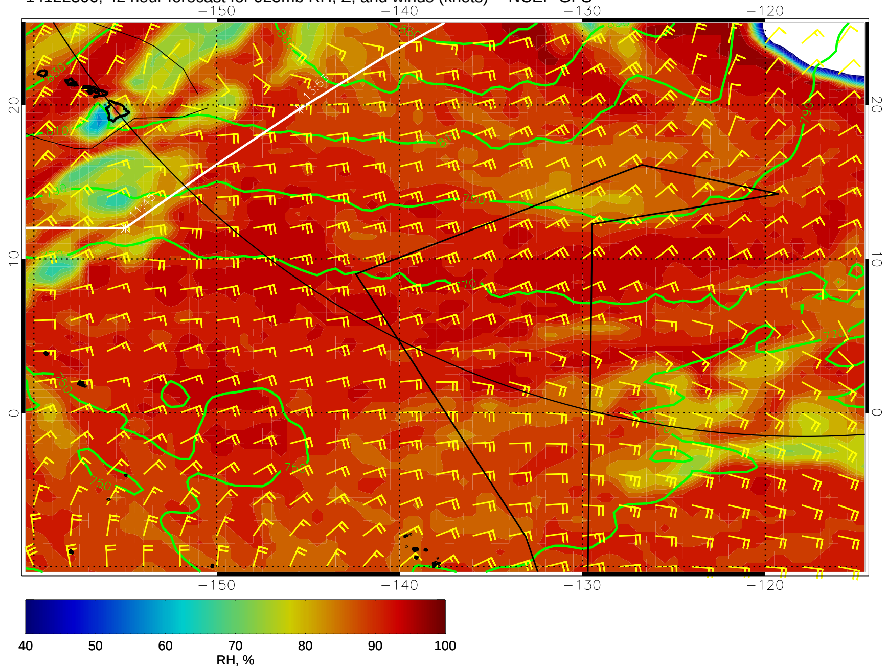
14122306, 42 hour forecast for 925mb RH, Z, and winds (knots) -- NCEP GFS
