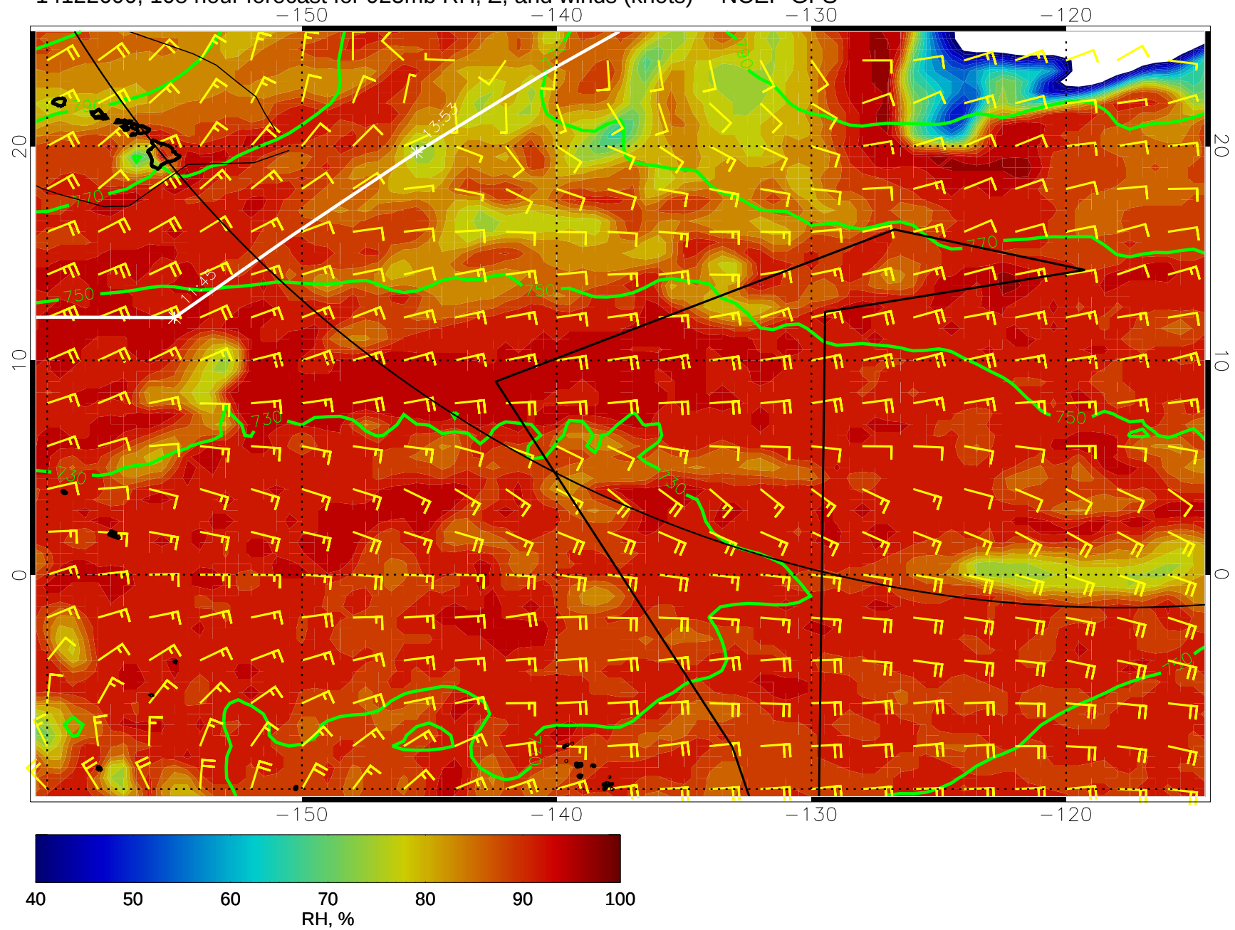
14122600, 108 hour forecast for 925mb RH, Z, and winds (knots) -- NCEP GFS
