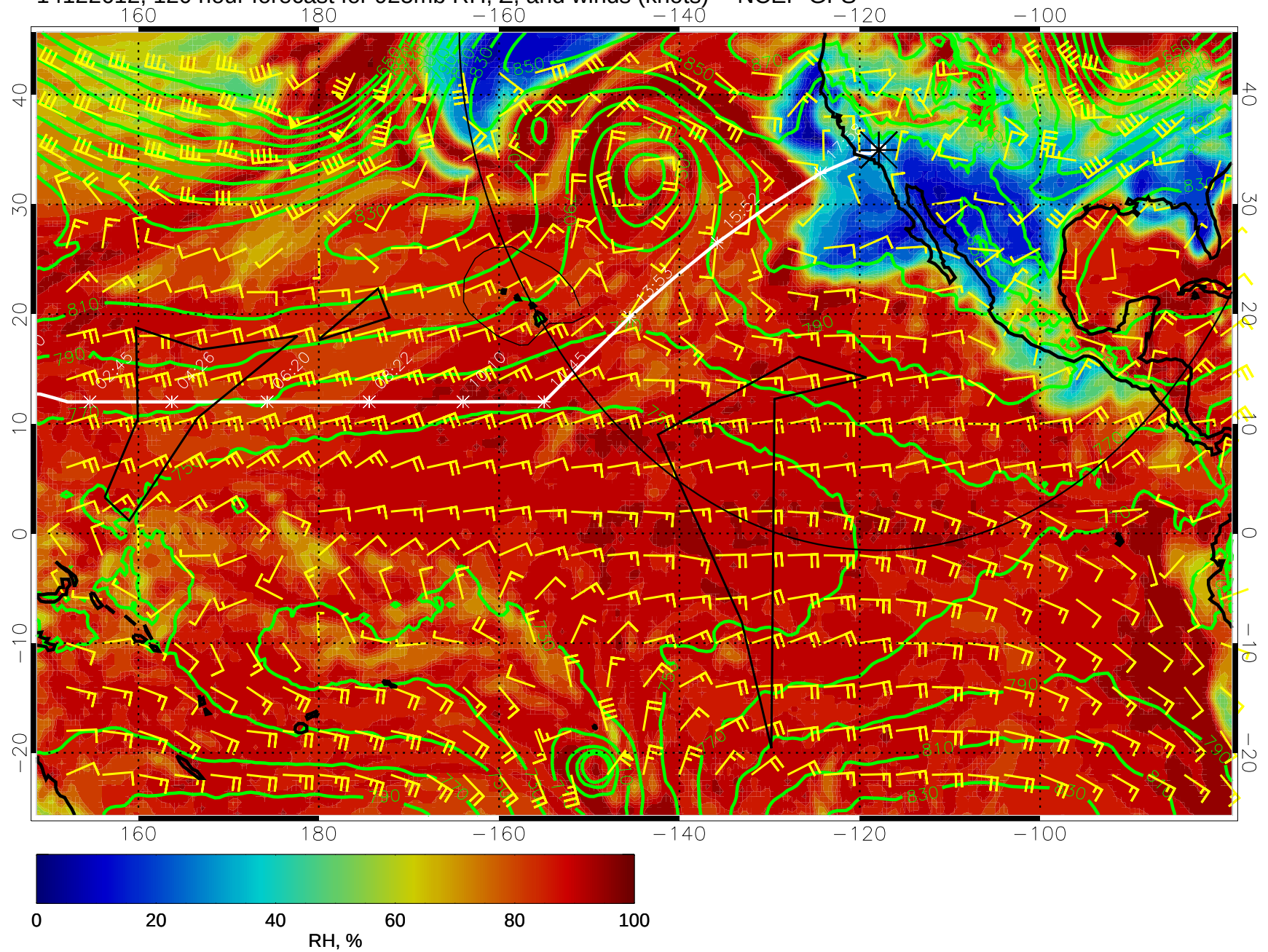
14122612, 120 hour forecast for 925mb RH, Z, and winds (knots) -- NCEP GFS
