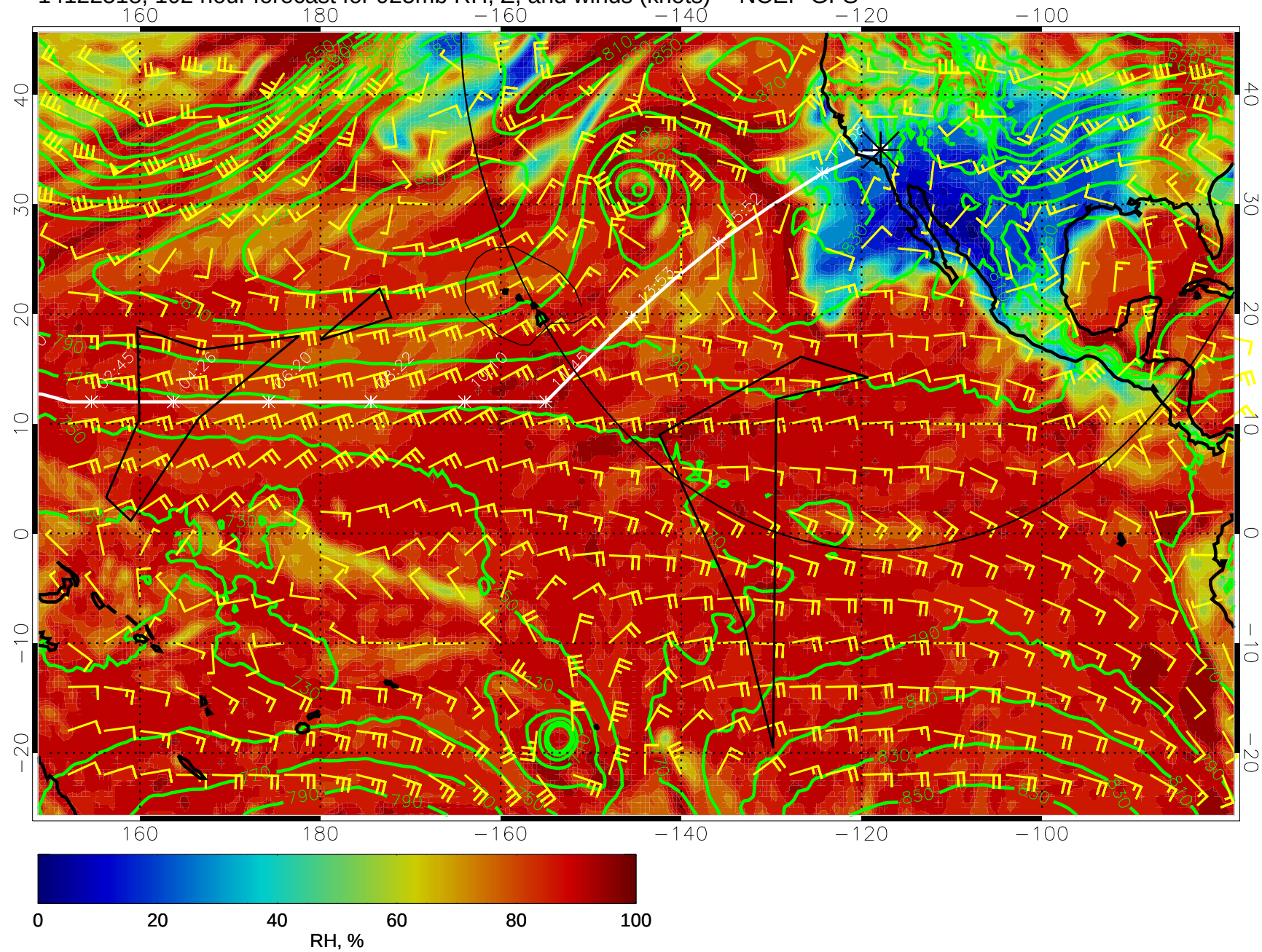
14122518, 102 hour forecast for 925mb RH, Z, and winds (knots) -- NCEP GFS
