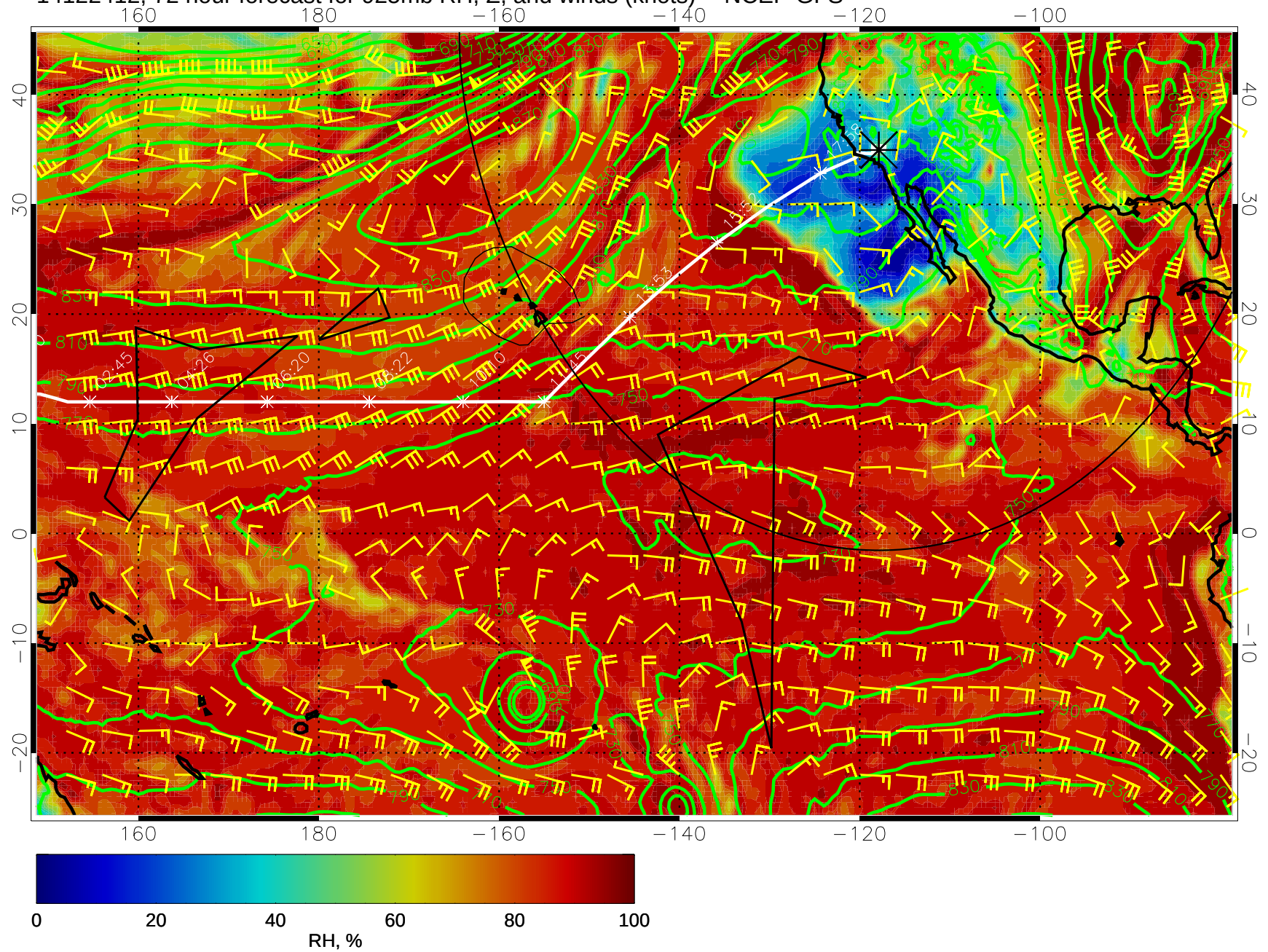
14122412, 72 hour forecast for 925mb RH, Z, and winds (knots) -- NCEP GFS
