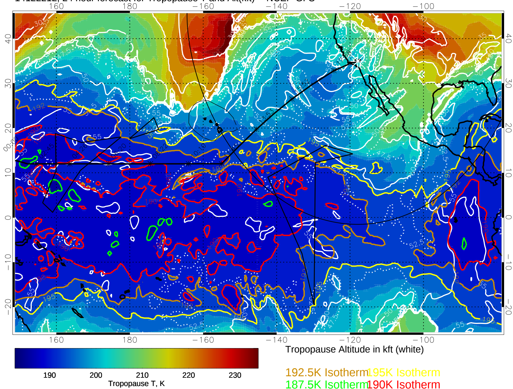
14122212, 24 hour forecast for Tropopause T and Alt(kft) -- NCEP GFS
