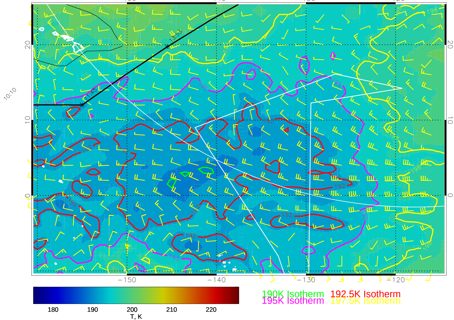
14122418, 78 hour forecast for 70mb T and winds (knots) -- NCEP GFS
