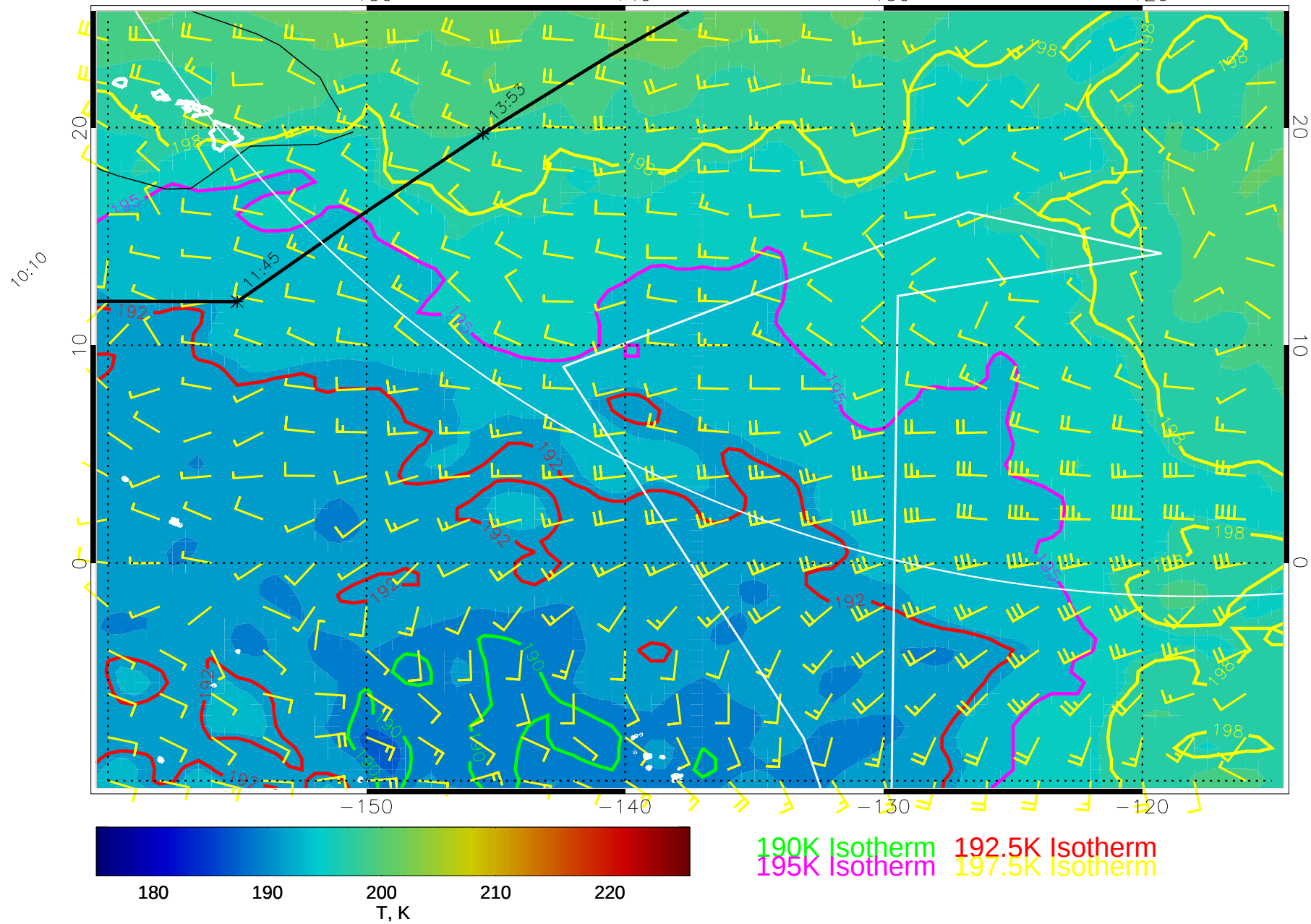
14122512, 96 hour forecast for 70mb T and winds (knots) -- NCEP GFS
