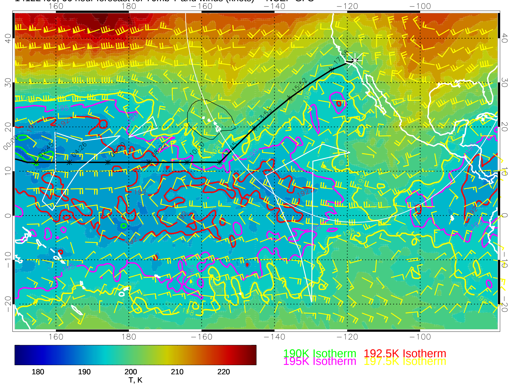
14122406, 66 hour forecast for 70mb T and winds (knots) -- NCEP GFS
