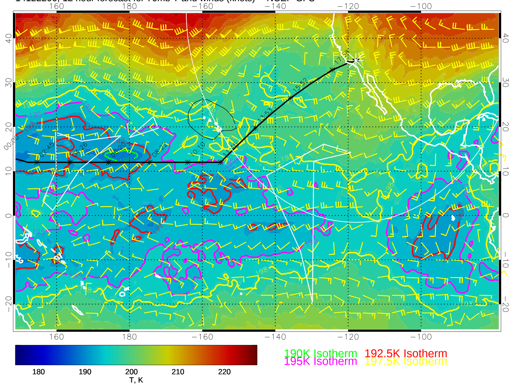
14122200, 12 hour forecast for 70mb T and winds (knots) -- NCEP GFS
