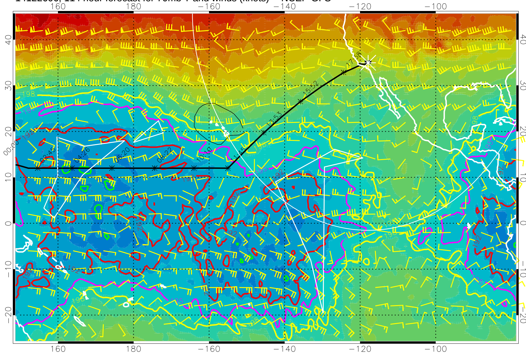
14122606, 114 hour forecast for 70mb T and winds (knots) -- NCEP GFS
