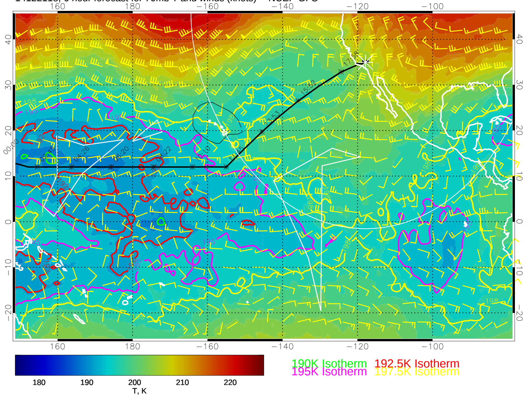
14122118, 6 hour forecast for 70mb T and winds (knots) -- NCEP GFS
