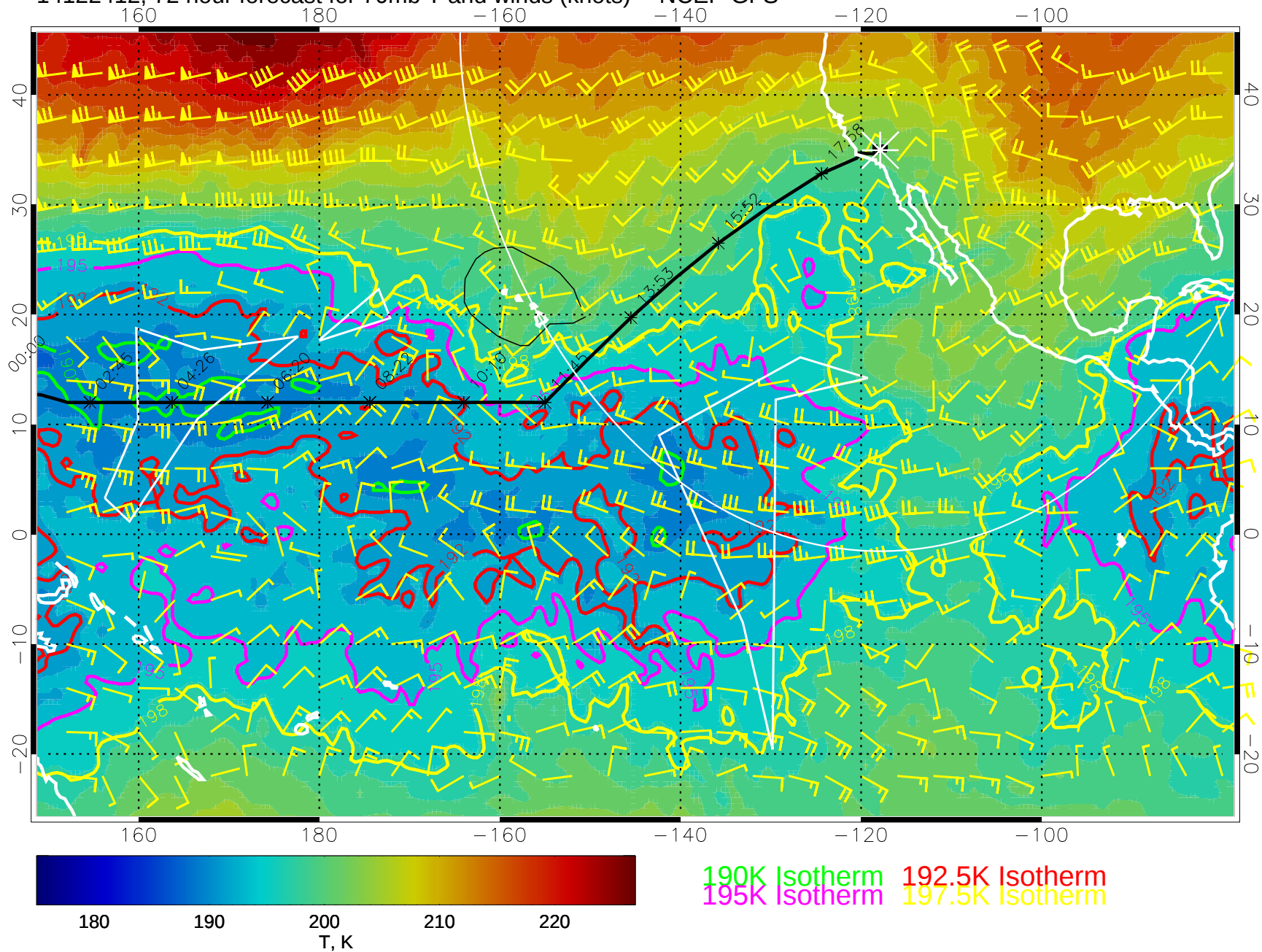
14122412, 72 hour forecast for 70mb T and winds (knots) -- NCEP GFS
