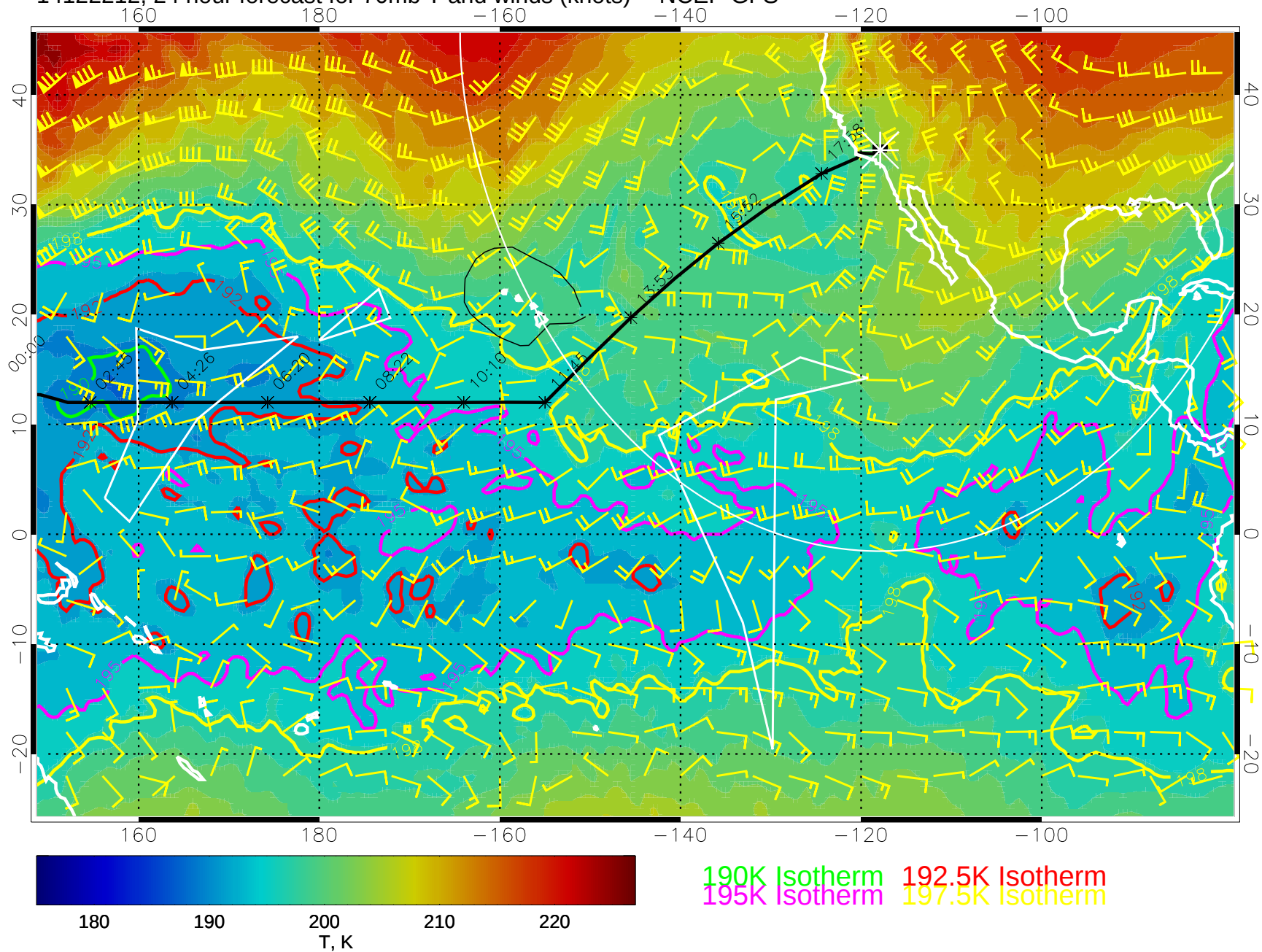
14122212, 24 hour forecast for 70mb T and winds (knots) -- NCEP GFS
