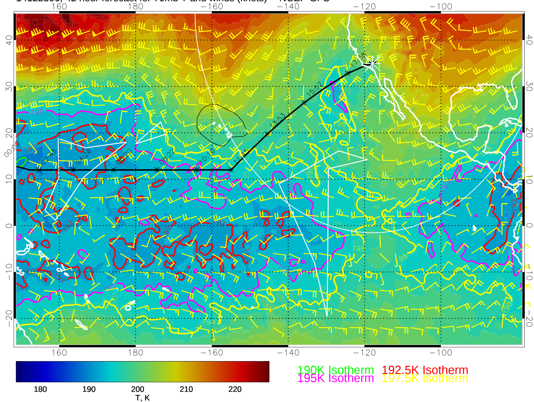
14122306, 42 hour forecast for 70mb T and winds (knots) -- NCEP GFS
