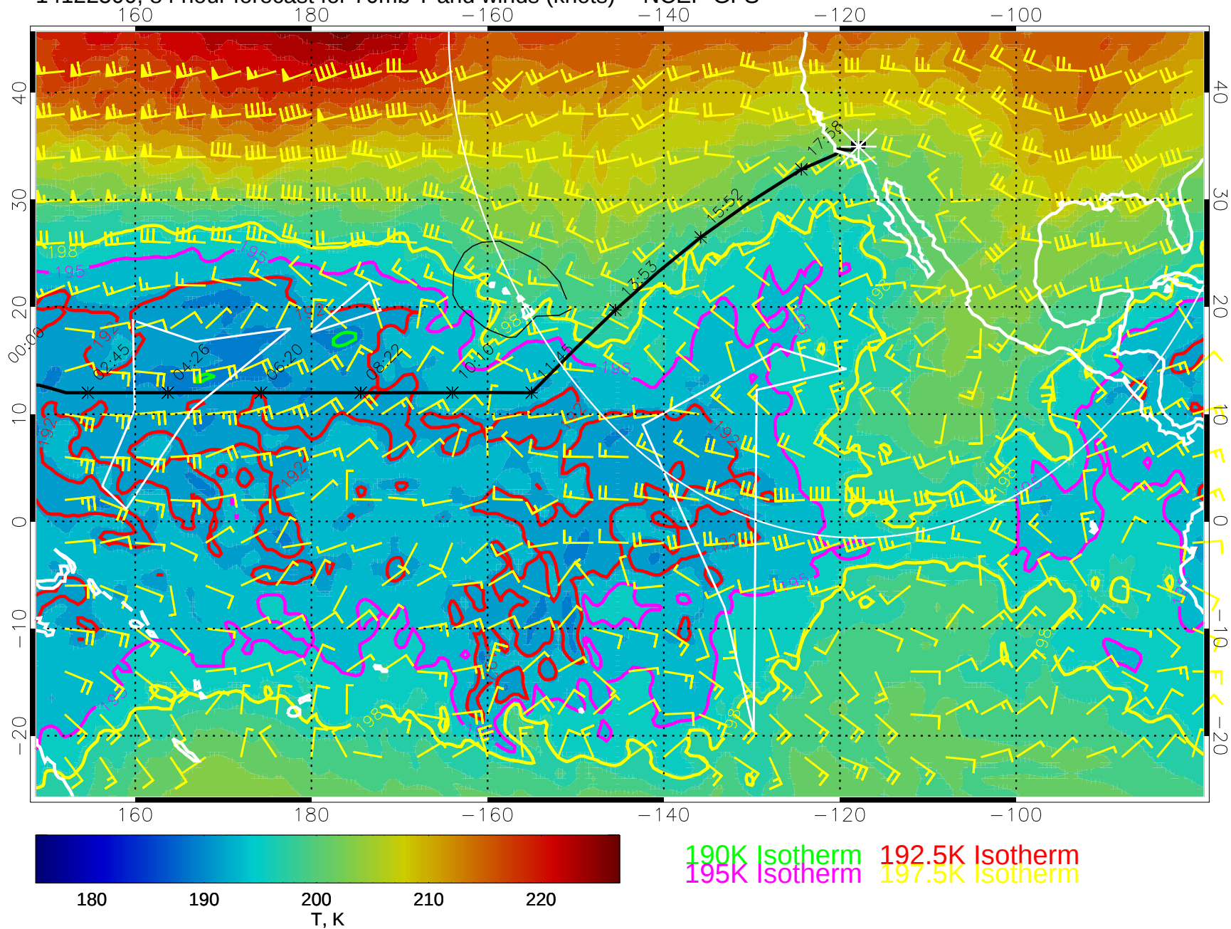
14122500, 84 hour forecast for 70mb T and winds (knots) -- NCEP GFS
