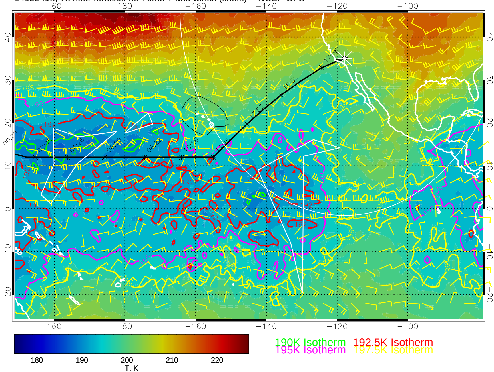
14122418, 78 hour forecast for 70mb T and winds (knots) -- NCEP GFS
