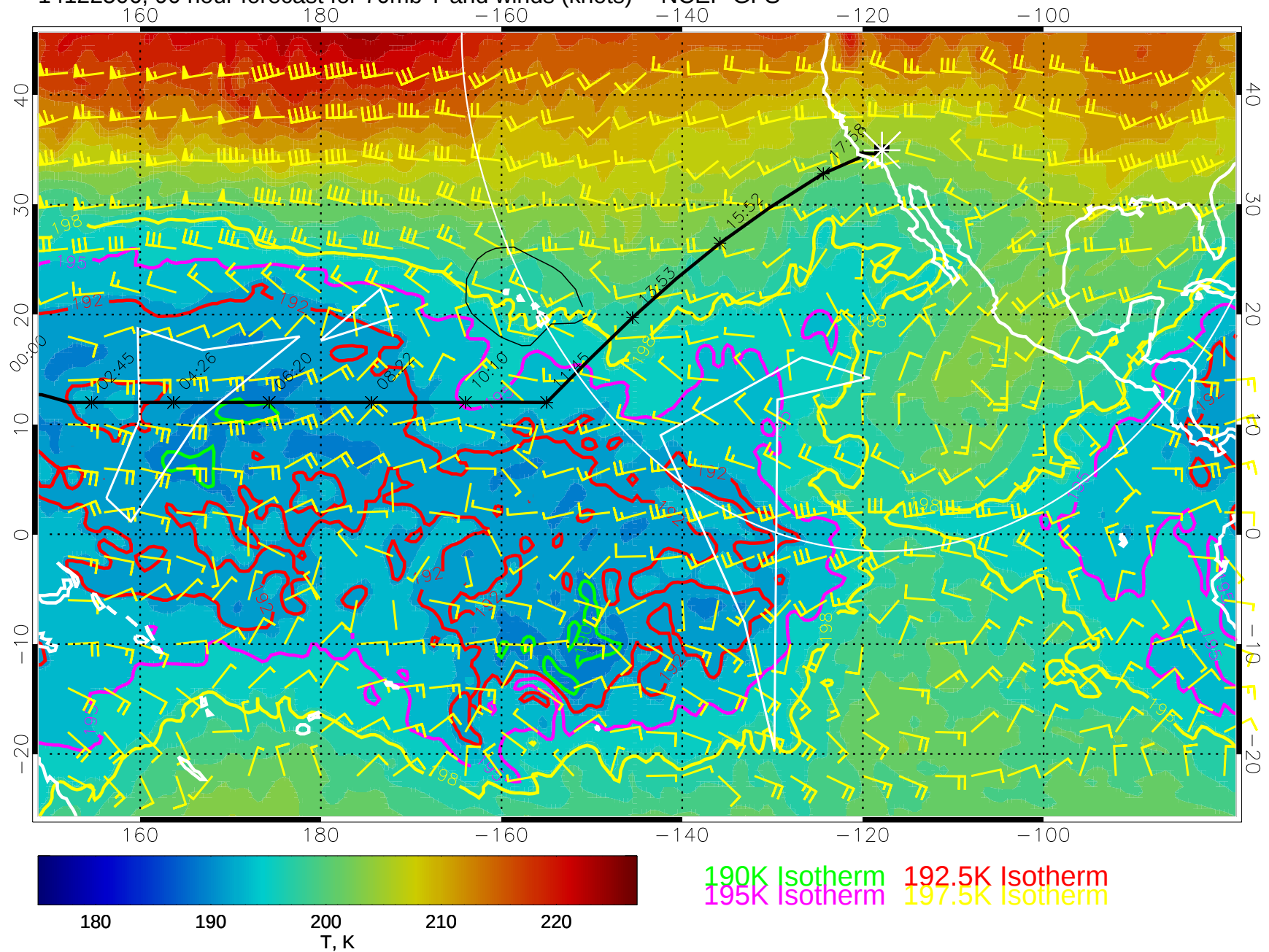
14122506, 90 hour forecast for 70mb T and winds (knots) -- NCEP GFS
