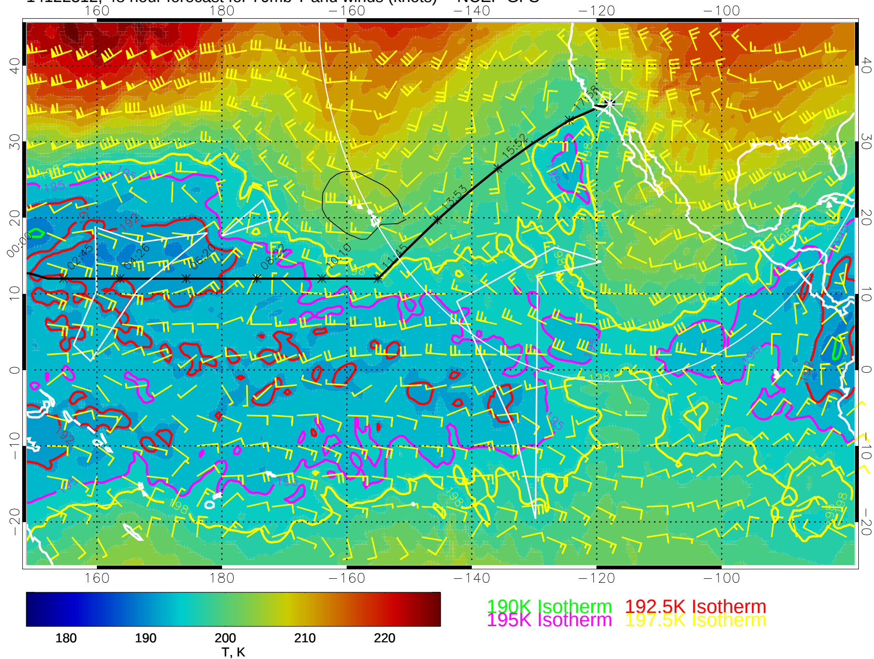
14122312, 48 hour forecast for 70mb T and winds (knots) -- NCEP GFS
