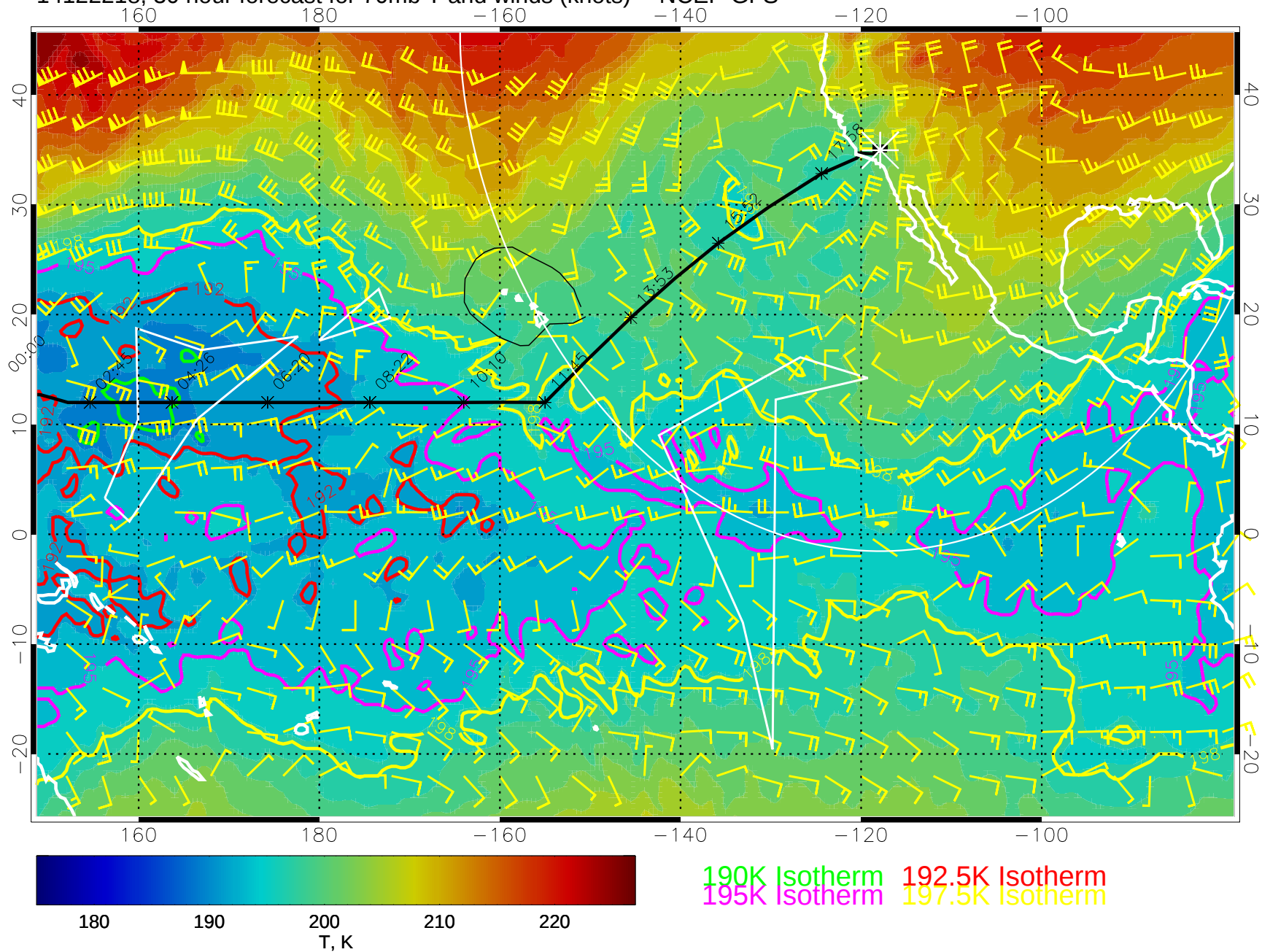
14122218, 30 hour forecast for 70mb T and winds (knots) -- NCEP GFS
