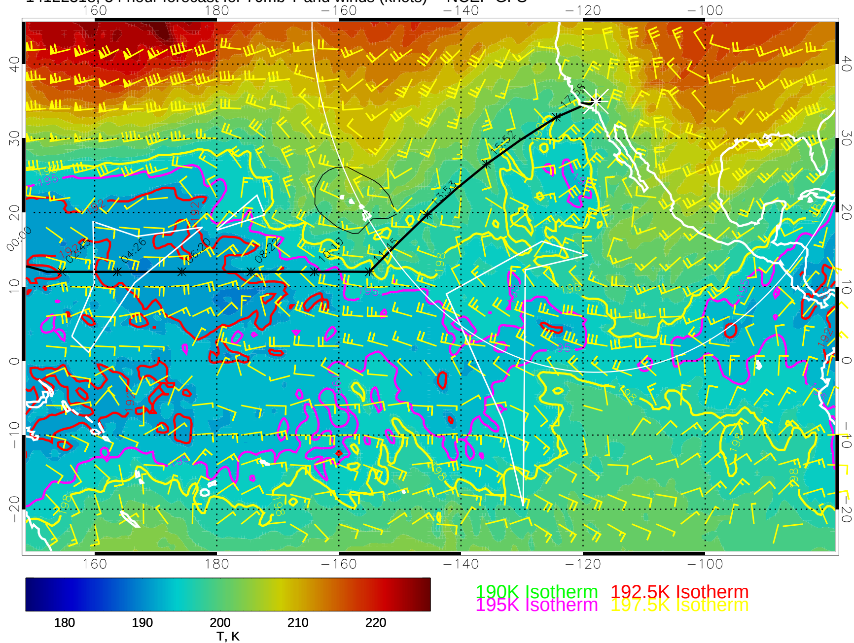
14122318, 54 hour forecast for 70mb T and winds (knots) -- NCEP GFS
