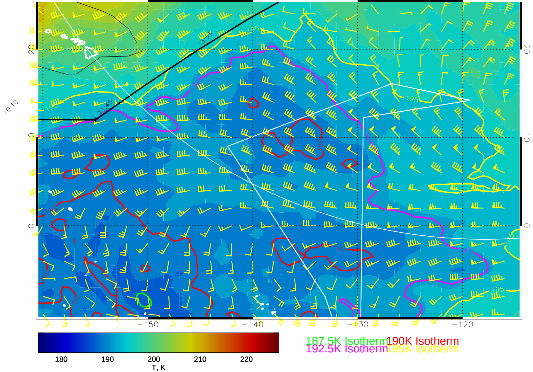
14122318, 54 hour forecast for 100mb T and winds (knots) -- NCEP GFS
