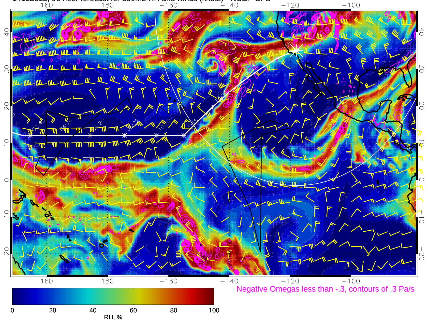
14122512, 96 hour forecast for 500mb RH and winds (knots) - NCEP GFS
