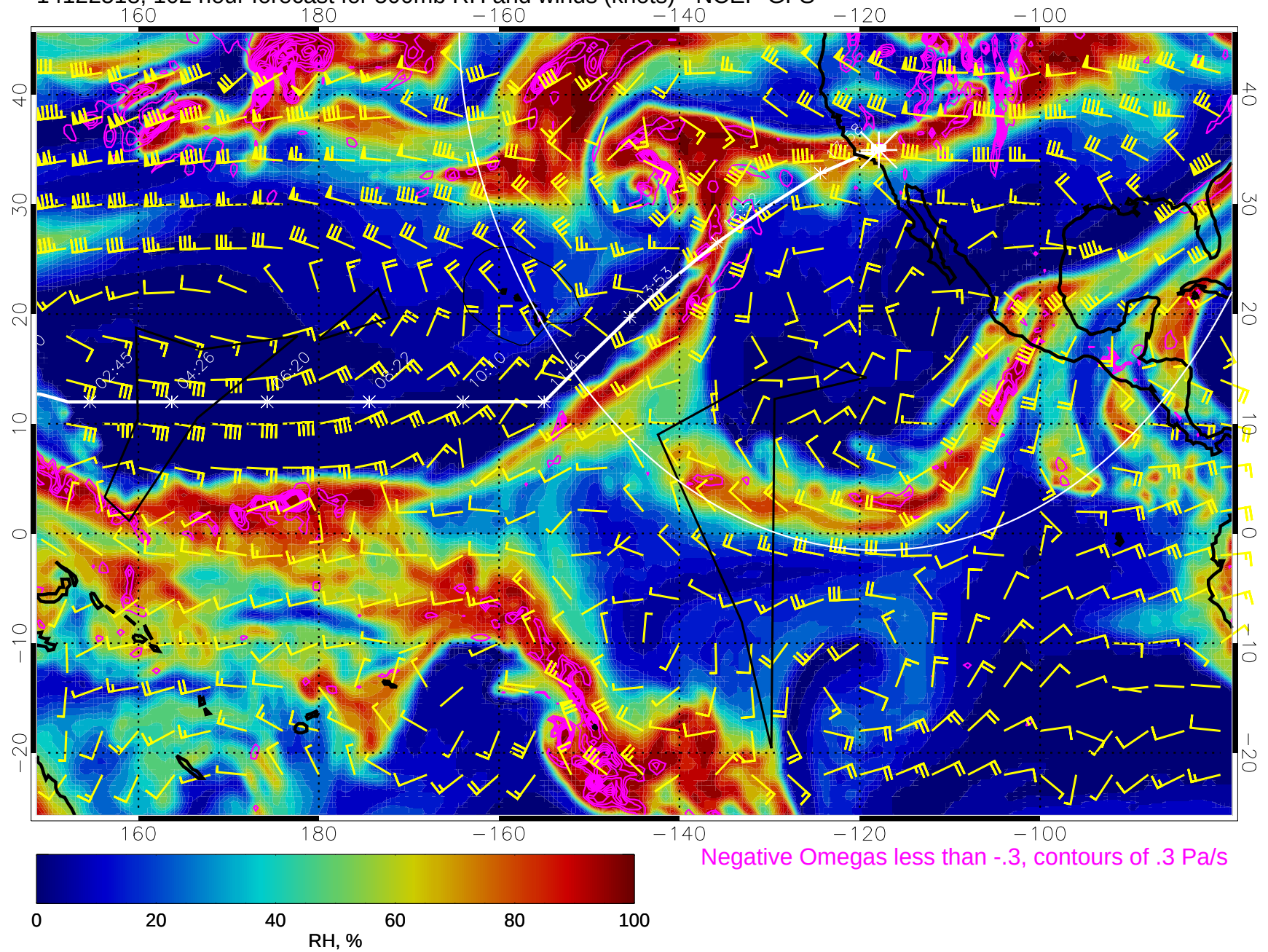
14122518, 102 hour forecast for 500mb RH and winds (knots) - NCEP GFS
