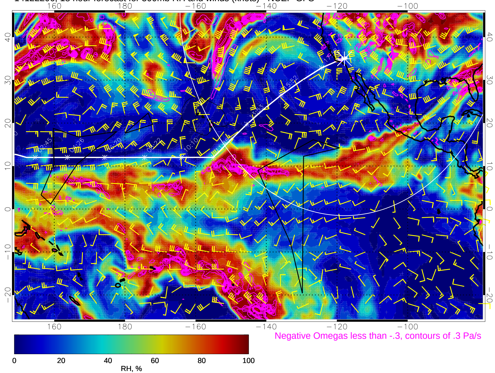
14122206, 18 hour forecast for 500mb RH and winds (knots) - NCEP GFS
