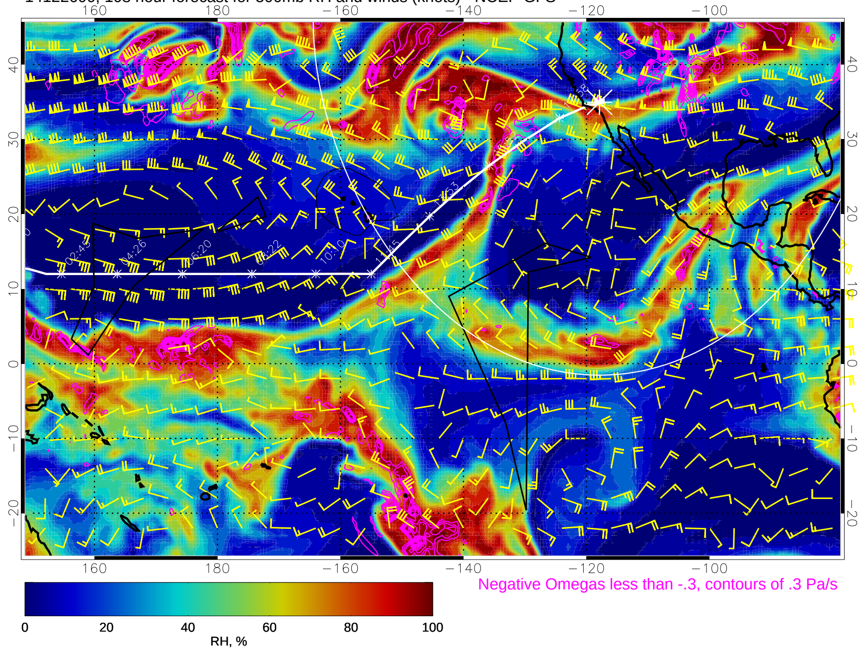
14122600, 108 hour forecast for 500mb RH and winds (knots) - NCEP GFS
