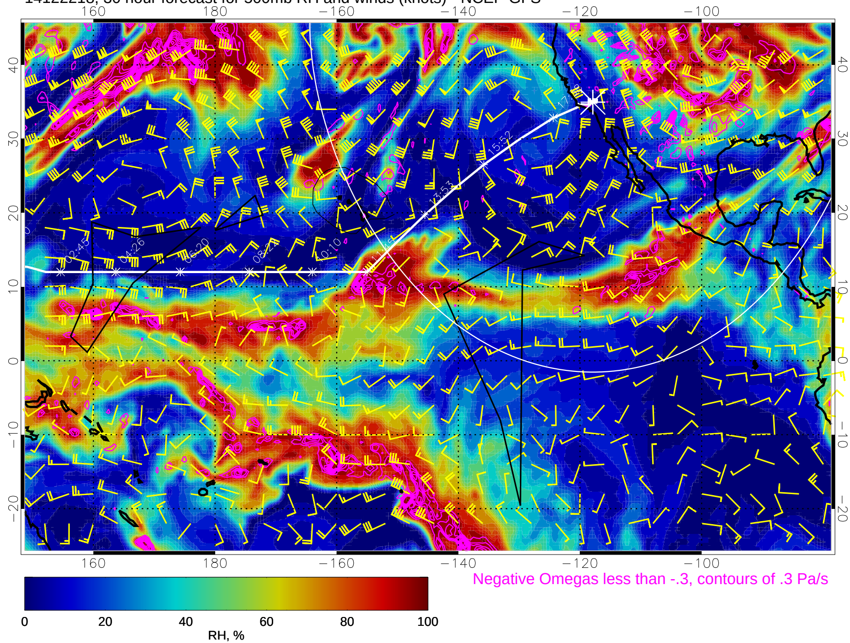
14122218, 30 hour forecast for 500mb RH and winds (knots) - NCEP GFS
