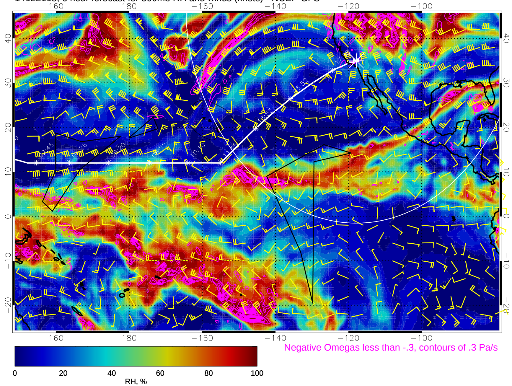
14122118, 6 hour forecast for 500mb RH and winds (knots) - NCEP GFS
