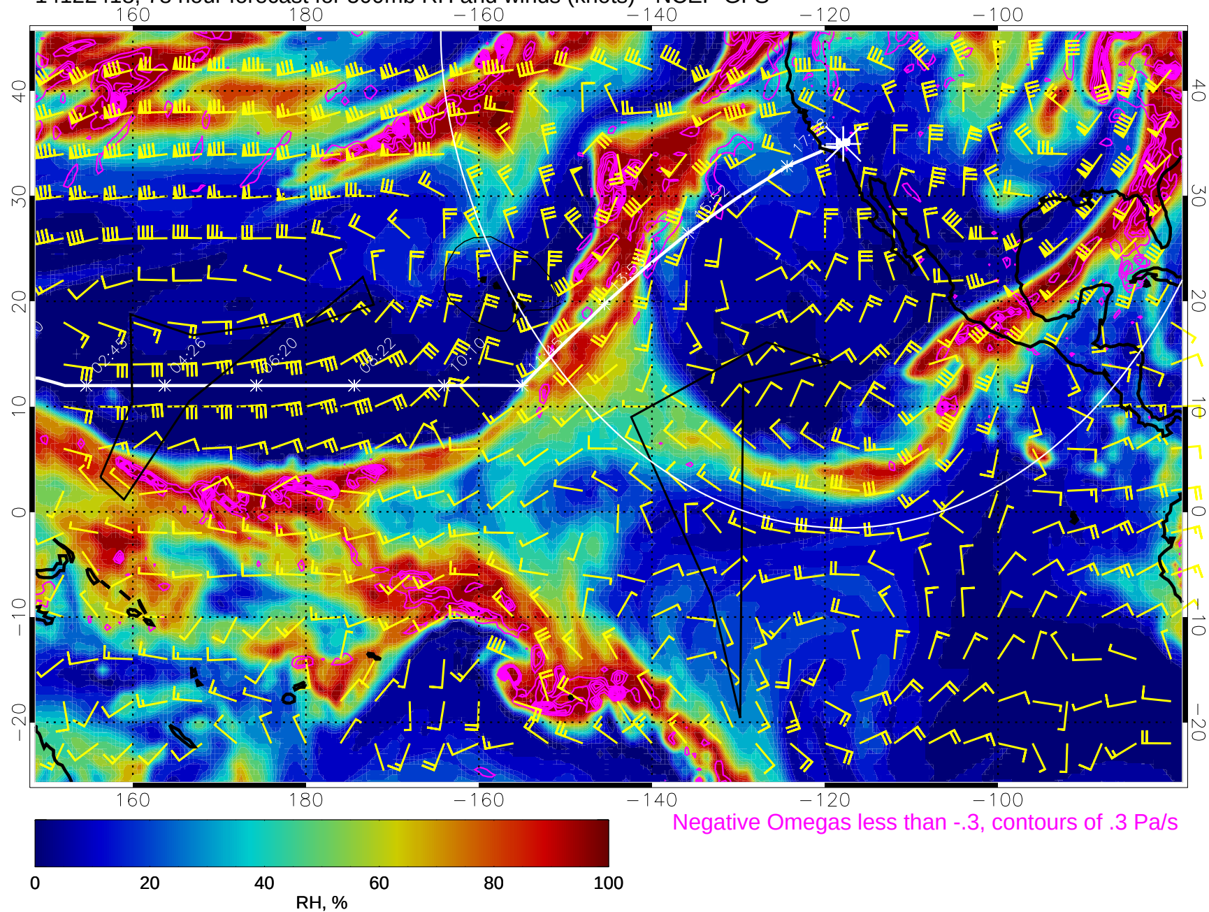
14122418, 78 hour forecast for 500mb RH and winds (knots) - NCEP GFS
