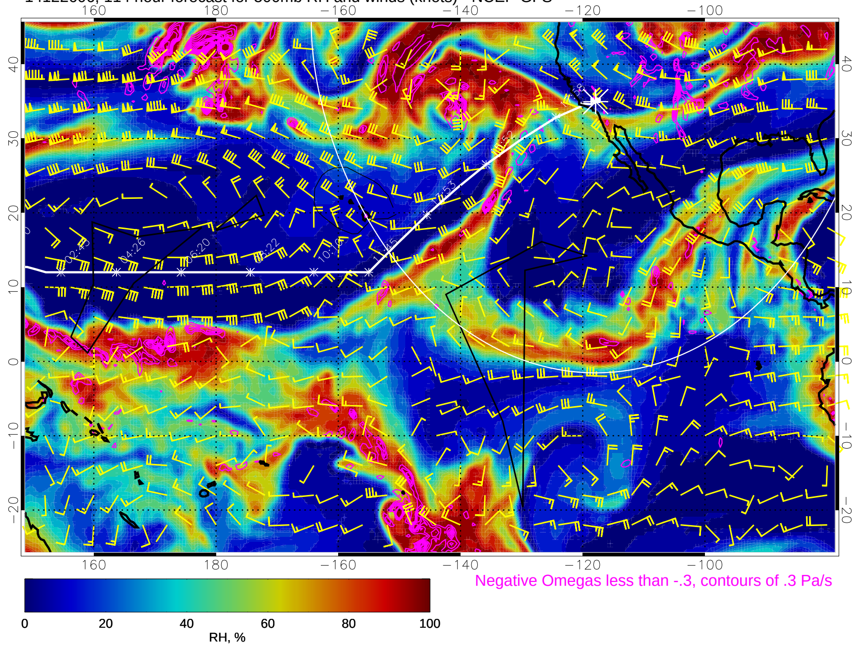
14122606, 114 hour forecast for 500mb RH and winds (knots) - NCEP GFS
