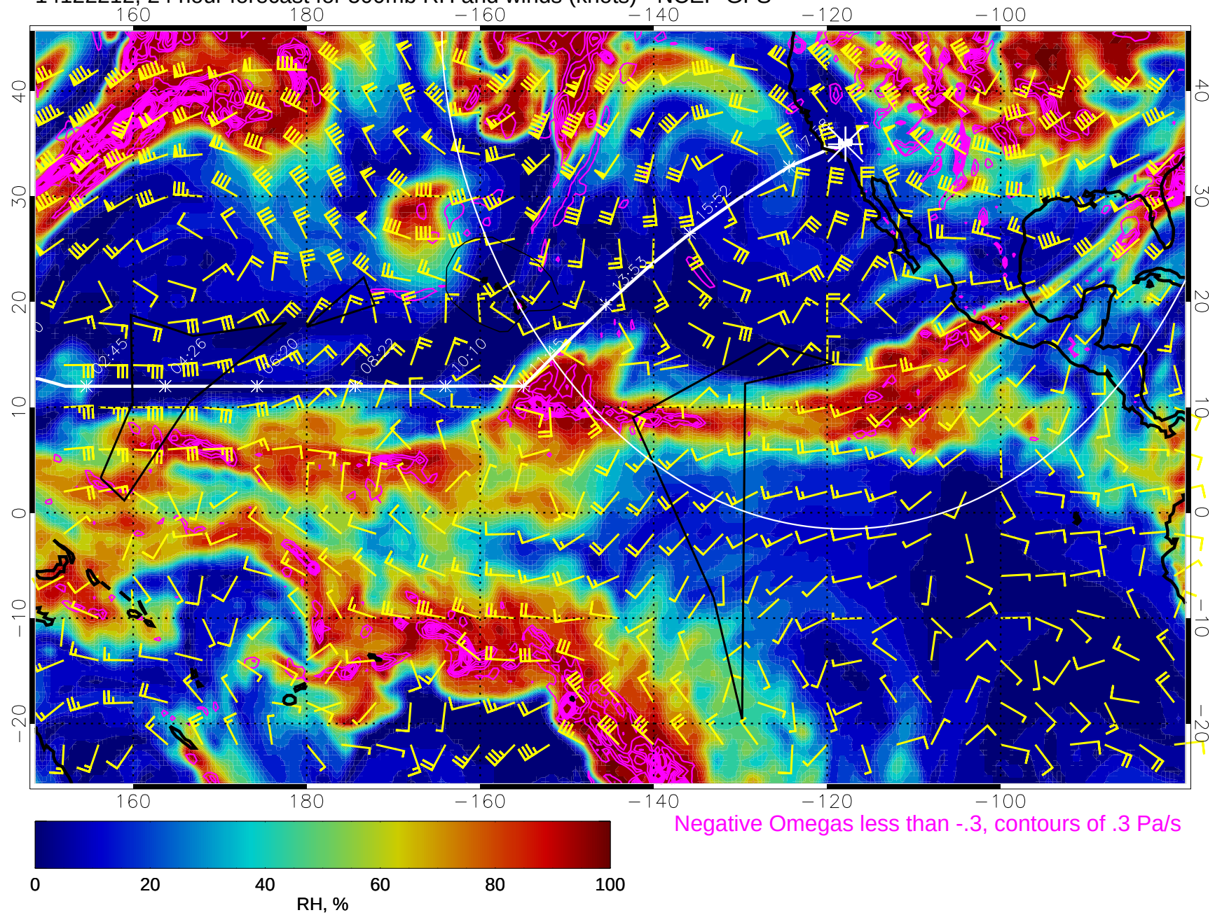
14122212, 24 hour forecast for 500mb RH and winds (knots) - NCEP GFS
