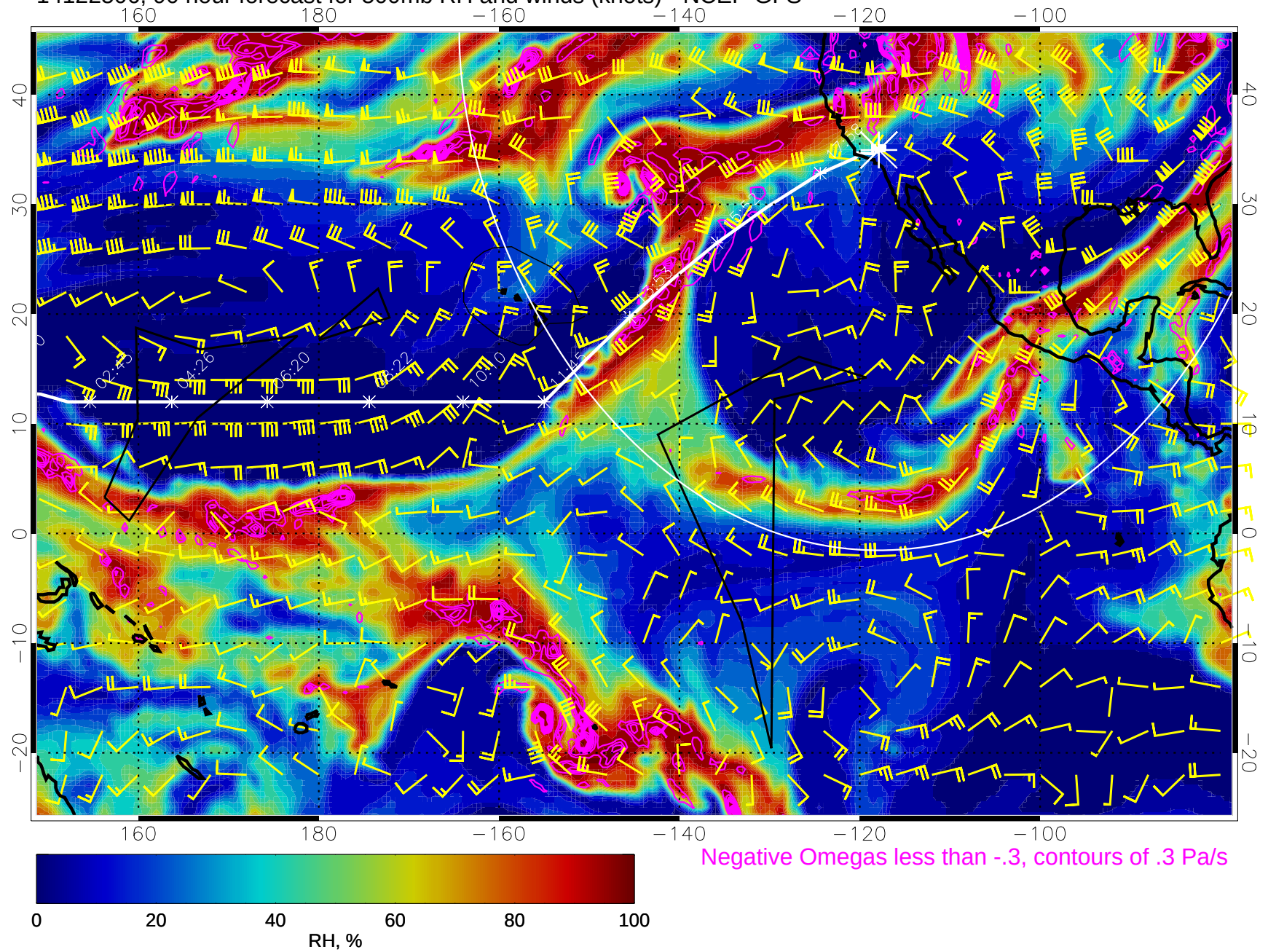
14122506, 90 hour forecast for 500mb RH and winds (knots) - NCEP GFS
