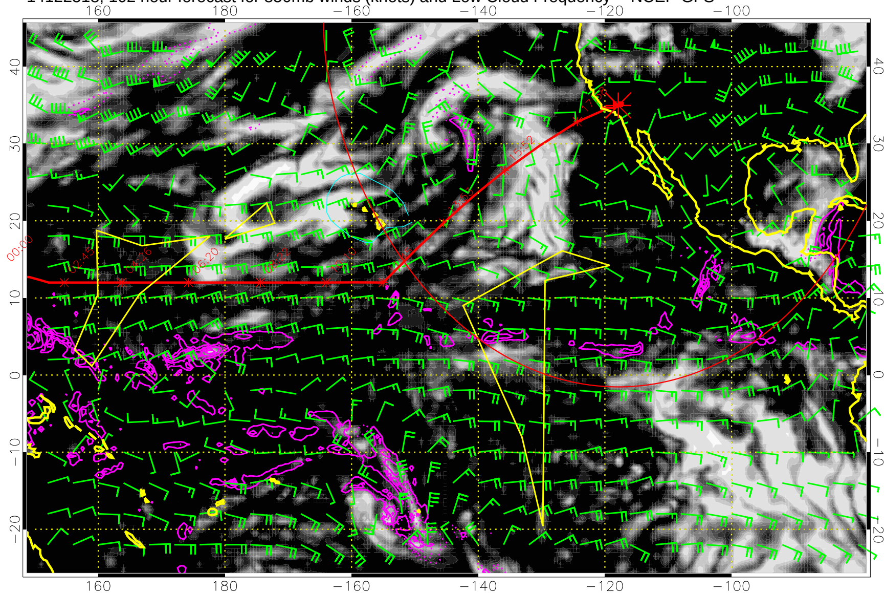
14122518, 102 hour forecast for 850mb winds (knots) and Low Cloud Frequency -- NCEP GFS
