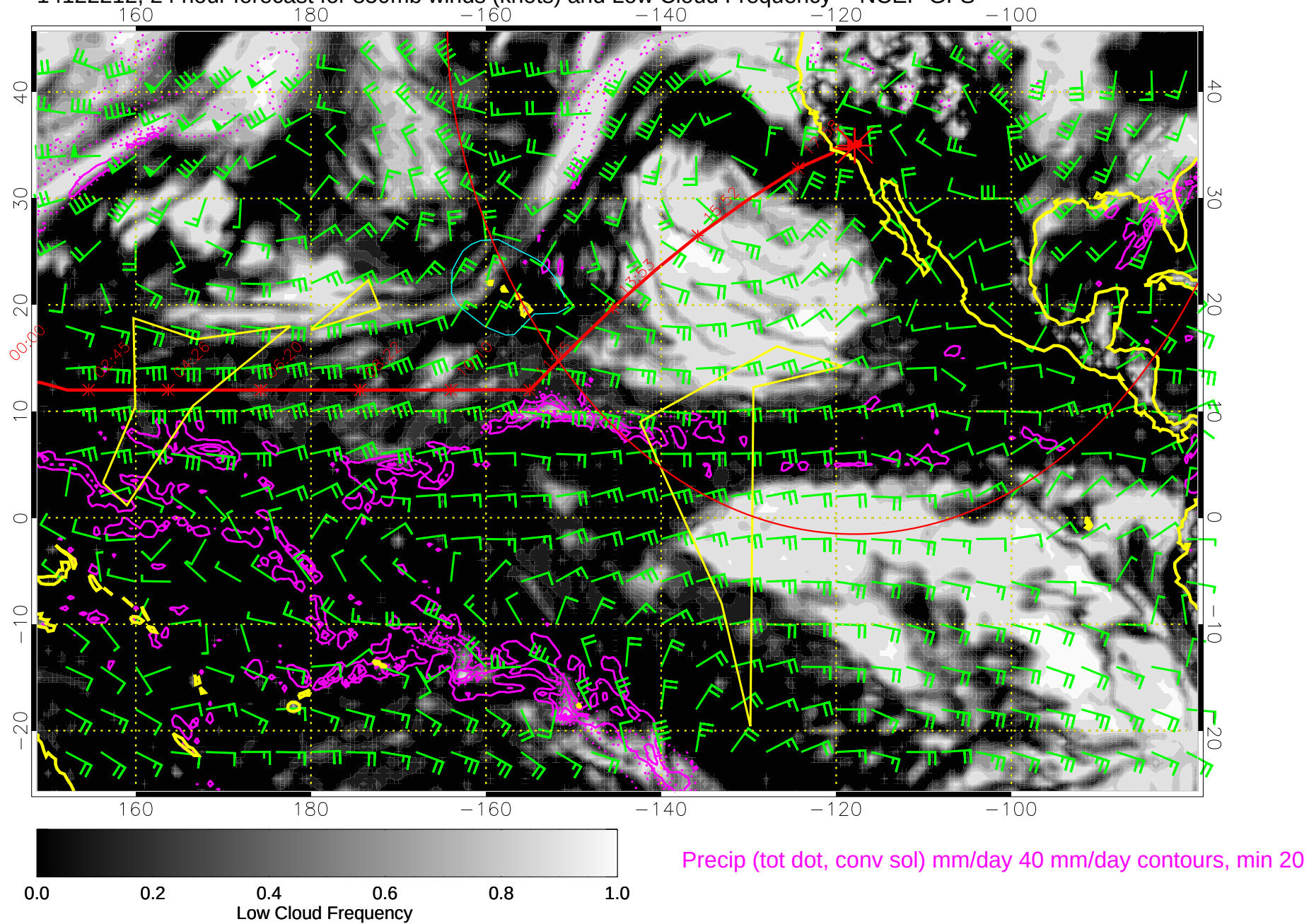
14122212, 24 hour forecast for 850mb winds (knots) and Low Cloud Frequency -- NCEP GFS
