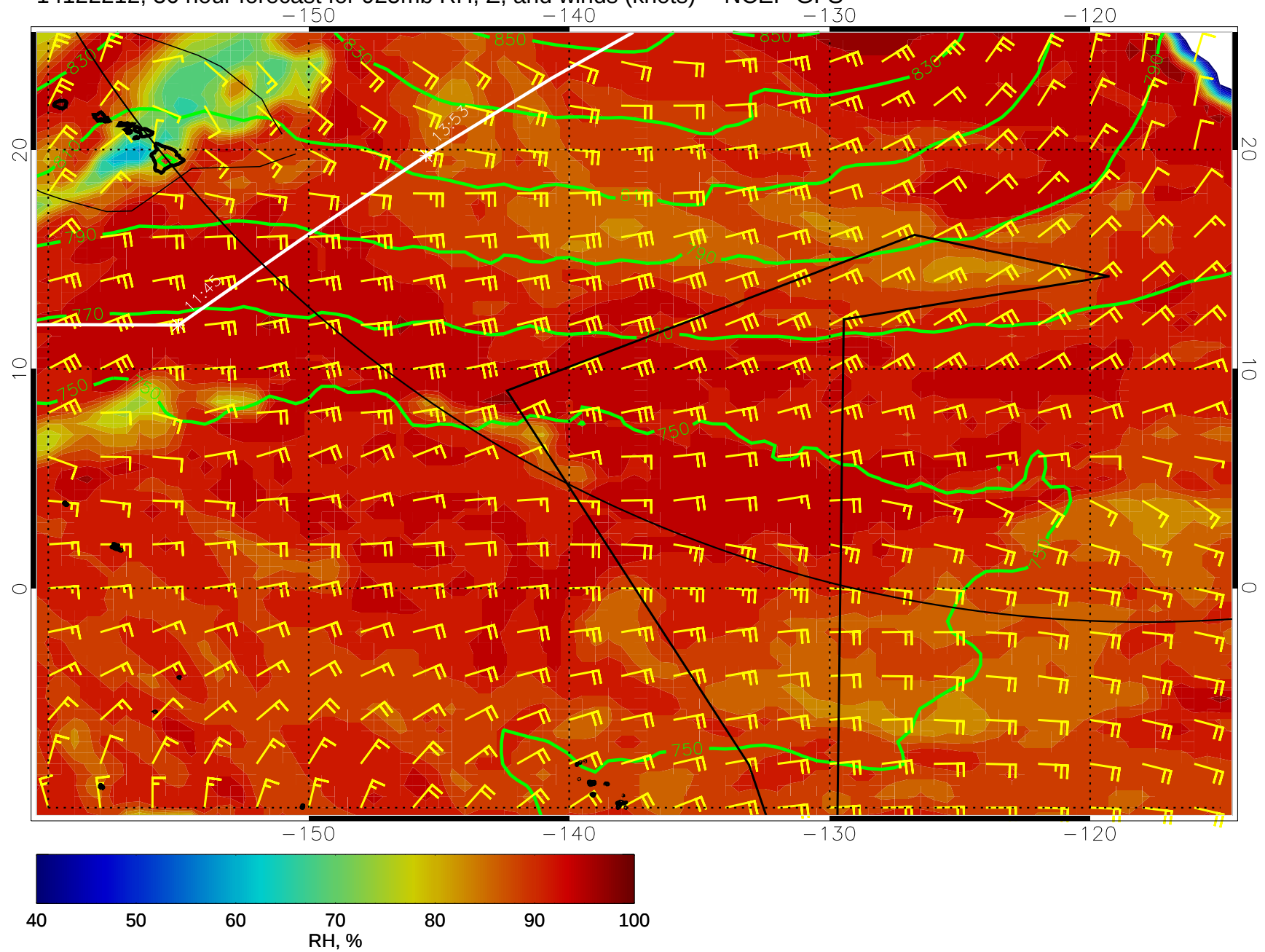
14122212, 36 hour forecast for 925mb RH, Z, and winds (knots) -- NCEP GFS
