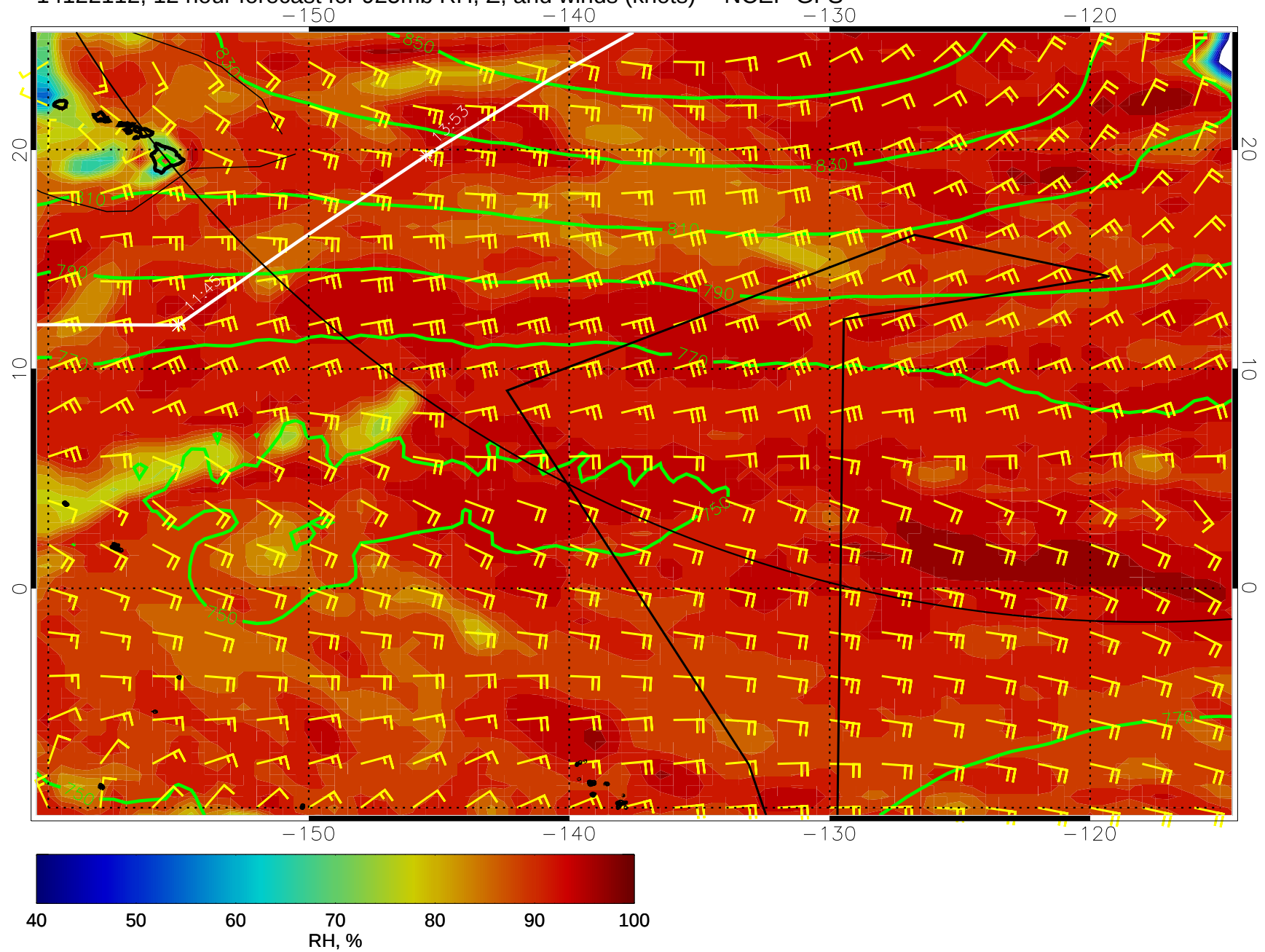
14122112, 12 hour forecast for 925mb RH, Z, and winds (knots) -- NCEP GFS
