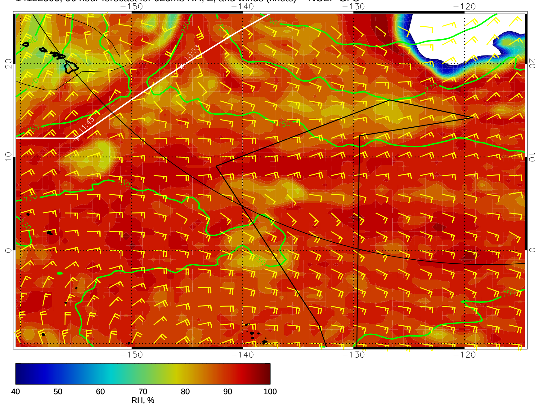
14122500, 96 hour forecast for 925mb RH, Z, and winds (knots) -- NCEP GFS
