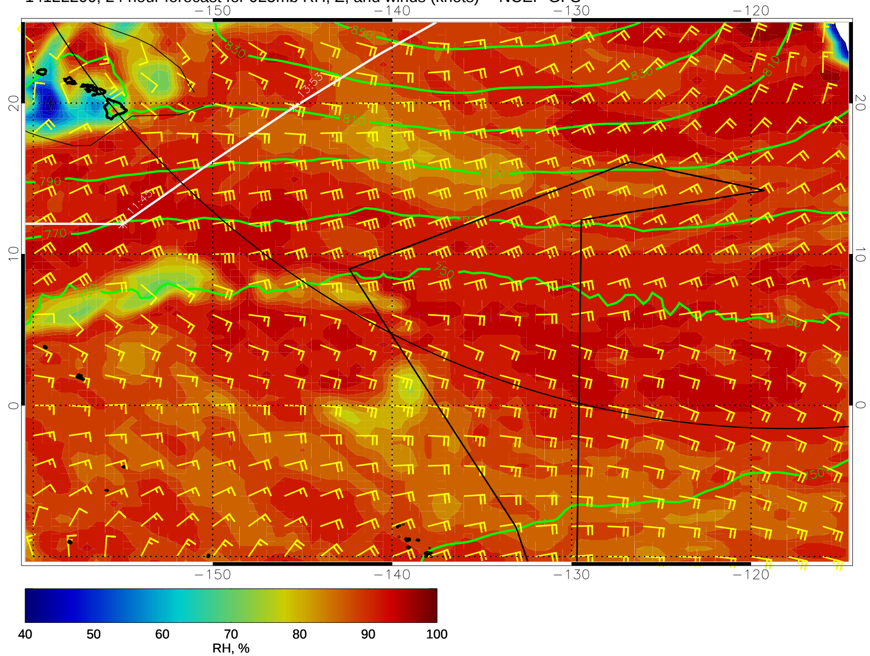
14122200, 24 hour forecast for 925mb RH, Z, and winds (knots) -- NCEP GFS
