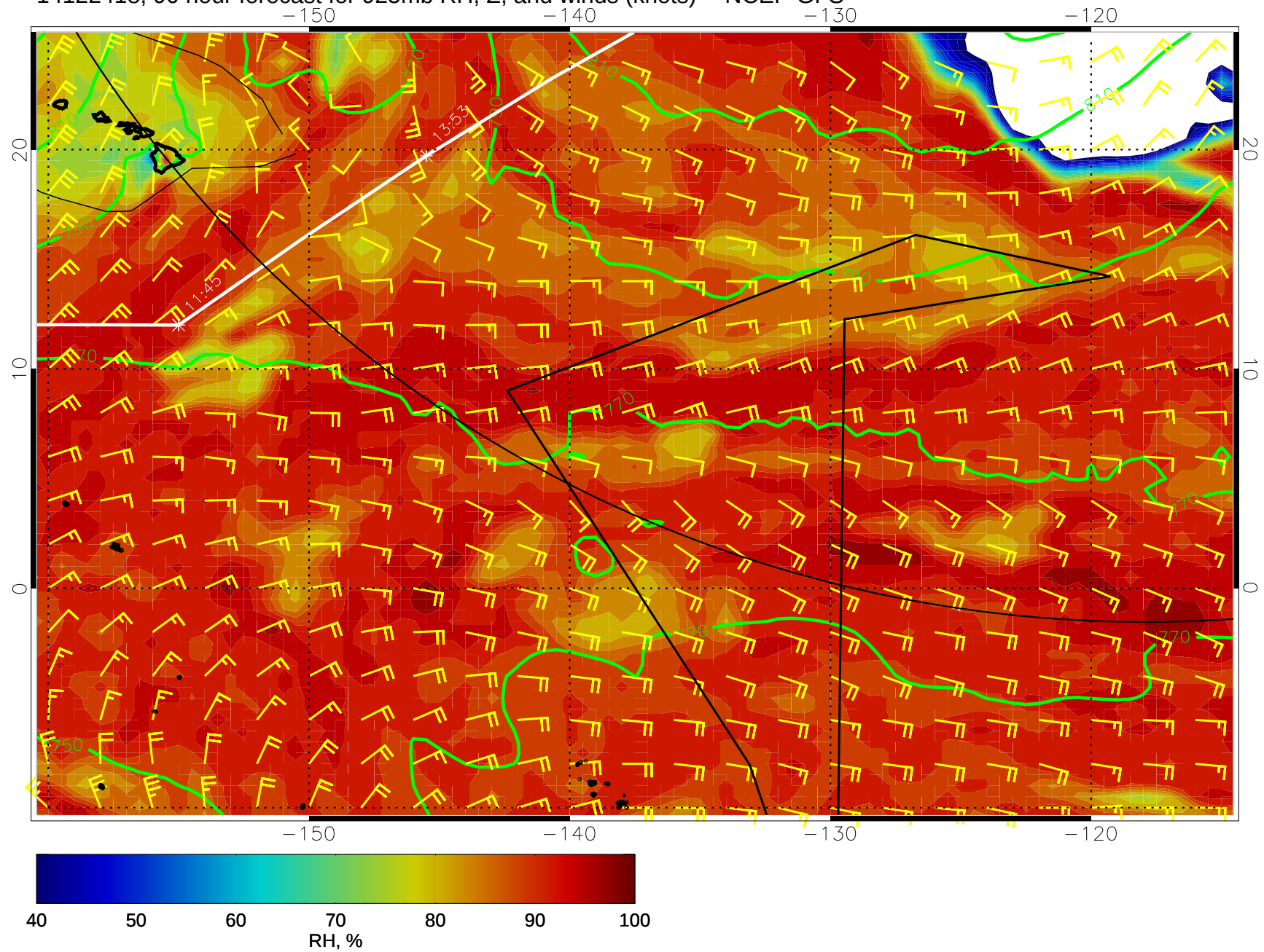
14122418, 90 hour forecast for 925mb RH, Z, and winds (knots) -- NCEP GFS
