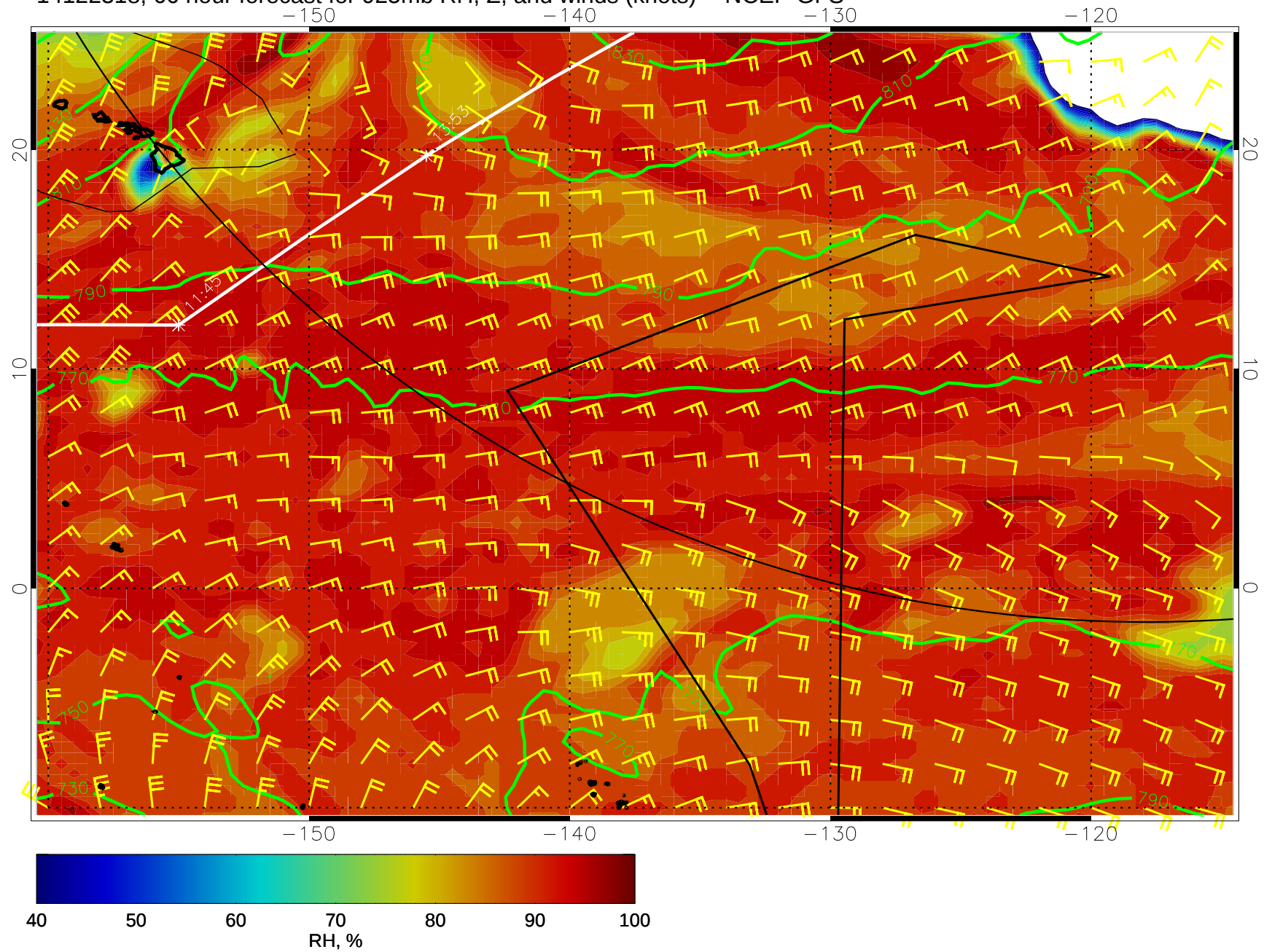
14122318, 66 hour forecast for 925mb RH, Z, and winds (knots) -- NCEP GFS
