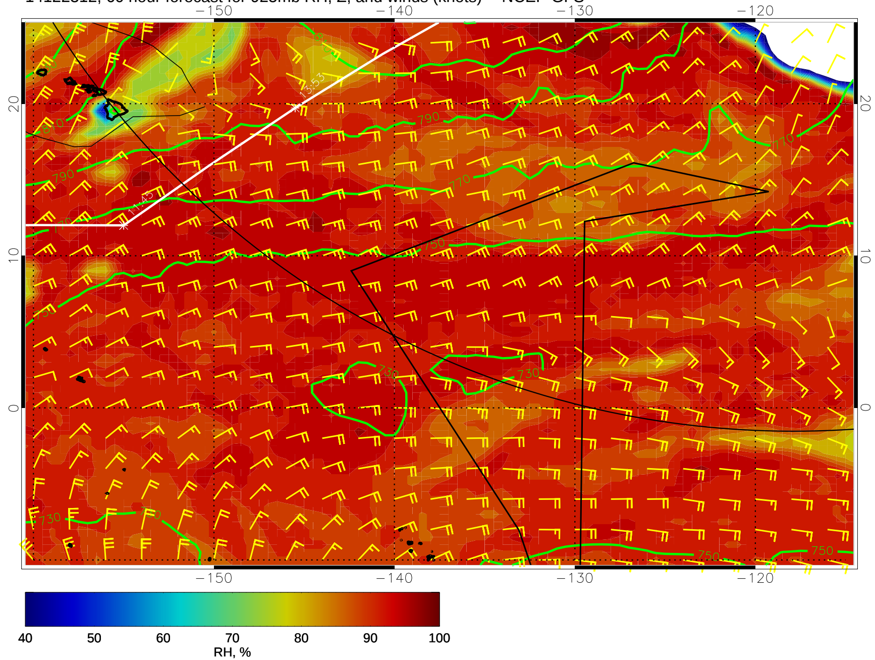
14122312, 60 hour forecast for 925mb RH, Z, and winds (knots) -- NCEP GFS
