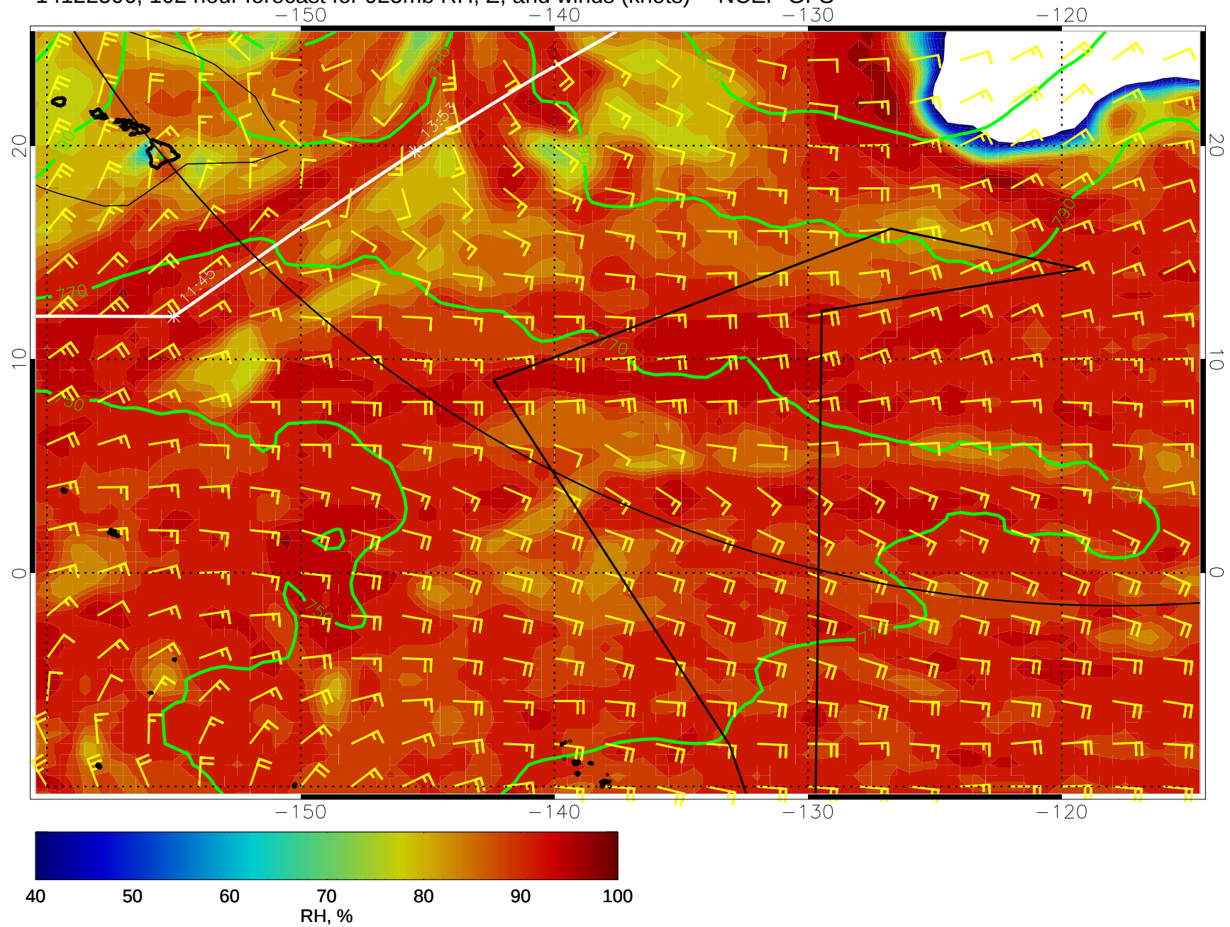
14122506, 102 hour forecast for 925mb RH, Z, and winds (knots) -- NCEP GFS
