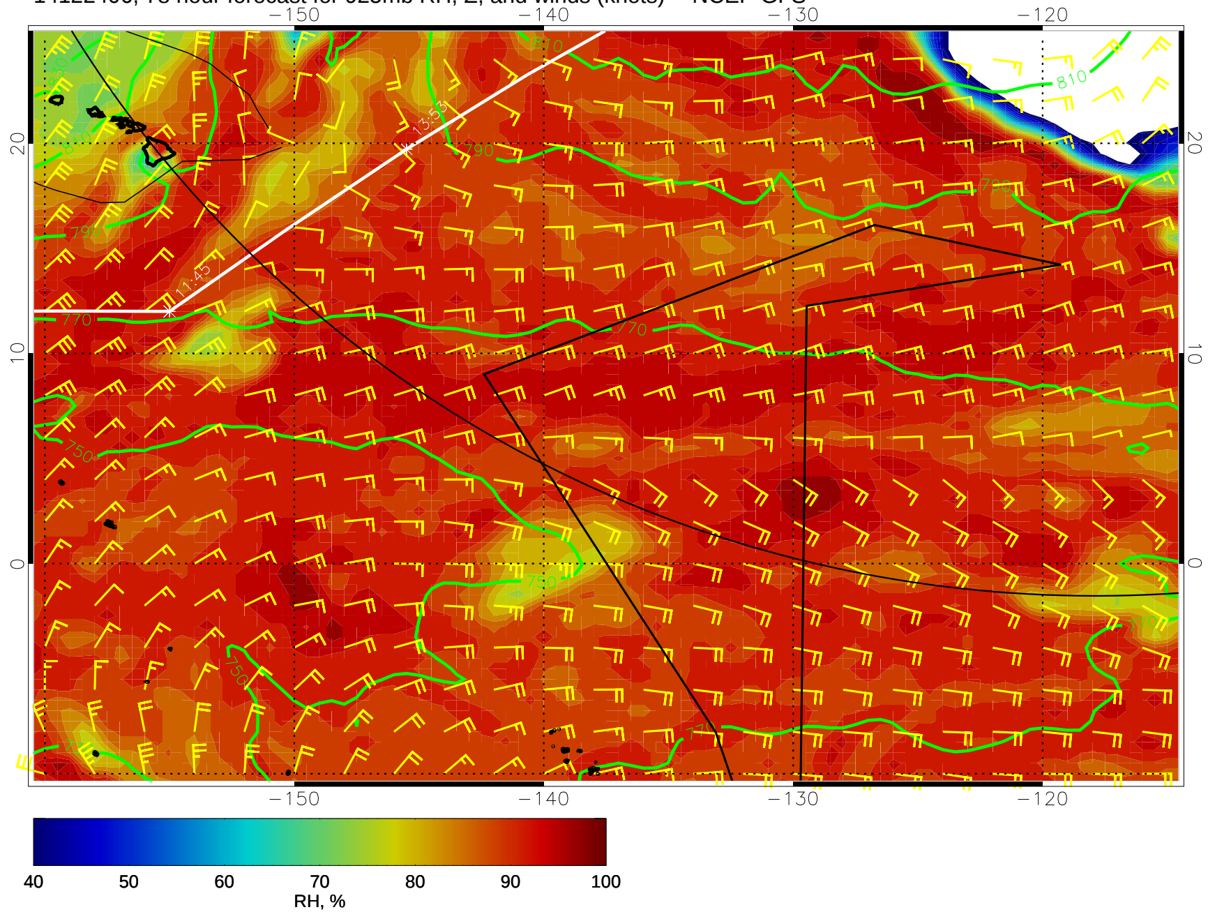
14122406, 78 hour forecast for 925mb RH, Z, and winds (knots) -- NCEP GFS
