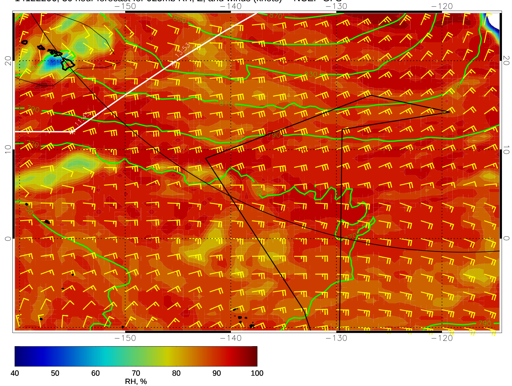
14122206, 30 hour forecast for 925mb RH, Z, and winds (knots) -- NCEP GFS
