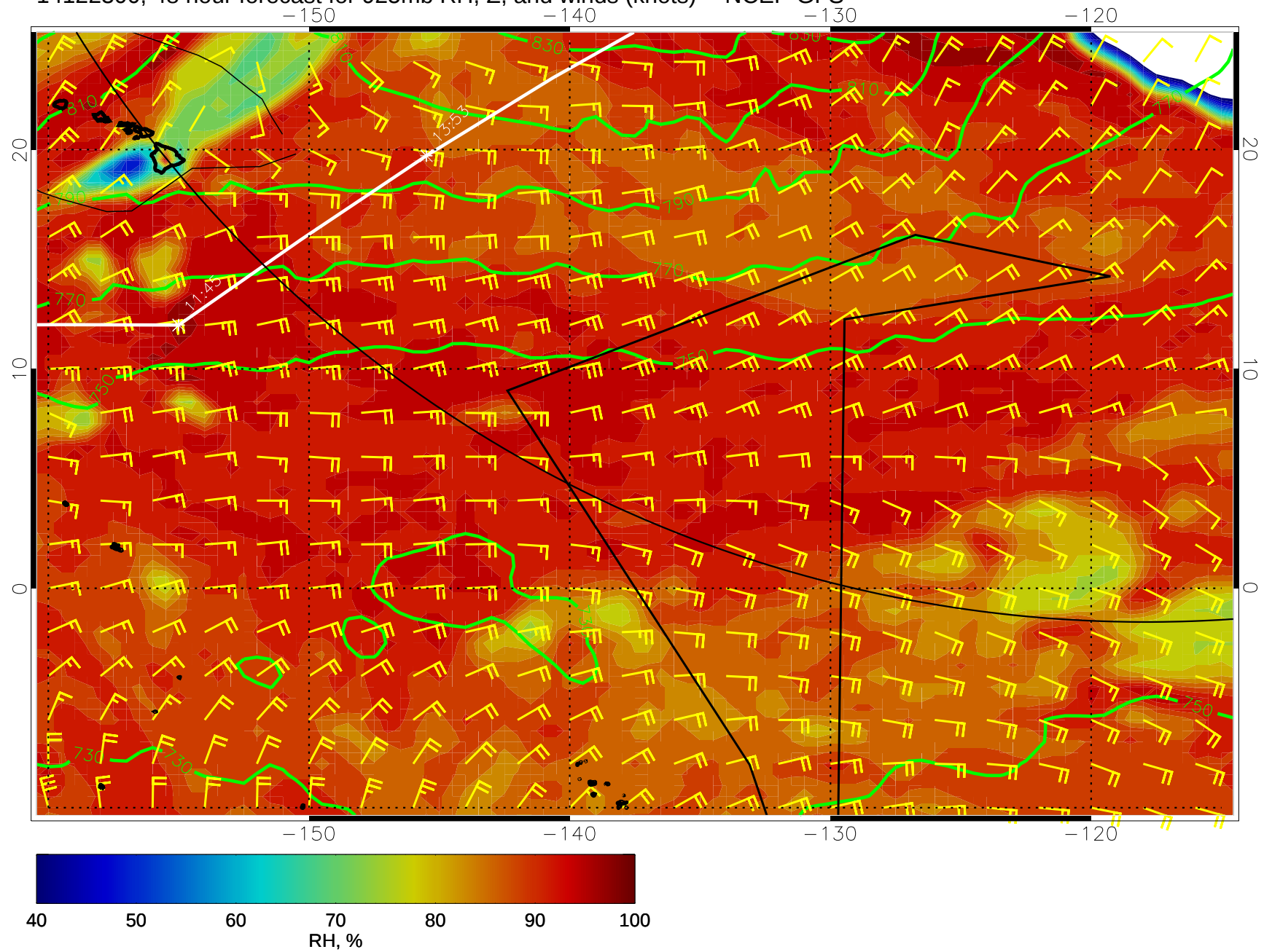
14122300, 48 hour forecast for 925mb RH, Z, and winds (knots) -- NCEP GFS
