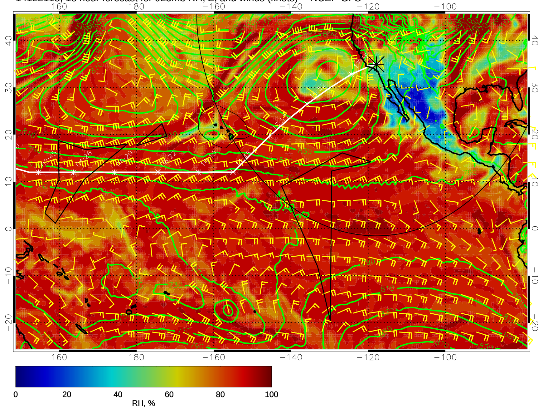
14122118, 18 hour forecast for 925mb RH, Z, and winds (knots) -- NCEP GFS
