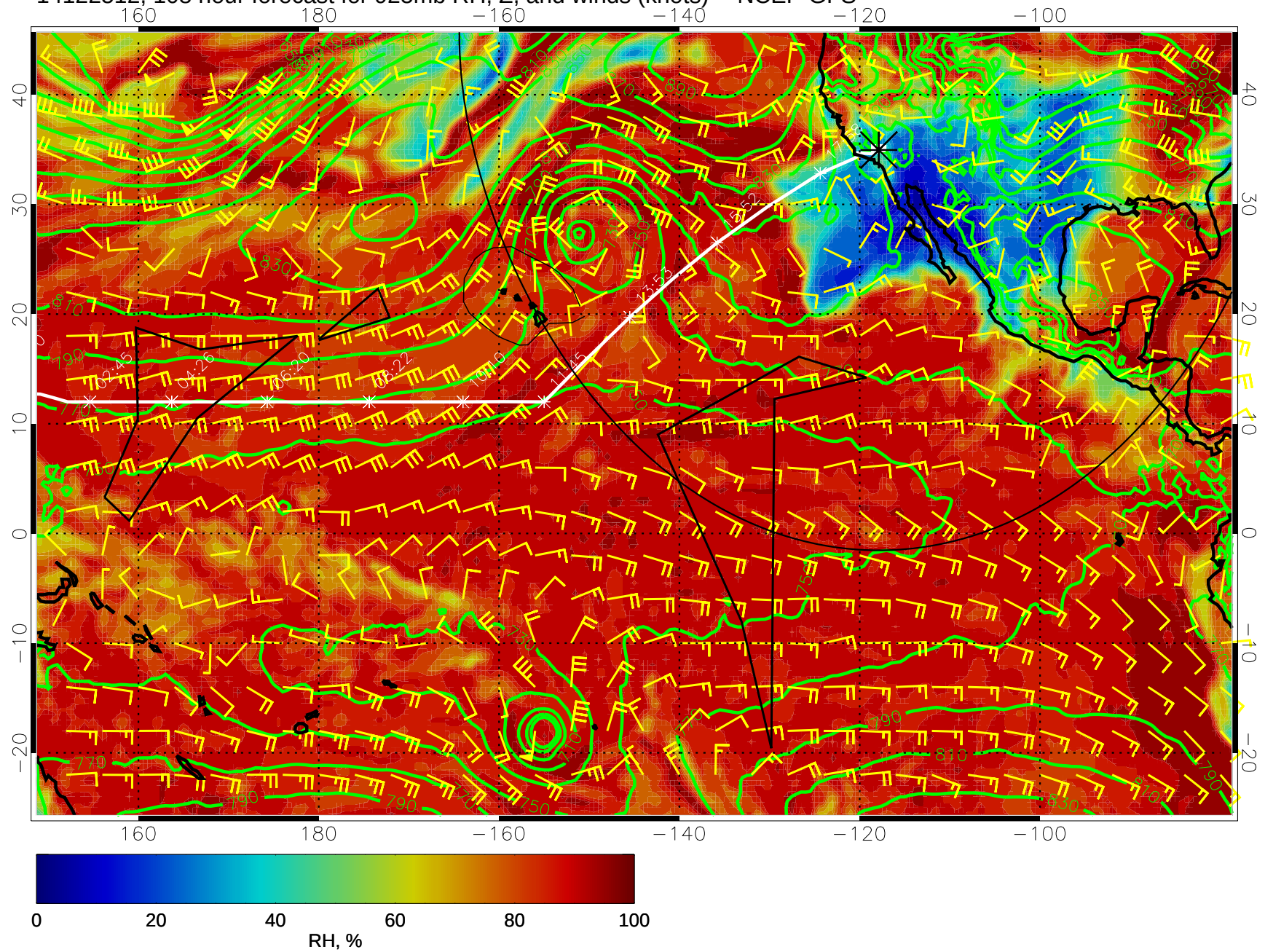
14122512, 108 hour forecast for 925mb RH, Z, and winds (knots) -- NCEP GFS
