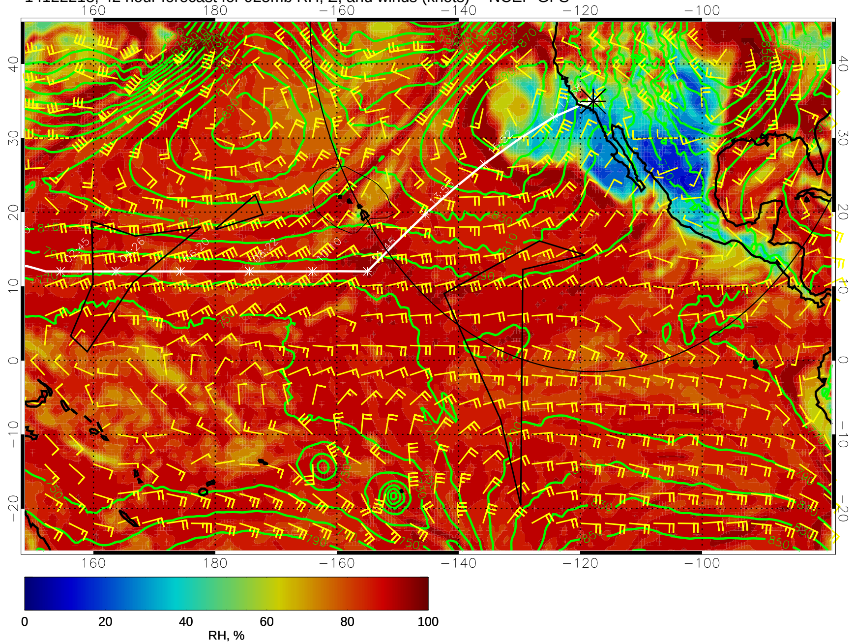
14122218, 42 hour forecast for 925mb RH, Z, and winds (knots) -- NCEP GFS
