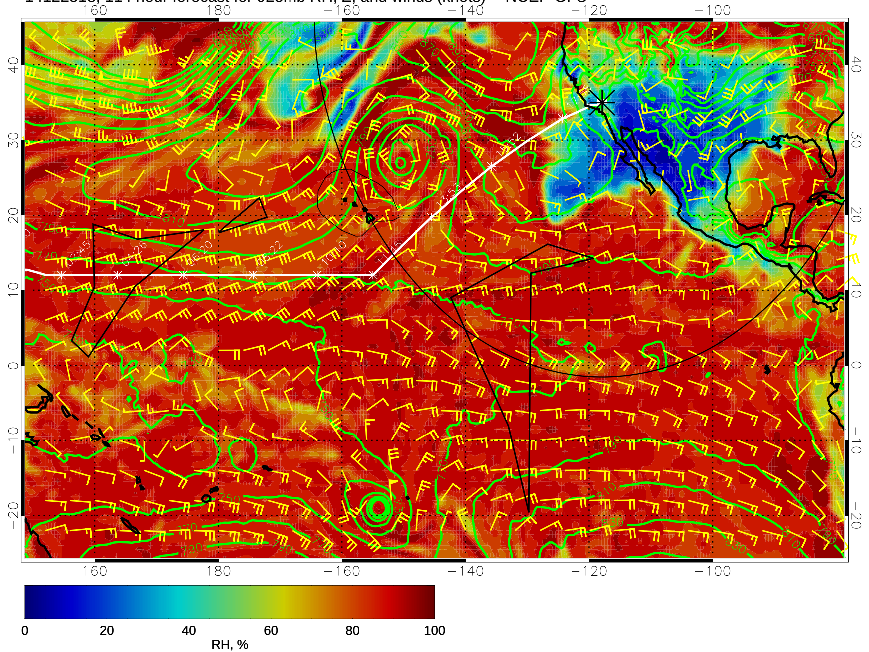
14122518, 114 hour forecast for 925mb RH, Z, and winds (knots) -- NCEP GFS
