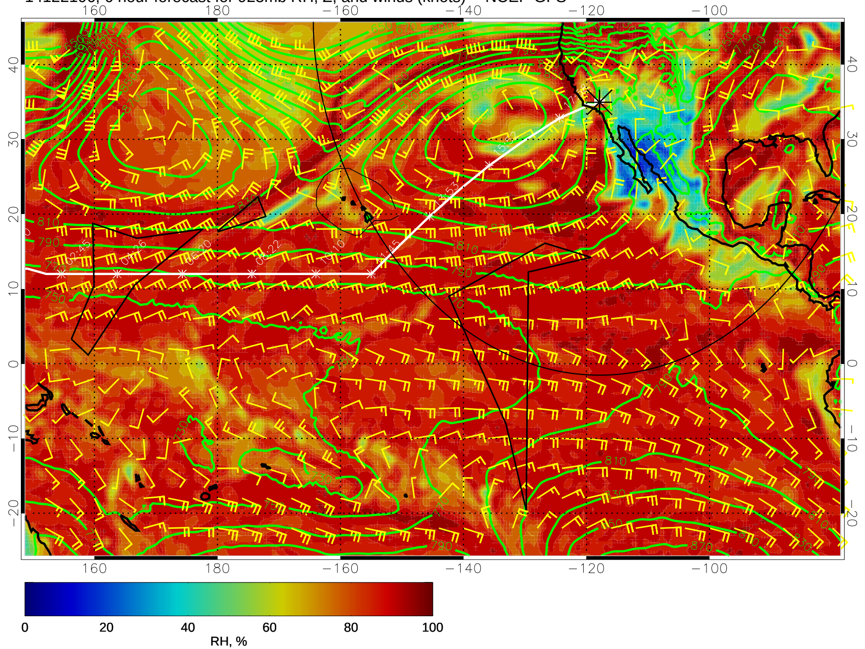
14122106, 6 hour forecast for 925mb RH, Z, and winds (knots) -- NCEP GFS
