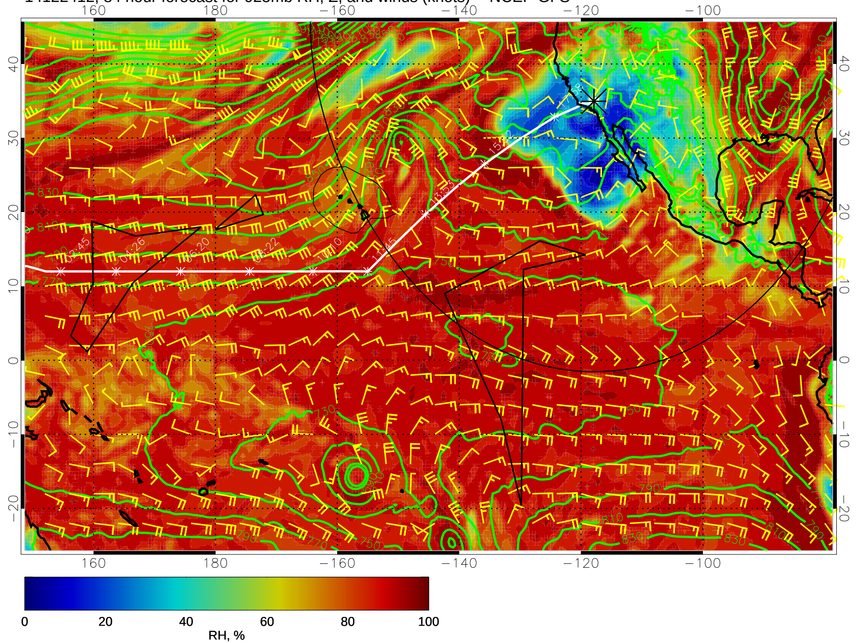
14122412, 84 hour forecast for 925mb RH, Z, and winds (knots) -- NCEP GFS
