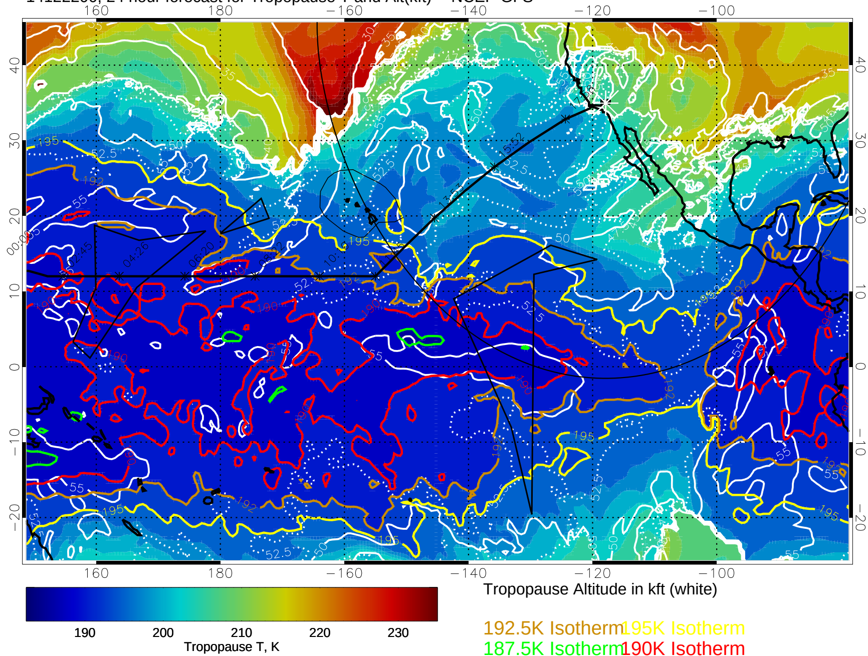
14122200, 24 hour forecast for Tropopause T and Alt(kft) -- NCEP GFS
