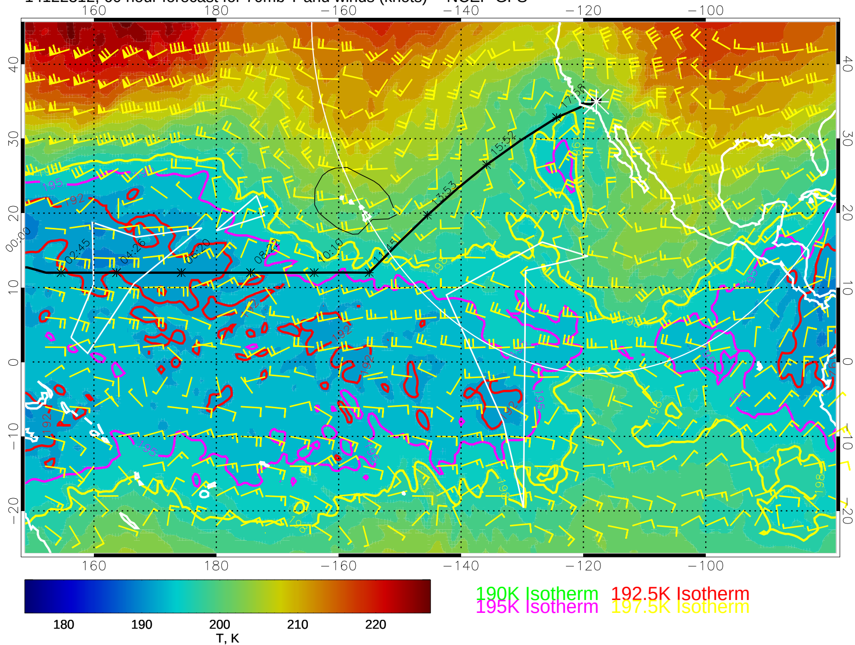
14122312, 60 hour forecast for 70mb T and winds (knots) -- NCEP GFS
