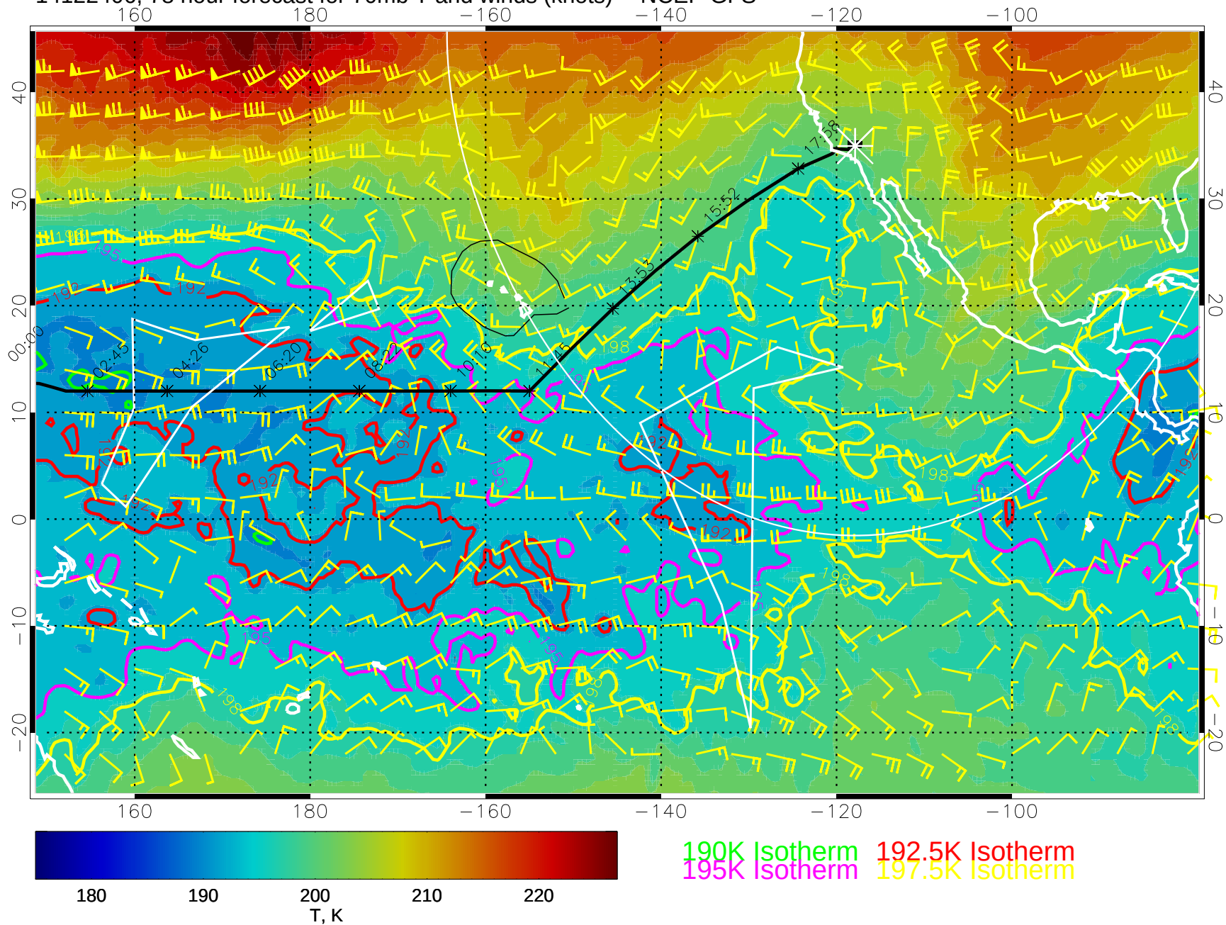
14122406, 78 hour forecast for 70mb T and winds (knots) -- NCEP GFS
