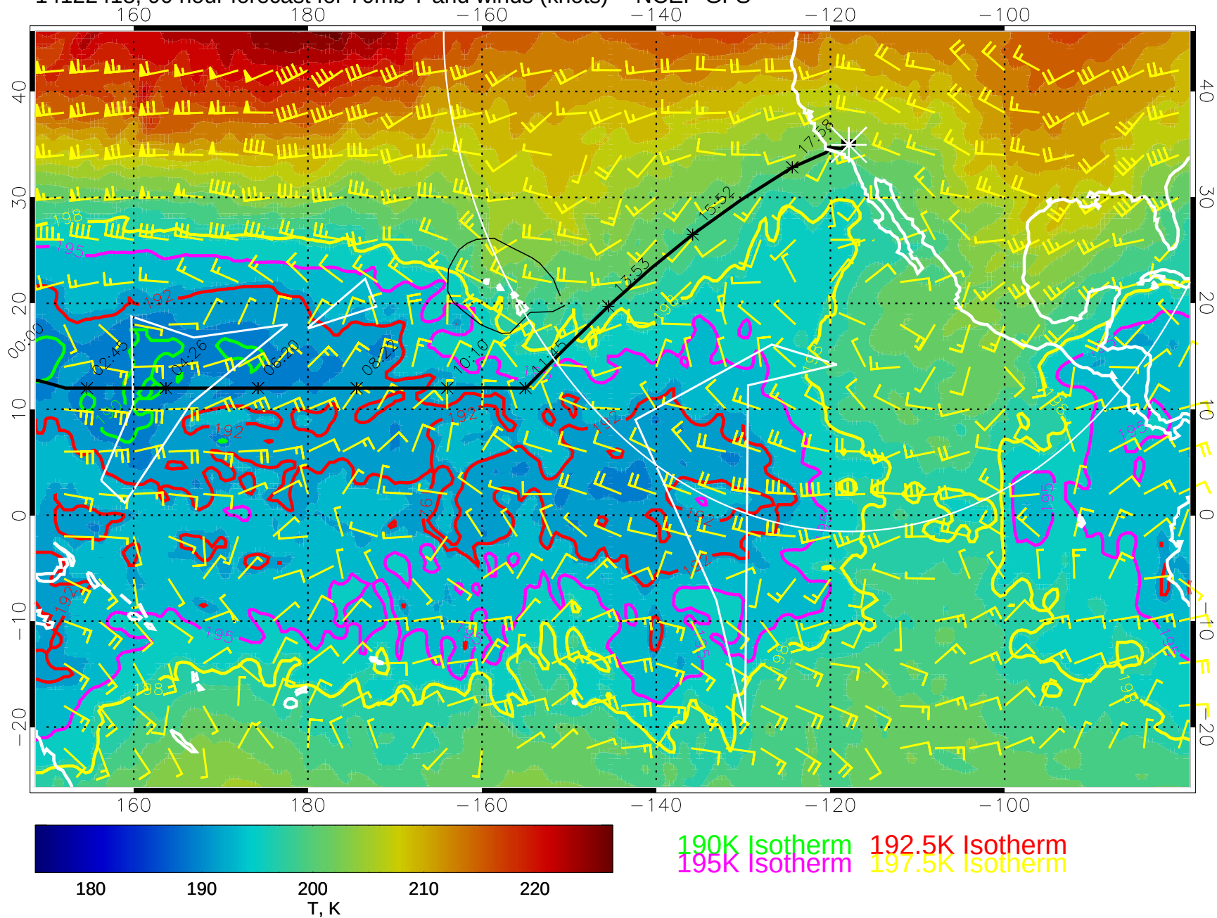
14122418, 90 hour forecast for 70mb T and winds (knots) -- NCEP GFS
