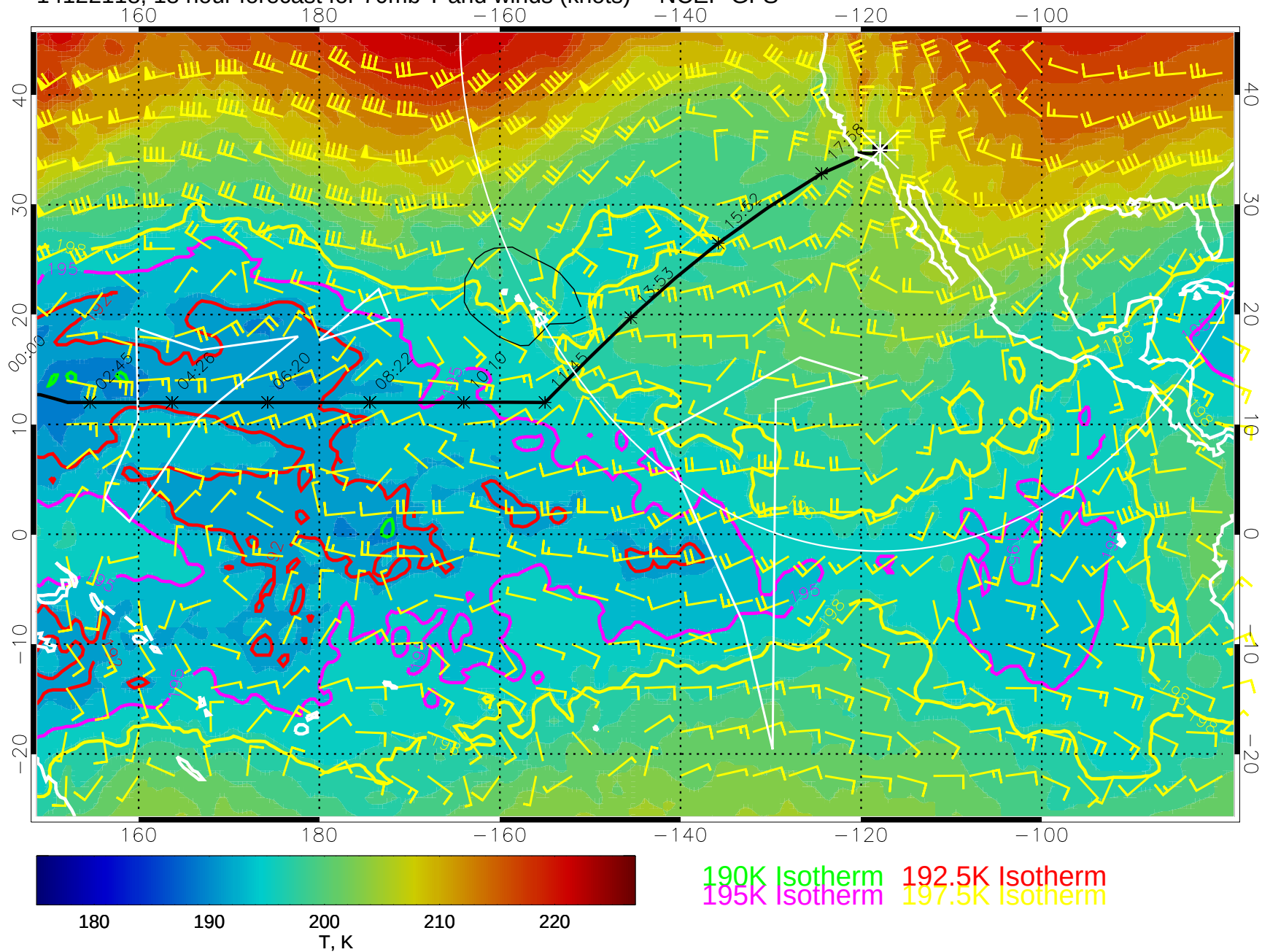
14122118, 18 hour forecast for 70mb T and winds (knots) -- NCEP GFS
