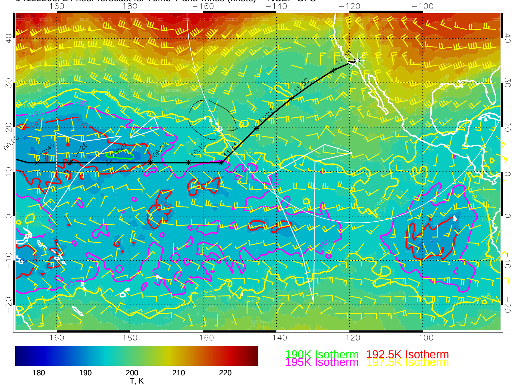
14122200, 24 hour forecast for 70mb T and winds (knots) -- NCEP GFS
