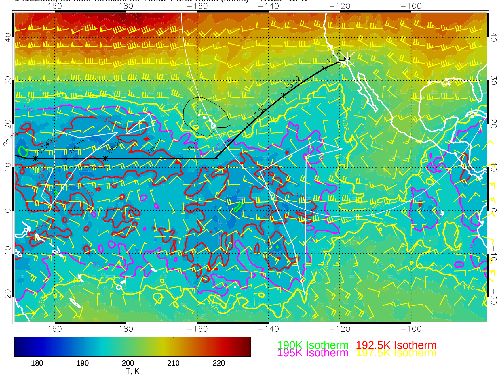
14122500, 96 hour forecast for 70mb T and winds (knots) -- NCEP GFS
