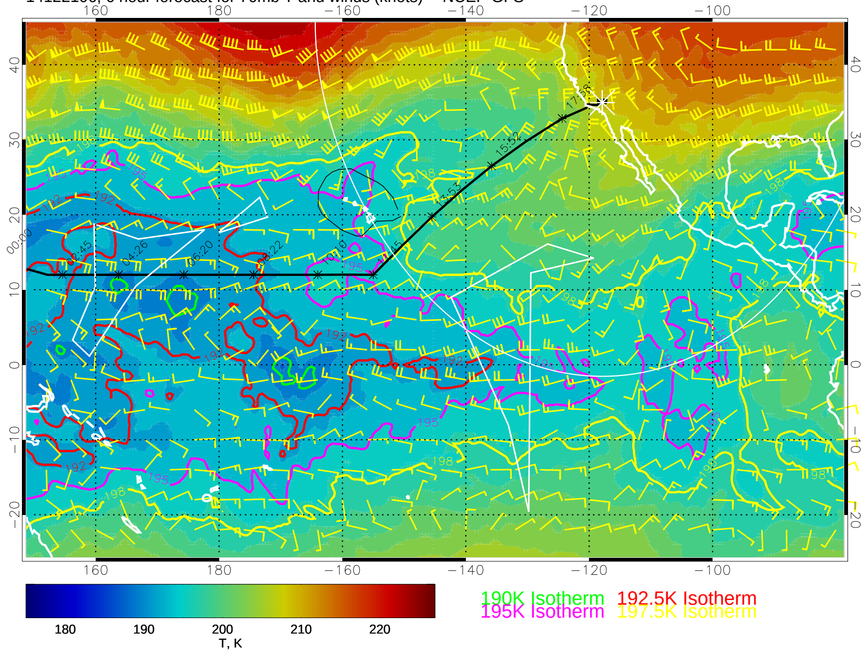
14122106, 6 hour forecast for 70mb T and winds (knots) -- NCEP GFS
