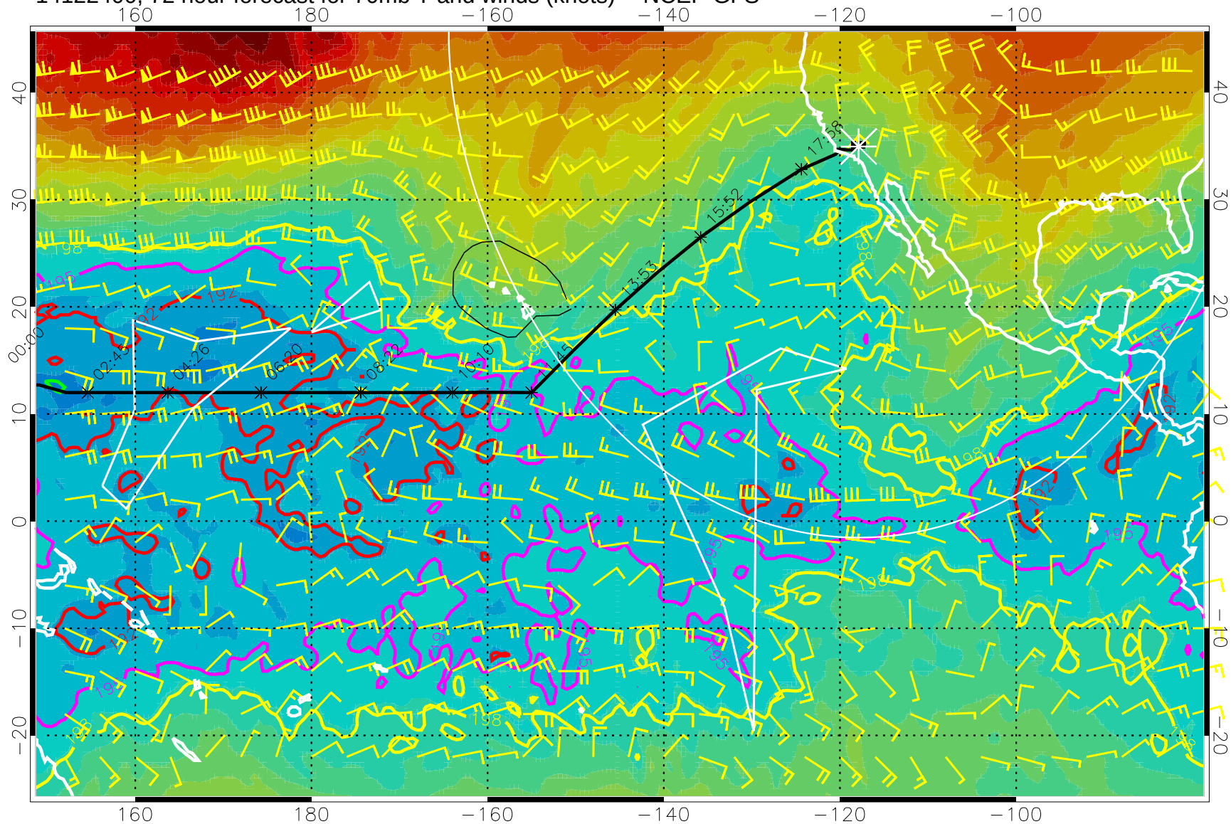
14122400, 72 hour forecast for 70mb T and winds (knots) -- NCEP GFS
