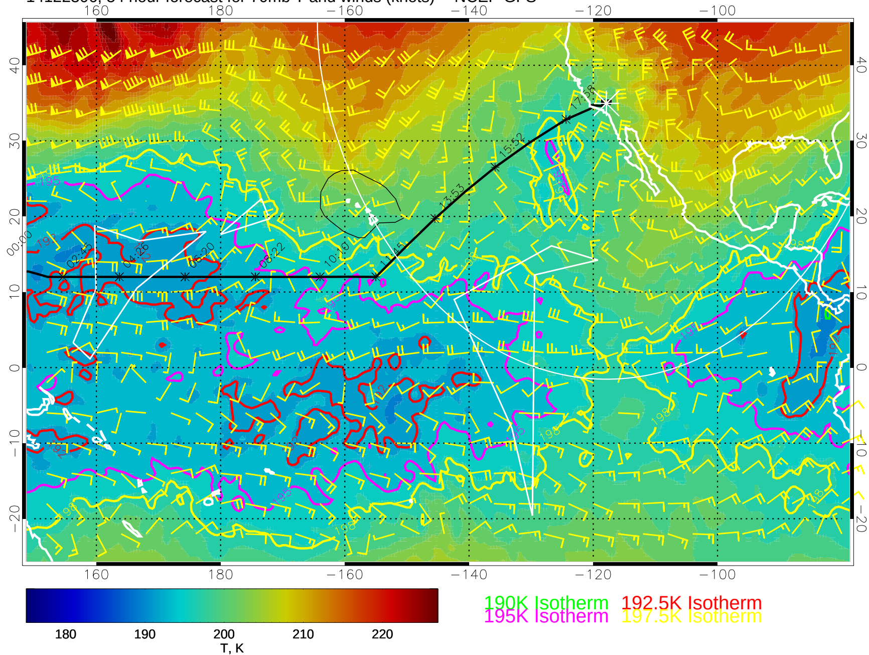
14122306, 54 hour forecast for 70mb T and winds (knots) -- NCEP GFS
