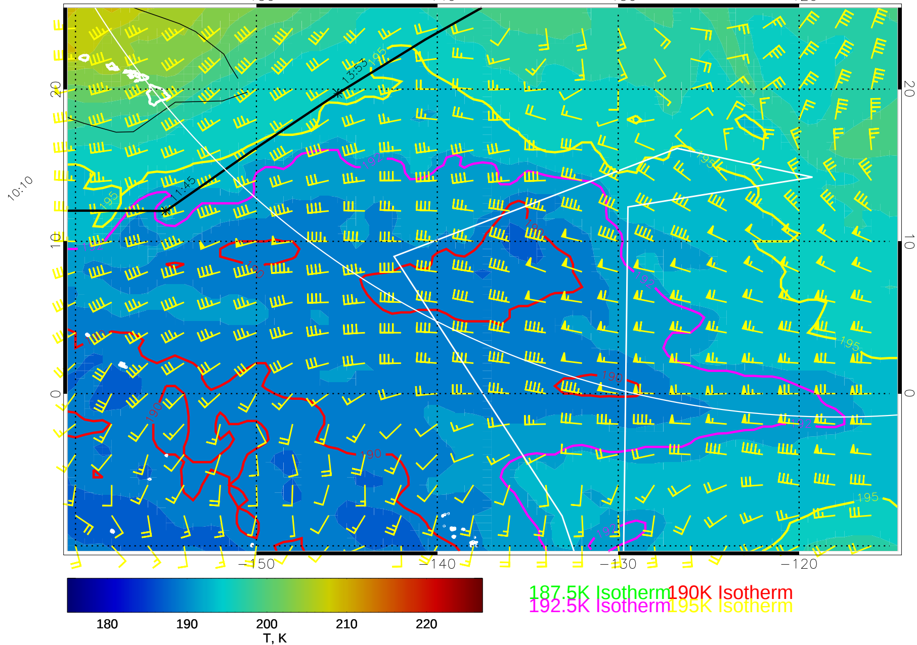
14122306, 54 hour forecast for 100mb T and winds (knots) -- NCEP GFS
