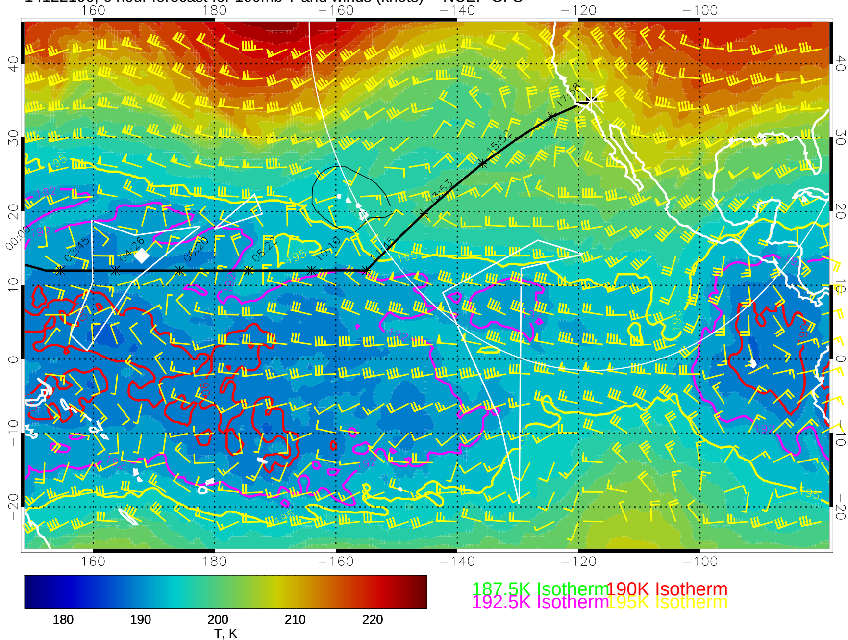
14122106, 6 hour forecast for 100mb T and winds (knots) -- NCEP GFS
