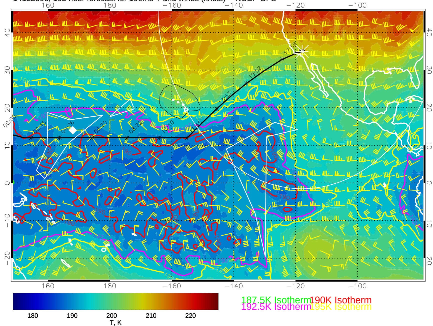
14122506, 102 hour forecast for 100mb T and winds (knots) -- NCEP GFS
