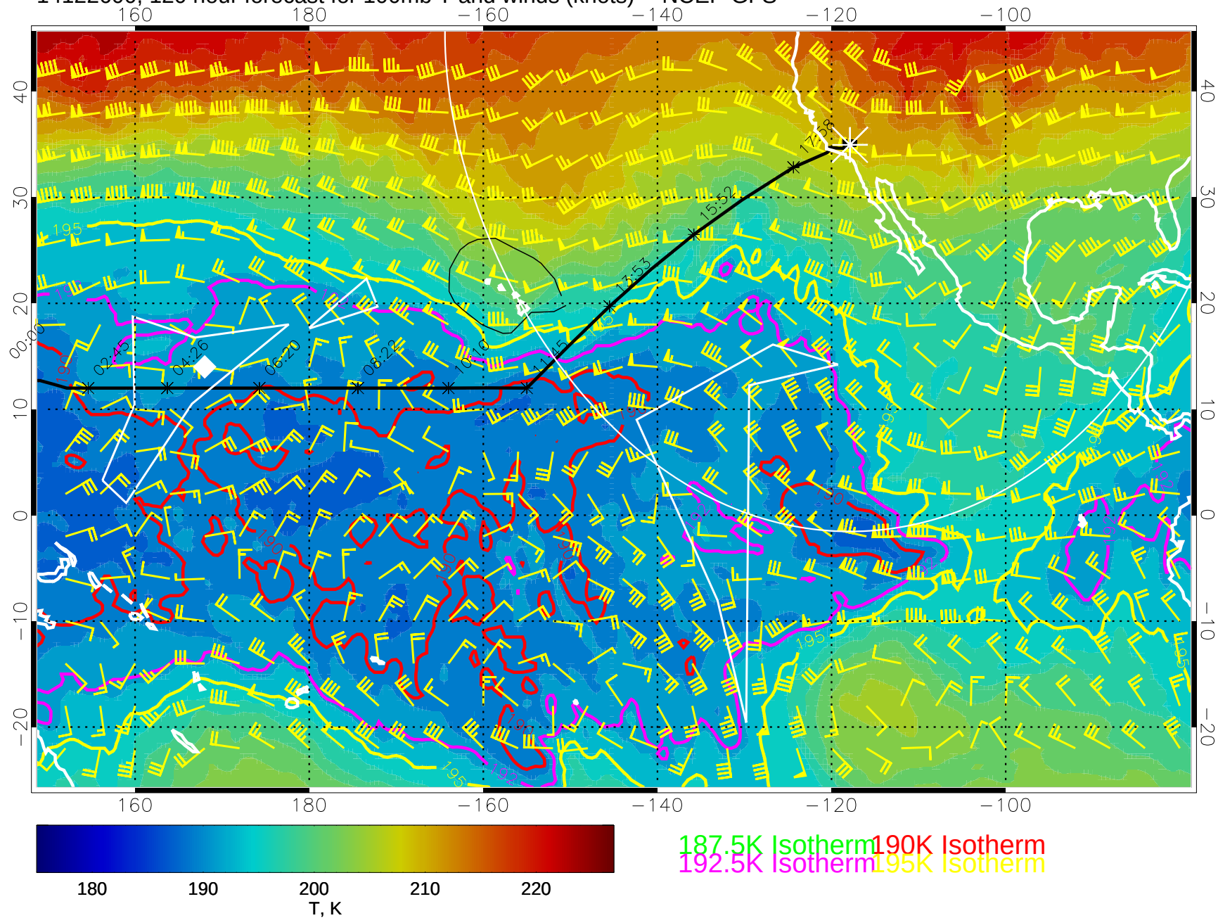
14122600, 120 hour forecast for 100mb T and winds (knots) -- NCEP GFS
