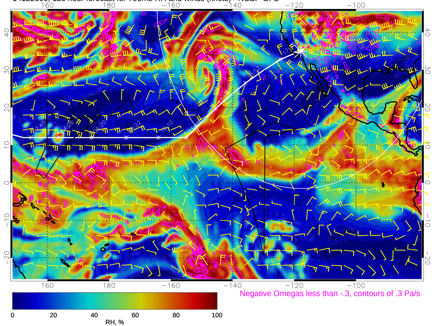
14122600, 120 hour forecast for 700mb RH and winds (knots) - NCEP GFS
