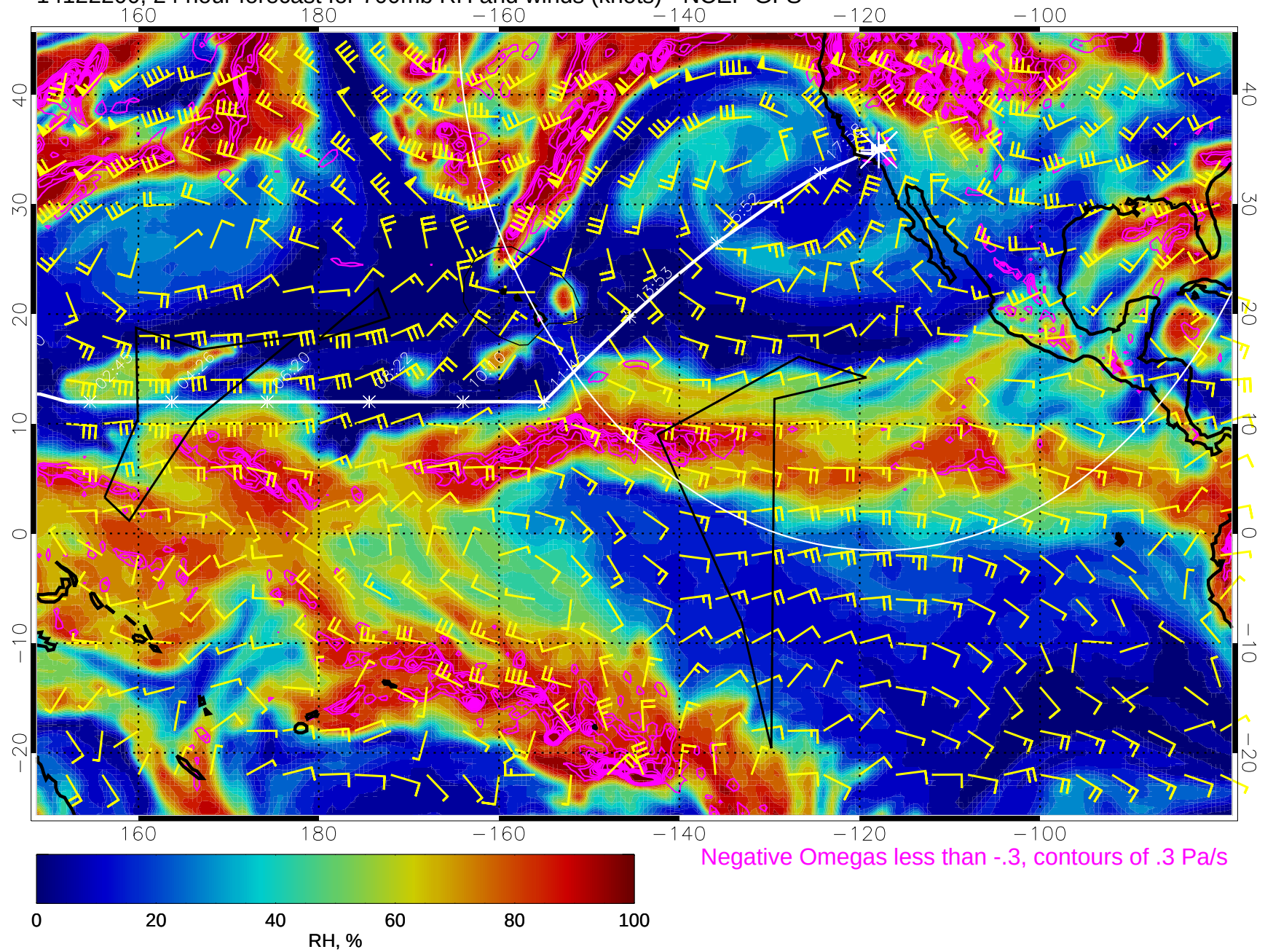
14122200, 24 hour forecast for 700mb RH and winds (knots) - NCEP GFS
