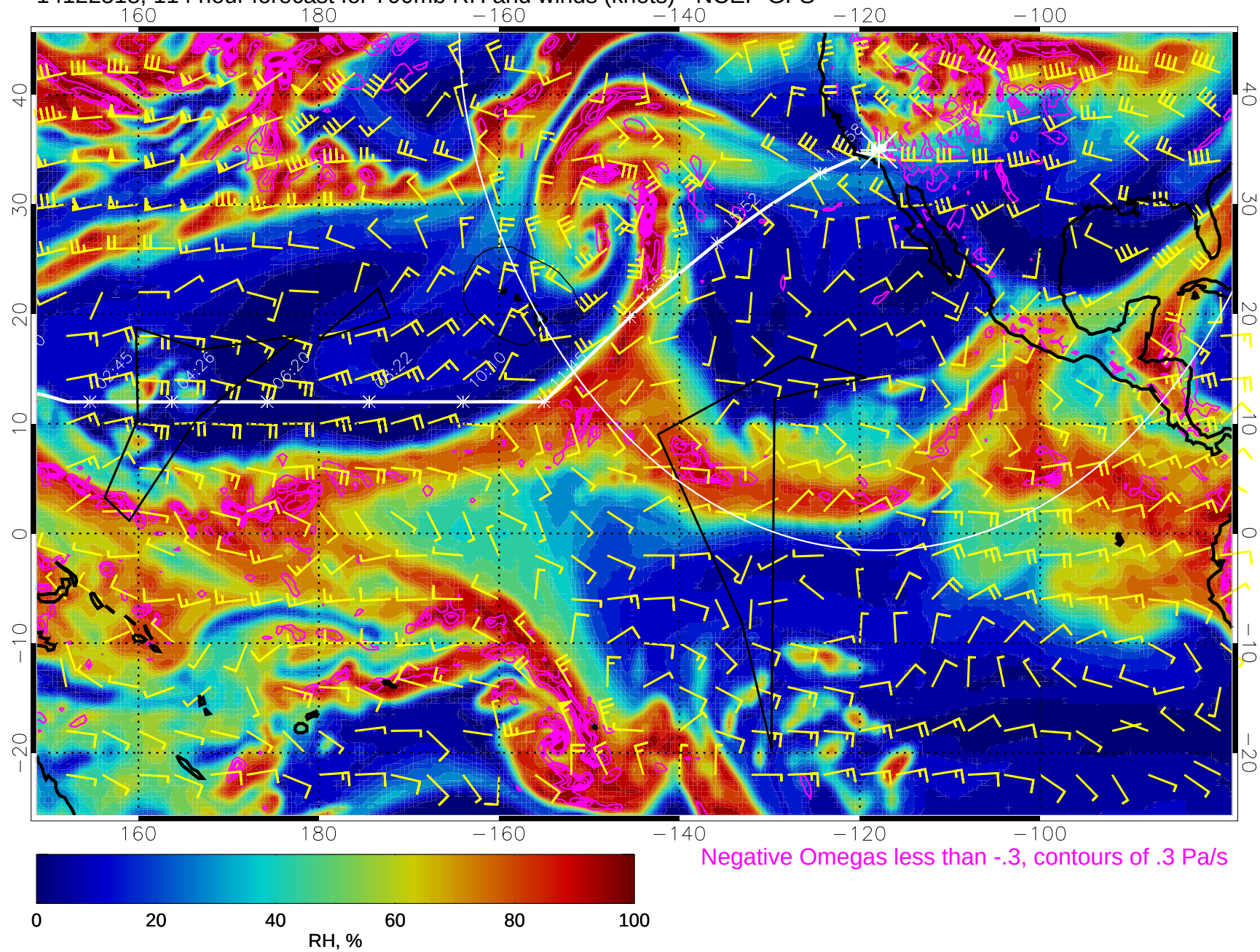
14122518, 114 hour forecast for 700mb RH and winds (knots) - NCEP GFS
