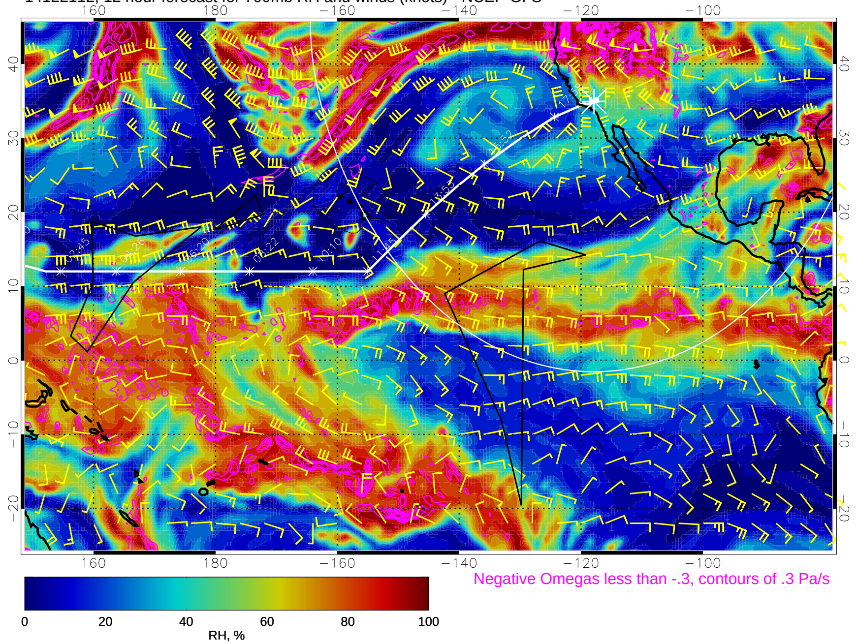
14122112, 12 hour forecast for 700mb RH and winds (knots) - NCEP GFS
