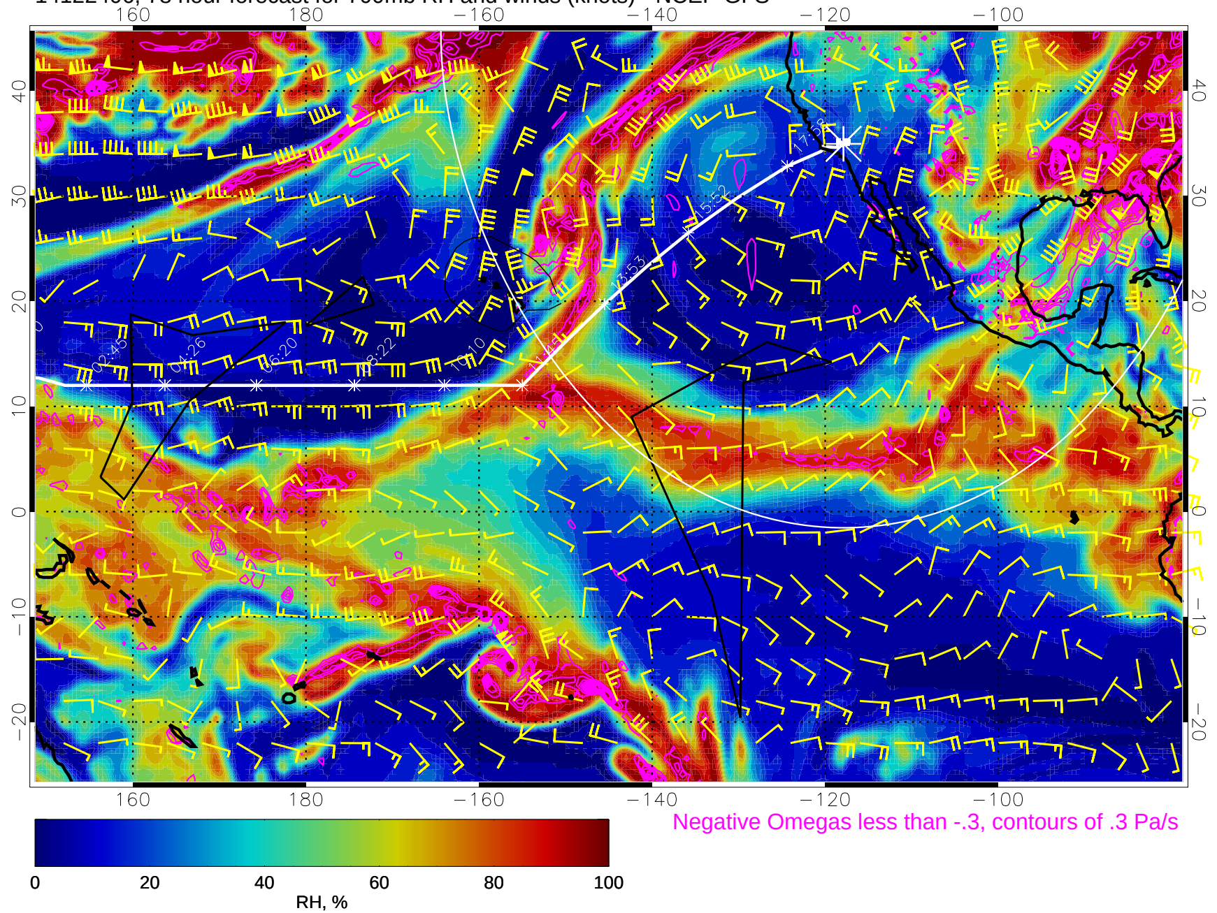
14122406, 78 hour forecast for 700mb RH and winds (knots) - NCEP GFS
