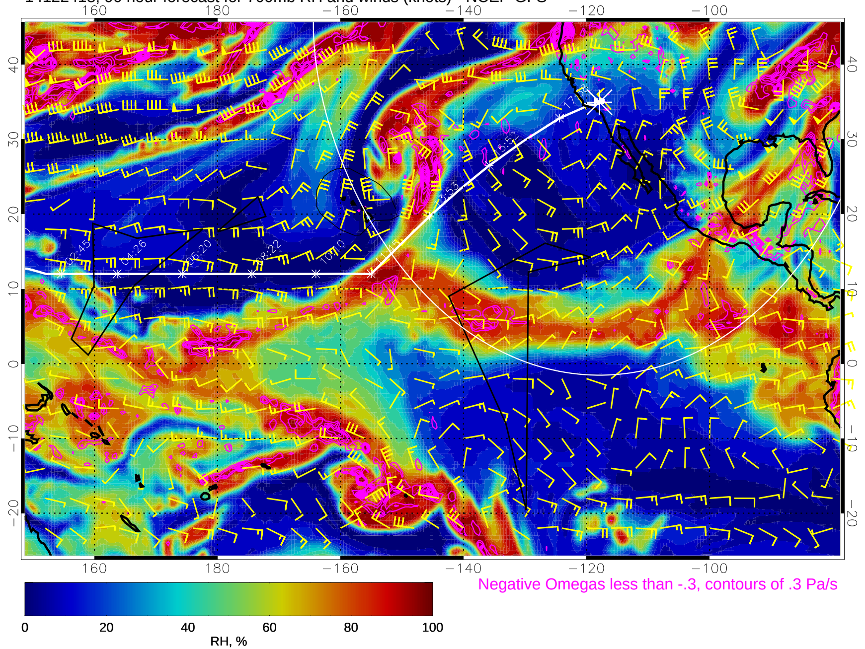
14122418, 90 hour forecast for 700mb RH and winds (knots) - NCEP GFS
