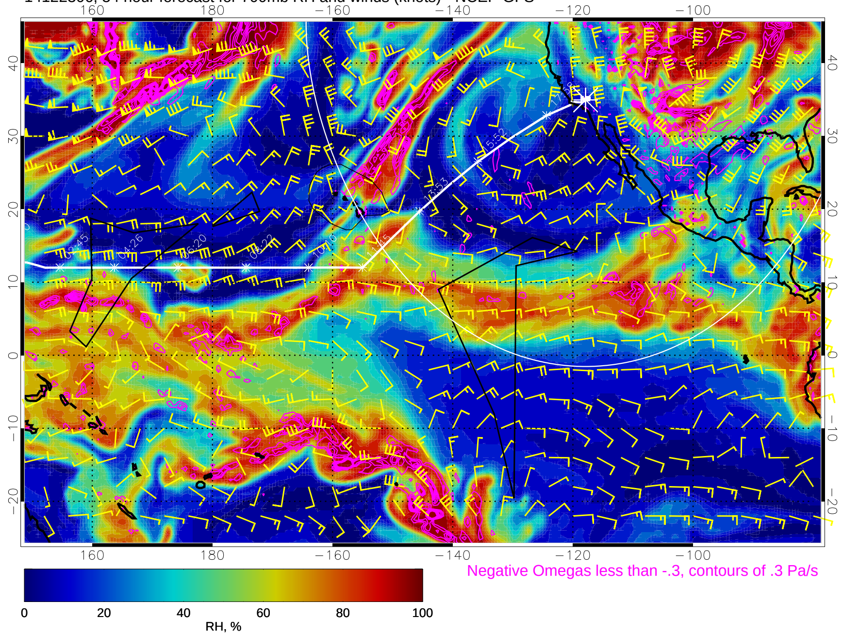
14122306, 54 hour forecast for 700mb RH and winds (knots) - NCEP GFS
