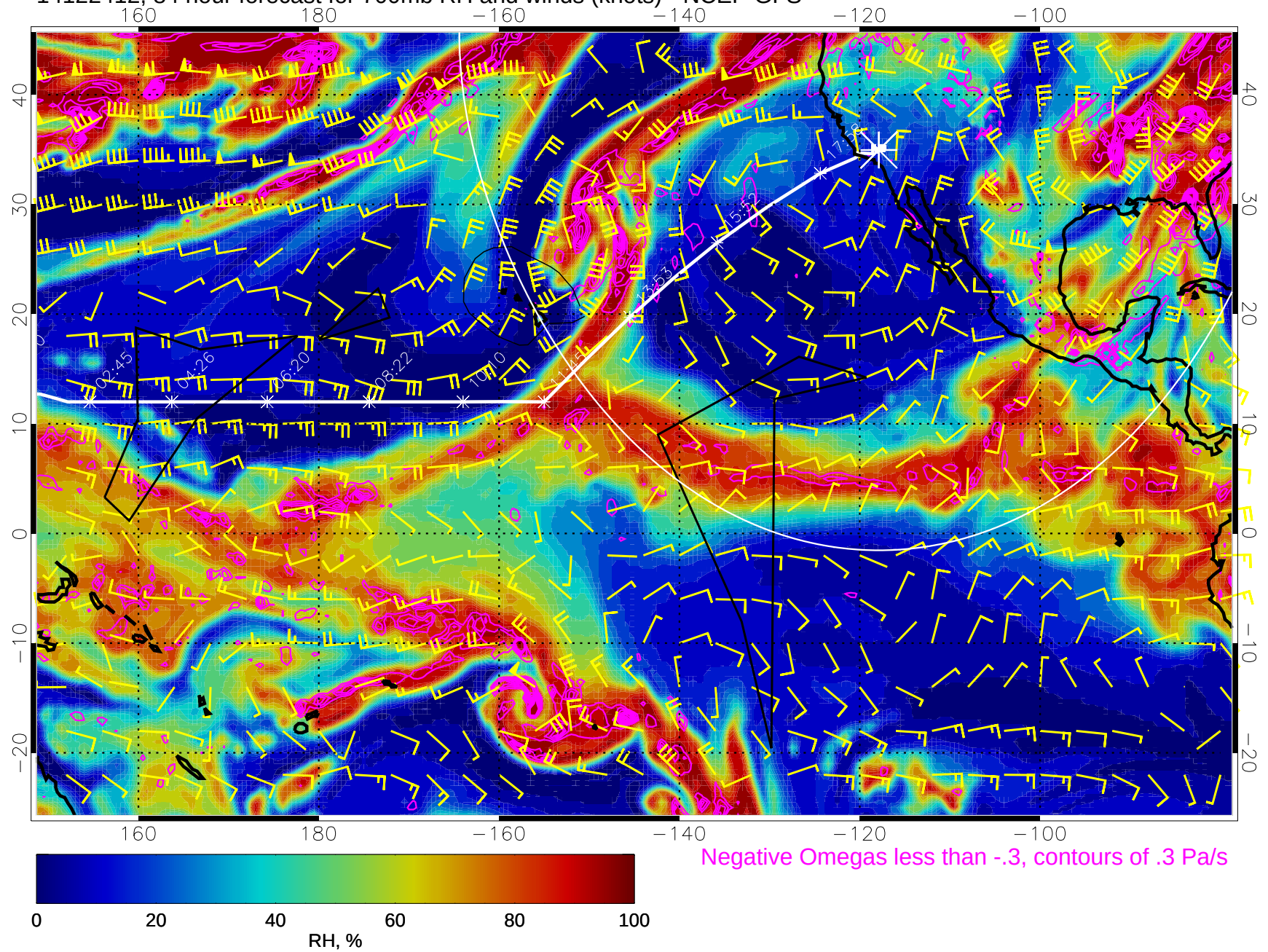
14122412, 84 hour forecast for 700mb RH and winds (knots) - NCEP GFS
