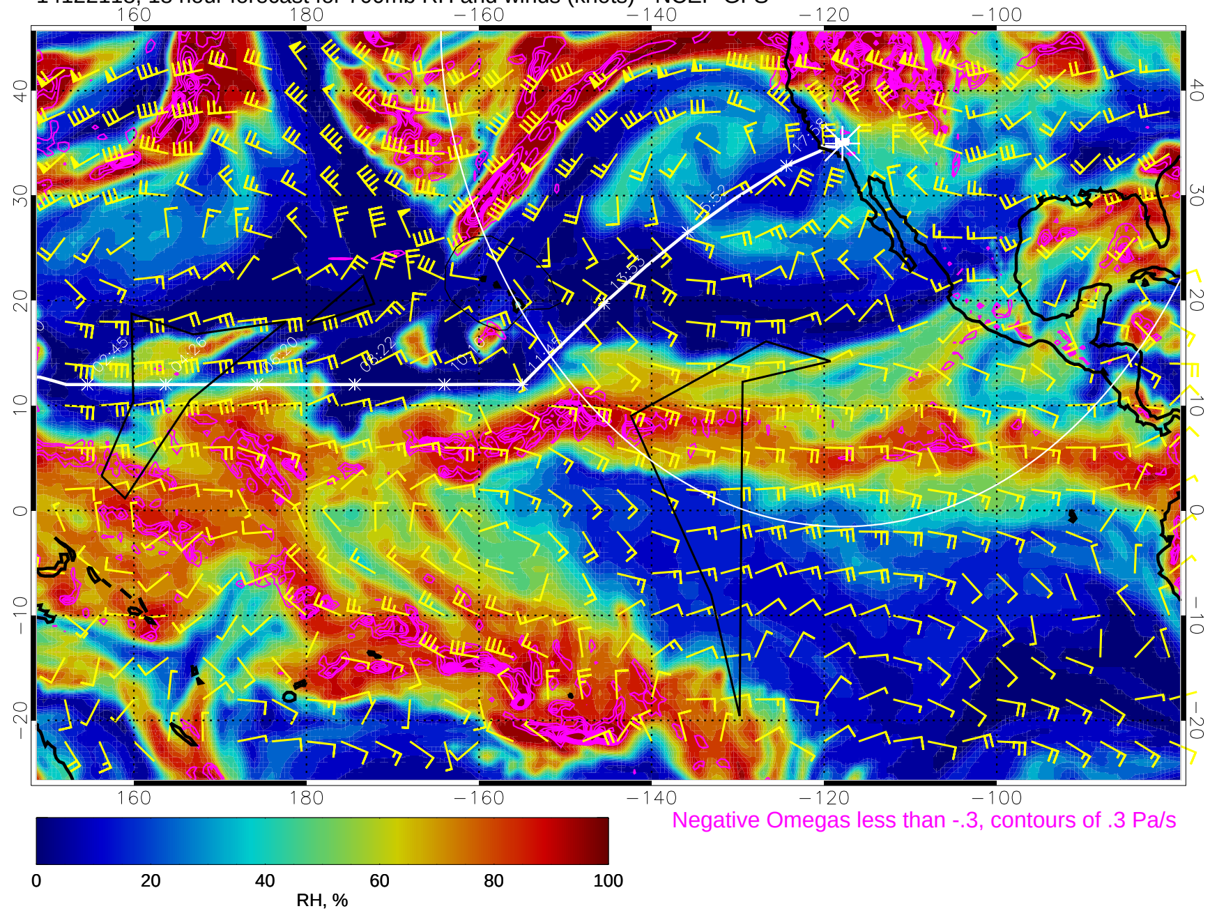
14122118, 18 hour forecast for 700mb RH and winds (knots) - NCEP GFS
