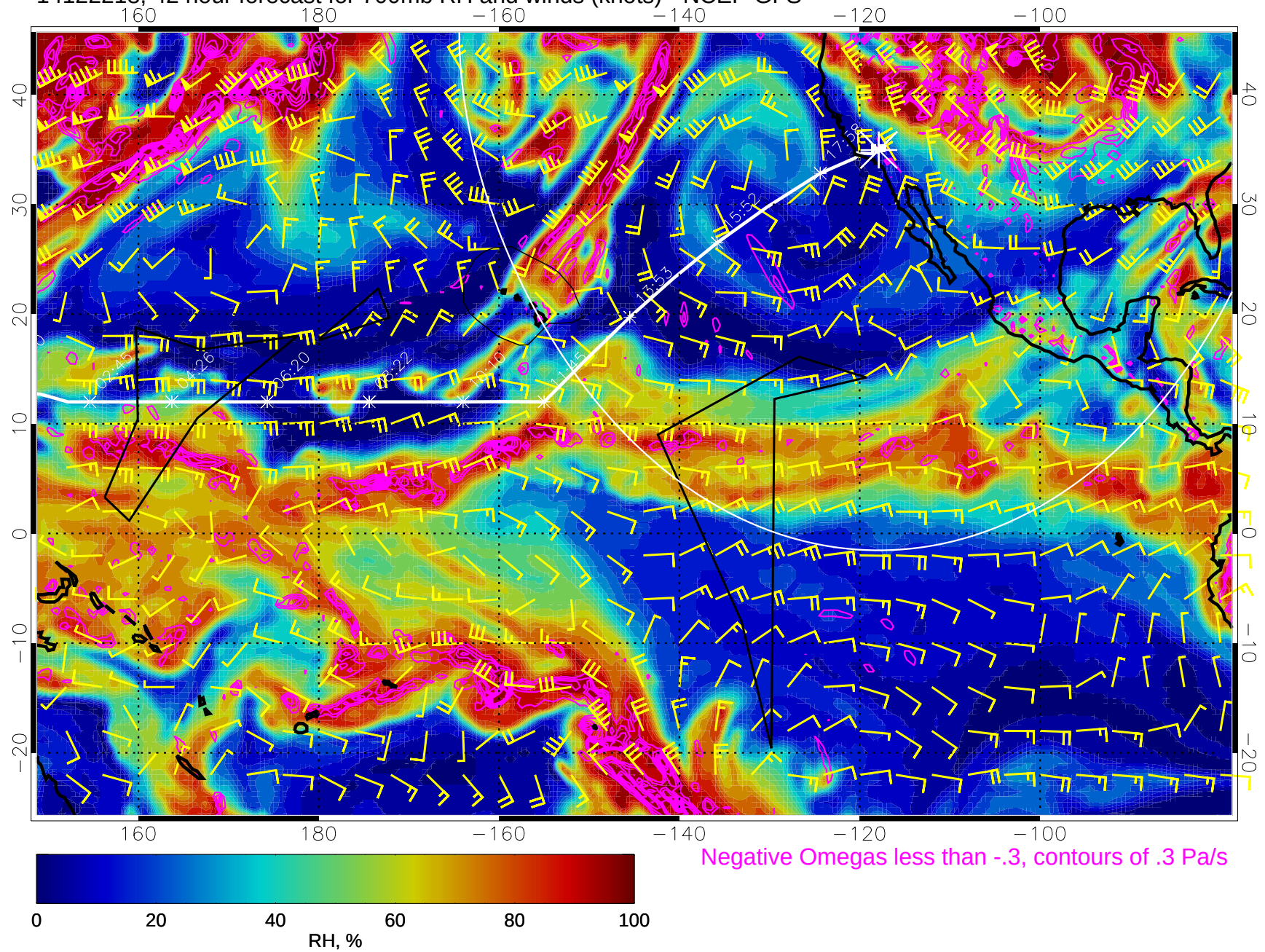
14122218, 42 hour forecast for 700mb RH and winds (knots) - NCEP GFS
