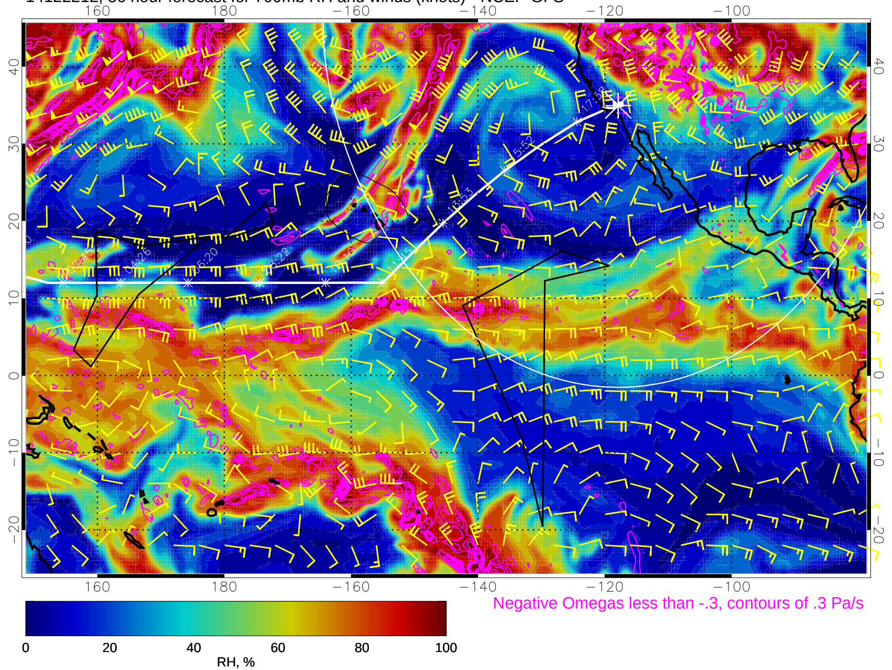
14122212, 36 hour forecast for 700mb RH and winds (knots) - NCEP GFS
