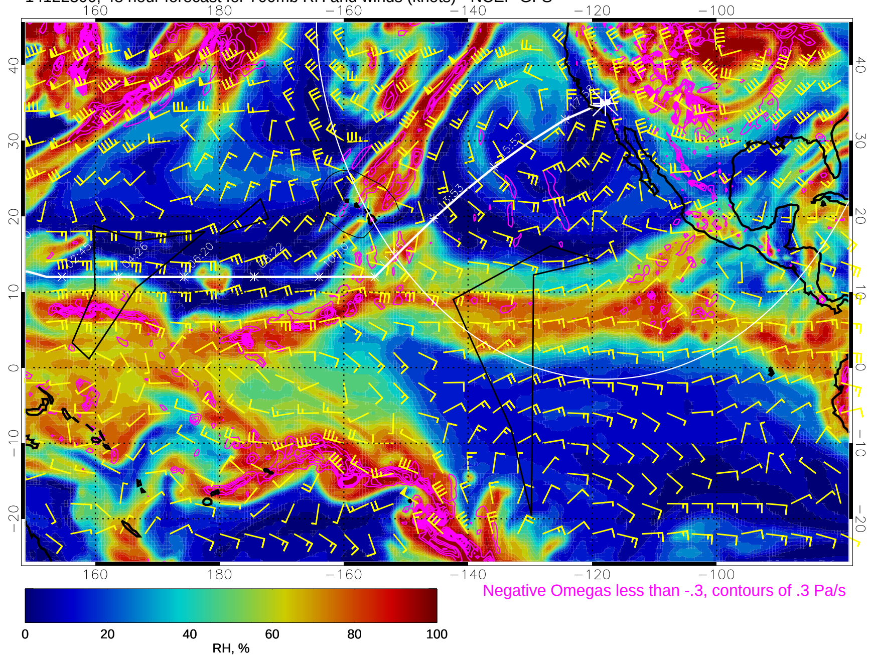
14122300, 48 hour forecast for 700mb RH and winds (knots) - NCEP GFS
