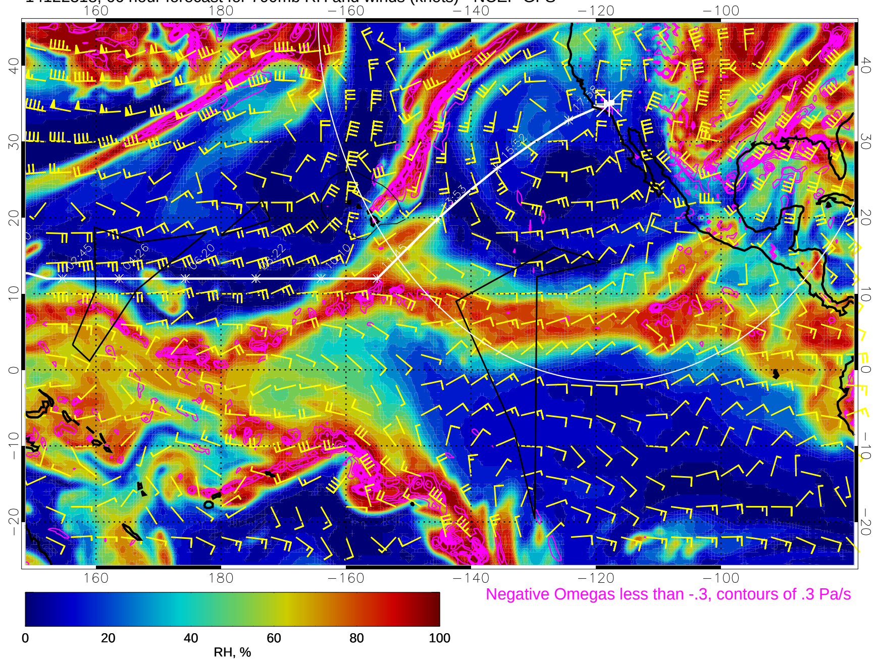
14122318, 66 hour forecast for 700mb RH and winds (knots) - NCEP GFS
