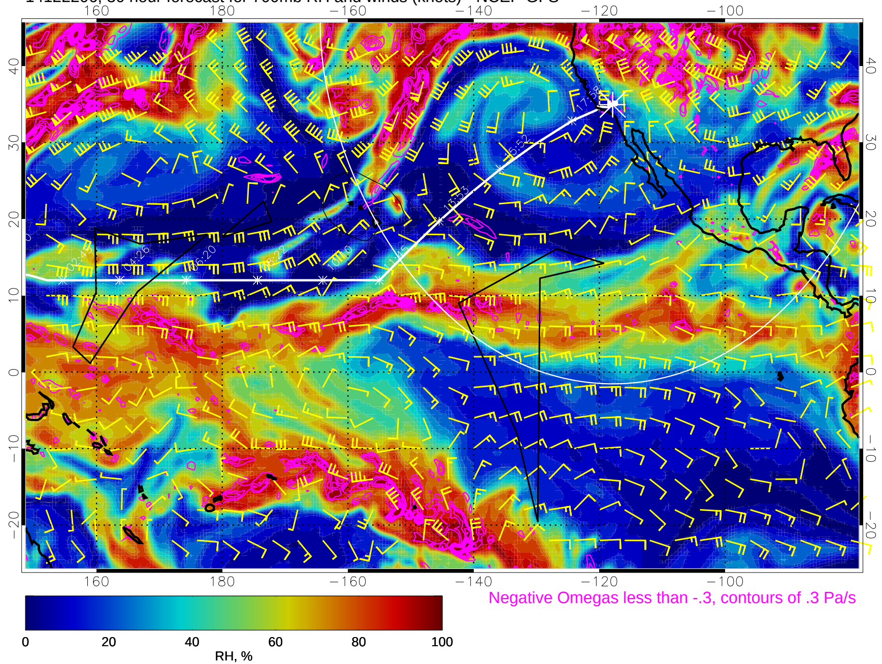
14122206, 30 hour forecast for 700mb RH and winds (knots) - NCEP GFS
