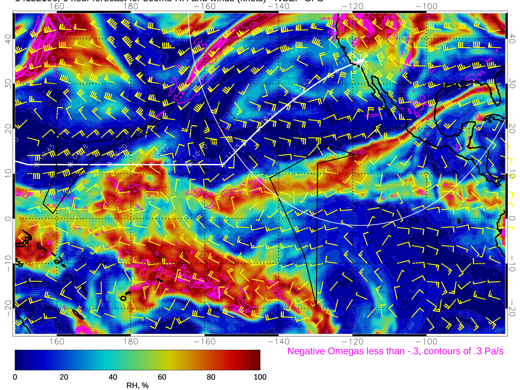
14122106, 6 hour forecast for 500mb RH and winds (knots) - NCEP GFS
