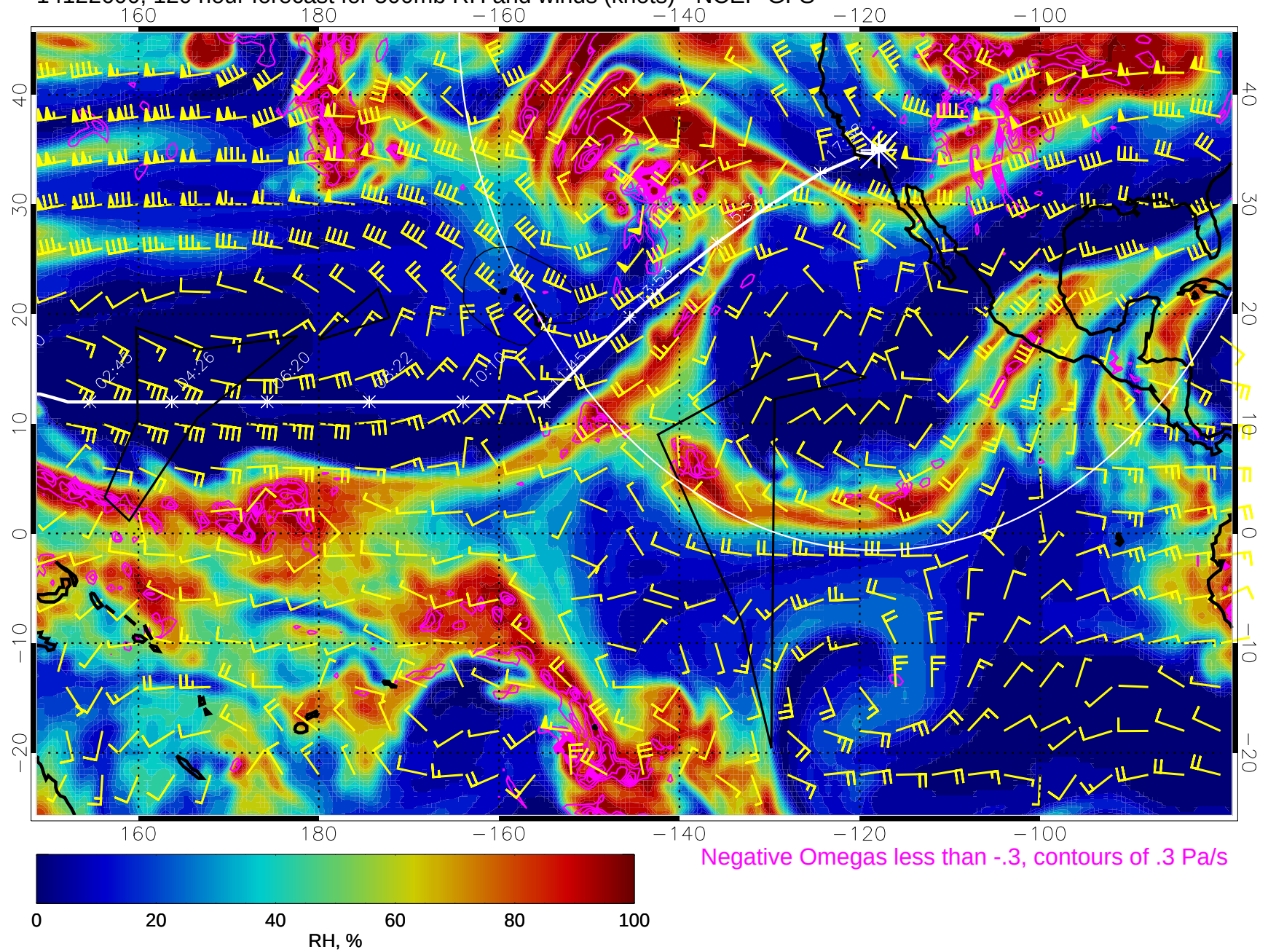
14122600, 120 hour forecast for 500mb RH and winds (knots) - NCEP GFS
