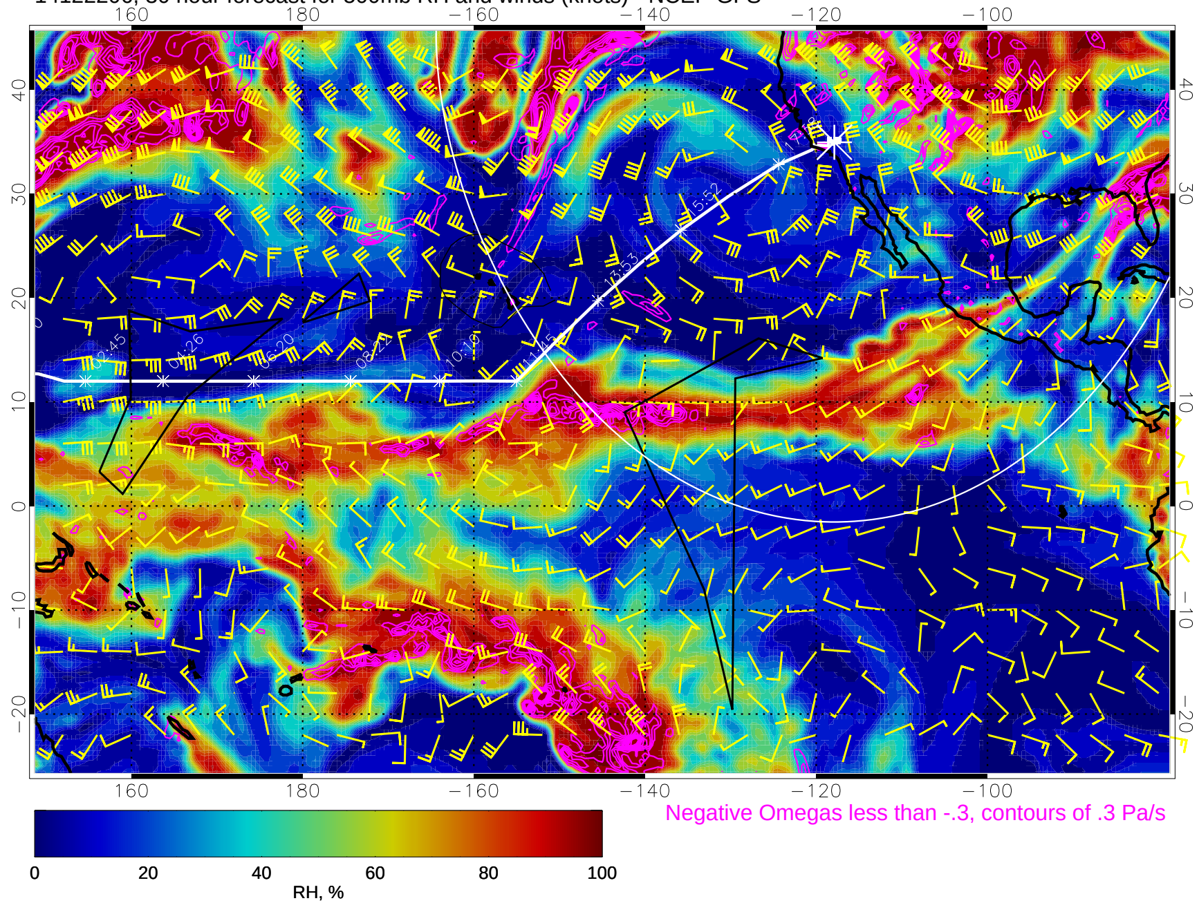
14122206, 30 hour forecast for 500mb RH and winds (knots) - NCEP GFS
