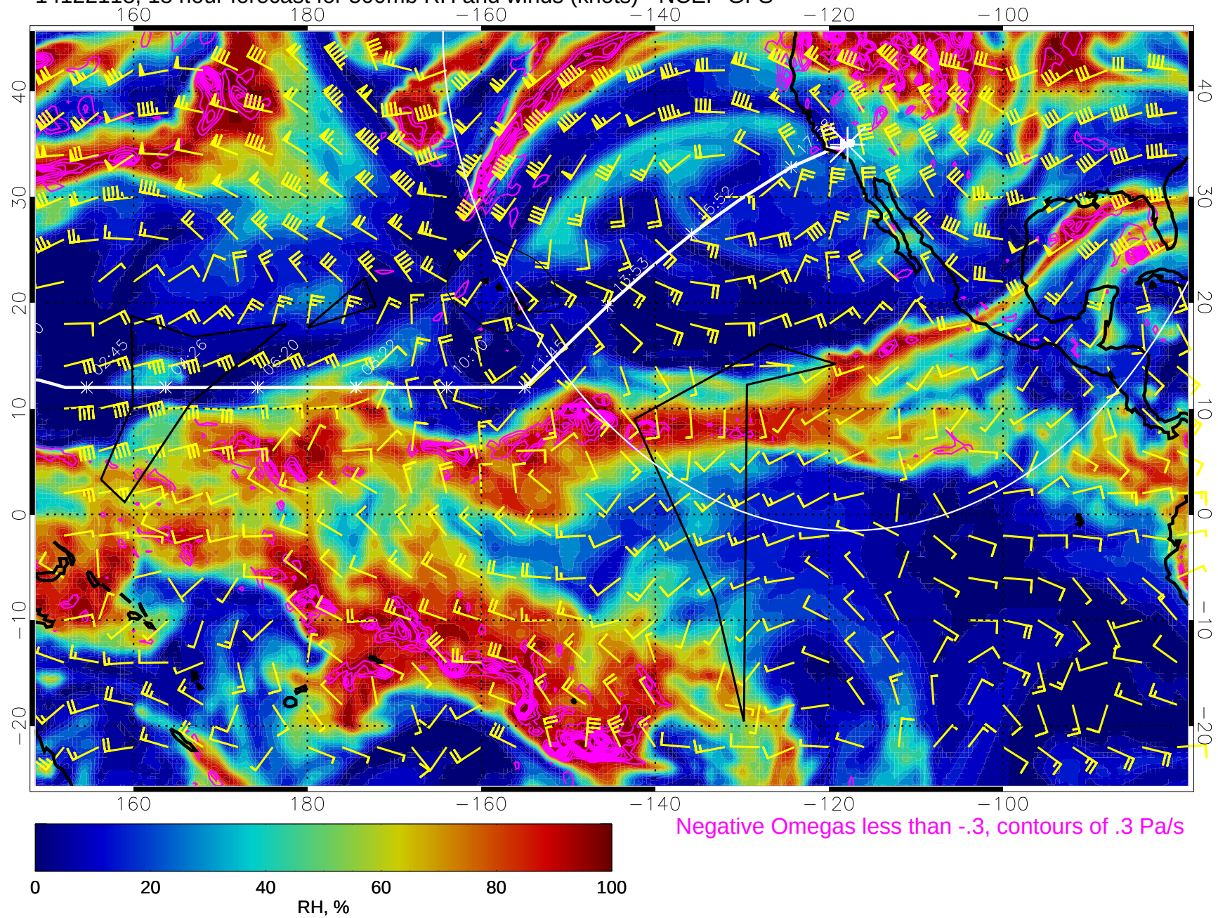
14122118, 18 hour forecast for 500mb RH and winds (knots) - NCEP GFS
