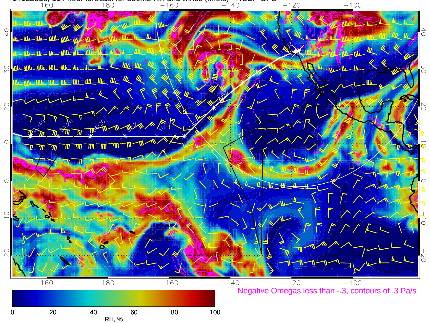
14122518, 114 hour forecast for 500mb RH and winds (knots) - NCEP GFS
