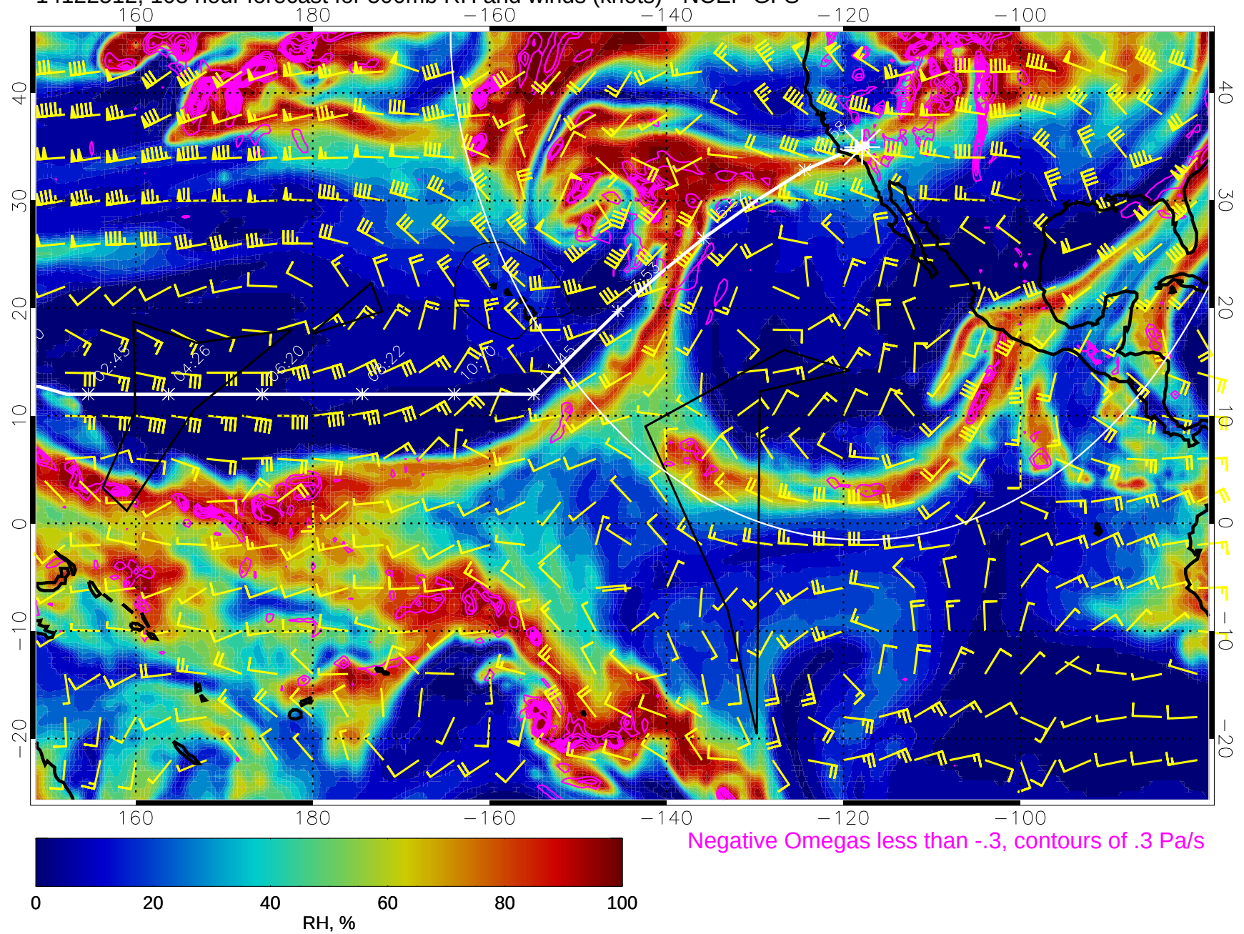
14122512, 108 hour forecast for 500mb RH and winds (knots) - NCEP GFS
