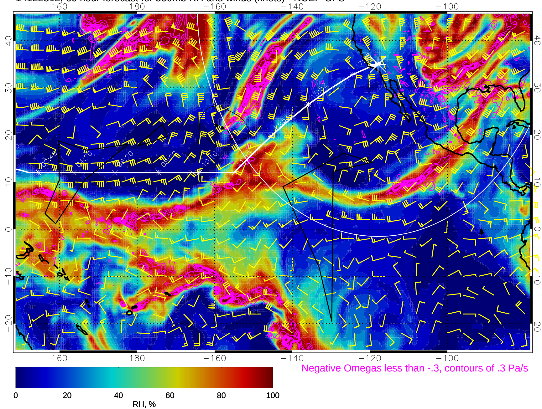
14122312, 60 hour forecast for 500mb RH and winds (knots) - NCEP GFS
