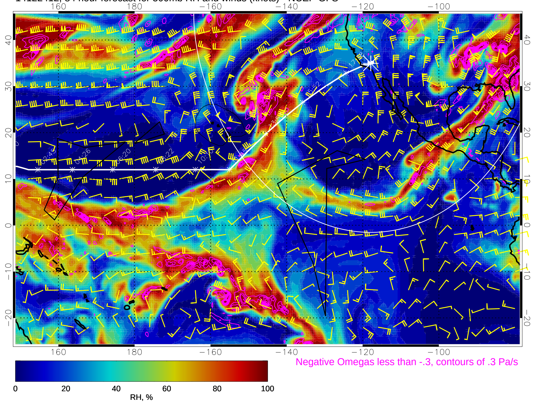
14122412, 84 hour forecast for 500mb RH and winds (knots) - NCEP GFS
