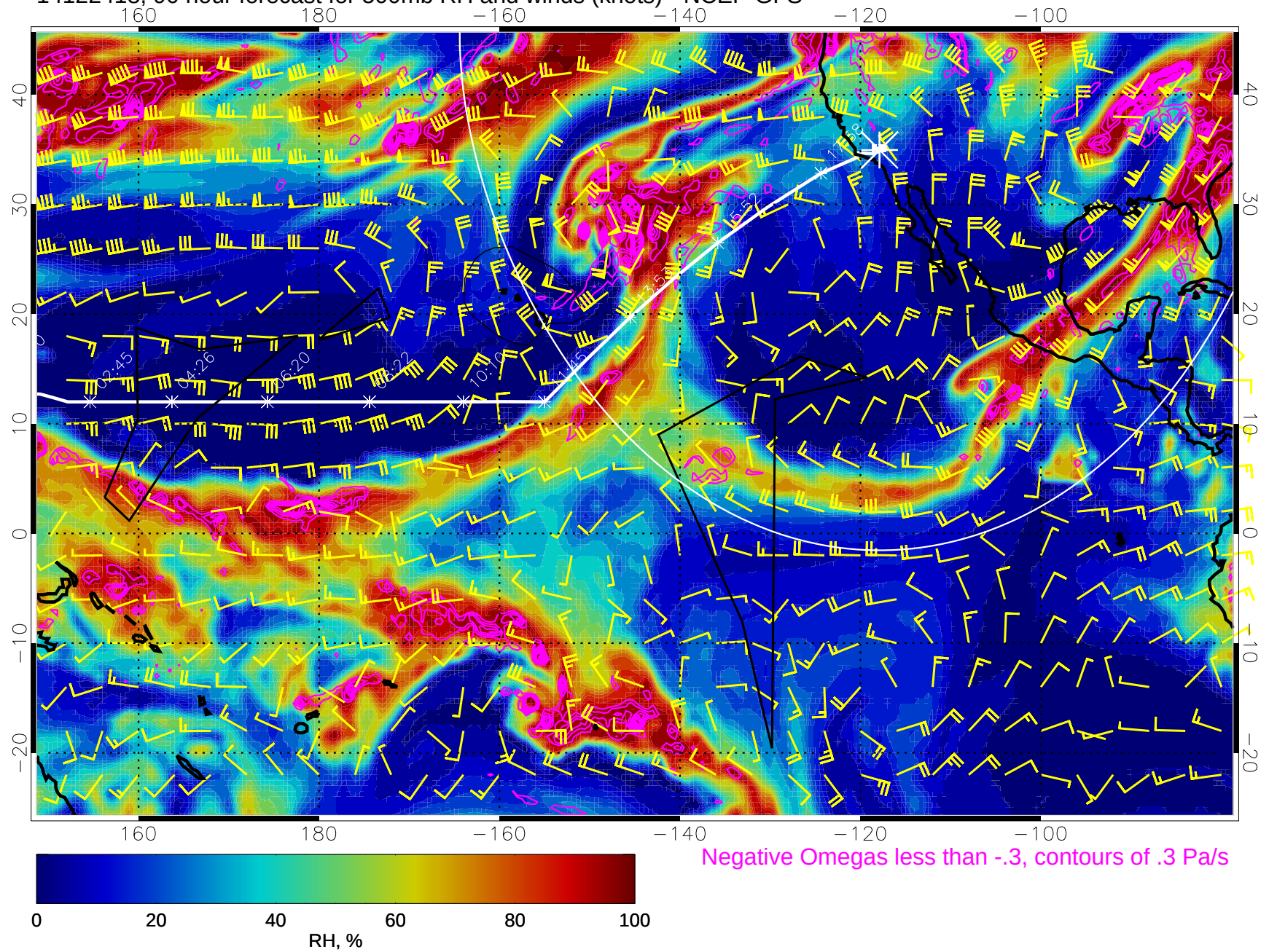
14122418, 90 hour forecast for 500mb RH and winds (knots) - NCEP GFS
