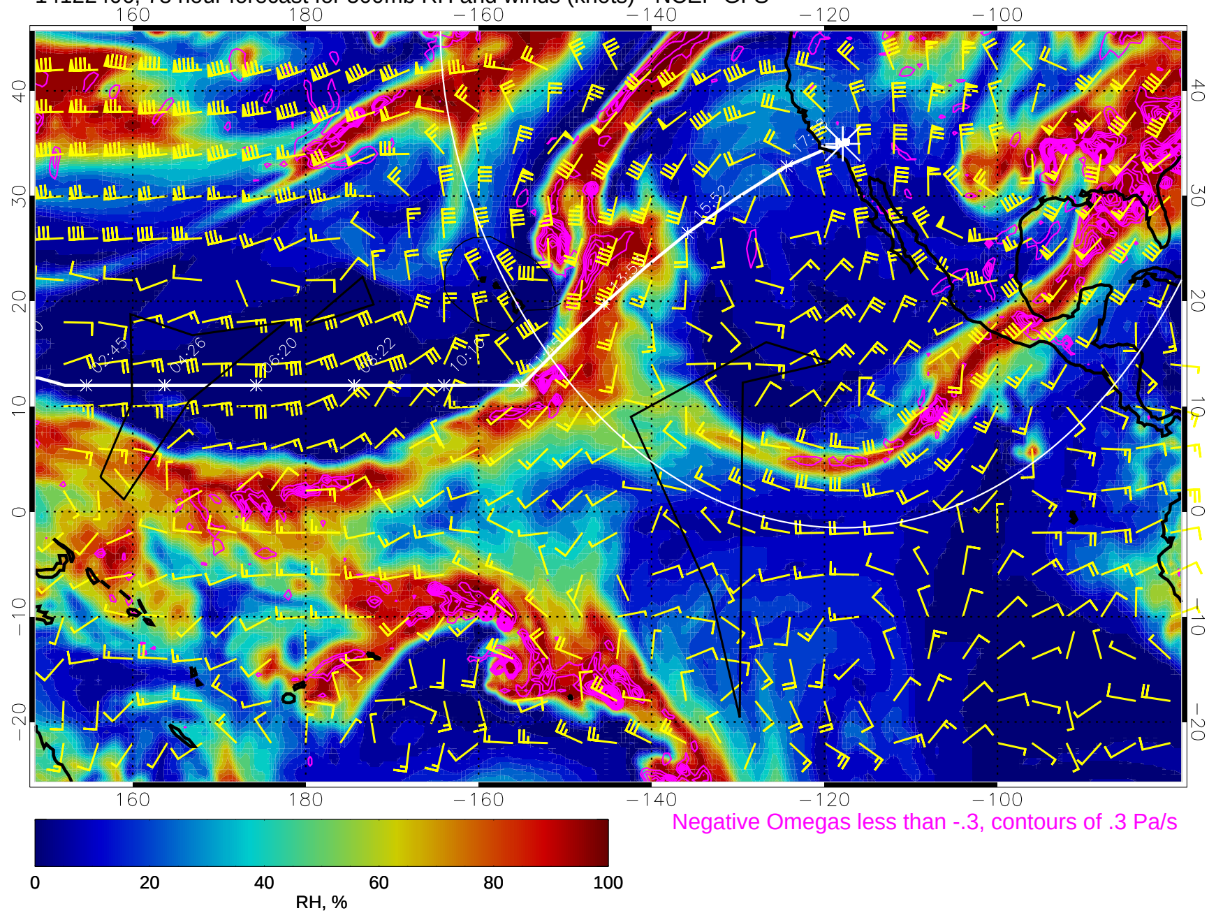
14122406, 78 hour forecast for 500mb RH and winds (knots) - NCEP GFS
