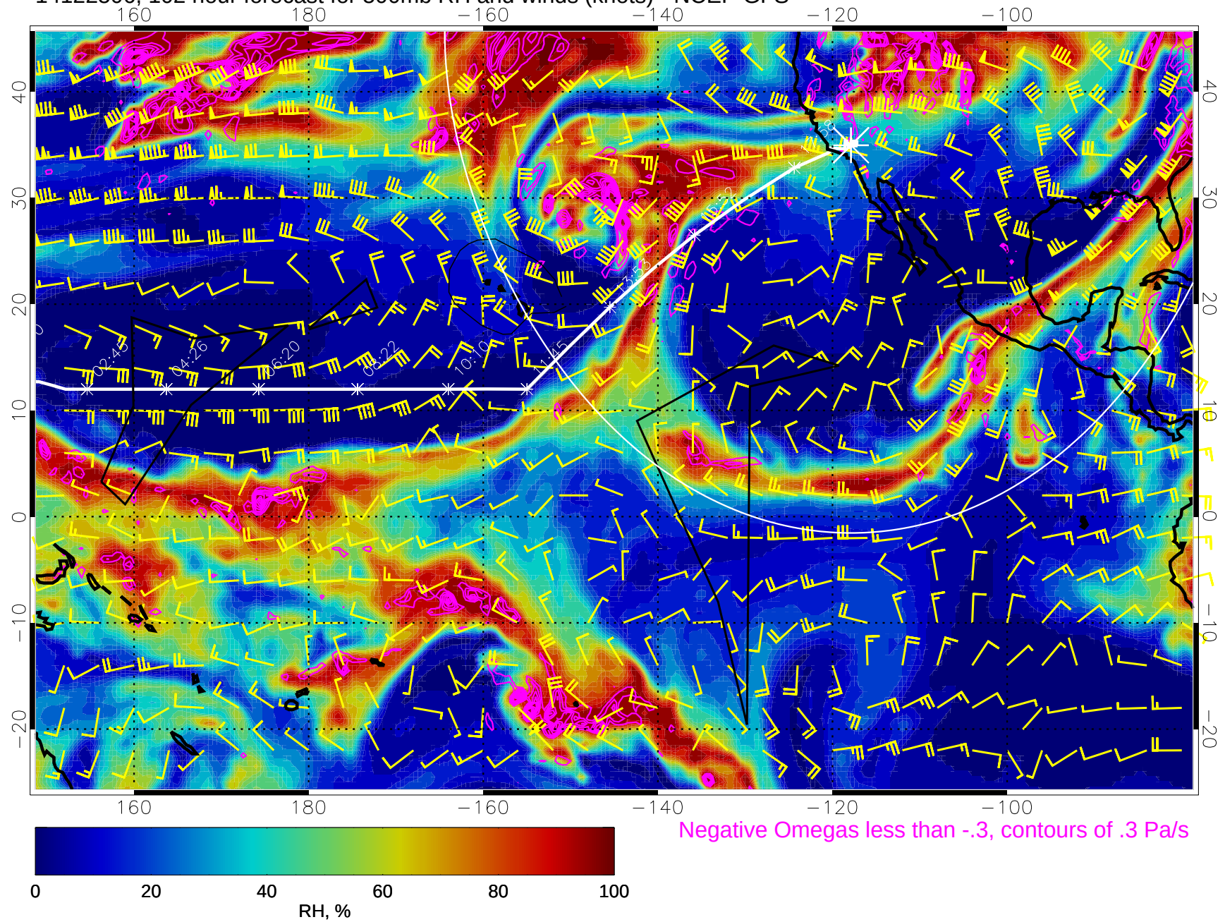
14122506, 102 hour forecast for 500mb RH and winds (knots) - NCEP GFS
