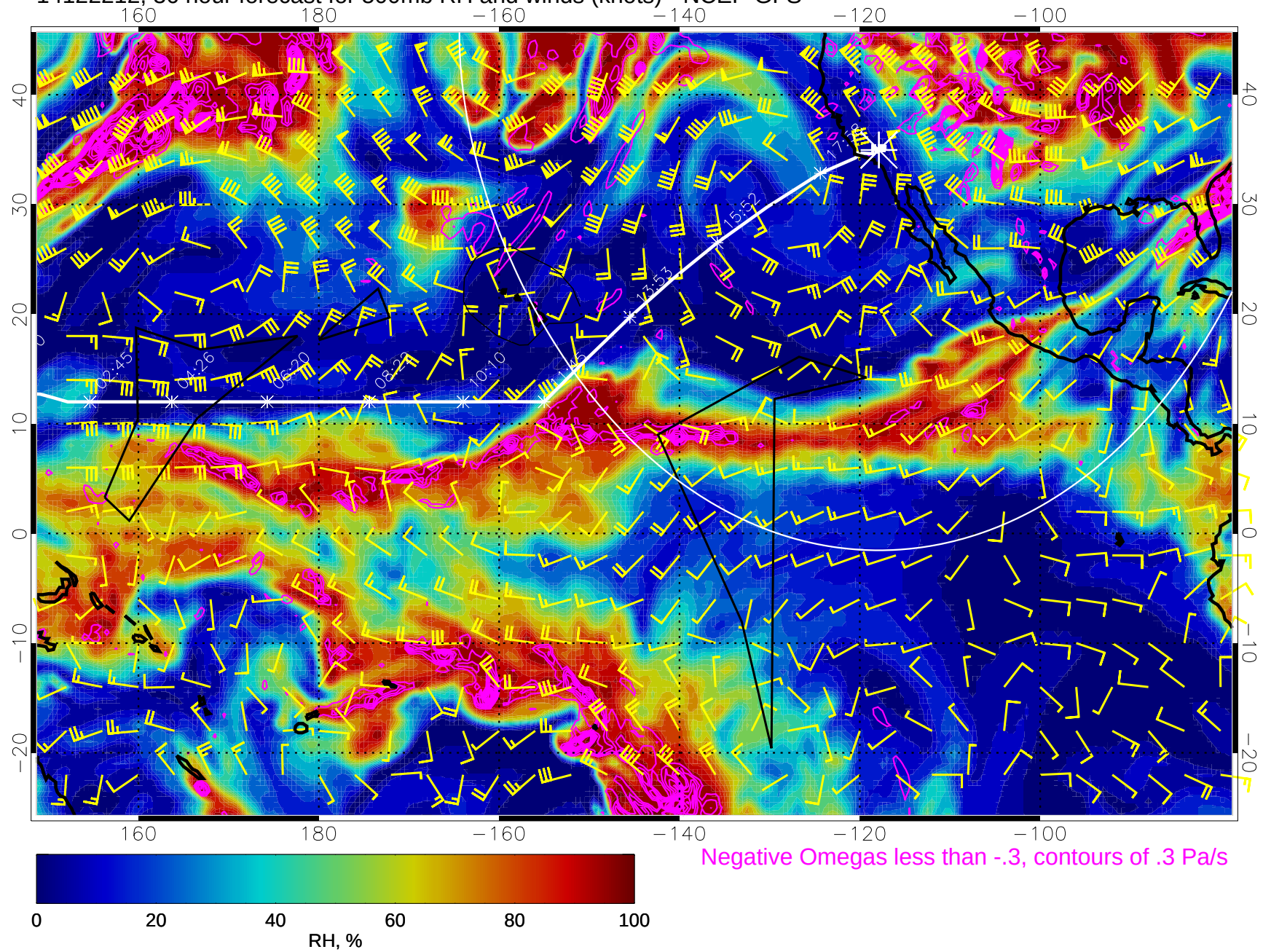
14122212, 36 hour forecast for 500mb RH and winds (knots) - NCEP GFS
