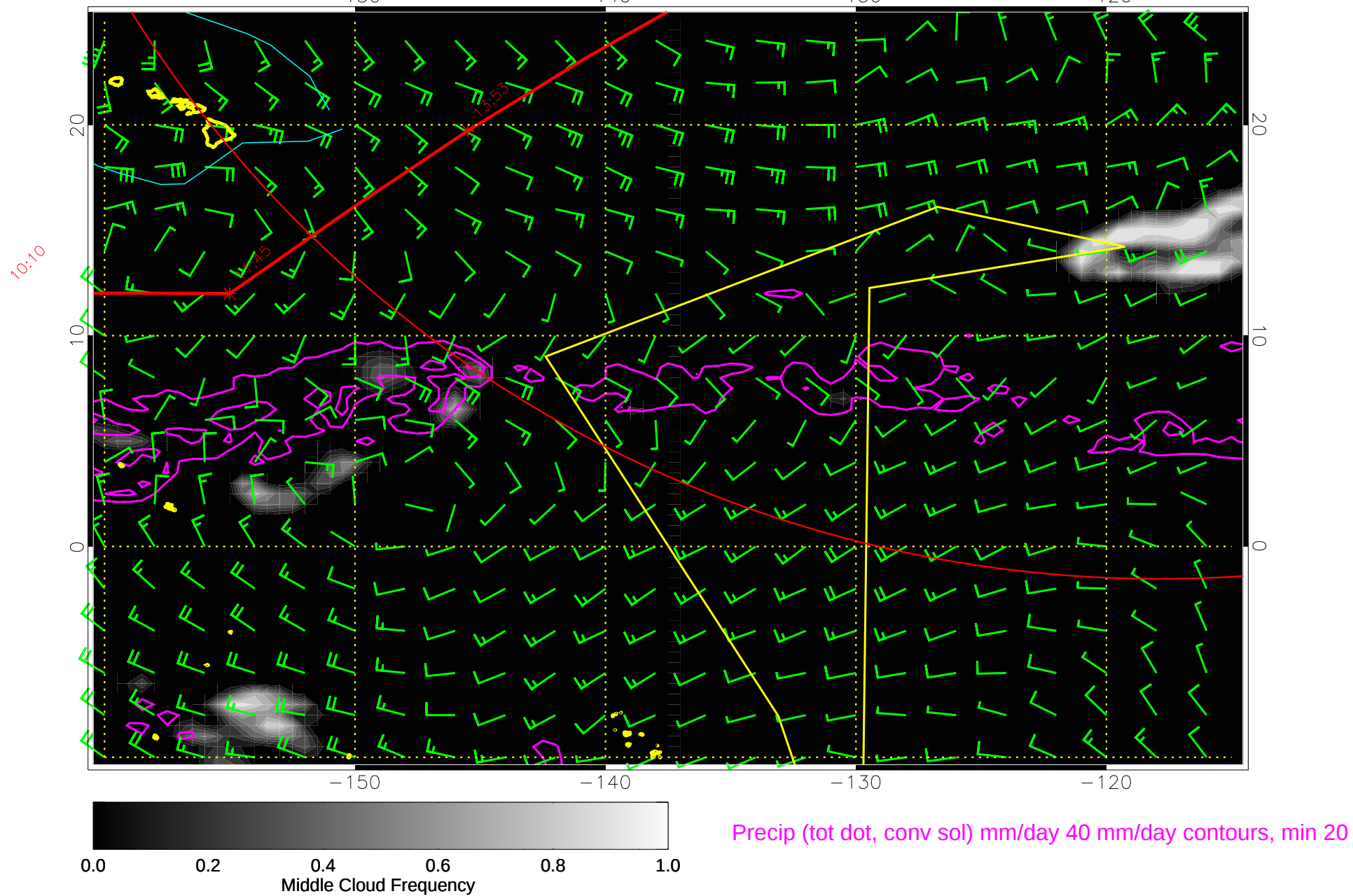
14122112, 12 hour forecast for 500mb winds (knots) and Middle Cloud Frequency -- NCEP GFS
