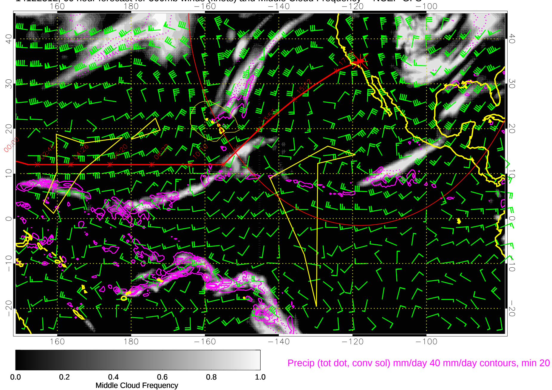
14122312, 60 hour forecast for 500mb winds (knots) and Middle Cloud Frequency -- NCEP GFS
