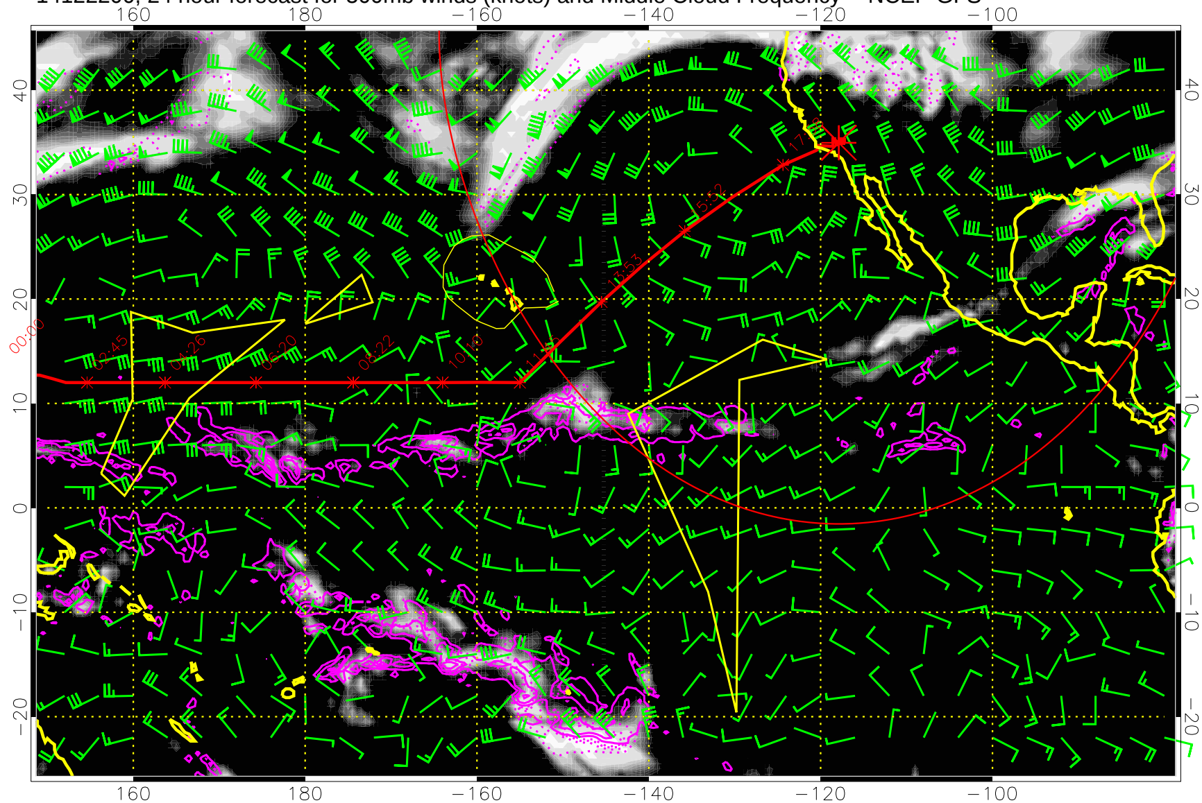
14122200, 24 hour forecast for 500mb winds (knots) and Middle Cloud Frequency -- NCEP GFS
