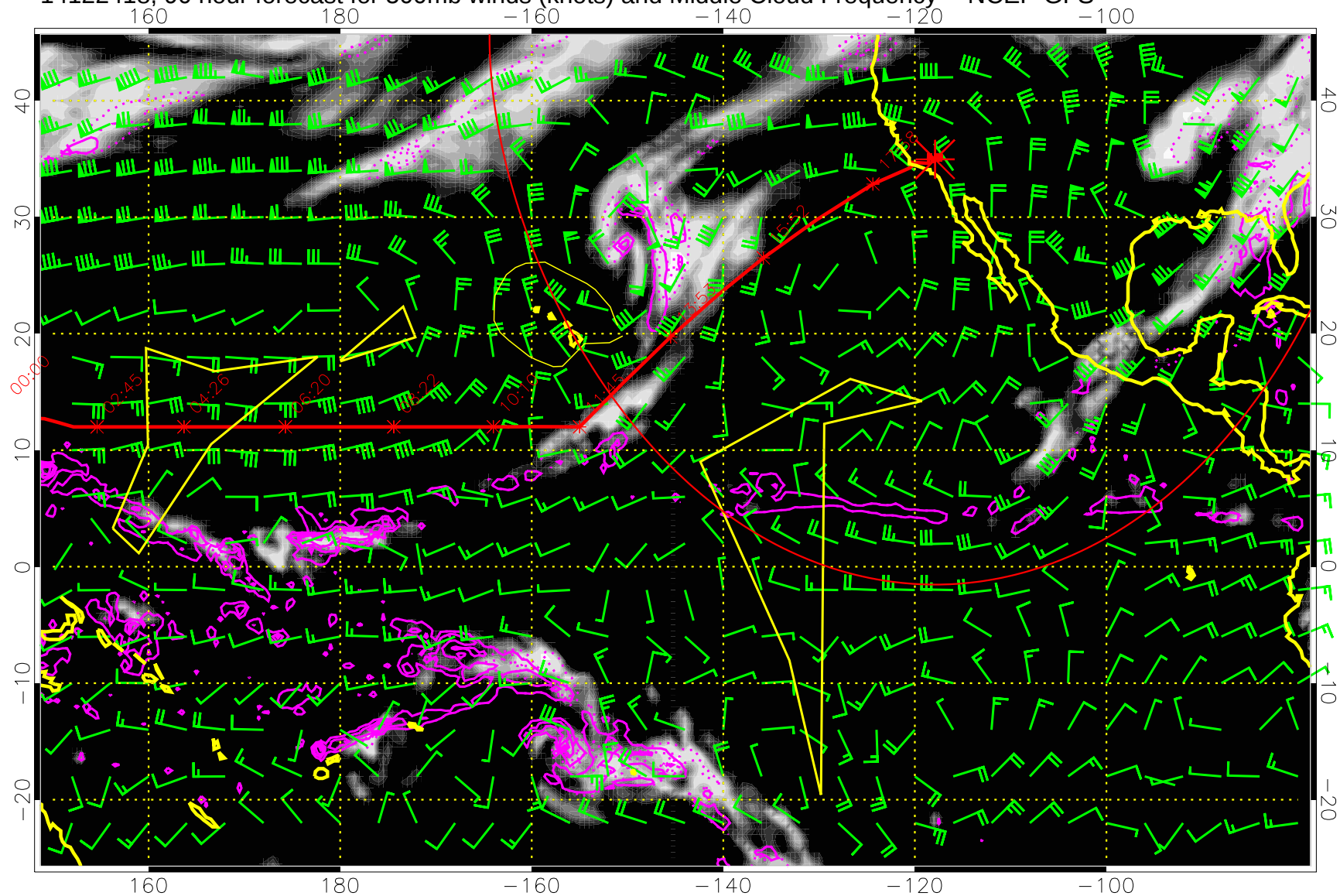
14122418, 90 hour forecast for 500mb winds (knots) and Middle Cloud Frequency -- NCEP GFS
