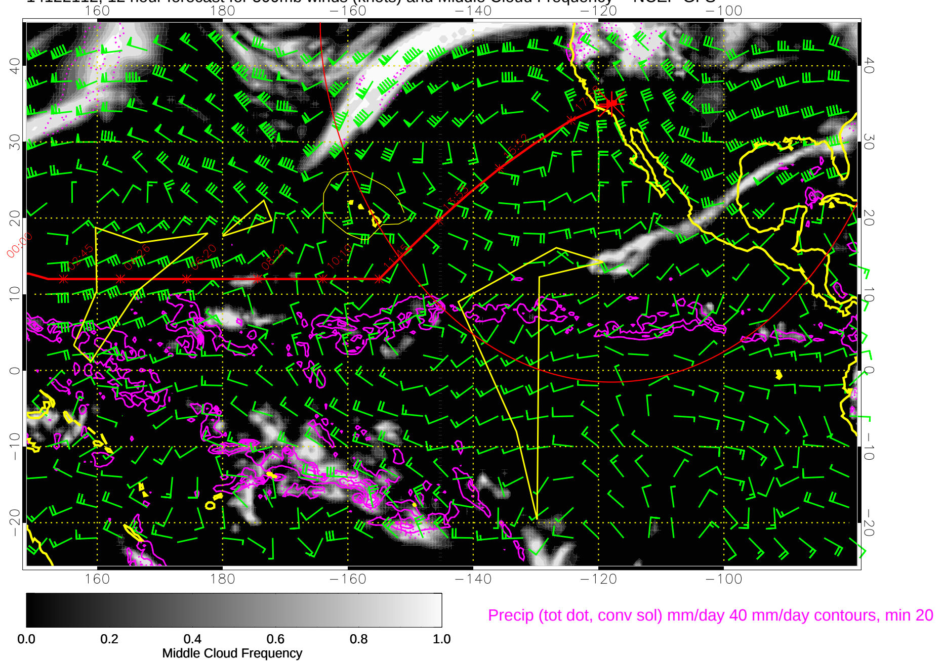
14122112, 12 hour forecast for 500mb winds (knots) and Middle Cloud Frequency -- NCEP GFS
