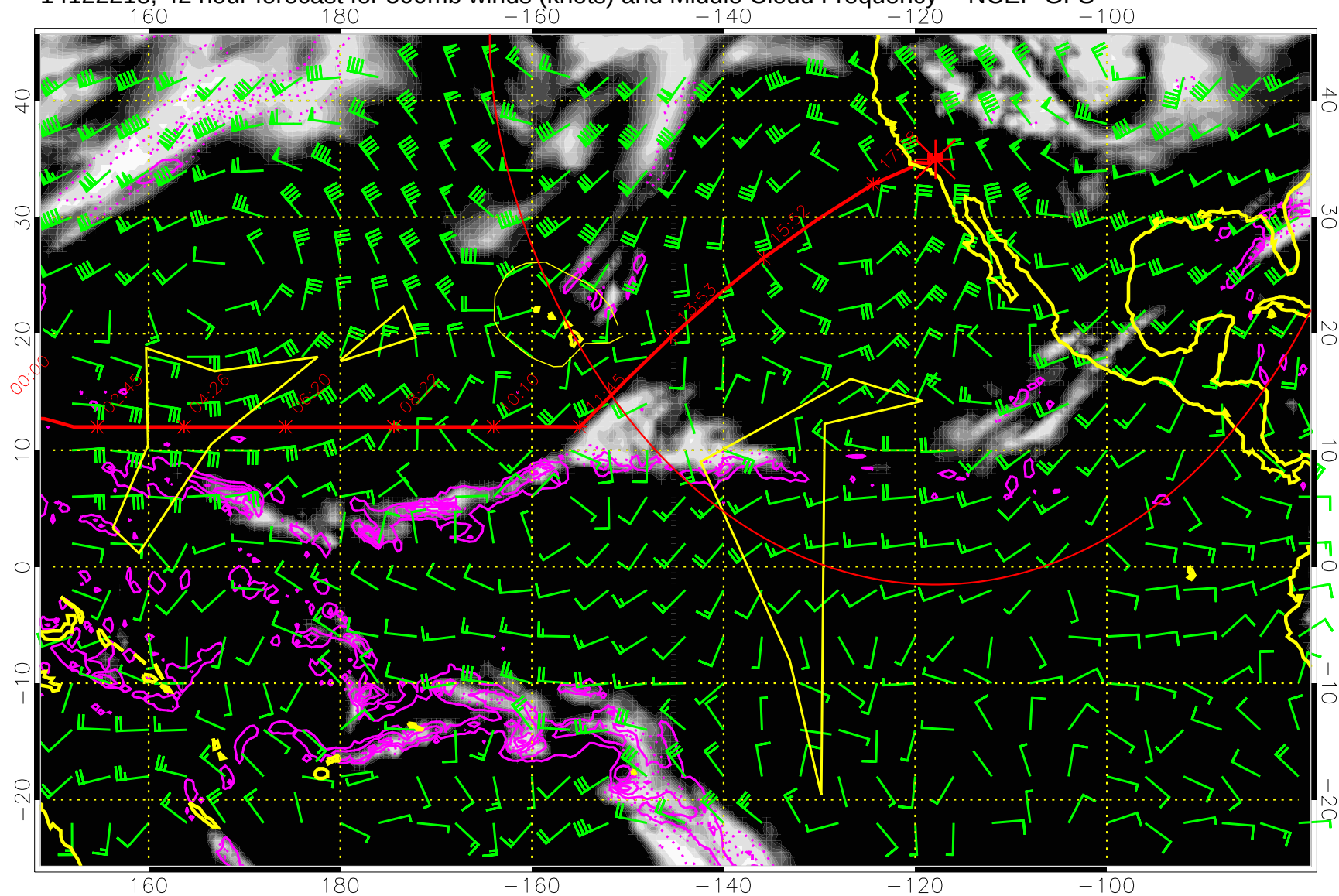
14122218, 42 hour forecast for 500mb winds (knots) and Middle Cloud Frequency -- NCEP GFS
