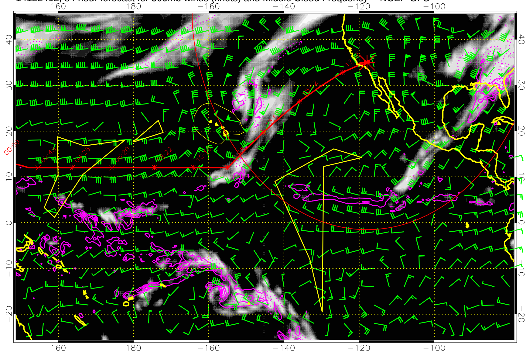
14122412, 84 hour forecast for 500mb winds (knots) and Middle Cloud Frequency -- NCEP GFS
