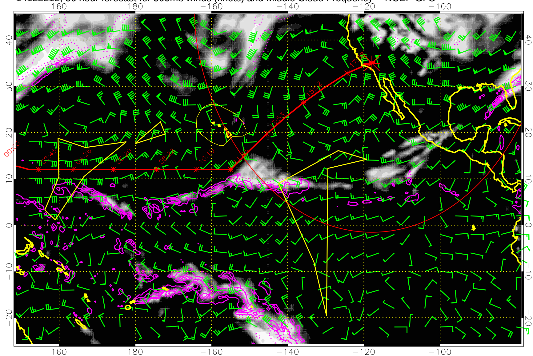
14122212, 36 hour forecast for 500mb winds (knots) and Middle Cloud Frequency -- NCEP GFS
