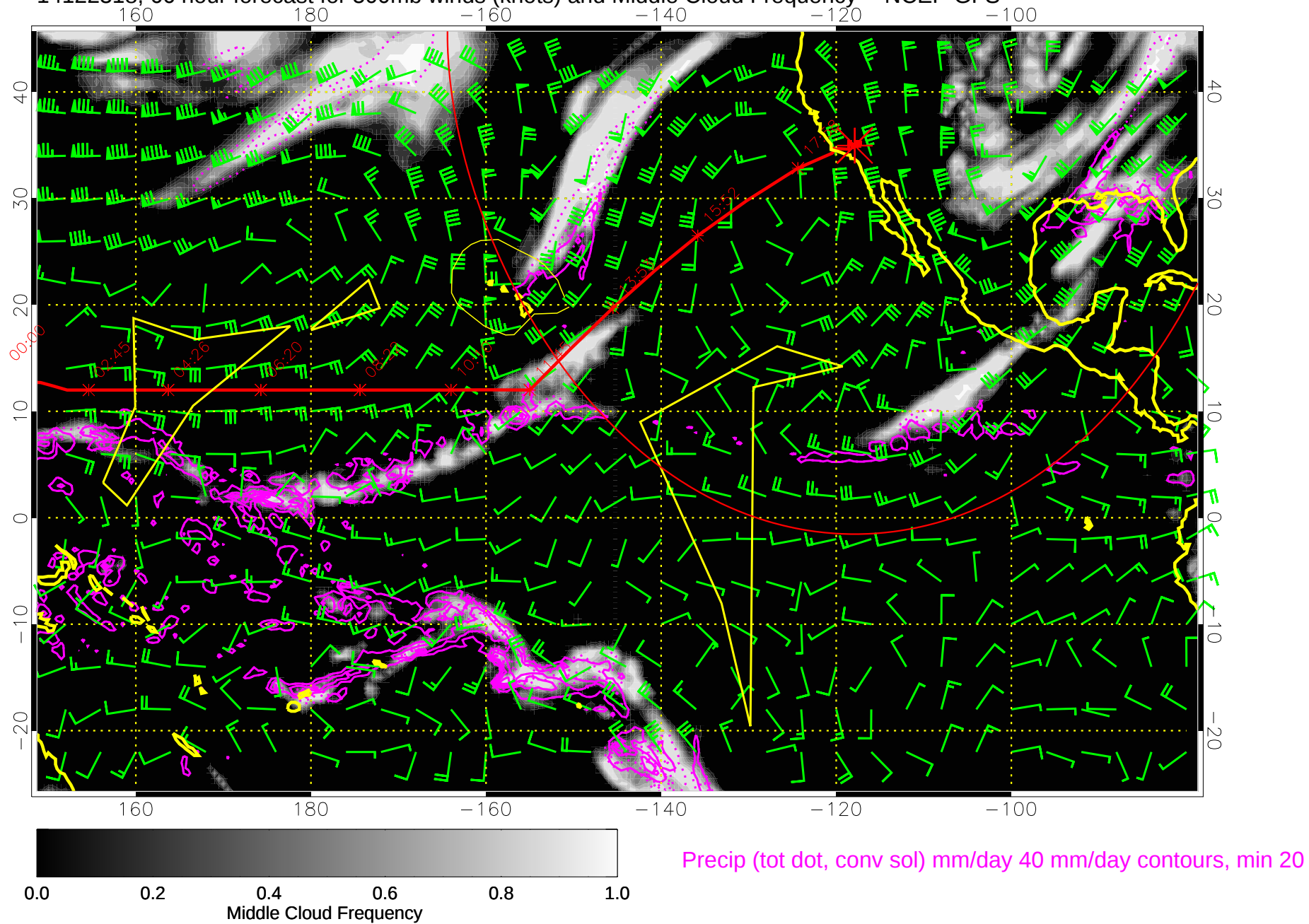
14122318, 66 hour forecast for 500mb winds (knots) and Middle Cloud Frequency -- NCEP GFS
