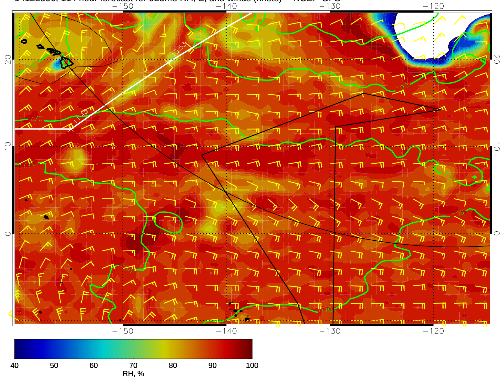
14122506, 114 hour forecast for 925mb RH, Z, and winds (knots) -- NCEP GFS
