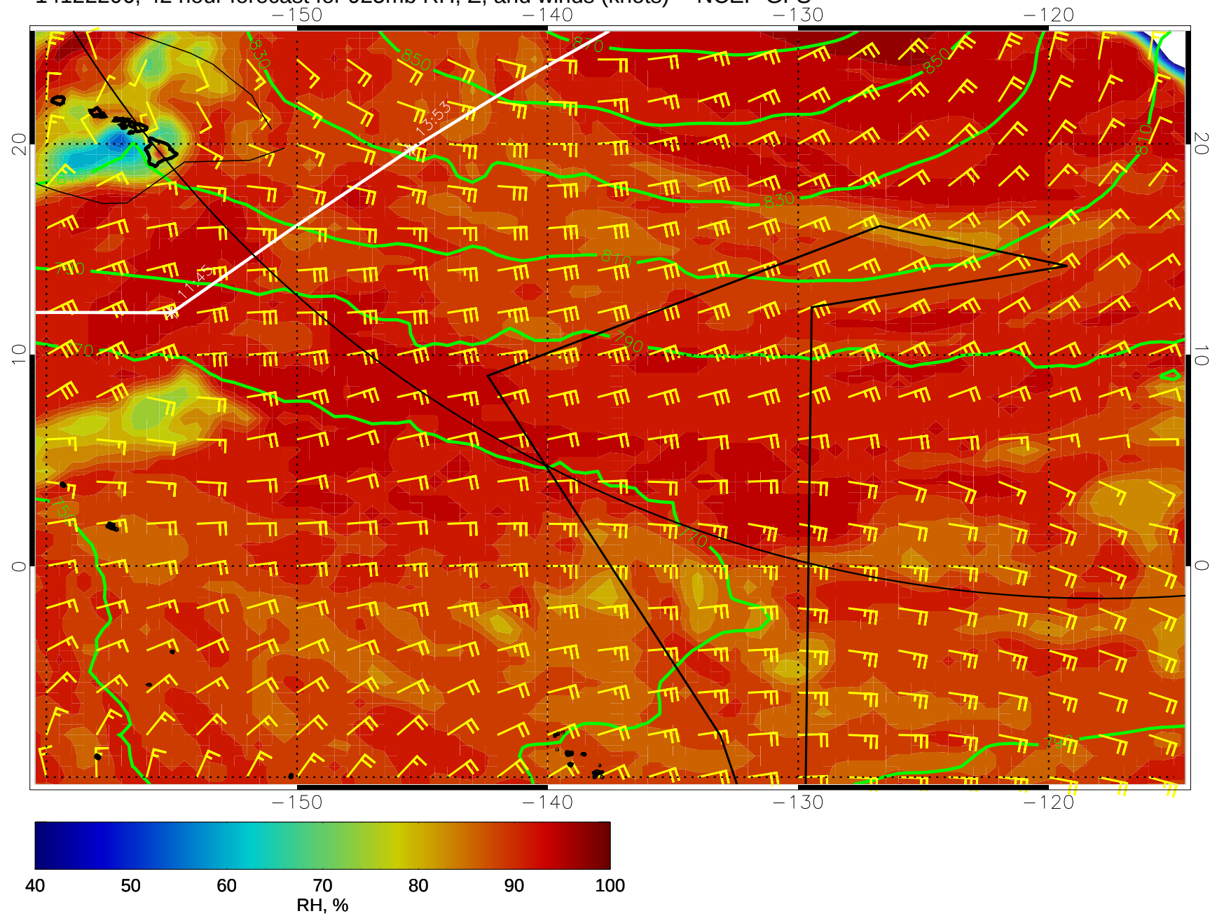
14122206, 42 hour forecast for 925mb RH, Z, and winds (knots) -- NCEP GFS
