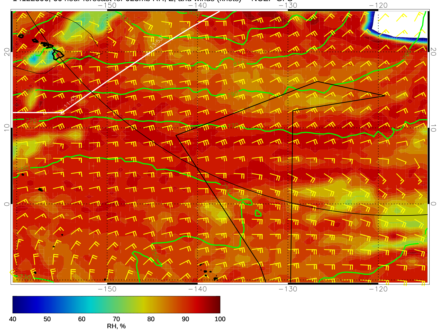
14122306, 66 hour forecast for 925mb RH, Z, and winds (knots) -- NCEP GFS
