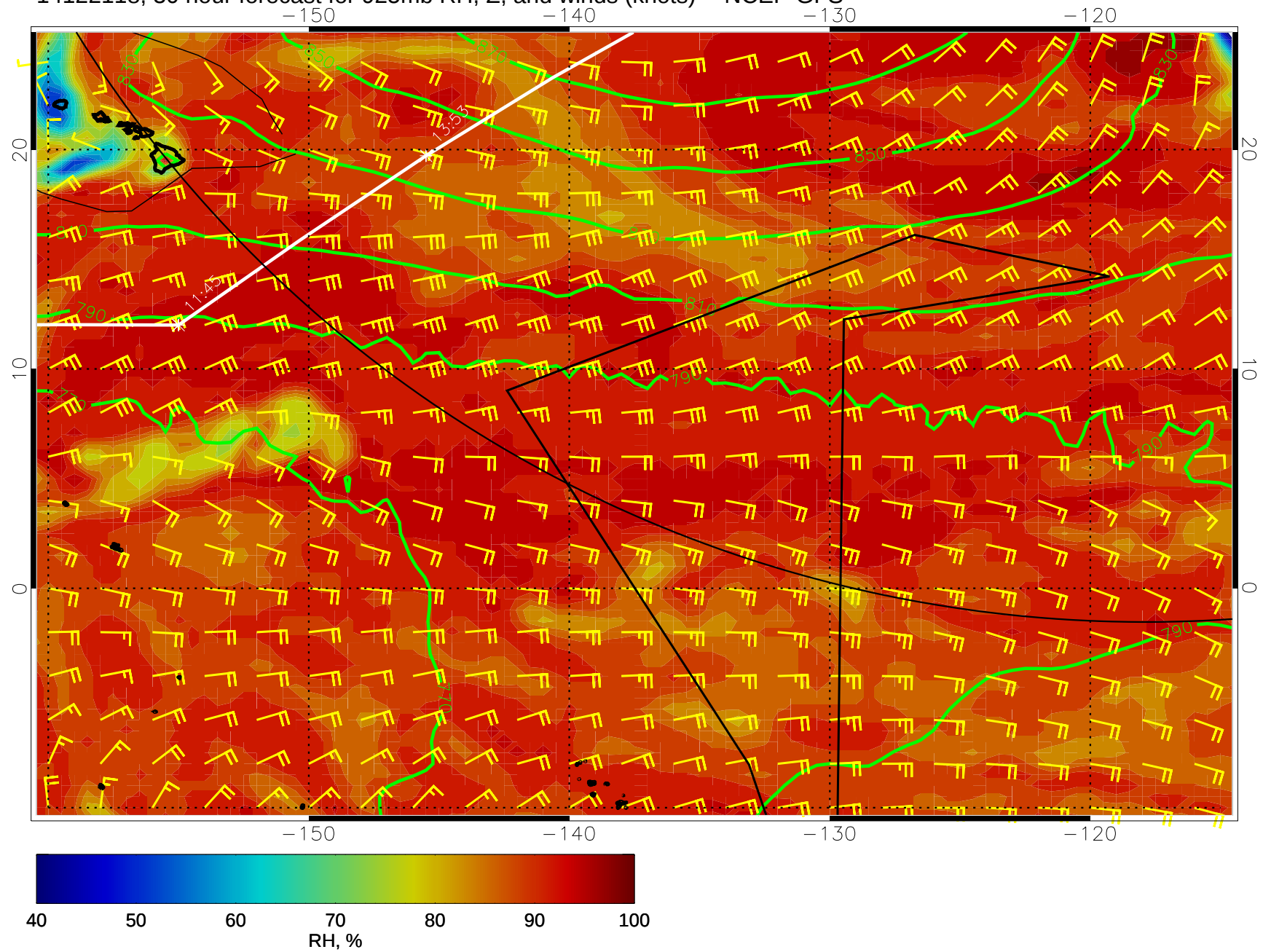
14122118, 30 hour forecast for 925mb RH, Z, and winds (knots) -- NCEP GFS
