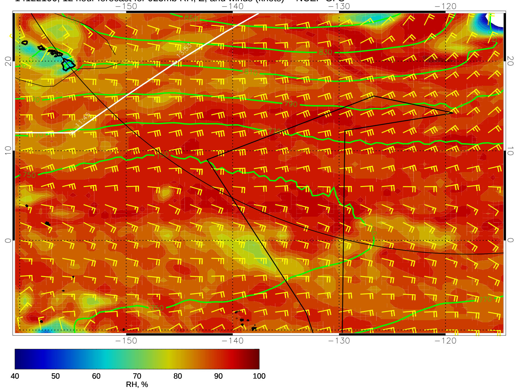
14122100, 12 hour forecast for 925mb RH, Z, and winds (knots) -- NCEP GFS
