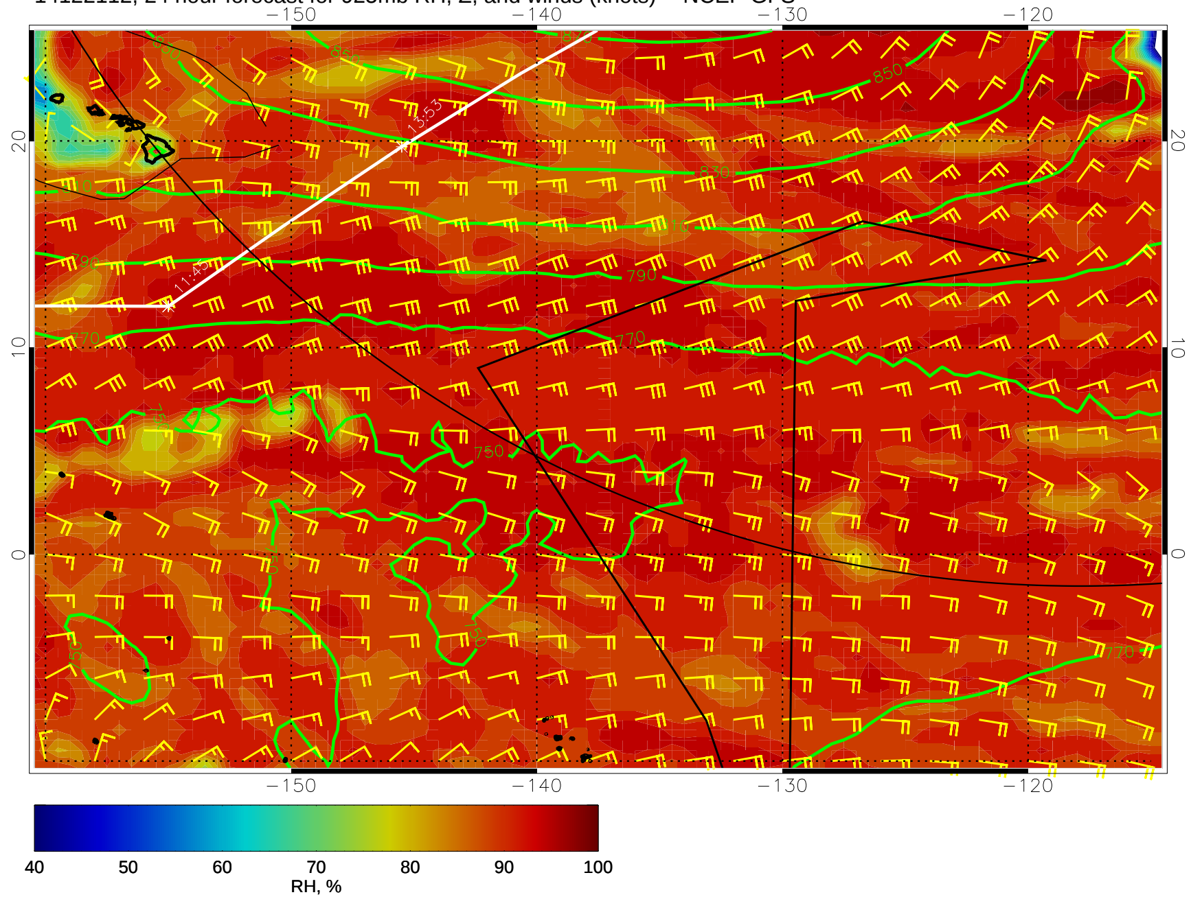
14122112, 24 hour forecast for 925mb RH, Z, and winds (knots) -- NCEP GFS
