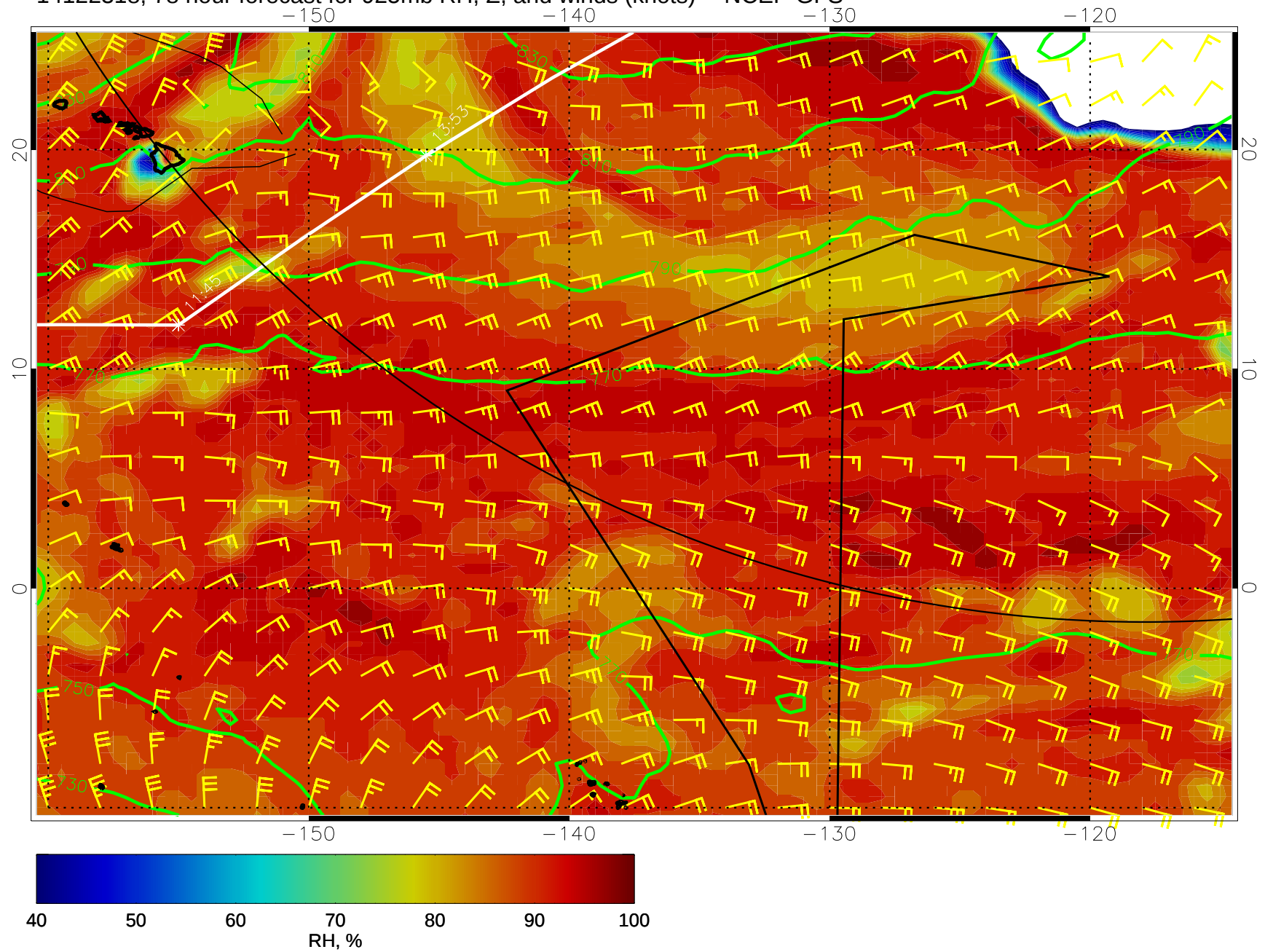
14122318, 78 hour forecast for 925mb RH, Z, and winds (knots) -- NCEP GFS
