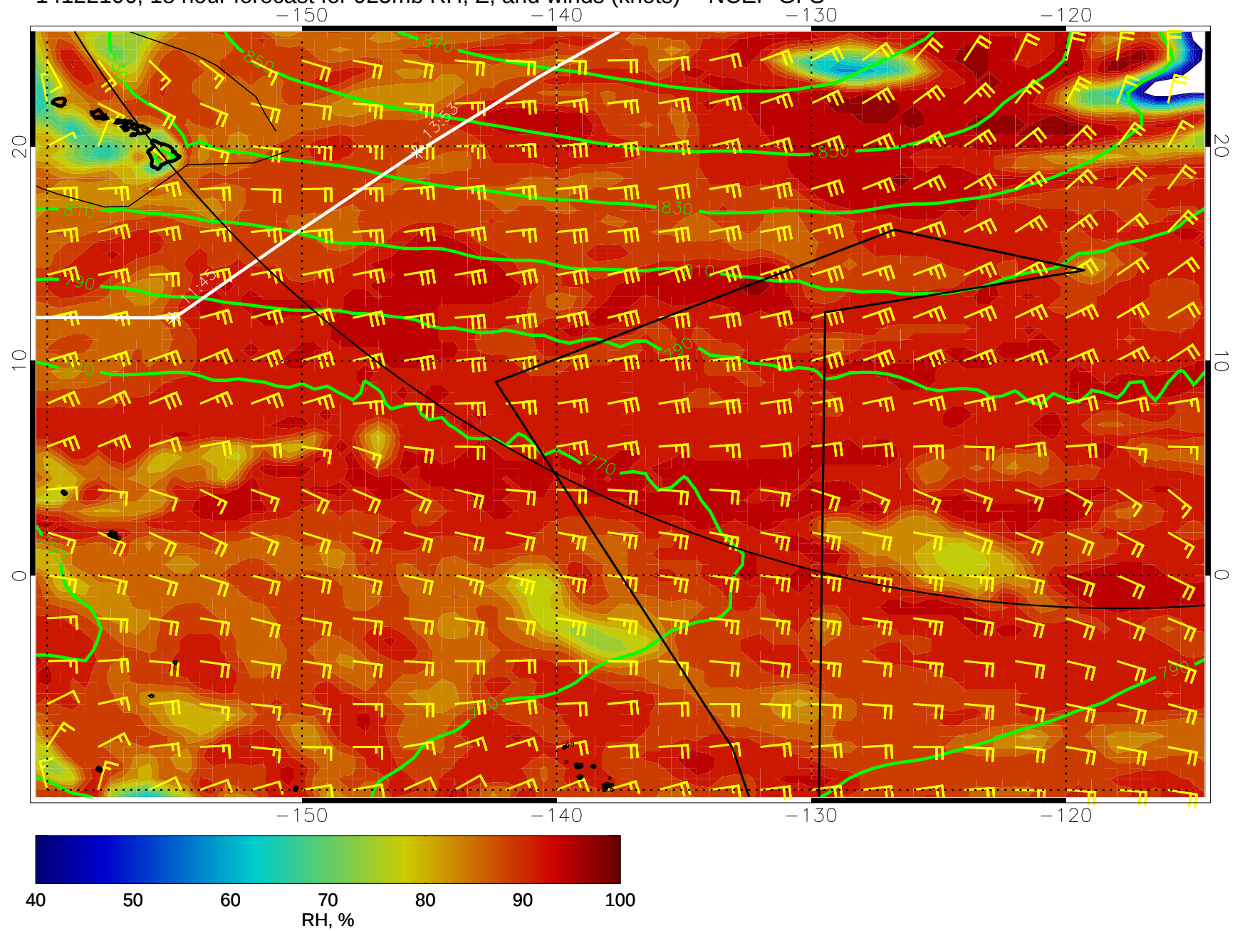
14122106, 18 hour forecast for 925mb RH, Z, and winds (knots) -- NCEP GFS
