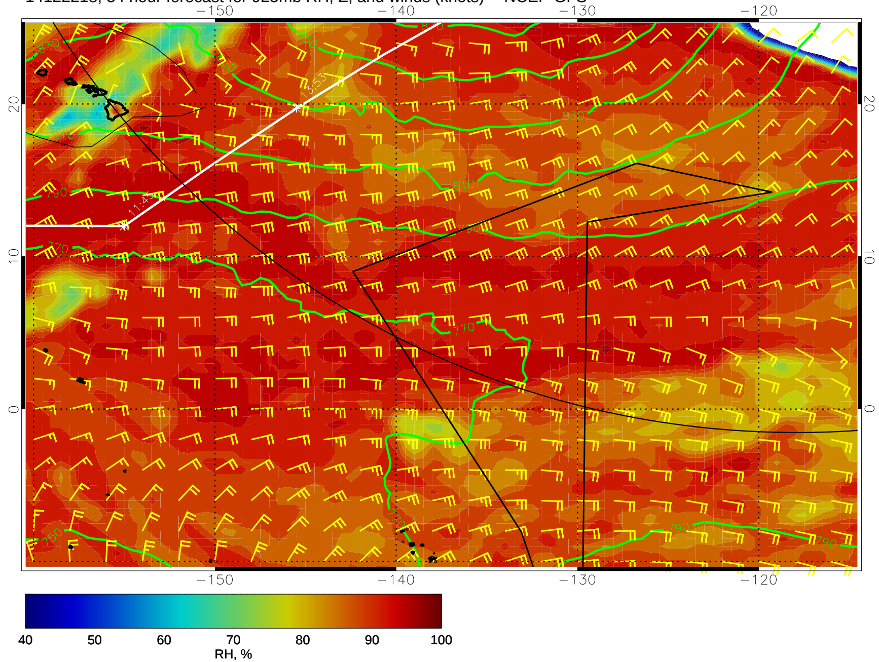
14122218, 54 hour forecast for 925mb RH, Z, and winds (knots) -- NCEP GFS
