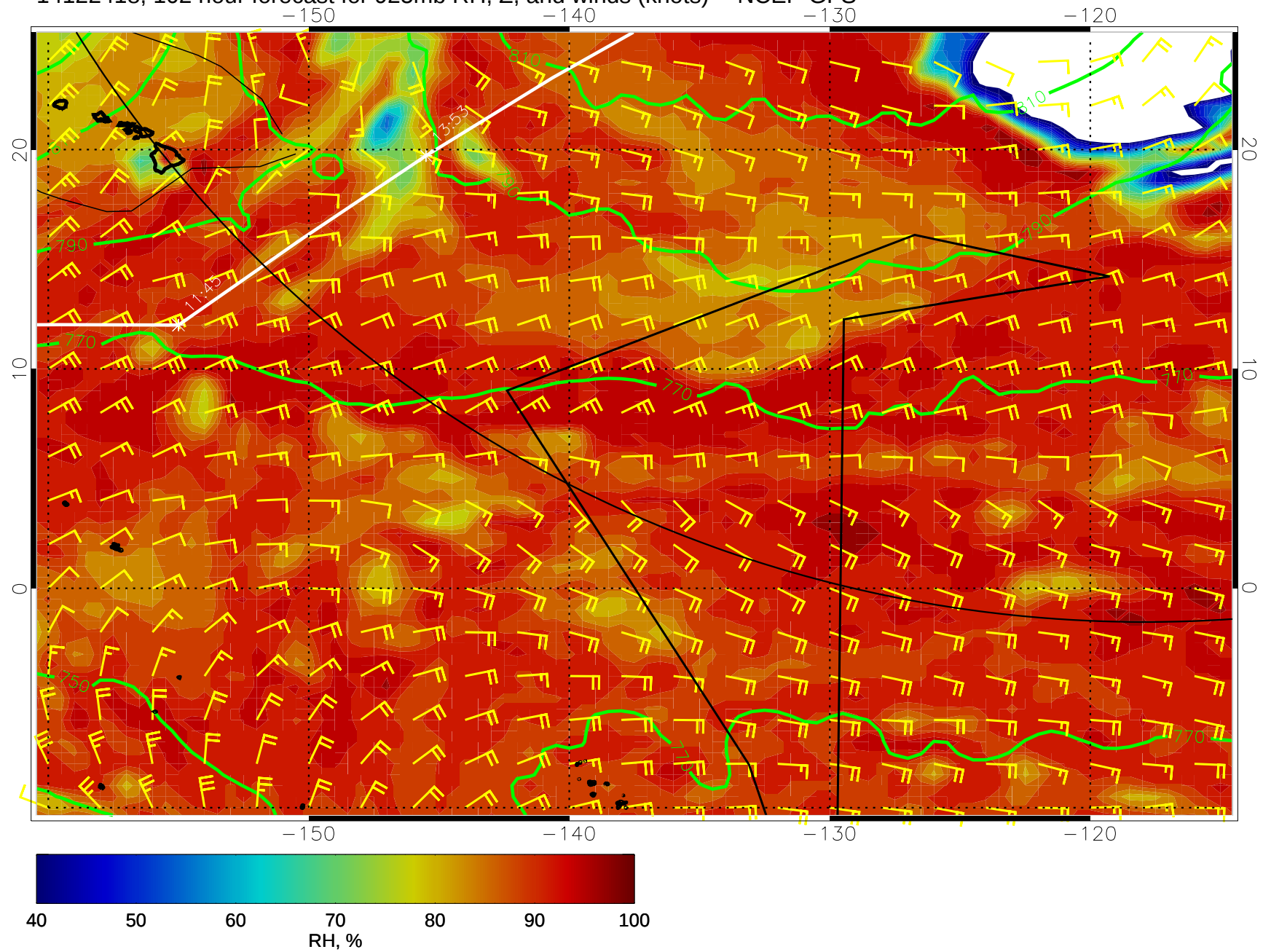
14122418, 102 hour forecast for 925mb RH, Z, and winds (knots) -- NCEP GFS
