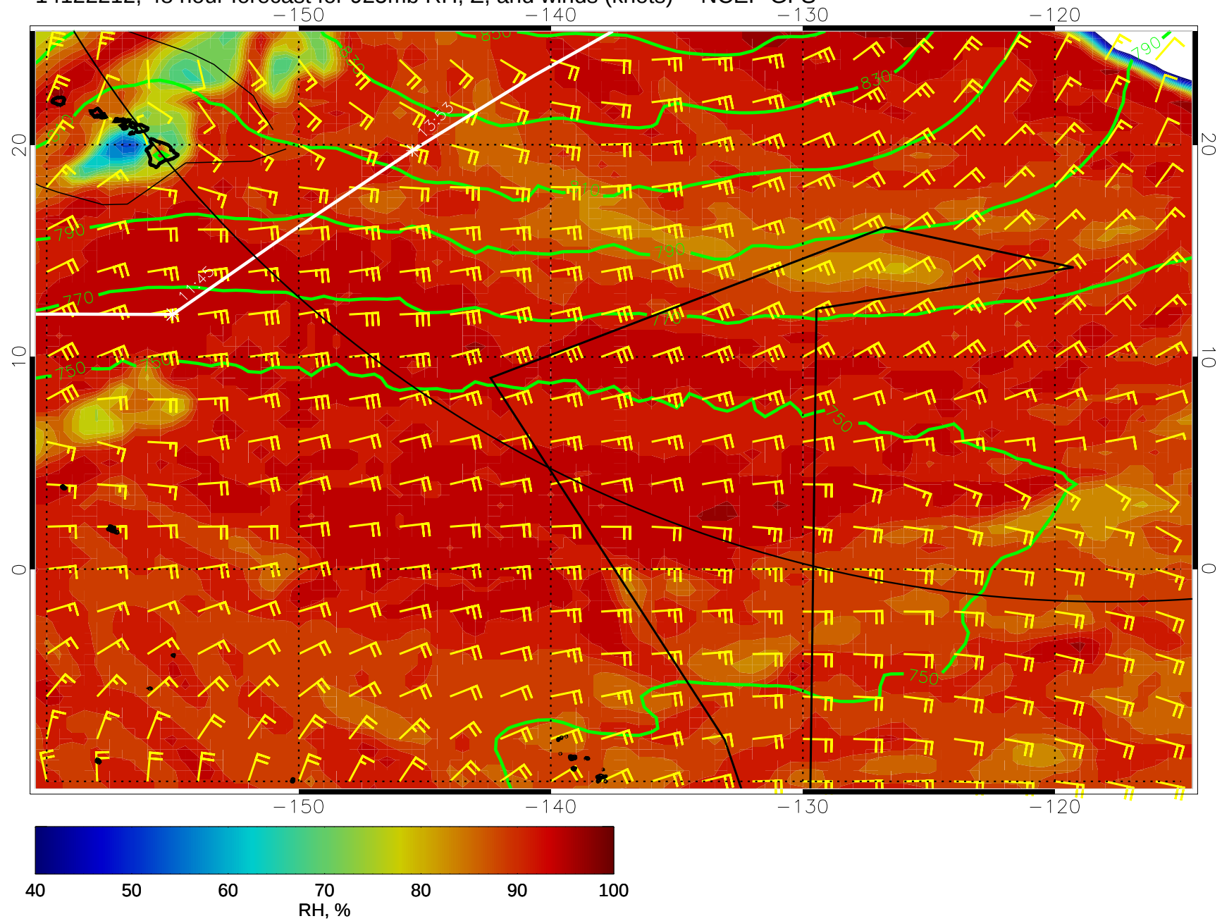
14122212, 48 hour forecast for 925mb RH, Z, and winds (knots) -- NCEP GFS
