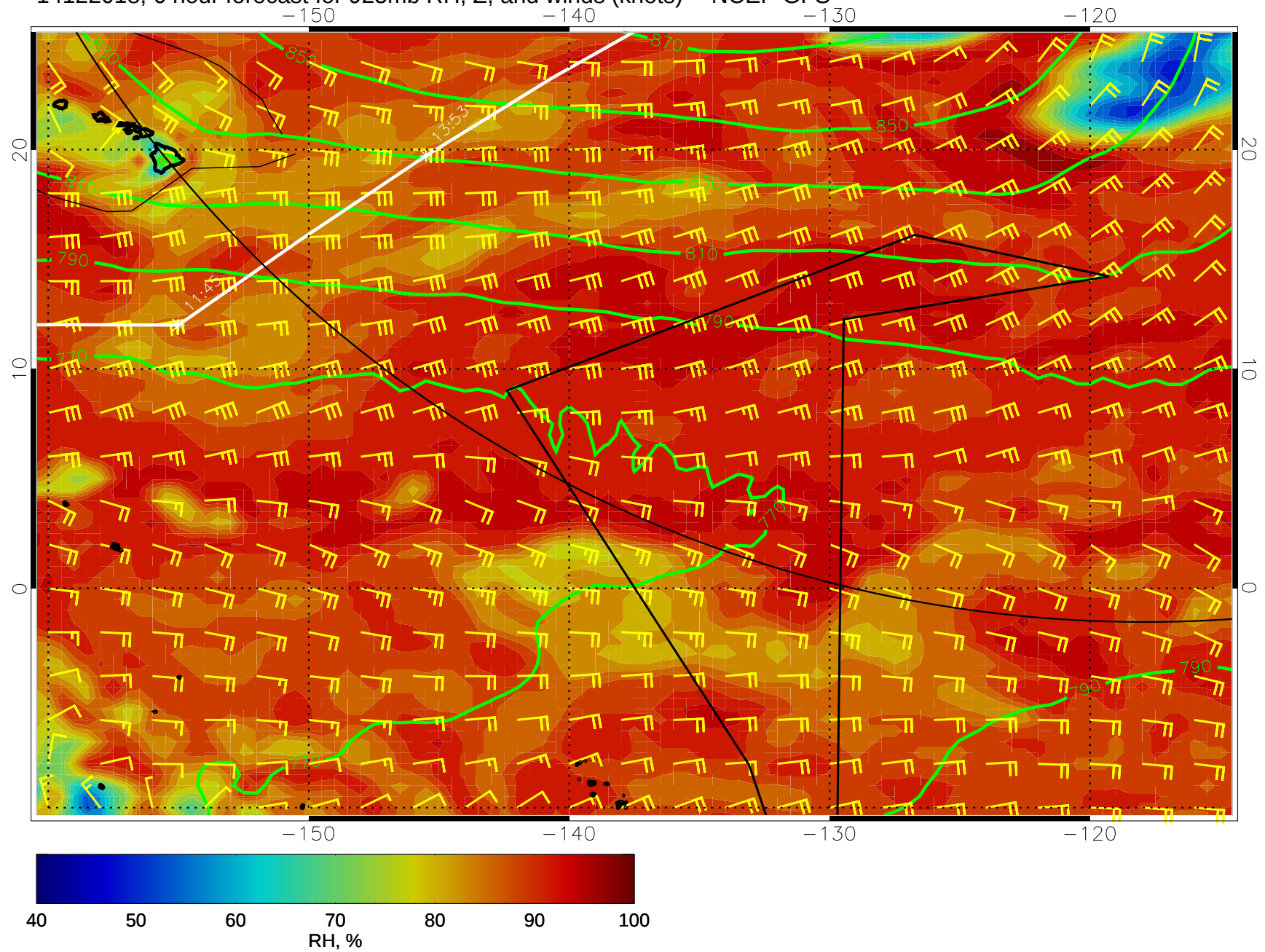
14122018, 6 hour forecast for 925mb RH, Z, and winds (knots) -- NCEP GFS
