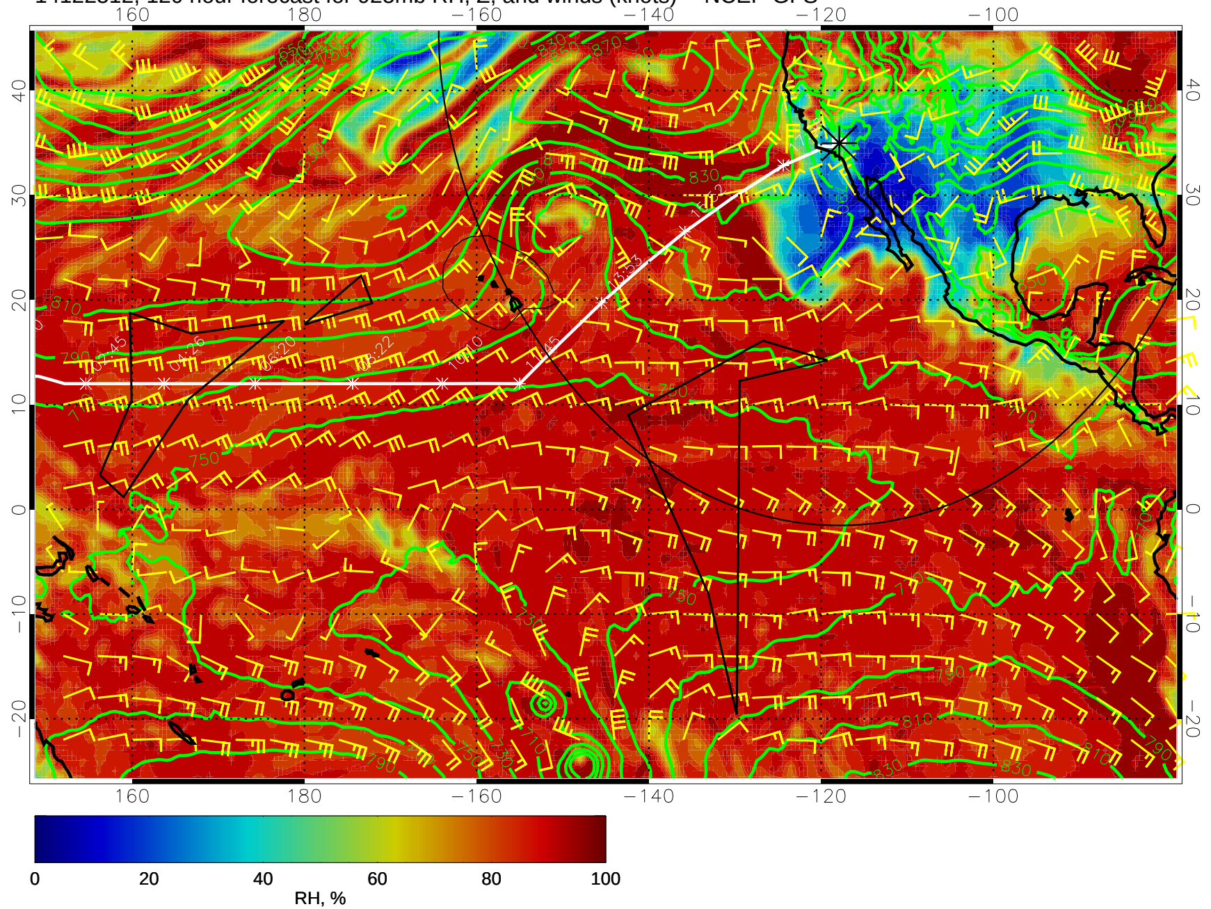
14122512, 120 hour forecast for 925mb RH, Z, and winds (knots) -- NCEP GFS
