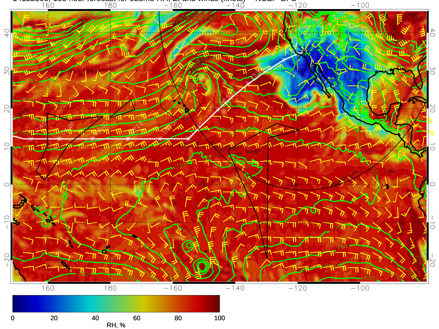
14122500, 108 hour forecast for 925mb RH, Z, and winds (knots) -- NCEP GFS
