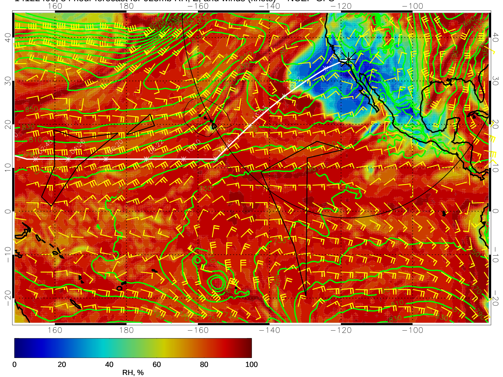
14122400, 84 hour forecast for 925mb RH, Z, and winds (knots) -- NCEP GFS
