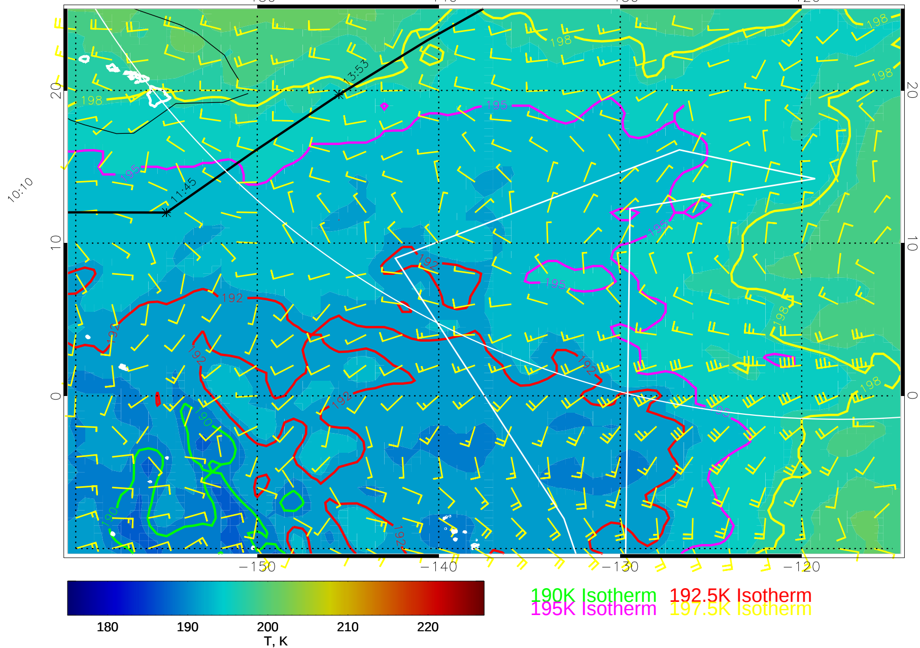
14122506, 114 hour forecast for 70mb T and winds (knots) -- NCEP GFS
