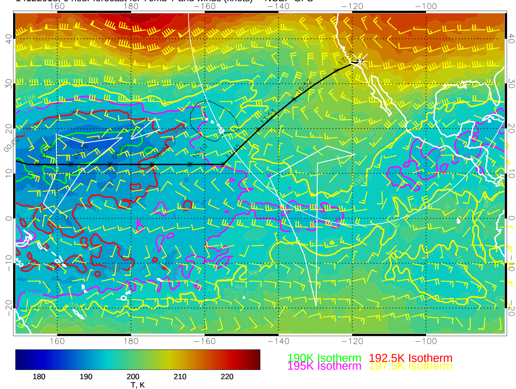
14122018, 6 hour forecast for 70mb T and winds (knots) -- NCEP GFS
