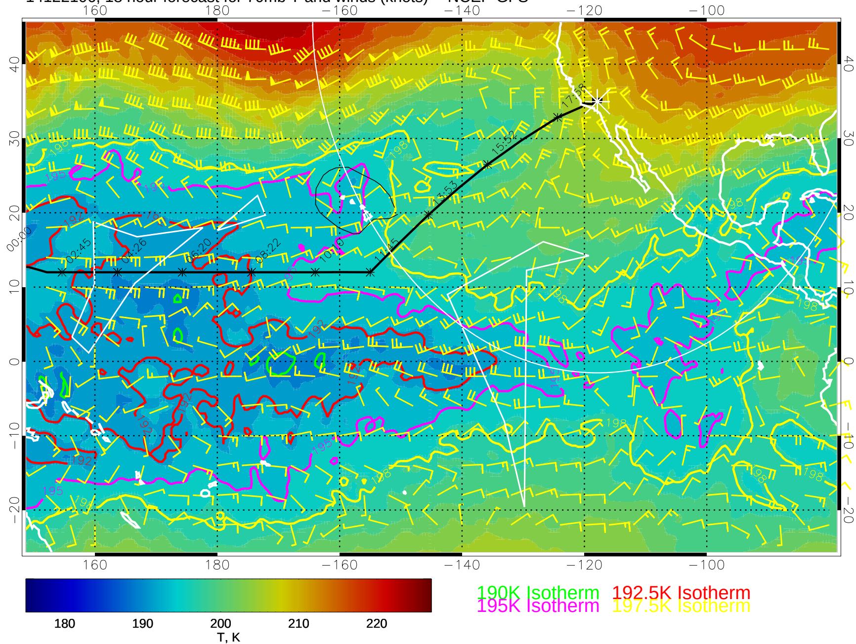
14122106, 18 hour forecast for 70mb T and winds (knots) -- NCEP GFS
