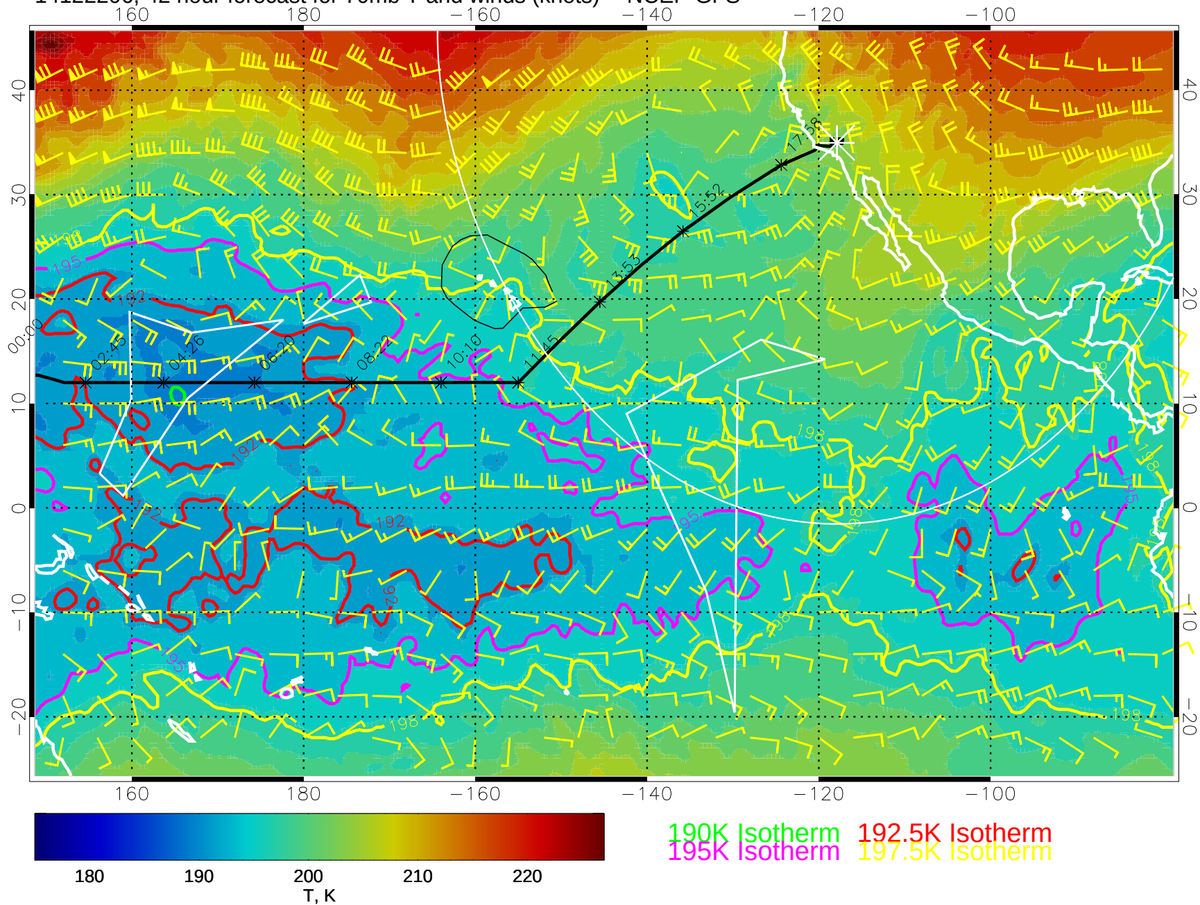
14122206, 42 hour forecast for 70mb T and winds (knots) -- NCEP GFS
