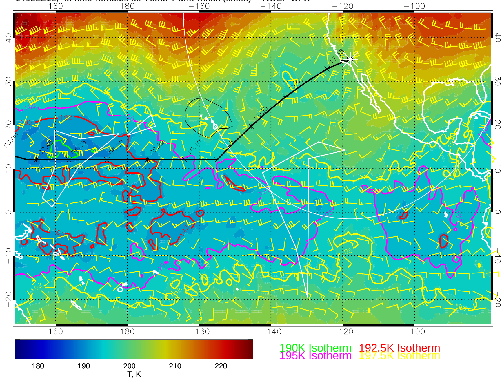
14122212, 48 hour forecast for 70mb T and winds (knots) -- NCEP GFS
