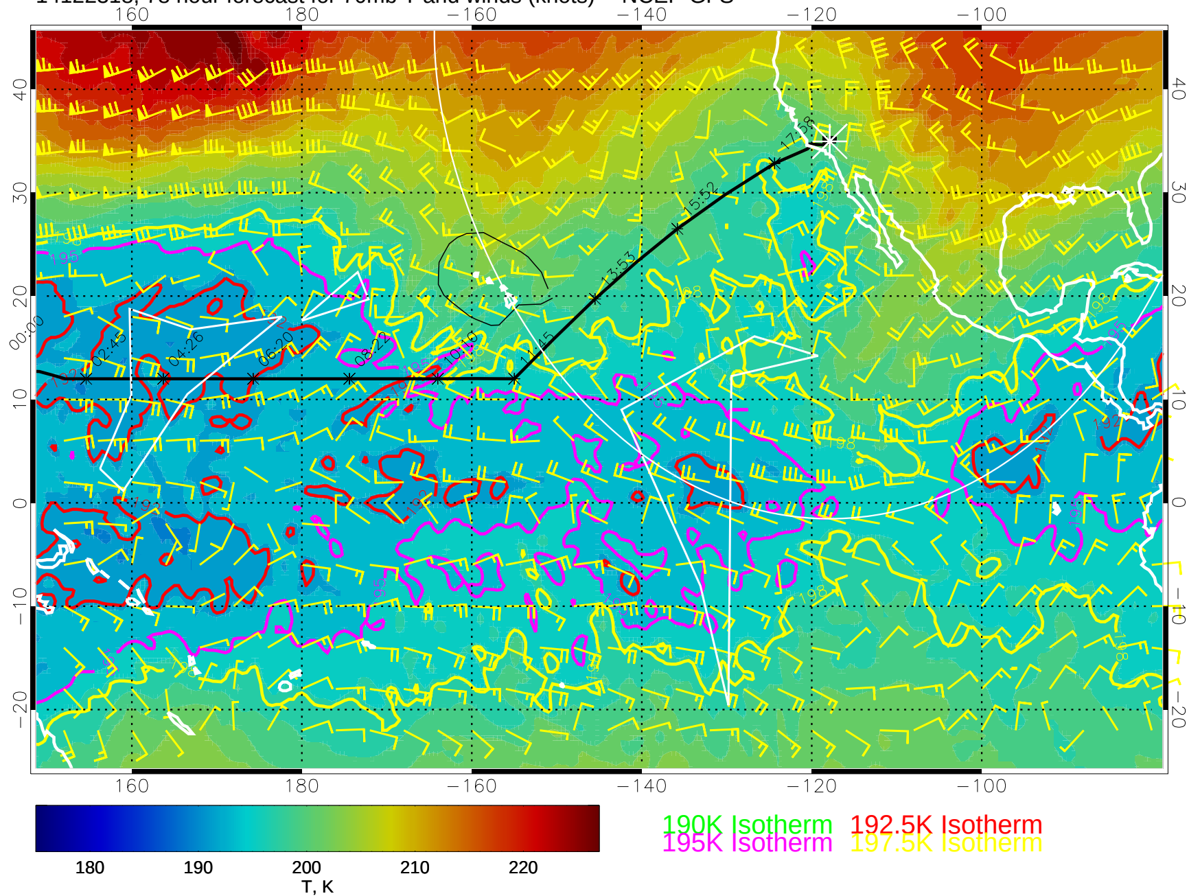
14122318, 78 hour forecast for 70mb T and winds (knots) -- NCEP GFS
