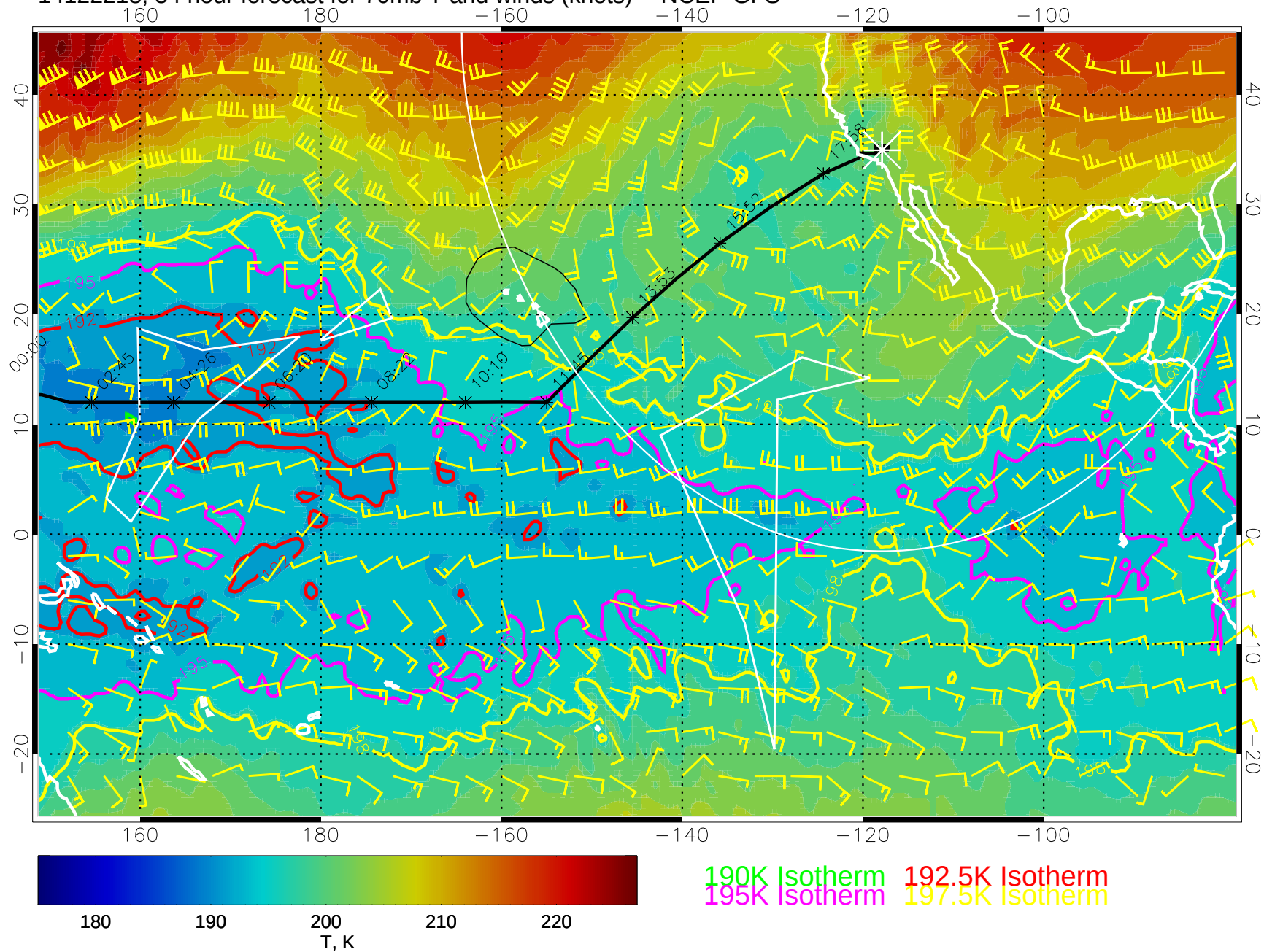
14122218, 54 hour forecast for 70mb T and winds (knots) -- NCEP GFS
