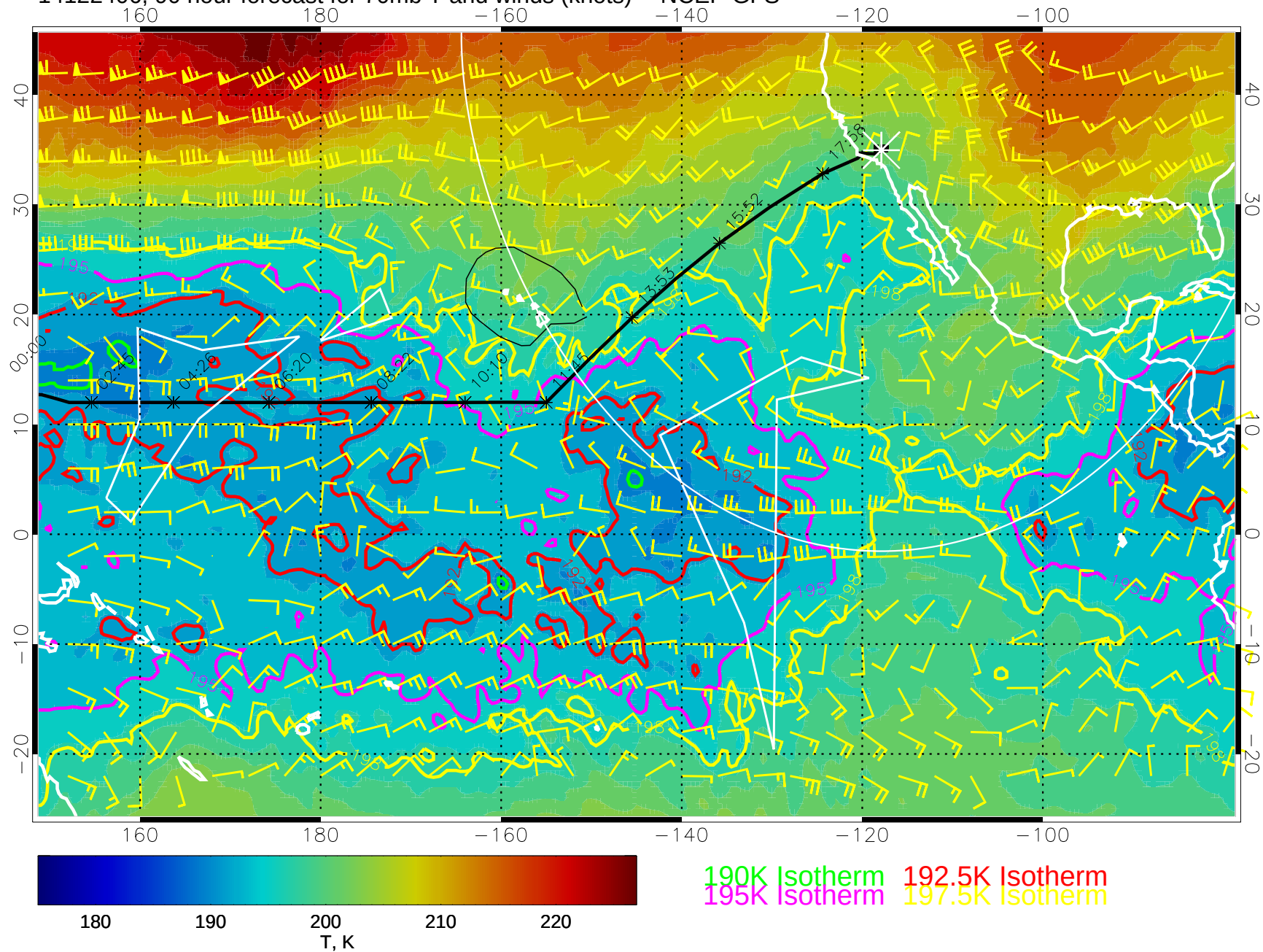
14122406, 90 hour forecast for 70mb T and winds (knots) -- NCEP GFS
