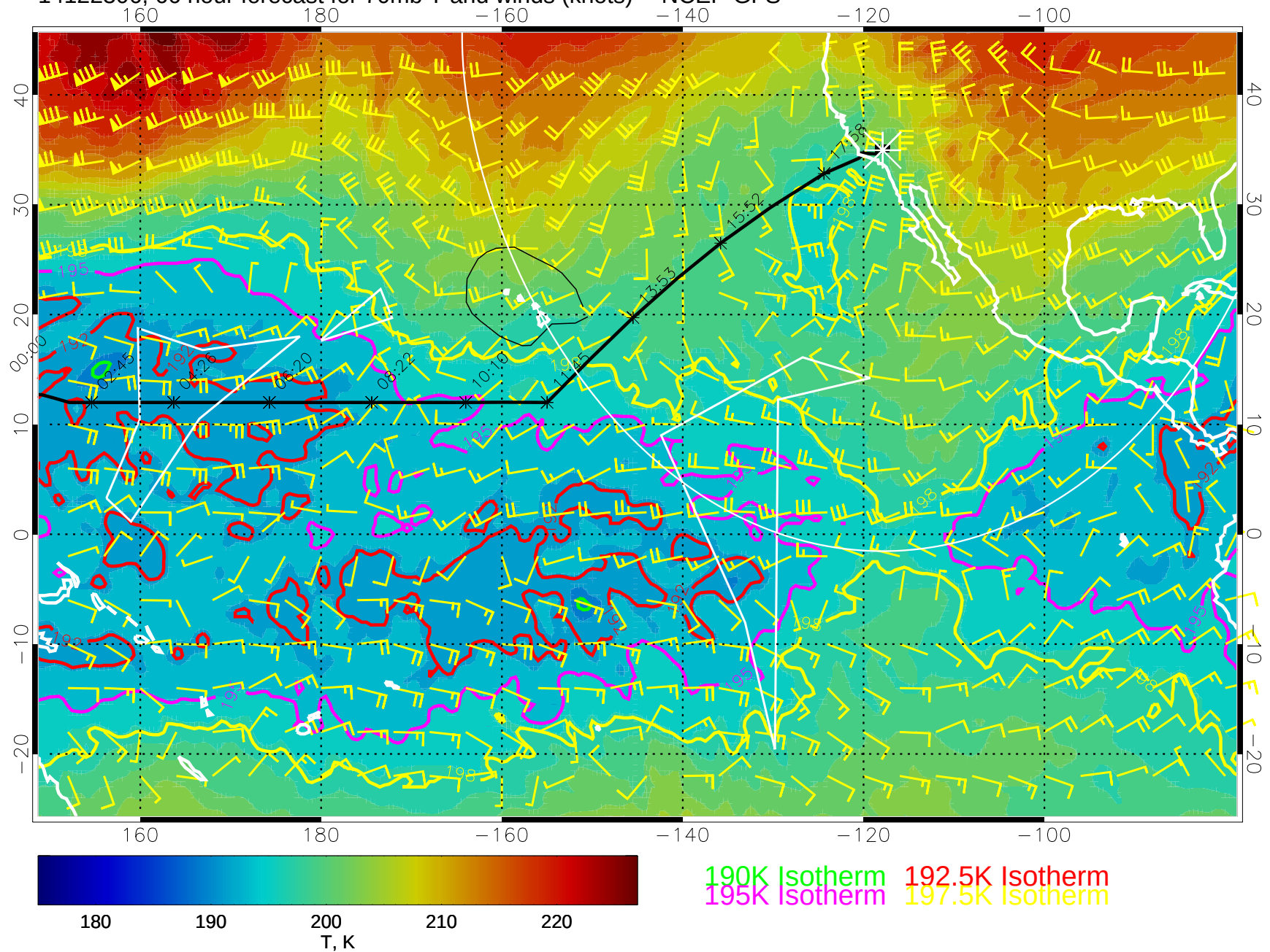
14122306, 66 hour forecast for 70mb T and winds (knots) -- NCEP GFS
