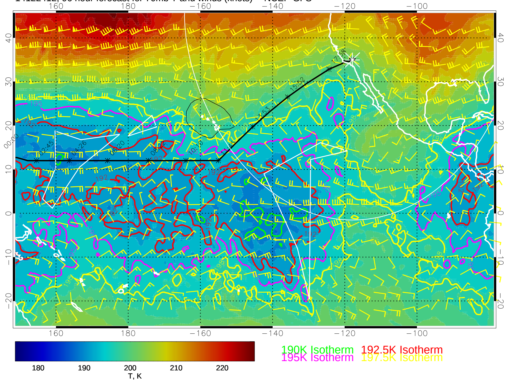
14122412, 96 hour forecast for 70mb T and winds (knots) -- NCEP GFS
