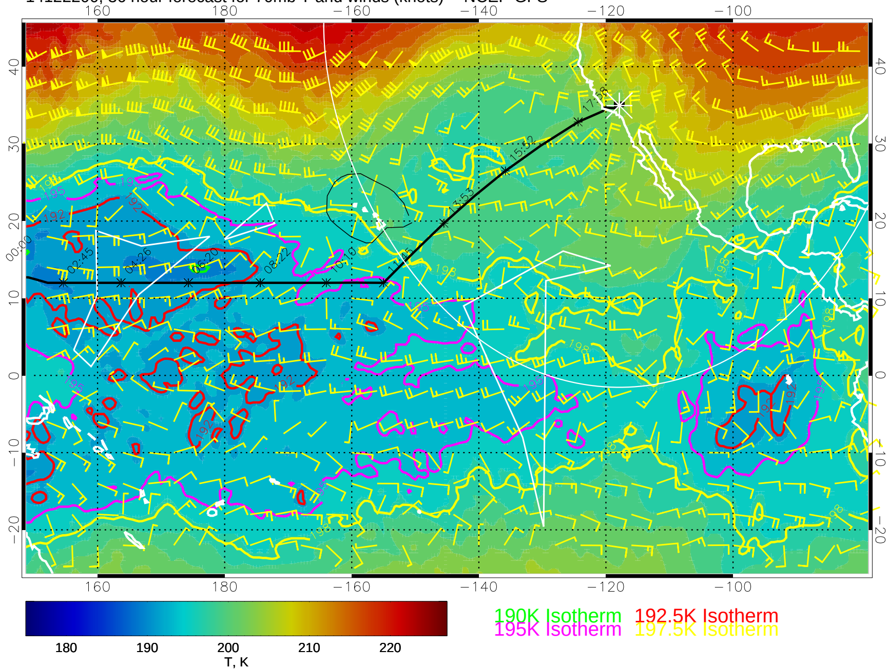
14122200, 36 hour forecast for 70mb T and winds (knots) -- NCEP GFS
