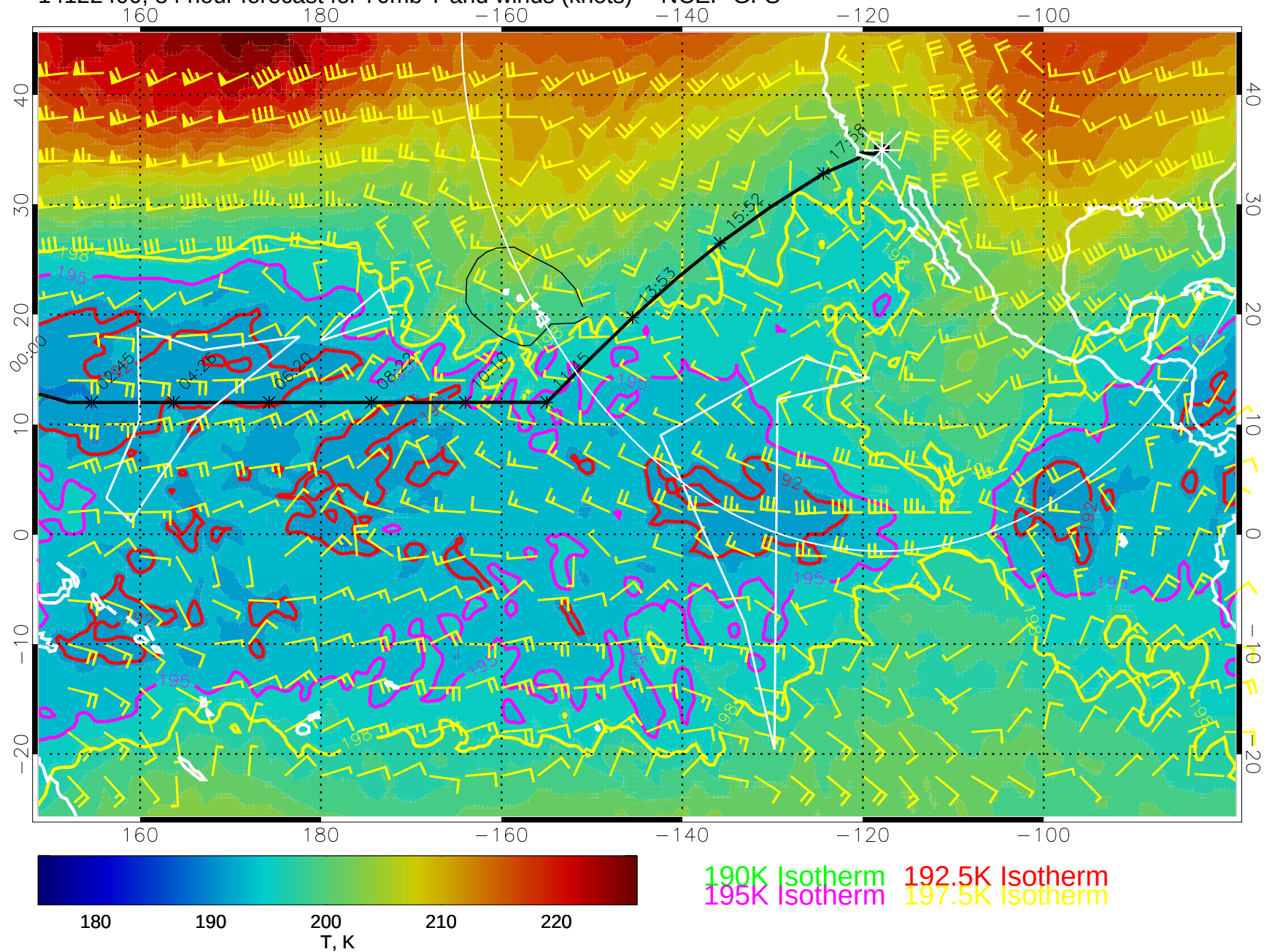
14122400, 84 hour forecast for 70mb T and winds (knots) -- NCEP GFS
