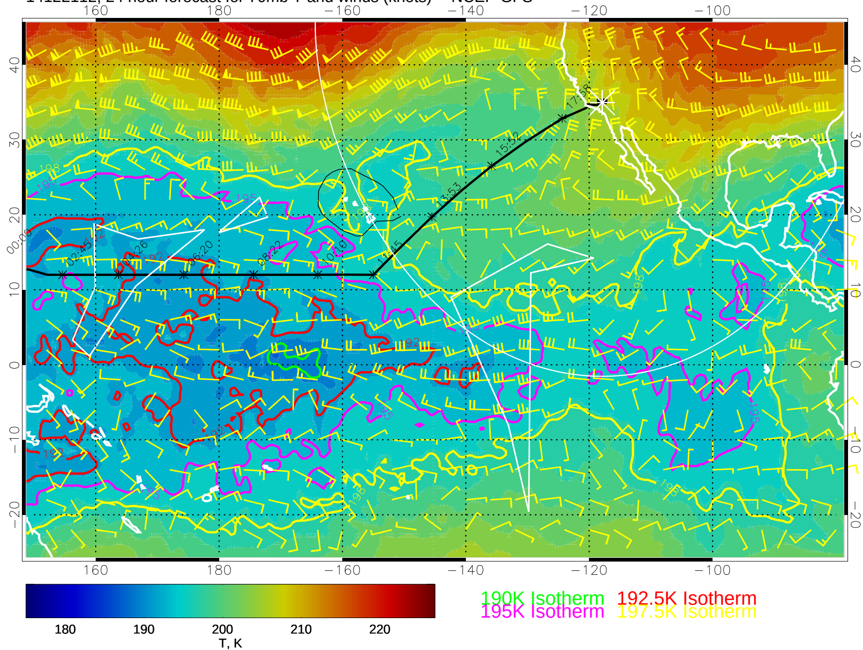
14122112, 24 hour forecast for 70mb T and winds (knots) -- NCEP GFS
