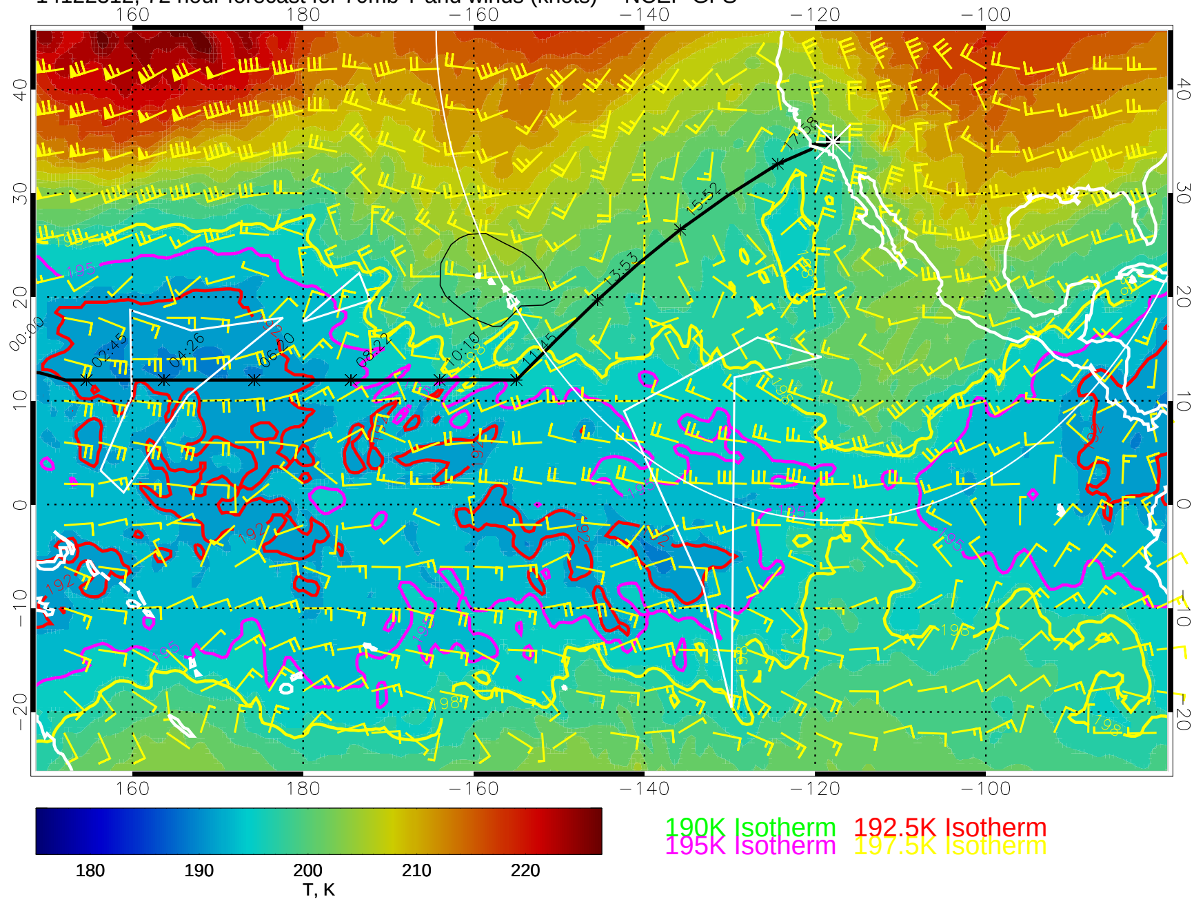
14122312, 72 hour forecast for 70mb T and winds (knots) -- NCEP GFS
