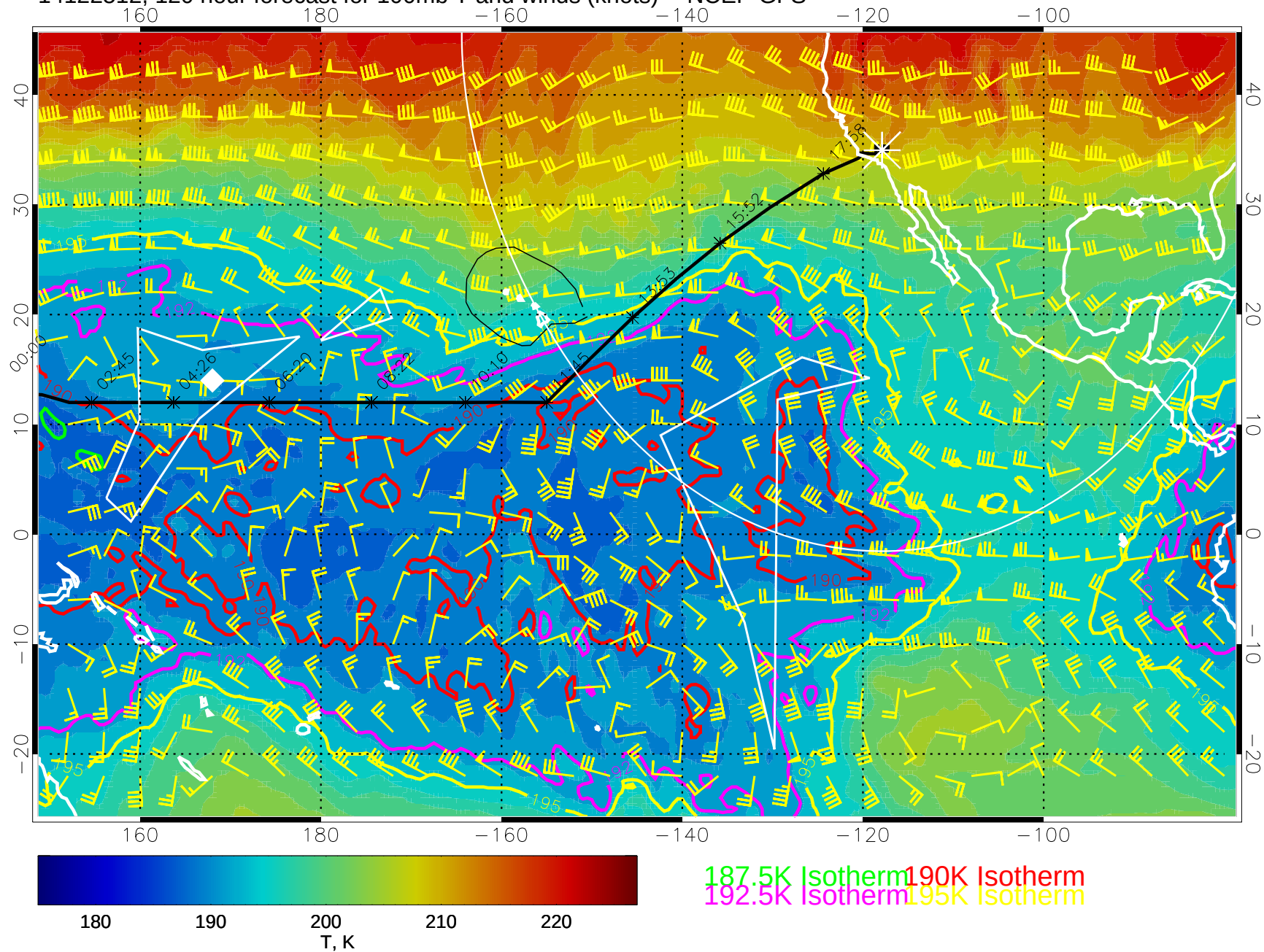
14122512, 120 hour forecast for 100mb T and winds (knots) -- NCEP GFS
