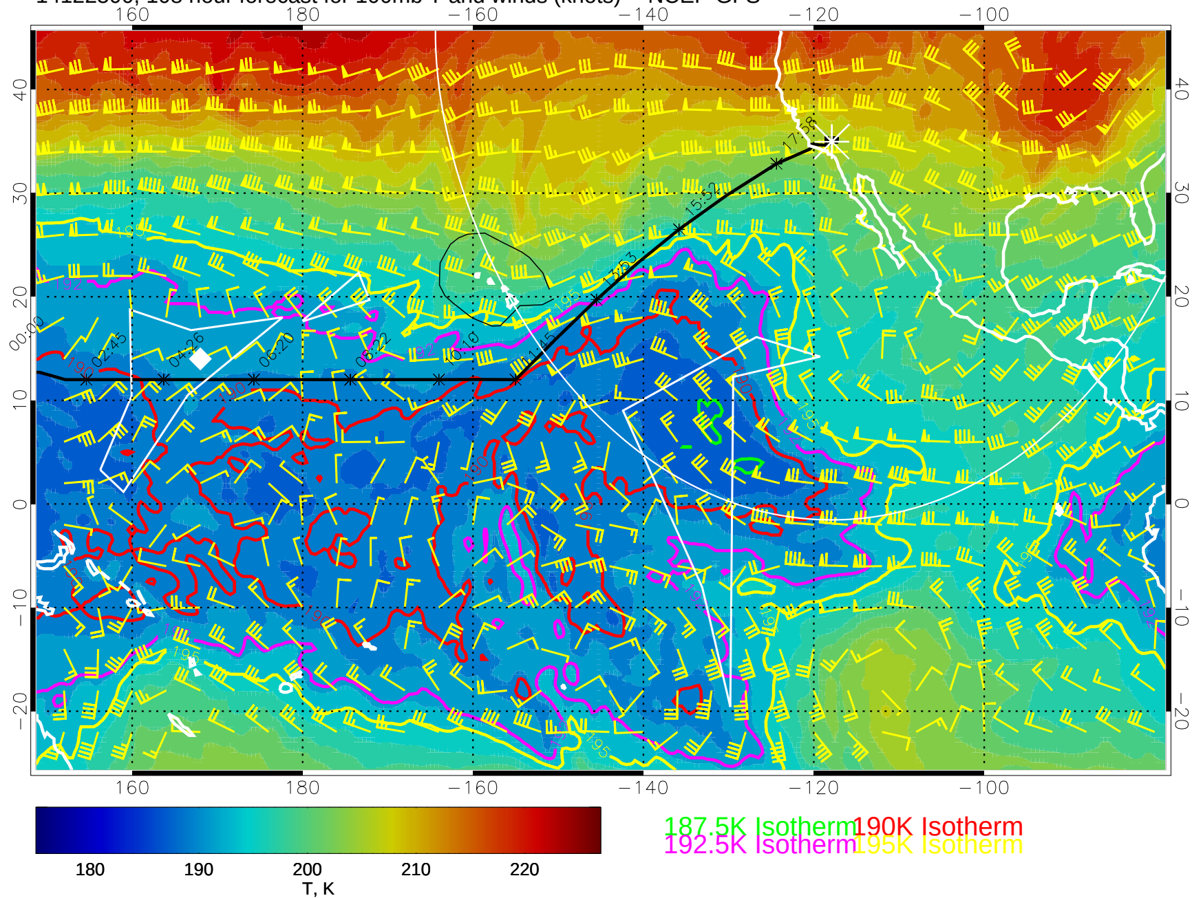
14122500, 108 hour forecast for 100mb T and winds (knots) -- NCEP GFS
