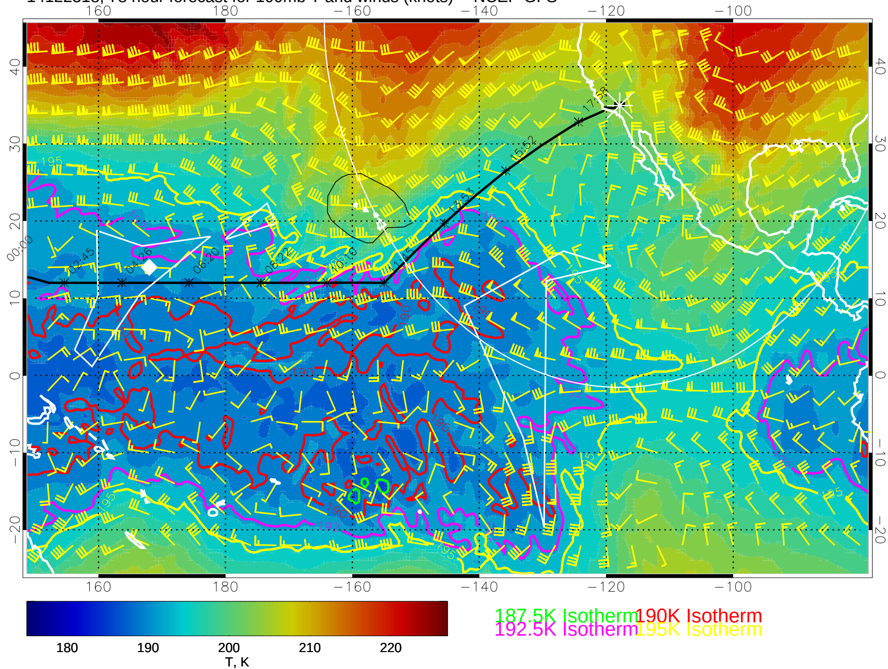
14122318, 78 hour forecast for 100mb T and winds (knots) -- NCEP GFS
