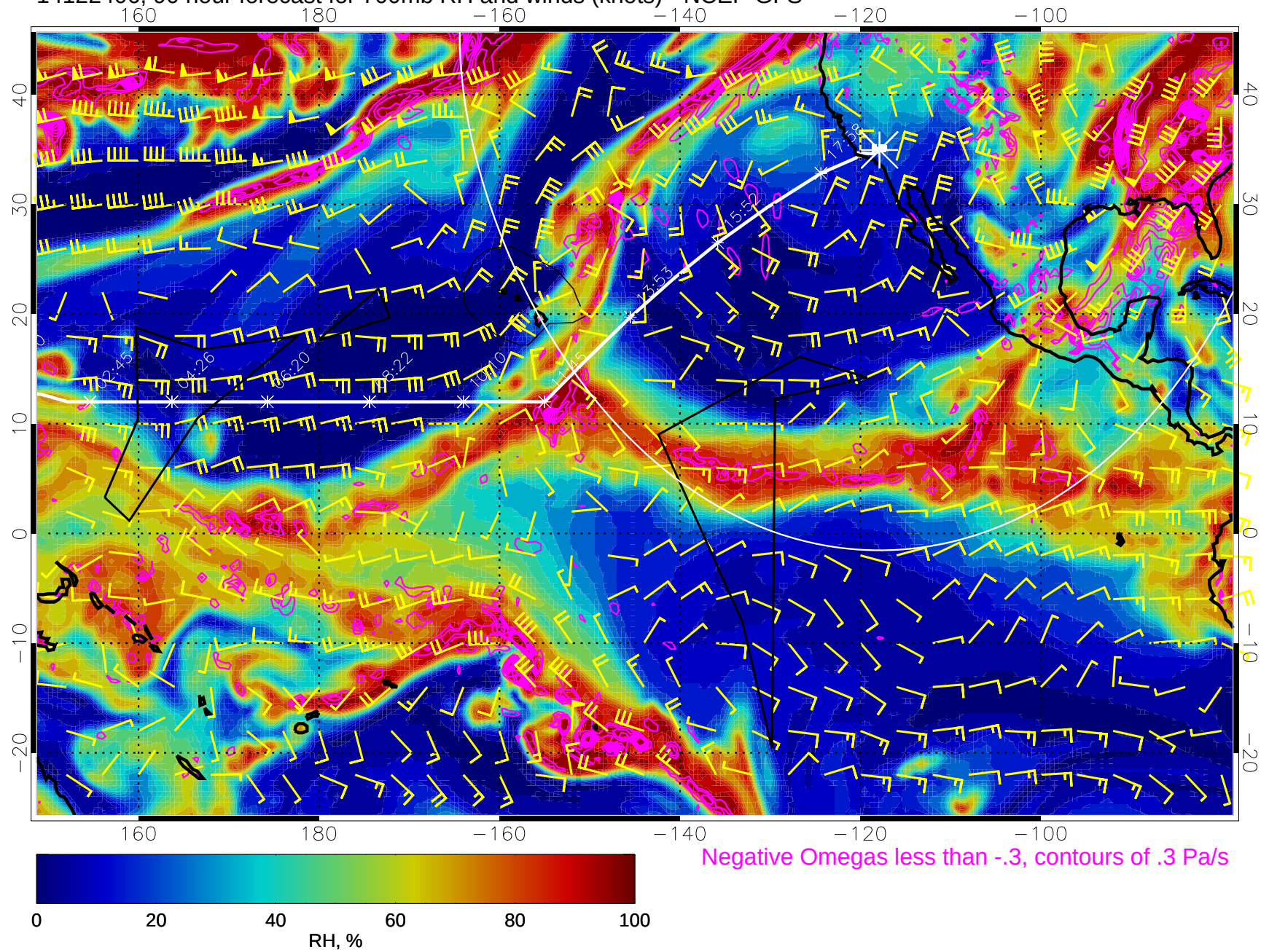
14122406, 90 hour forecast for 700mb RH and winds (knots) - NCEP GFS
