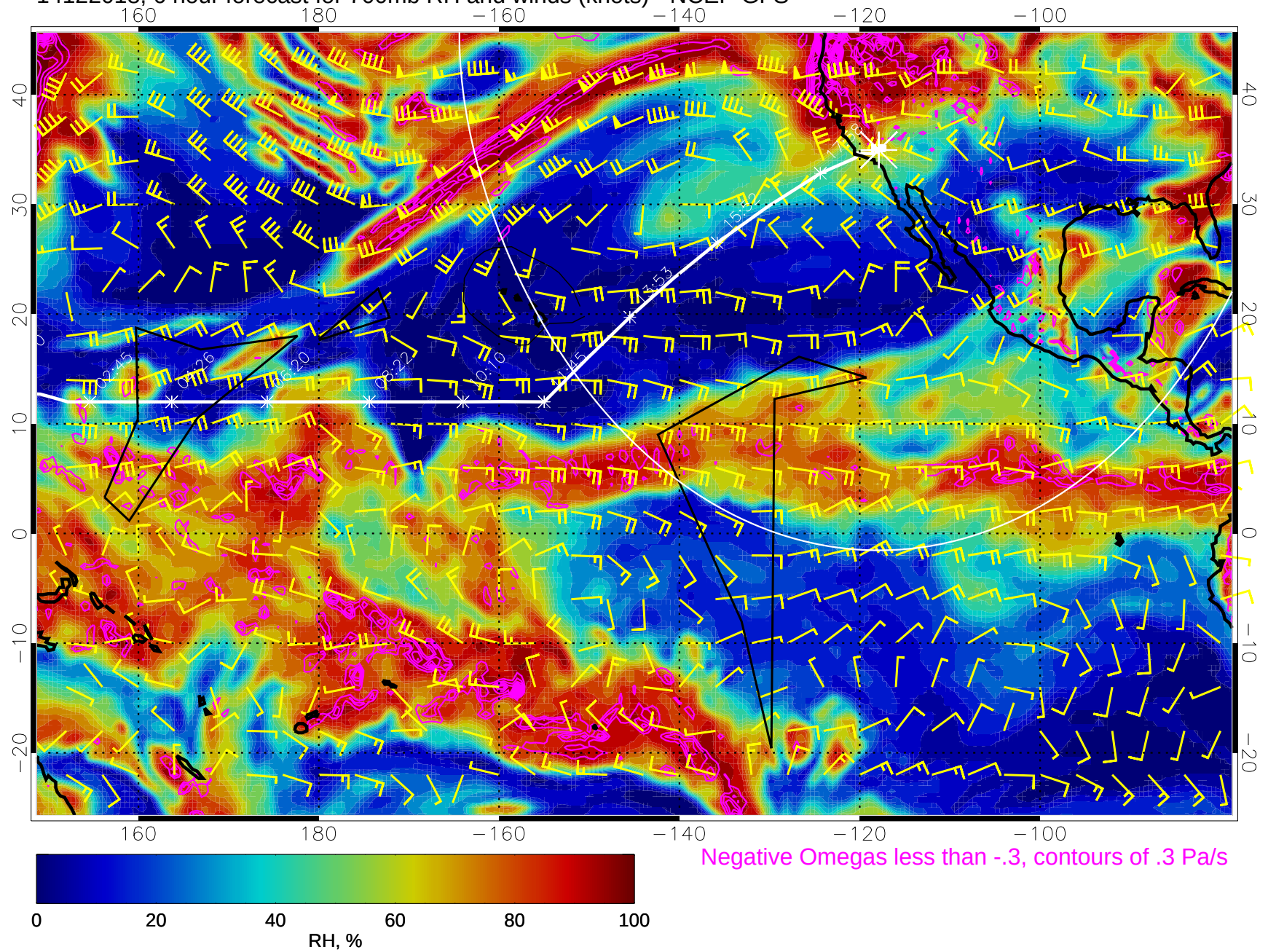
14122018, 6 hour forecast for 700mb RH and winds (knots) - NCEP GFS
