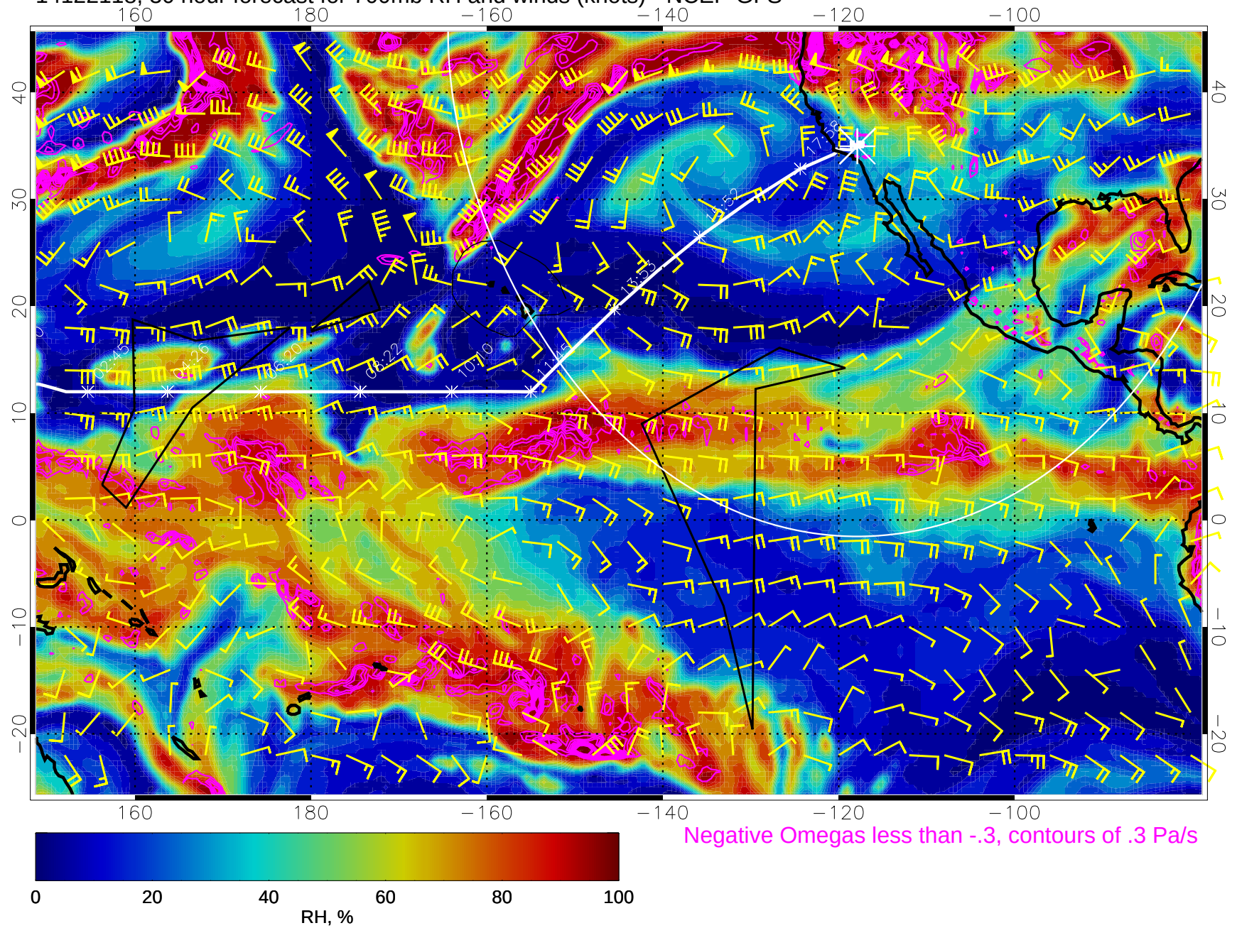
14122118, 30 hour forecast for 700mb RH and winds (knots) - NCEP GFS
