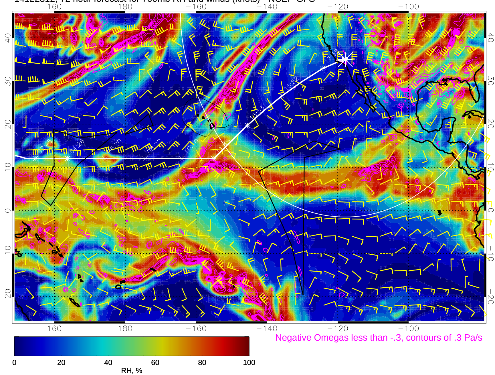
14122312, 72 hour forecast for 700mb RH and winds (knots) - NCEP GFS
