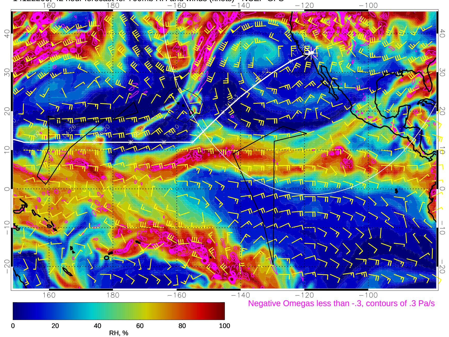
14122206, 42 hour forecast for 700mb RH and winds (knots) - NCEP GFS
