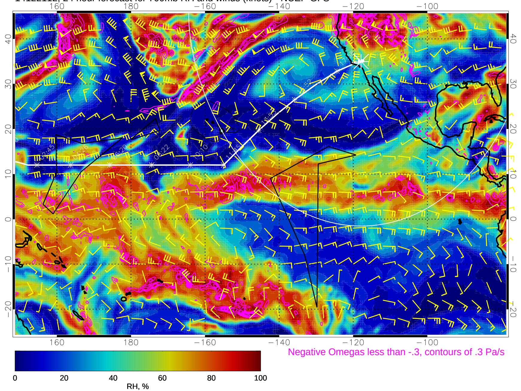
14122112, 24 hour forecast for 700mb RH and winds (knots) - NCEP GFS
