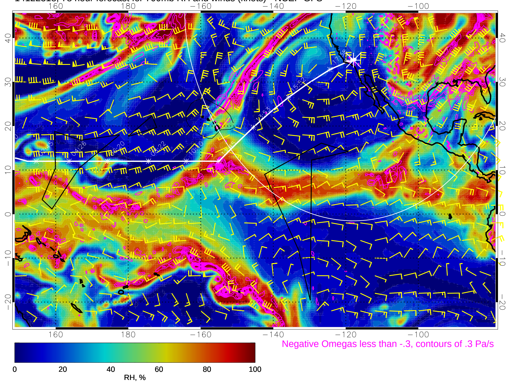
14122318, 78 hour forecast for 700mb RH and winds (knots) - NCEP GFS
