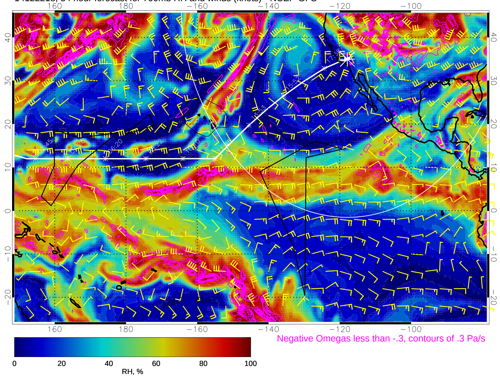
14122218, 54 hour forecast for 700mb RH and winds (knots) - NCEP GFS
