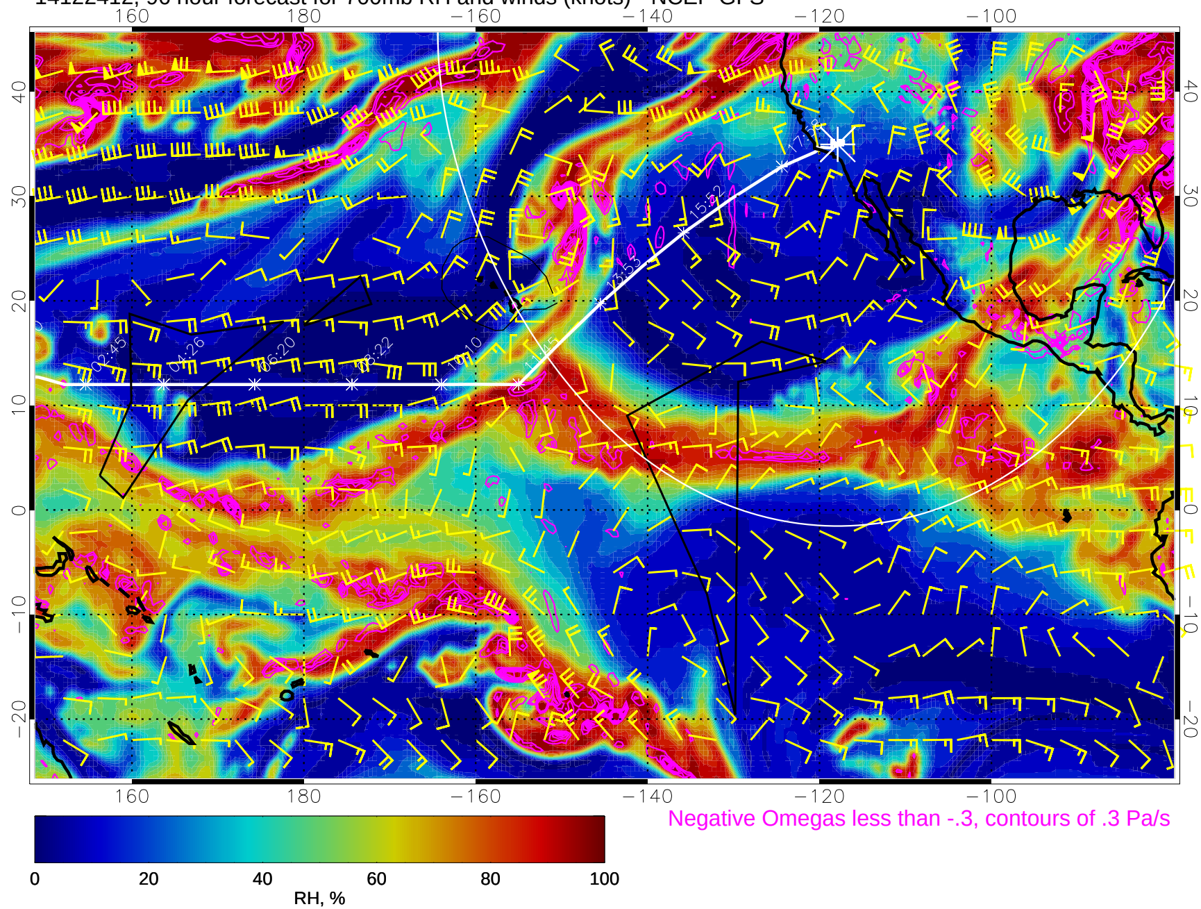
14122412, 96 hour forecast for 700mb RH and winds (knots) - NCEP GFS
