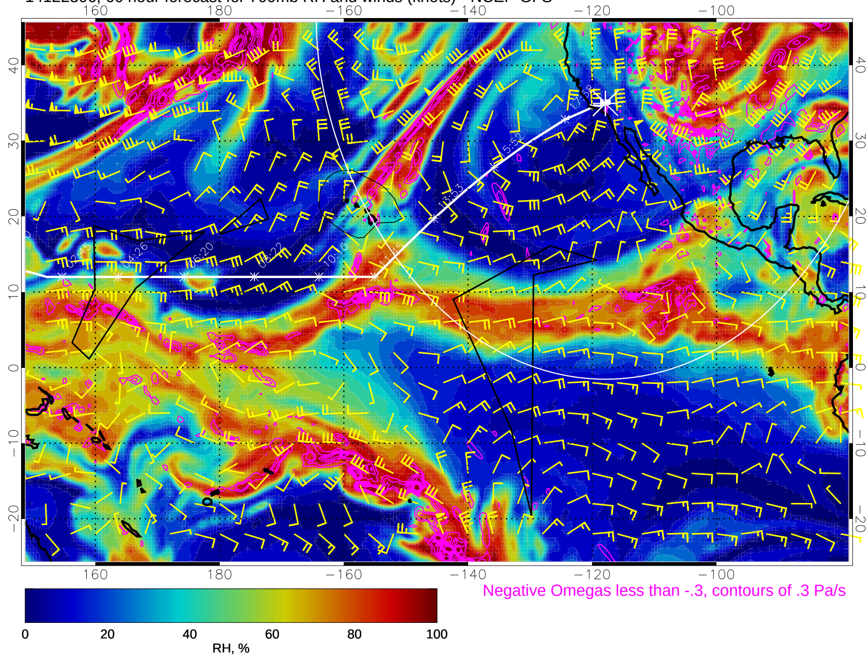
14122306, 66 hour forecast for 700mb RH and winds (knots) - NCEP GFS
