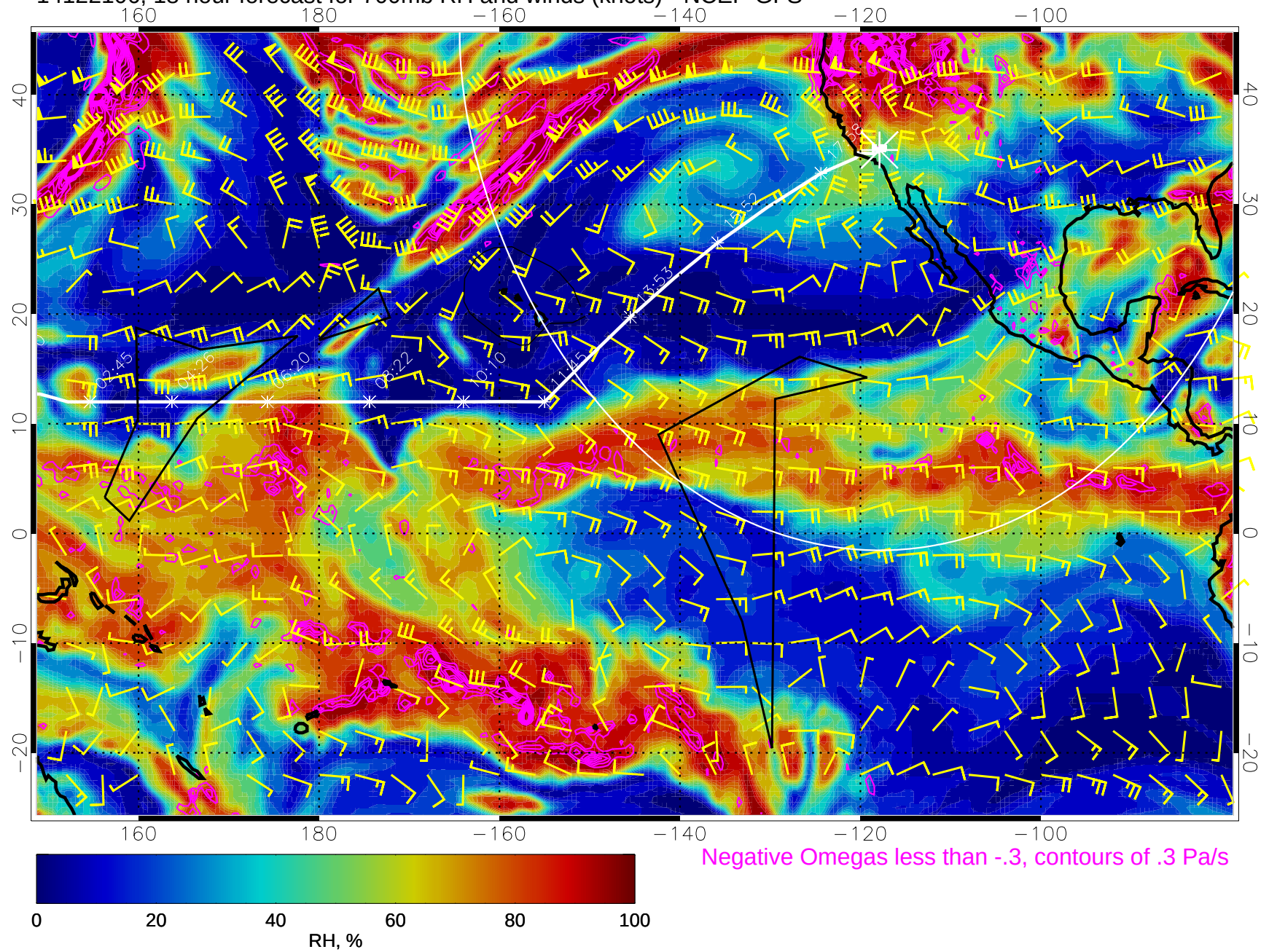
14122106, 18 hour forecast for 700mb RH and winds (knots) - NCEP GFS
