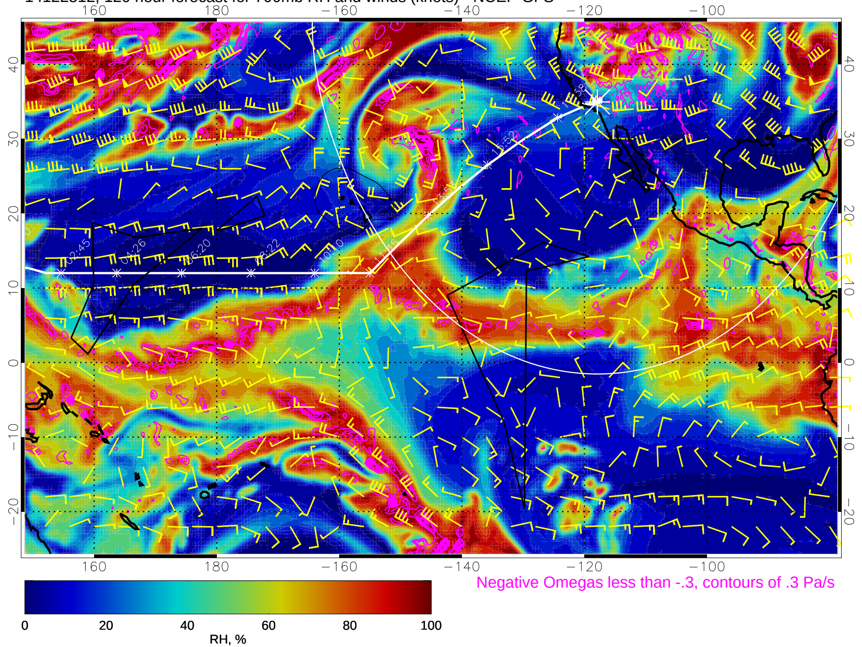
14122512, 120 hour forecast for 700mb RH and winds (knots) - NCEP GFS
