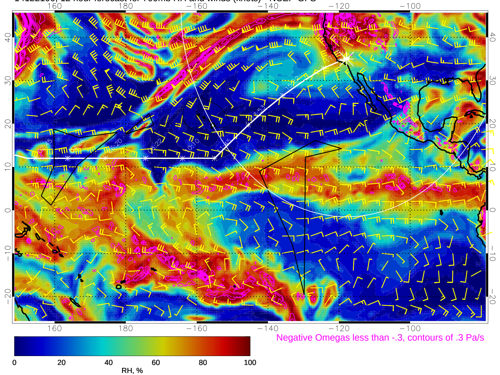
14122100, 12 hour forecast for 700mb RH and winds (knots) - NCEP GFS
