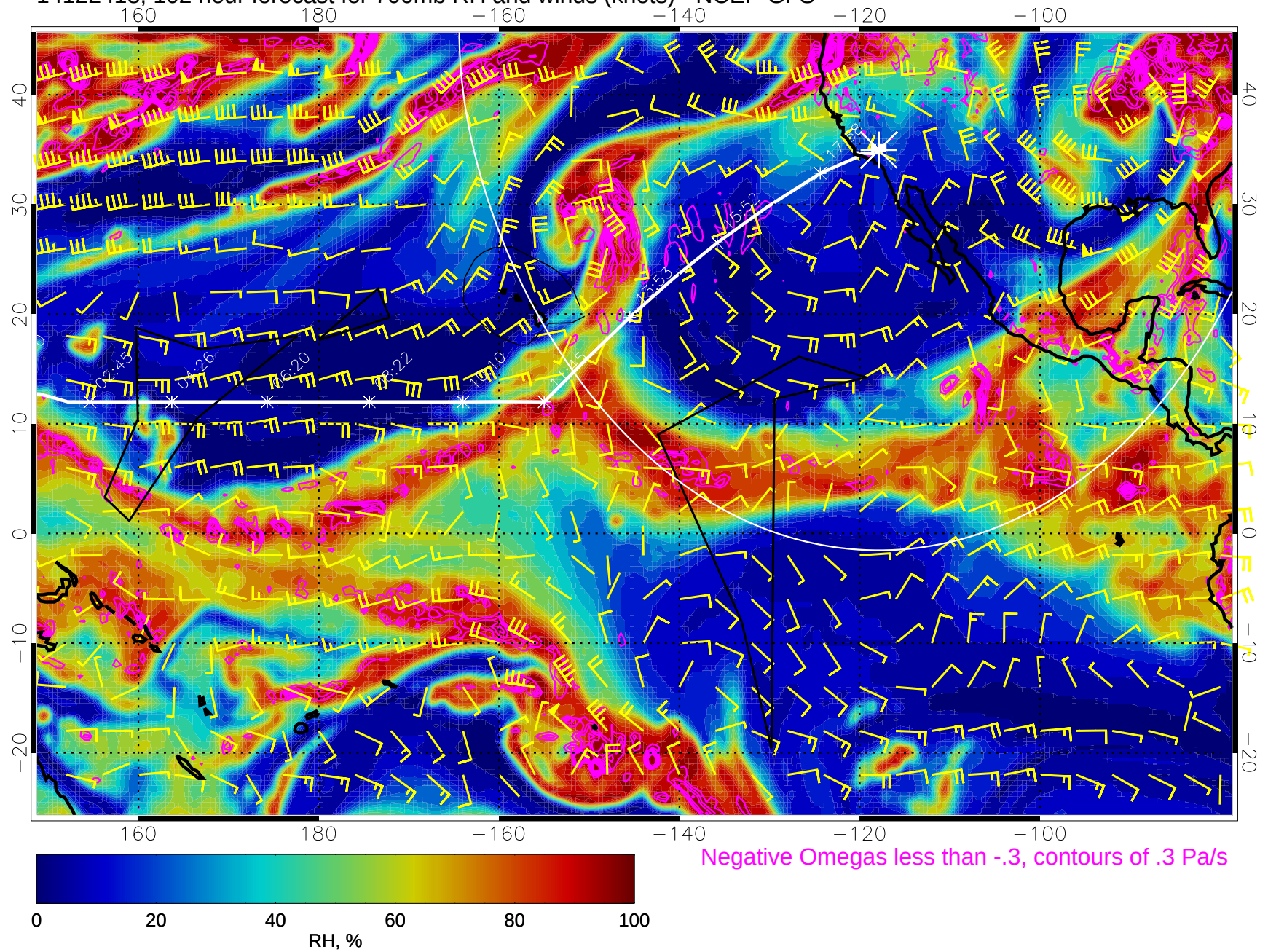
14122418, 102 hour forecast for 700mb RH and winds (knots) - NCEP GFS
