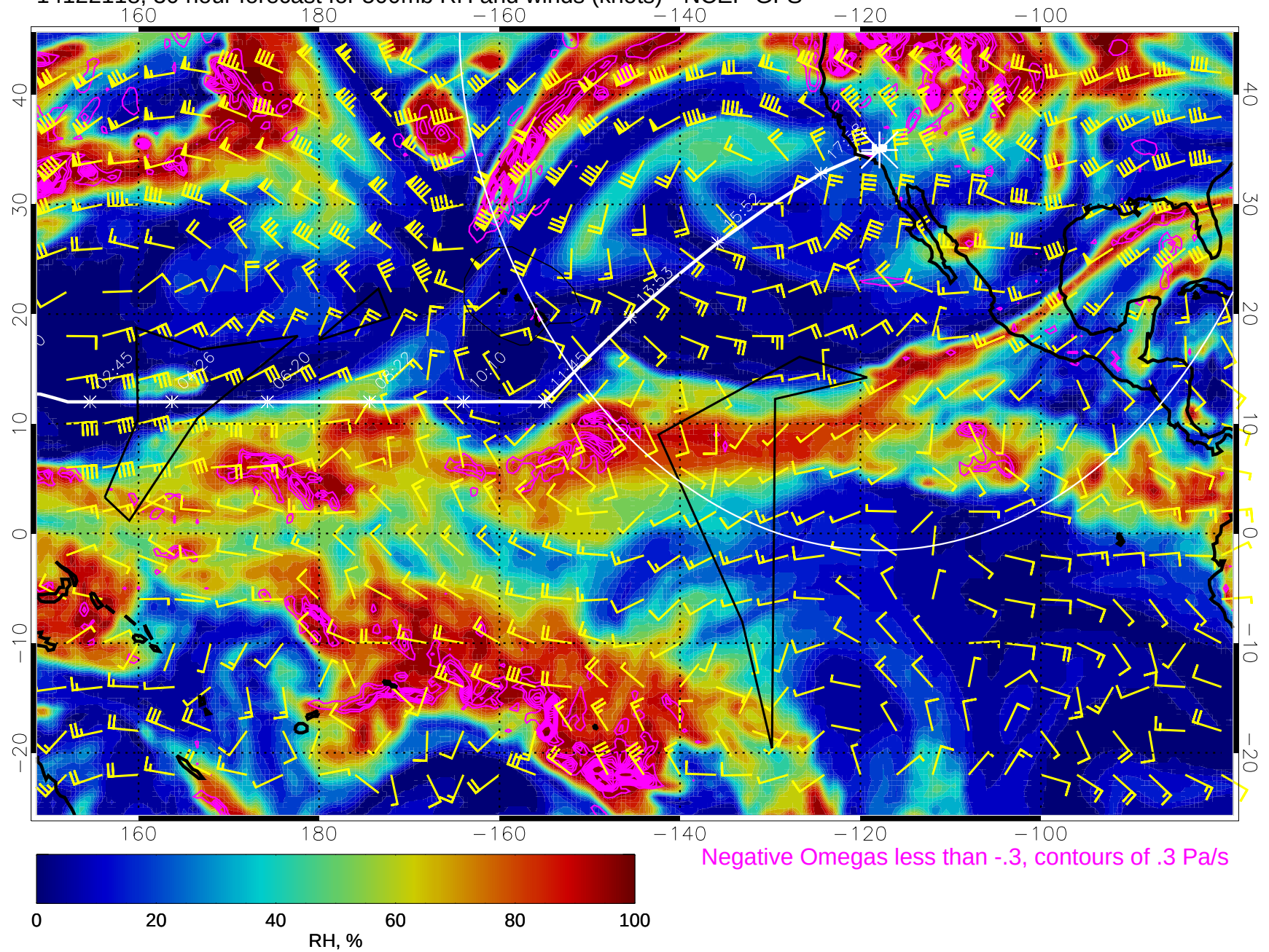
14122118, 30 hour forecast for 500mb RH and winds (knots) - NCEP GFS
