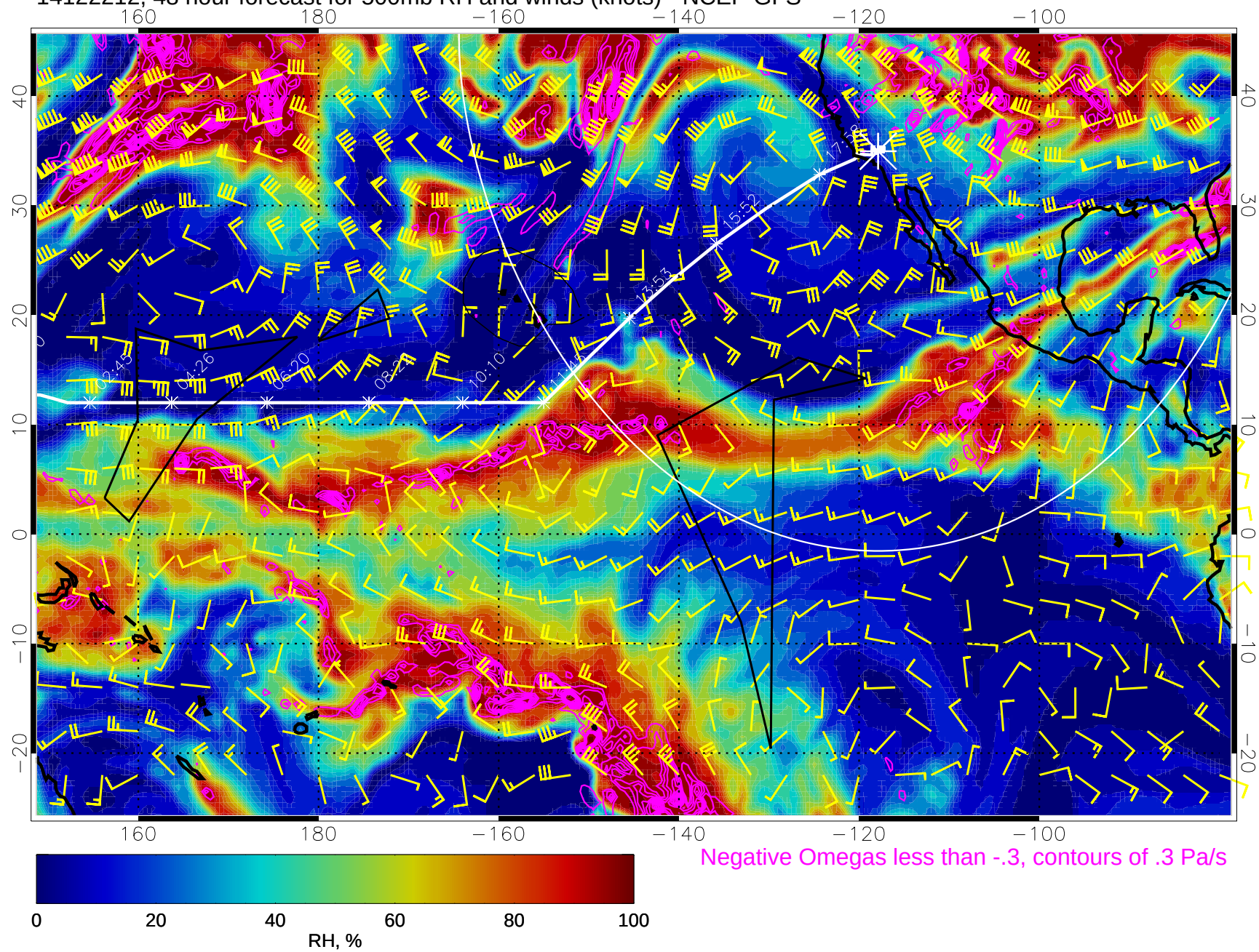
14122212, 48 hour forecast for 500mb RH and winds (knots) - NCEP GFS
