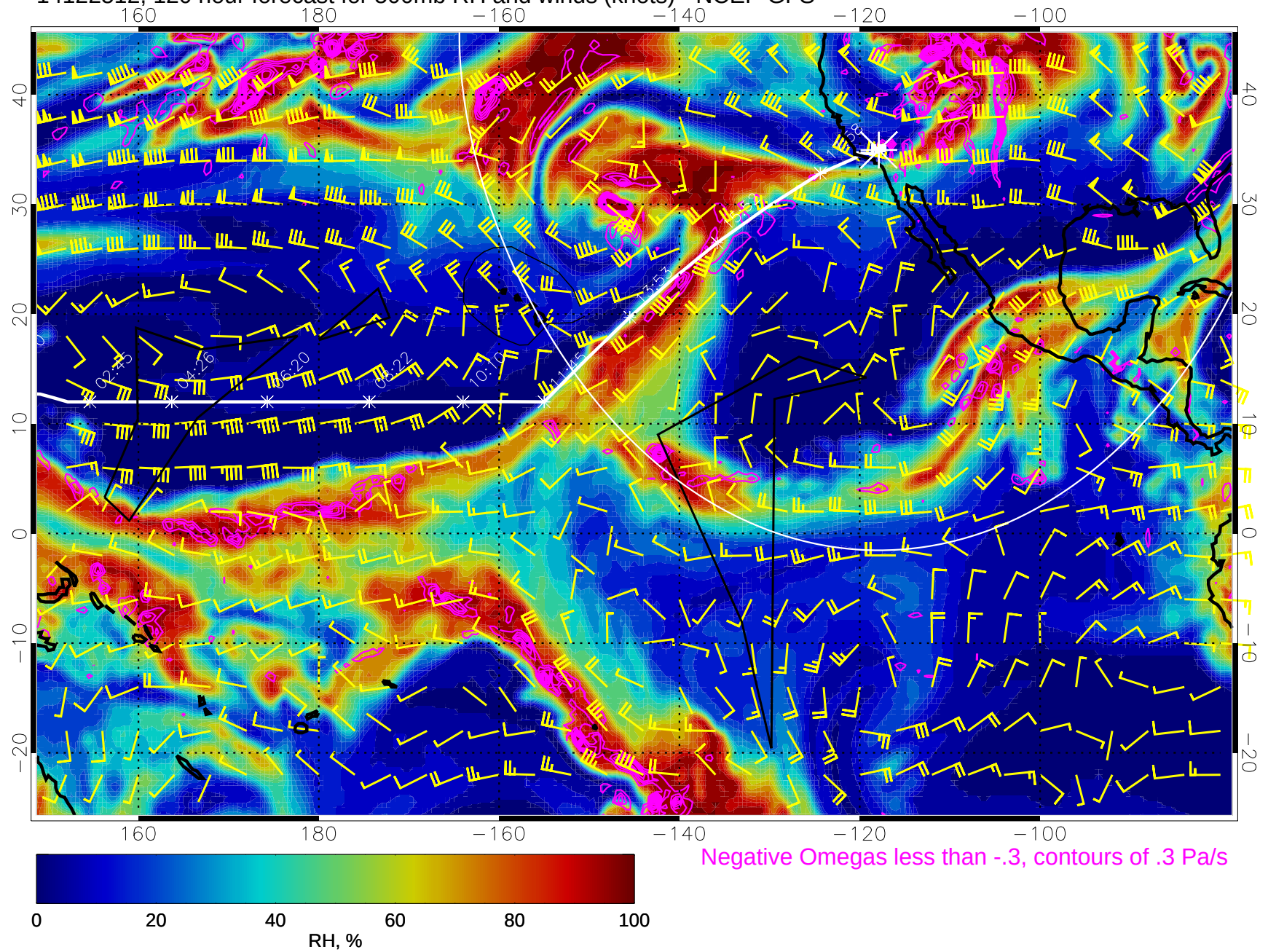
14122512, 120 hour forecast for 500mb RH and winds (knots) - NCEP GFS
