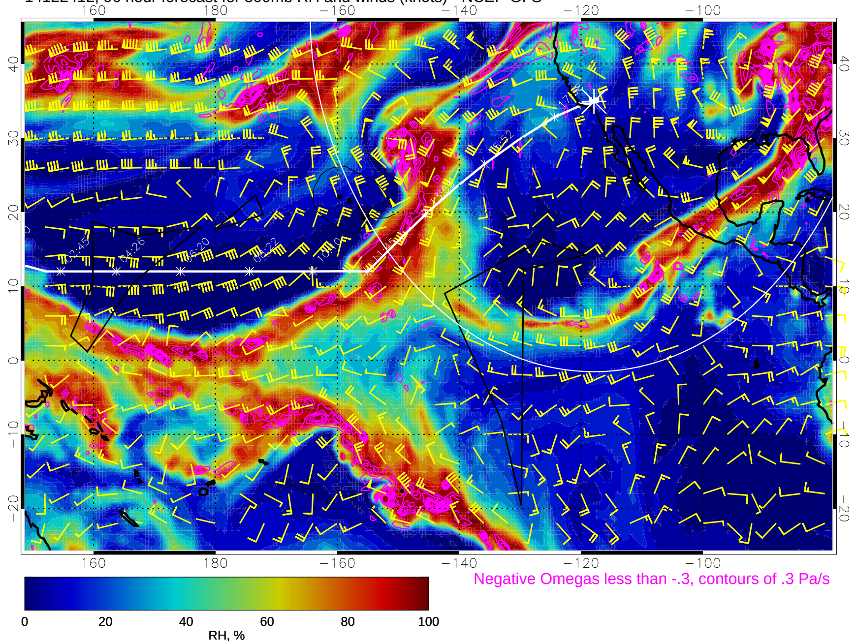
14122412, 96 hour forecast for 500mb RH and winds (knots) - NCEP GFS
