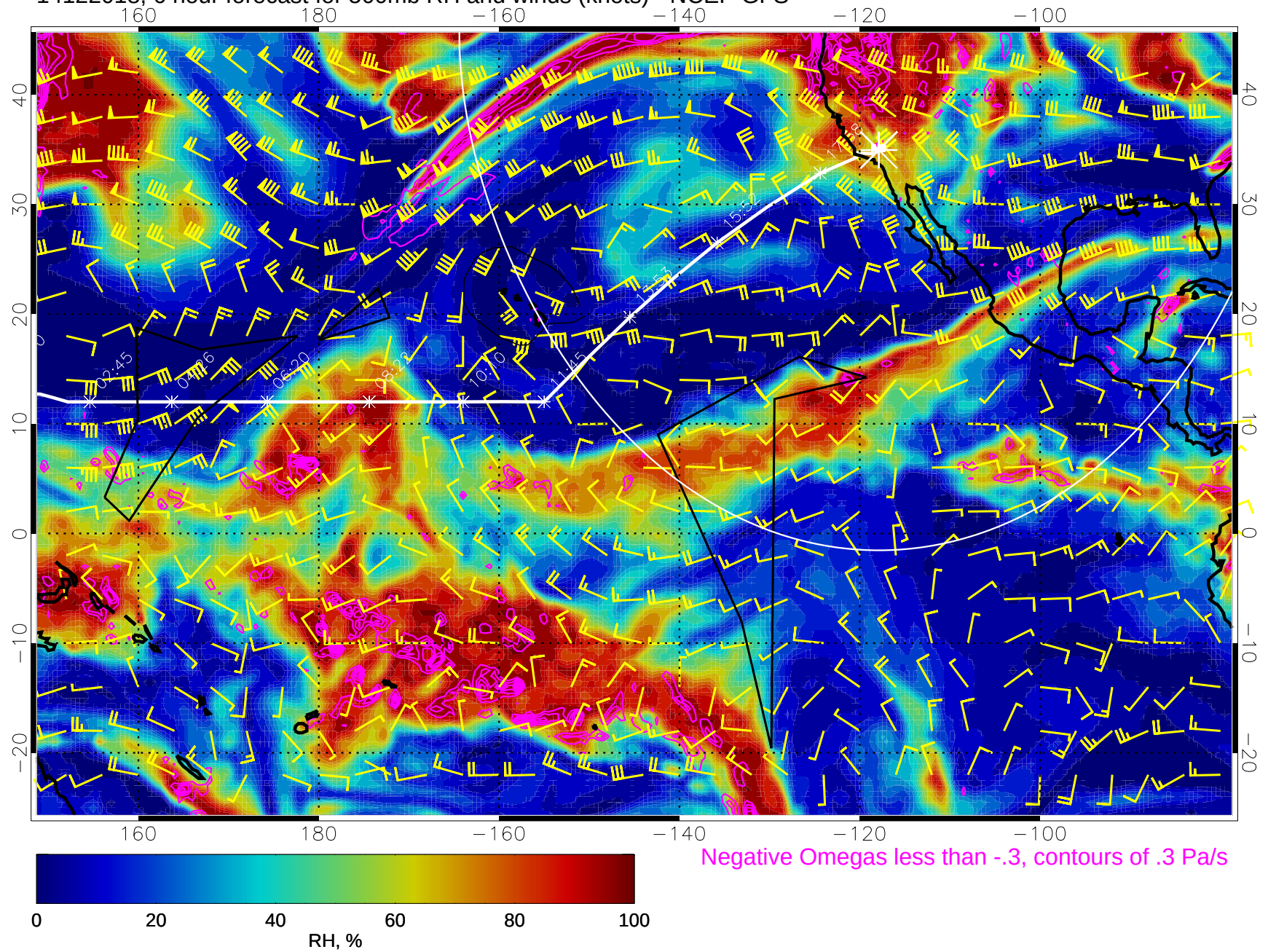
14122018, 6 hour forecast for 500mb RH and winds (knots) - NCEP GFS
