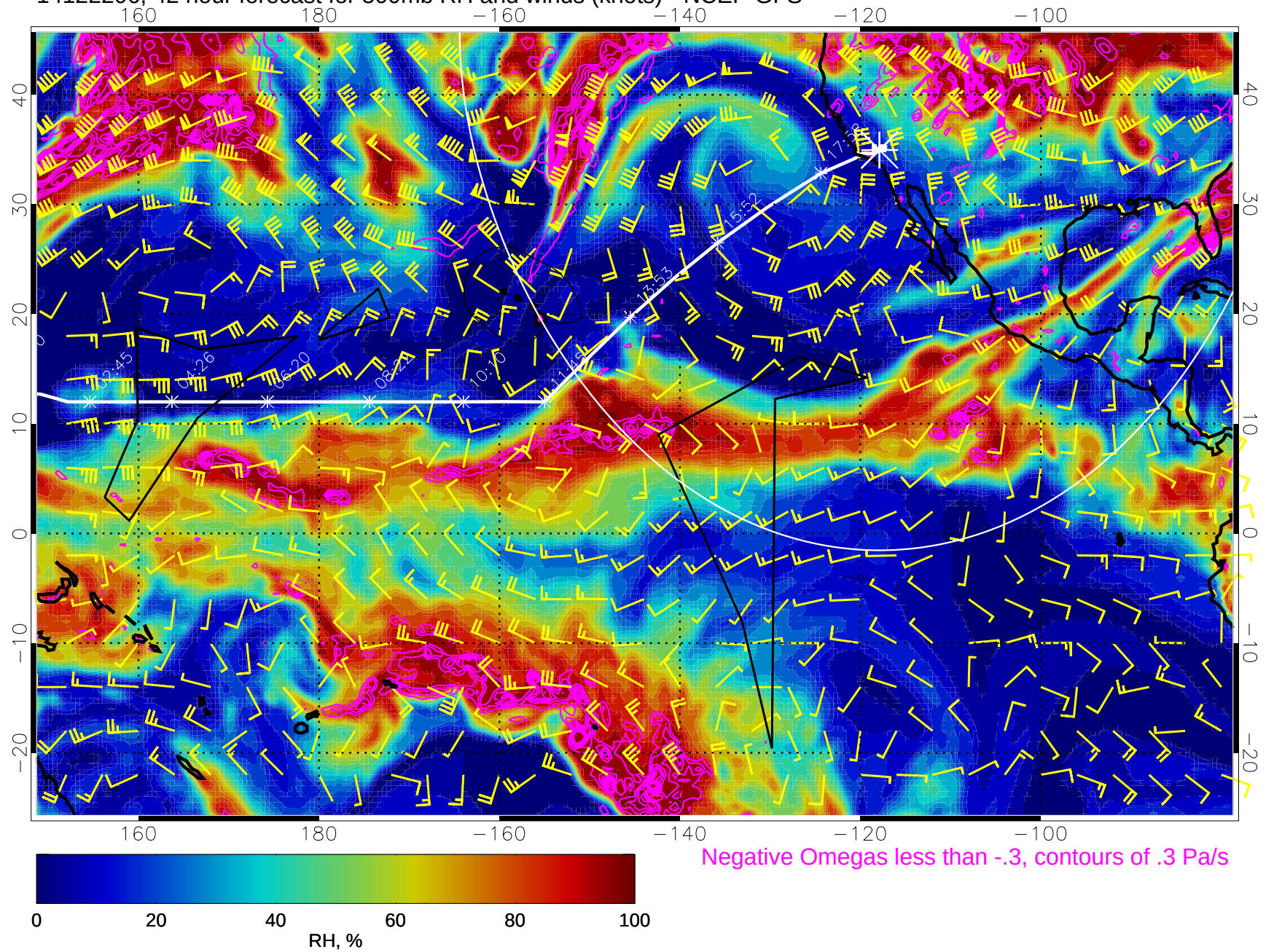
14122206, 42 hour forecast for 500mb RH and winds (knots) - NCEP GFS
