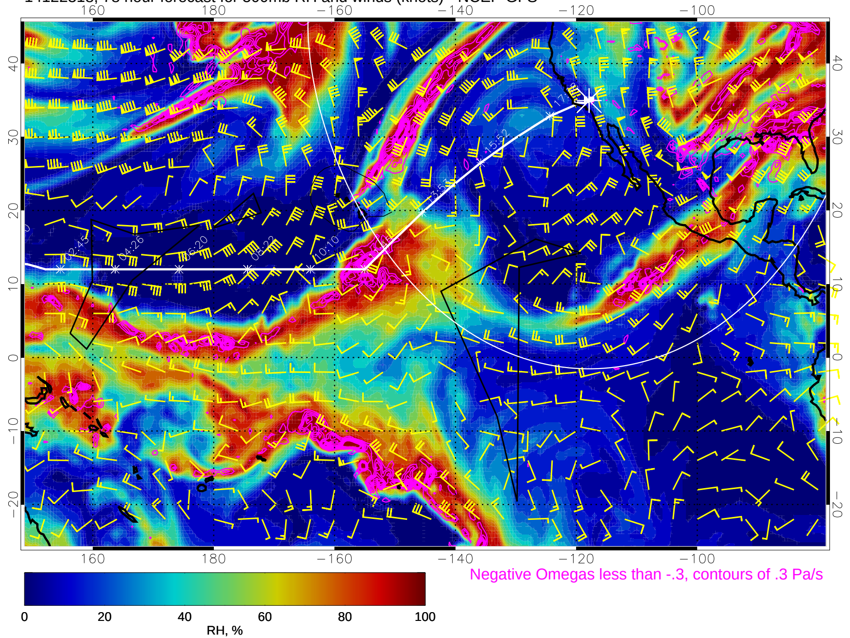
14122318, 78 hour forecast for 500mb RH and winds (knots) - NCEP GFS
