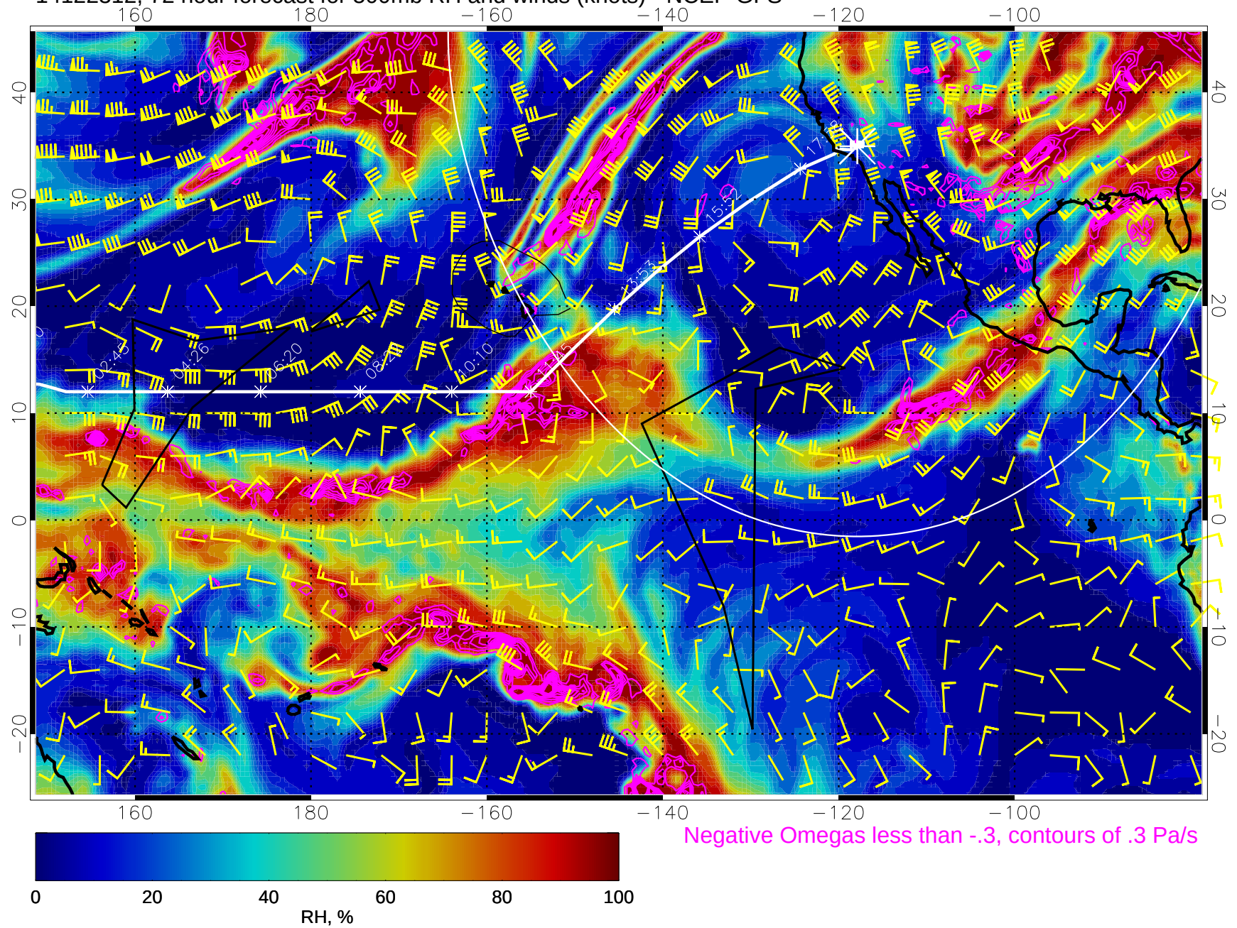
14122312, 72 hour forecast for 500mb RH and winds (knots) - NCEP GFS
