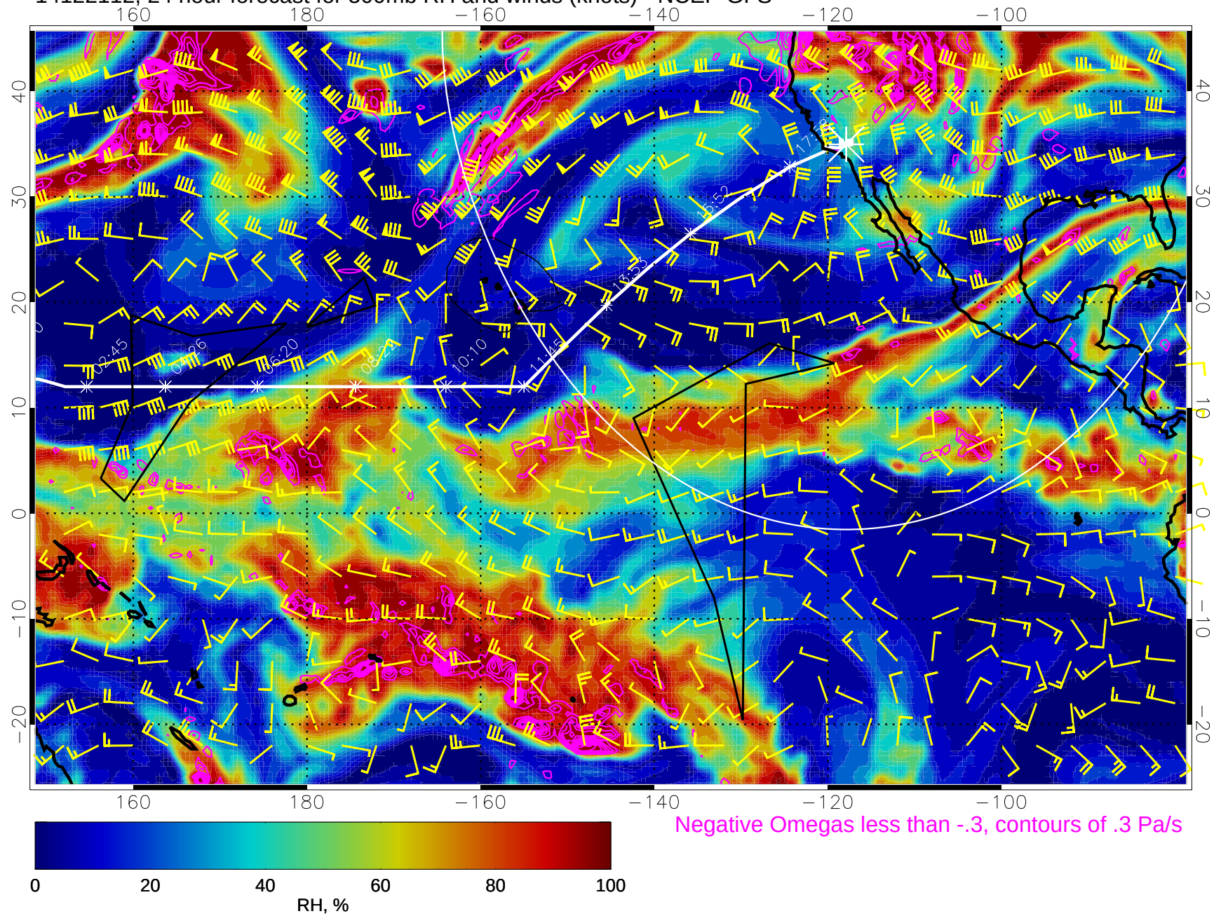
14122112, 24 hour forecast for 500mb RH and winds (knots) - NCEP GFS
