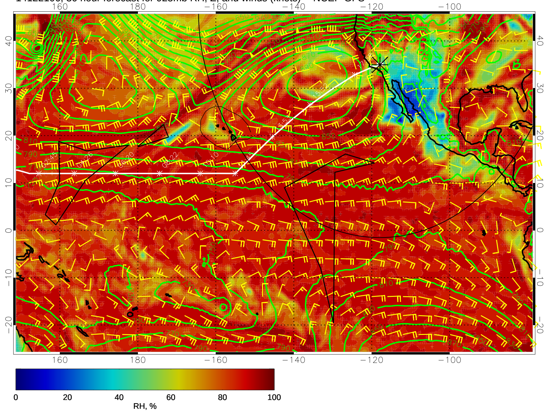
14122106, 30 hour forecast for 925mb RH, Z, and winds (knots) -- NCEP GFS
