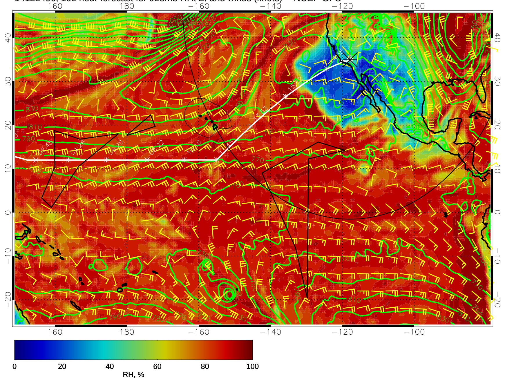
14122406, 102 hour forecast for 925mb RH, Z, and winds (knots) -- NCEP GFS
