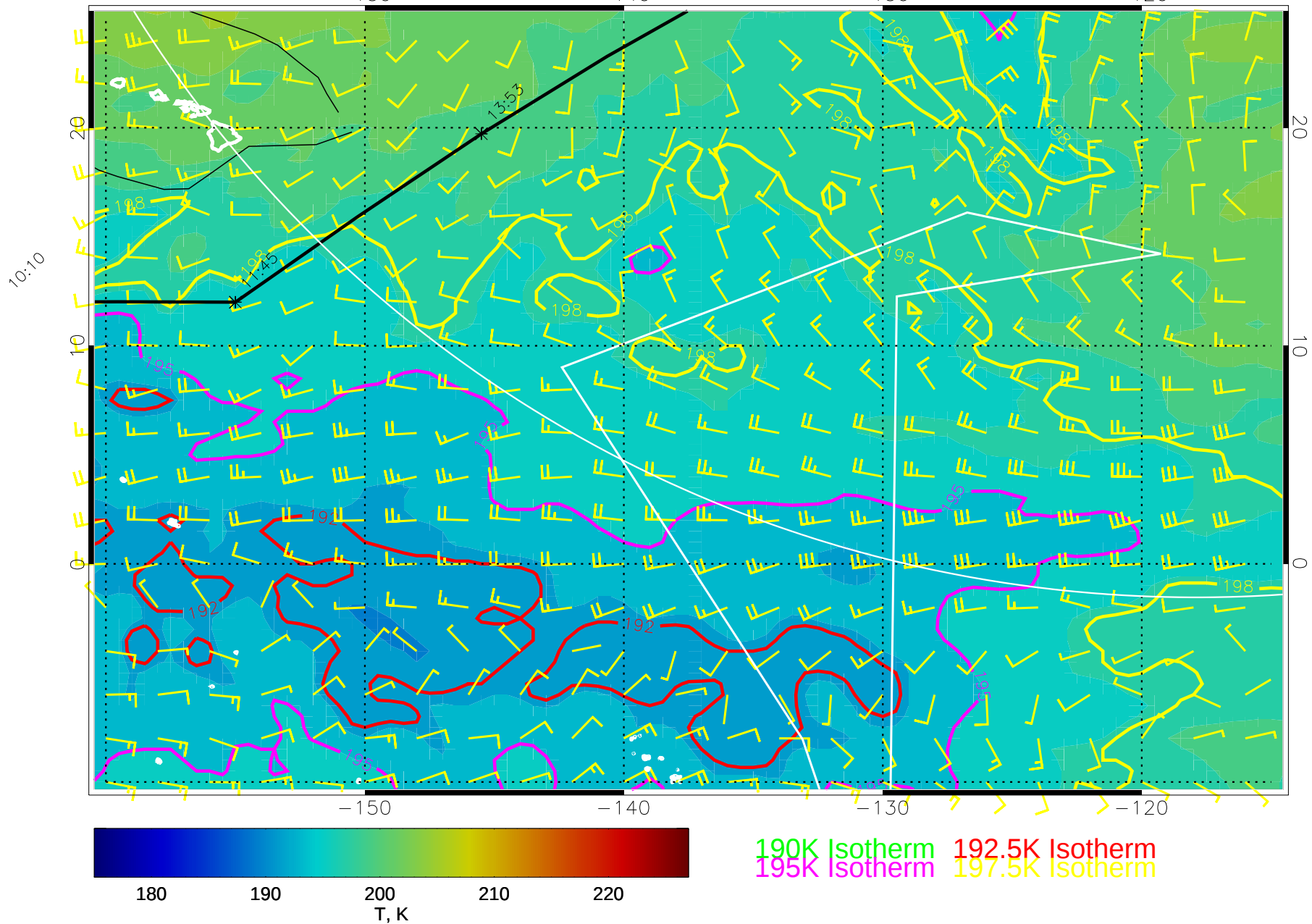
14122312, 84 hour forecast for 70mb T and winds (knots) -- NCEP GFS
