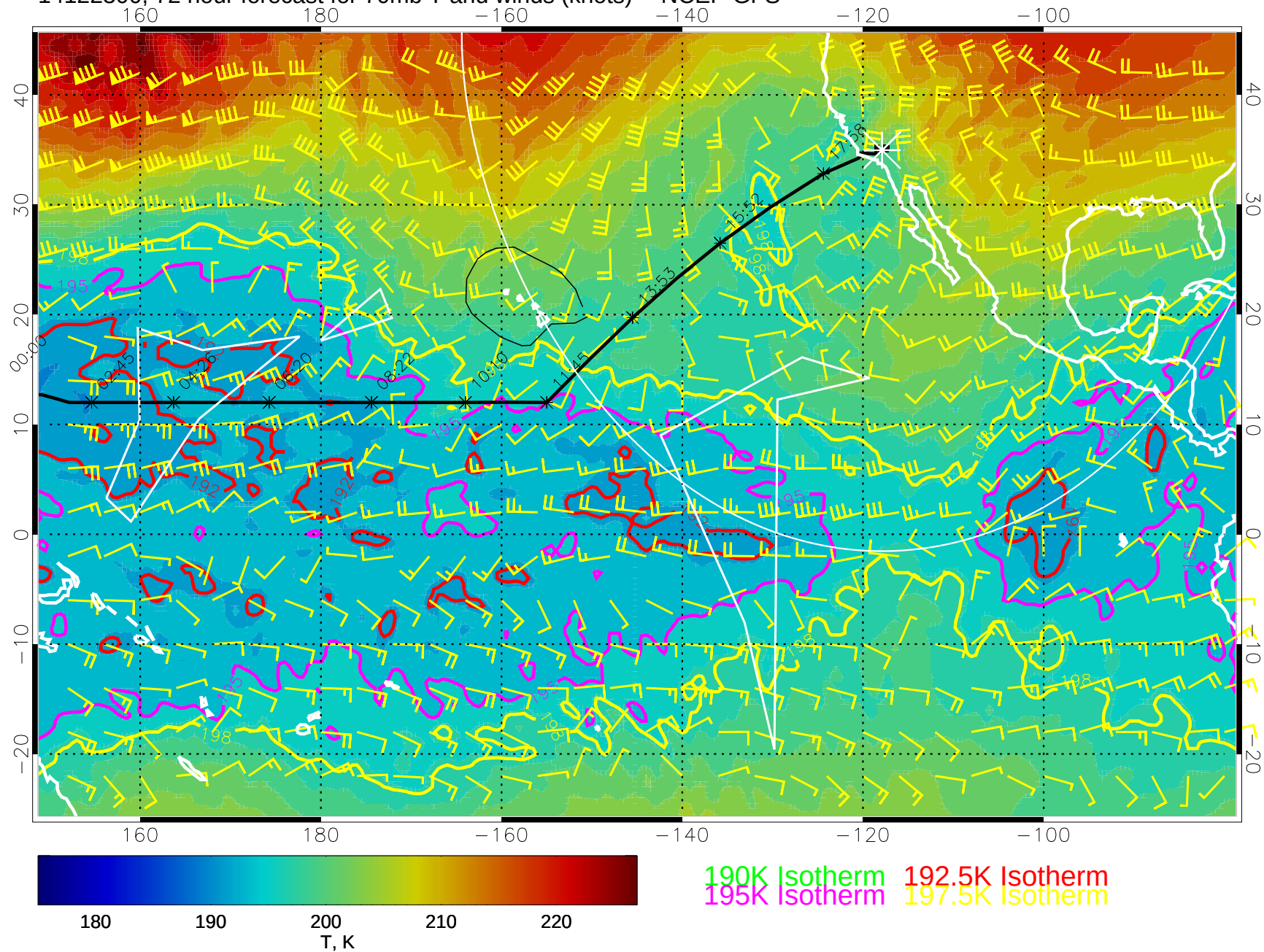
14122300, 72 hour forecast for 70mb T and winds (knots) -- NCEP GFS
