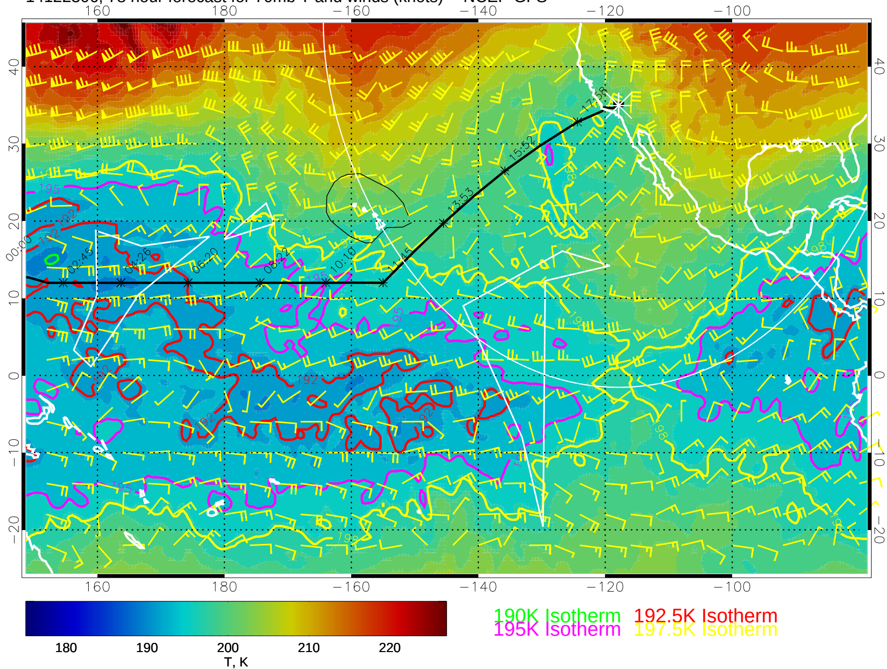
14122306, 78 hour forecast for 70mb T and winds (knots) -- NCEP GFS
