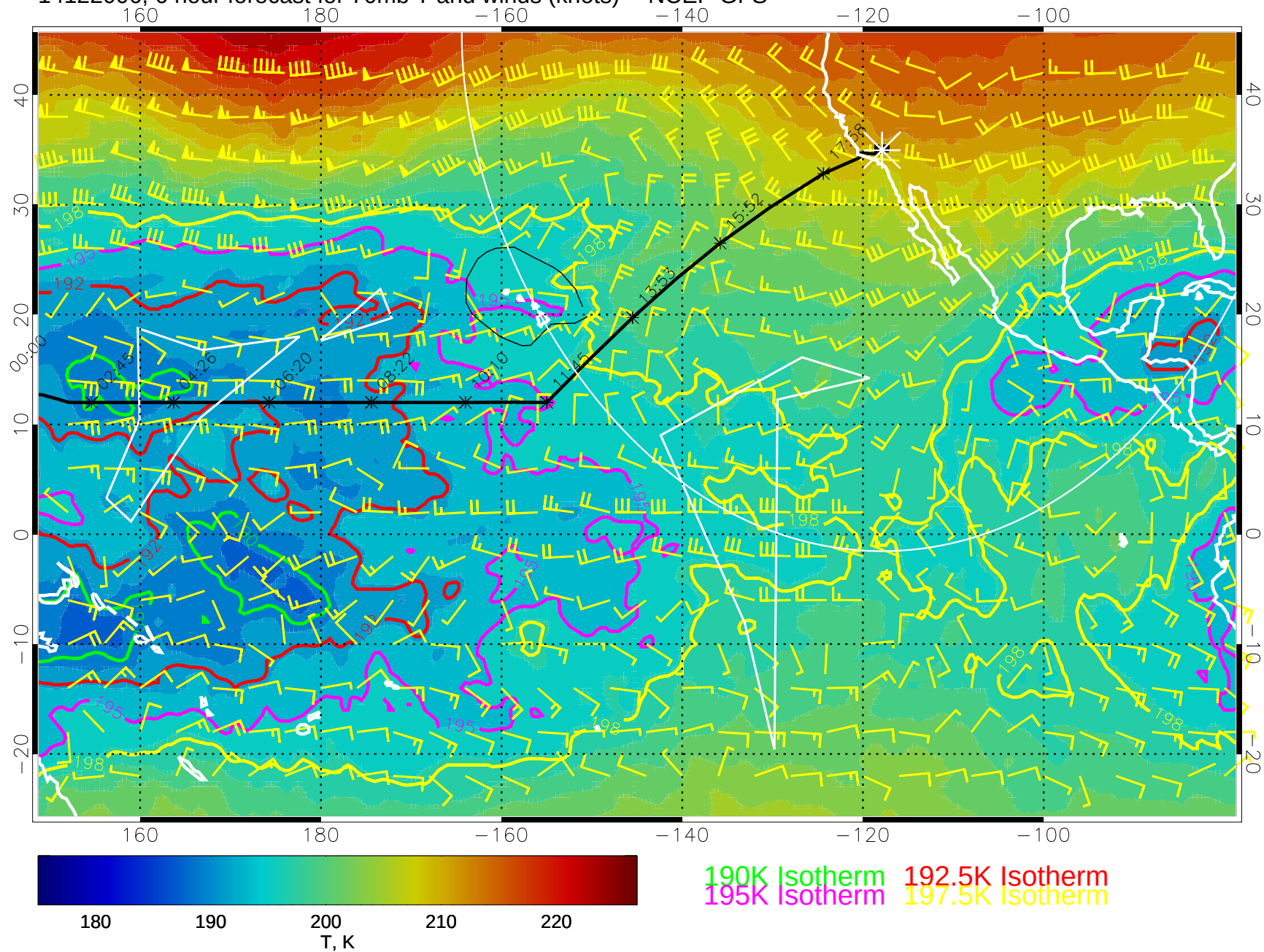
14122006, 6 hour forecast for 70mb T and winds (knots) -- NCEP GFS
