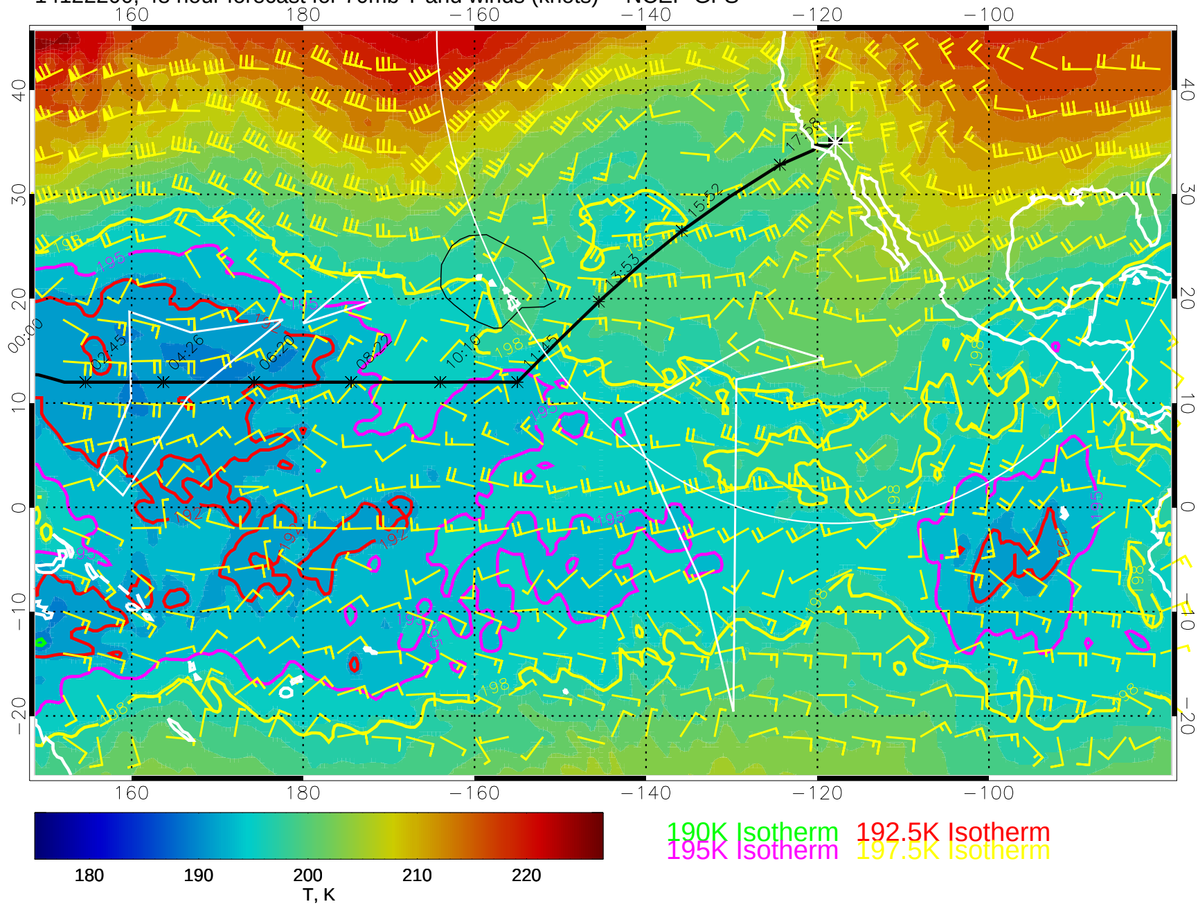
14122200, 48 hour forecast for 70mb T and winds (knots) -- NCEP GFS
