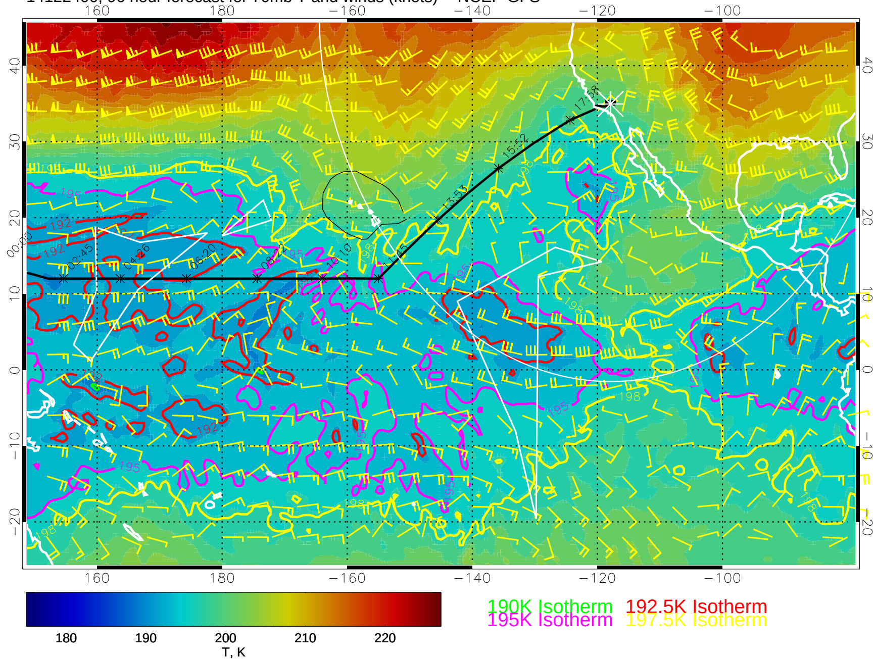
14122400, 96 hour forecast for 70mb T and winds (knots) -- NCEP GFS
