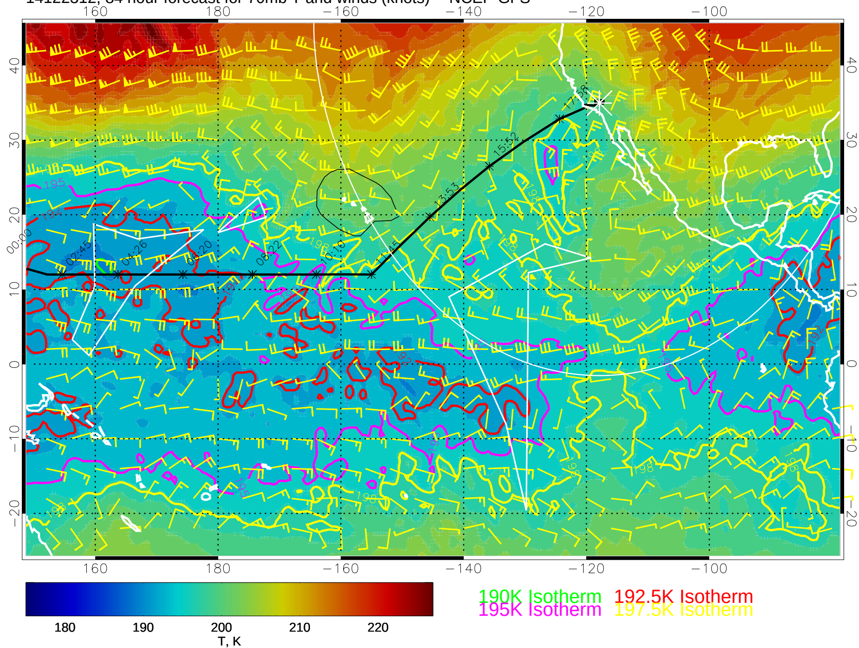
14122312, 84 hour forecast for 70mb T and winds (knots) -- NCEP GFS
