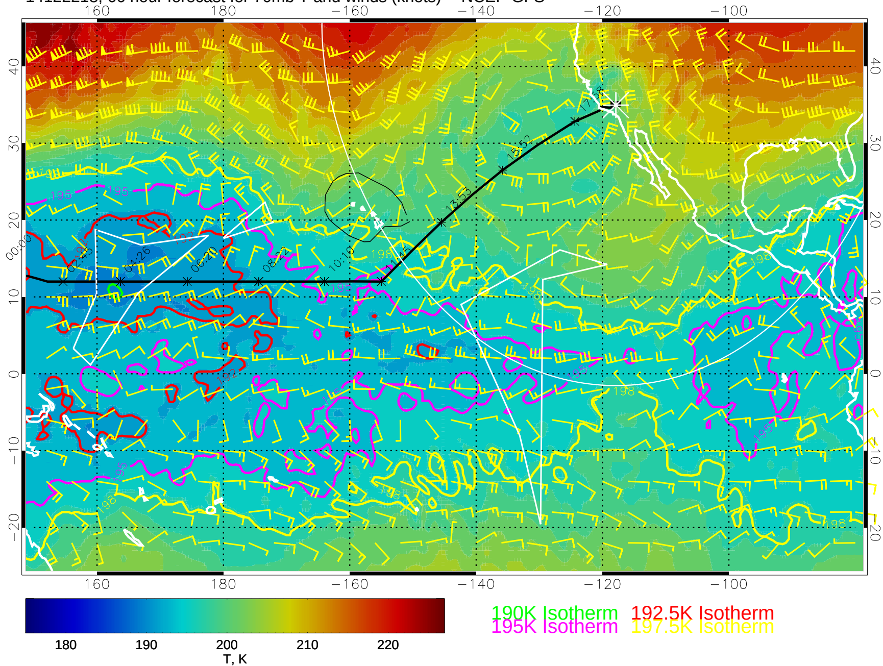
14122218, 66 hour forecast for 70mb T and winds (knots) -- NCEP GFS
