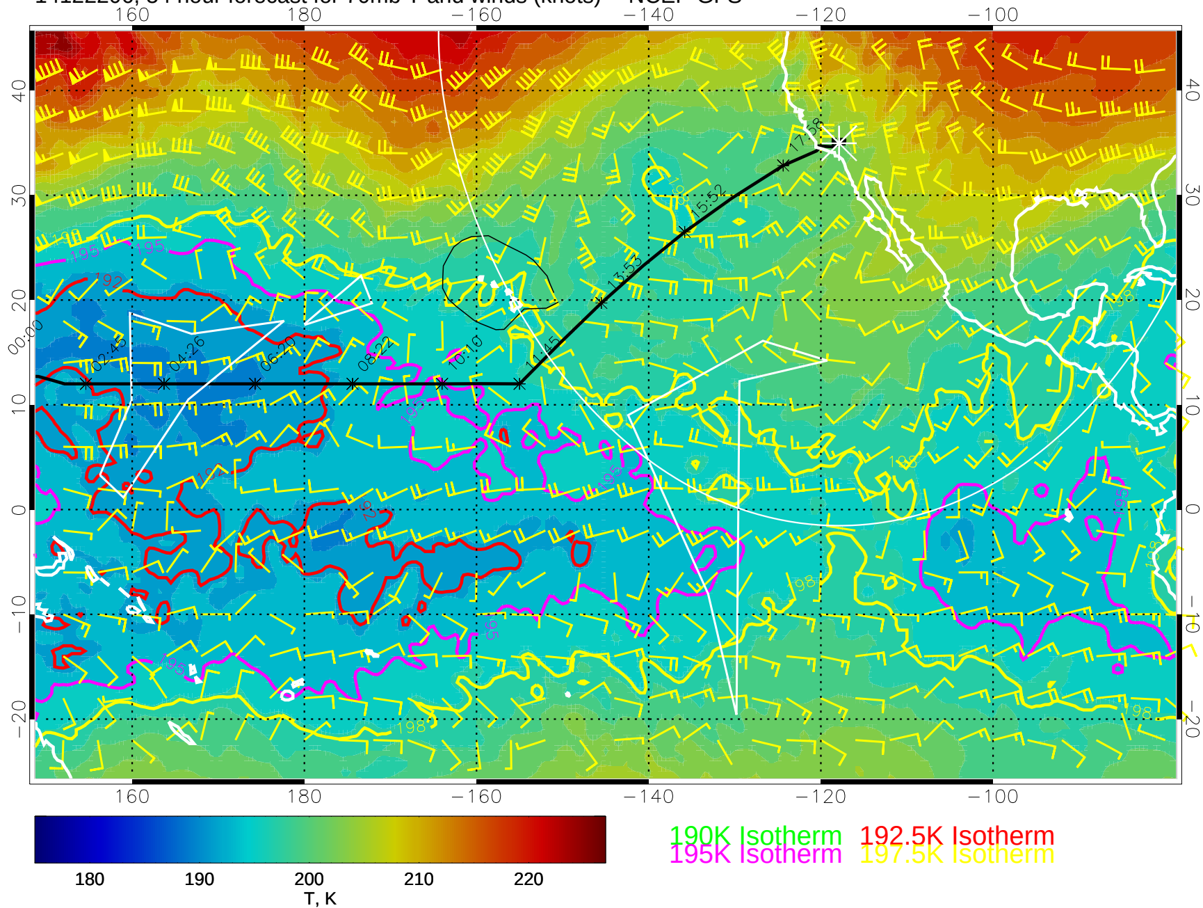
14122206, 54 hour forecast for 70mb T and winds (knots) -- NCEP GFS
