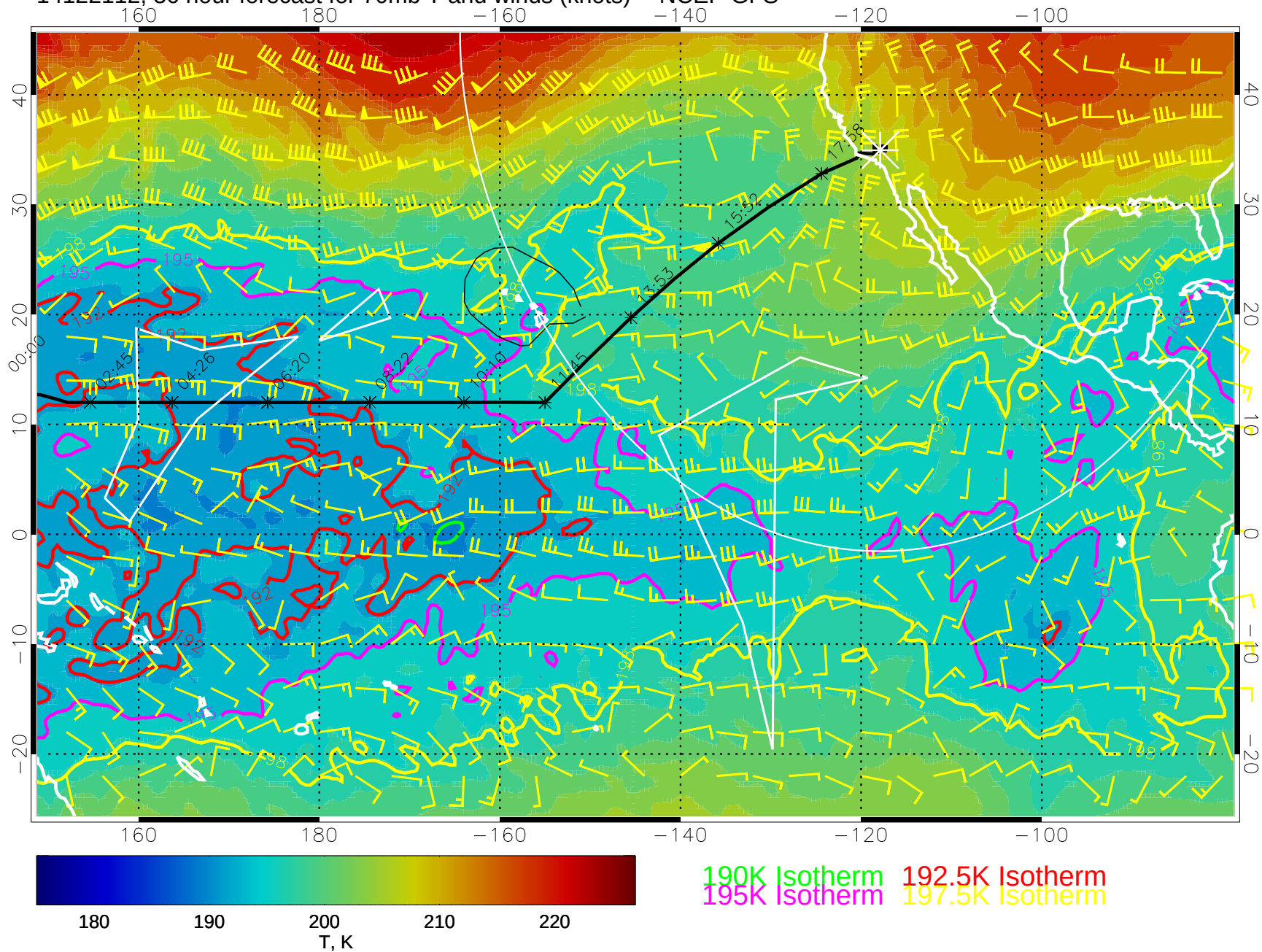
14122112, 36 hour forecast for 70mb T and winds (knots) -- NCEP GFS
