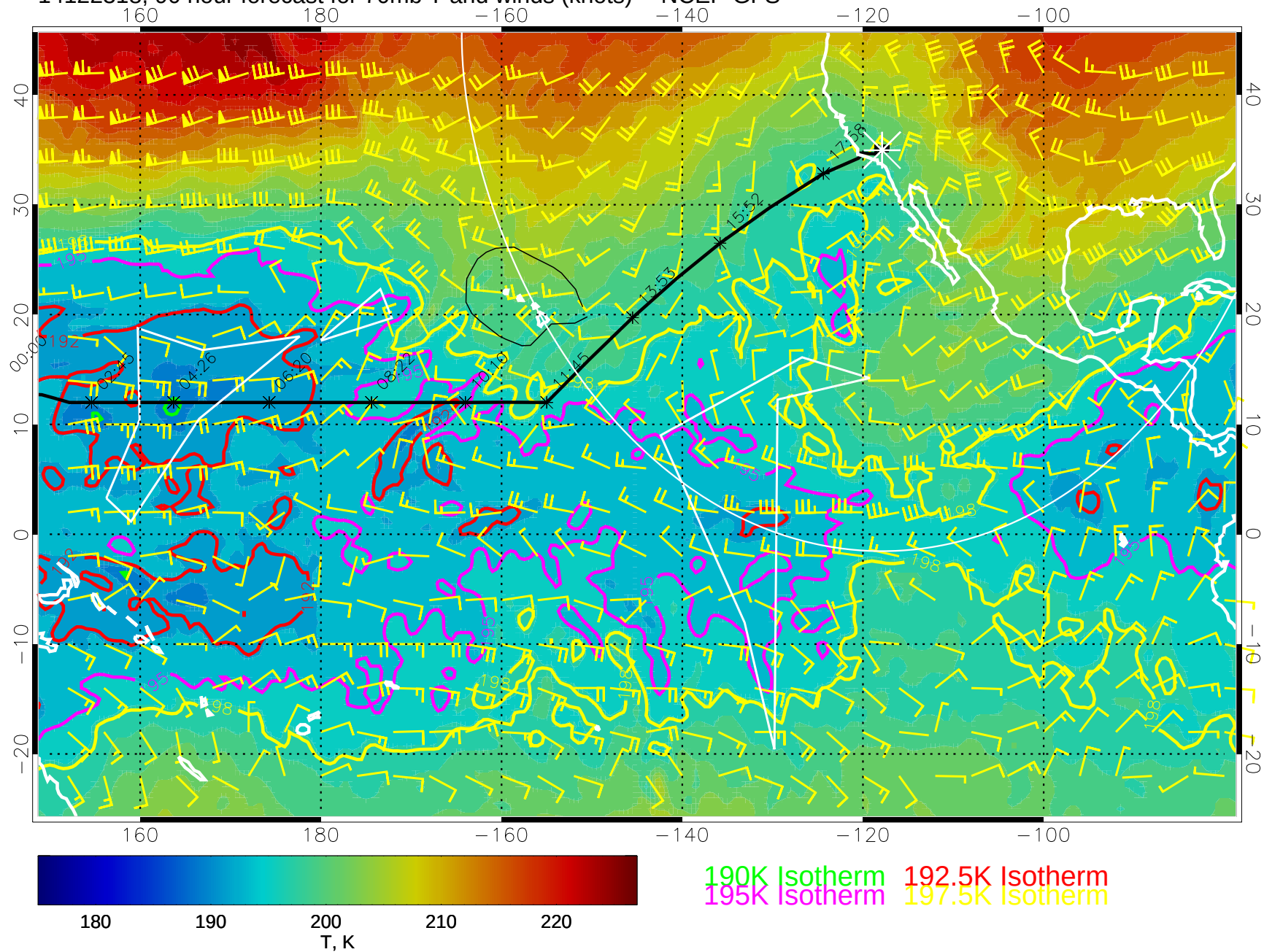
14122318, 90 hour forecast for 70mb T and winds (knots) -- NCEP GFS
