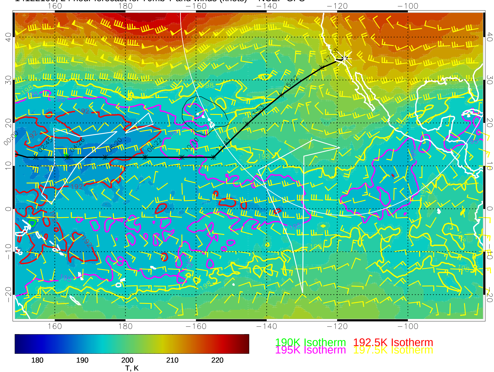
14122100, 24 hour forecast for 70mb T and winds (knots) -- NCEP GFS
