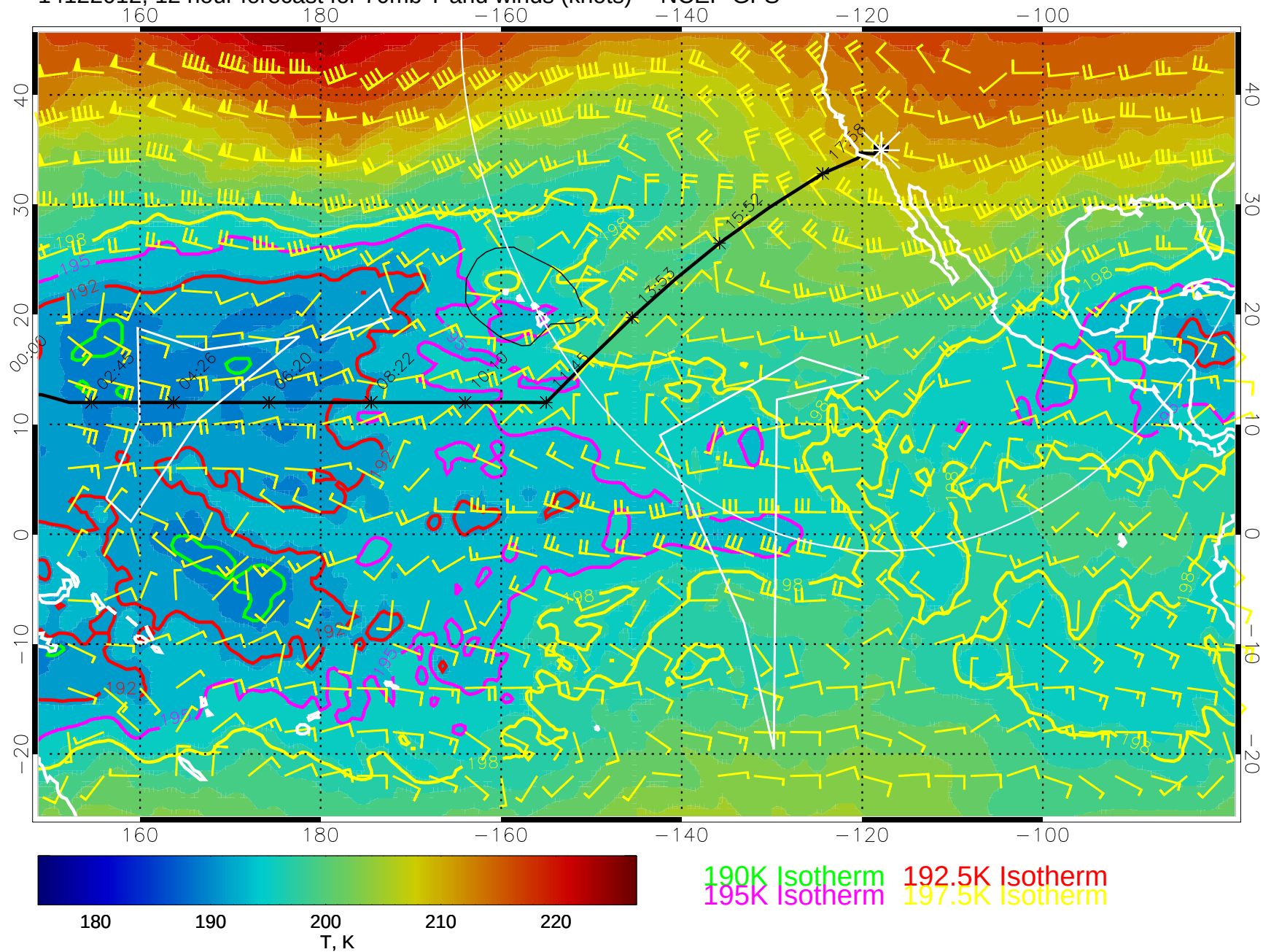
14122012, 12 hour forecast for 70mb T and winds (knots) -- NCEP GFS
