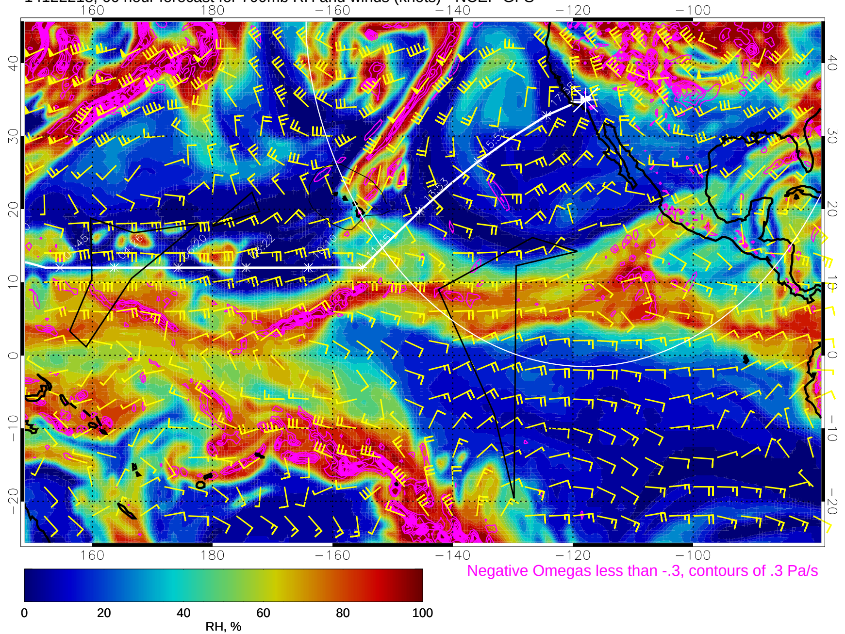
14122218, 66 hour forecast for 700mb RH and winds (knots) - NCEP GFS
