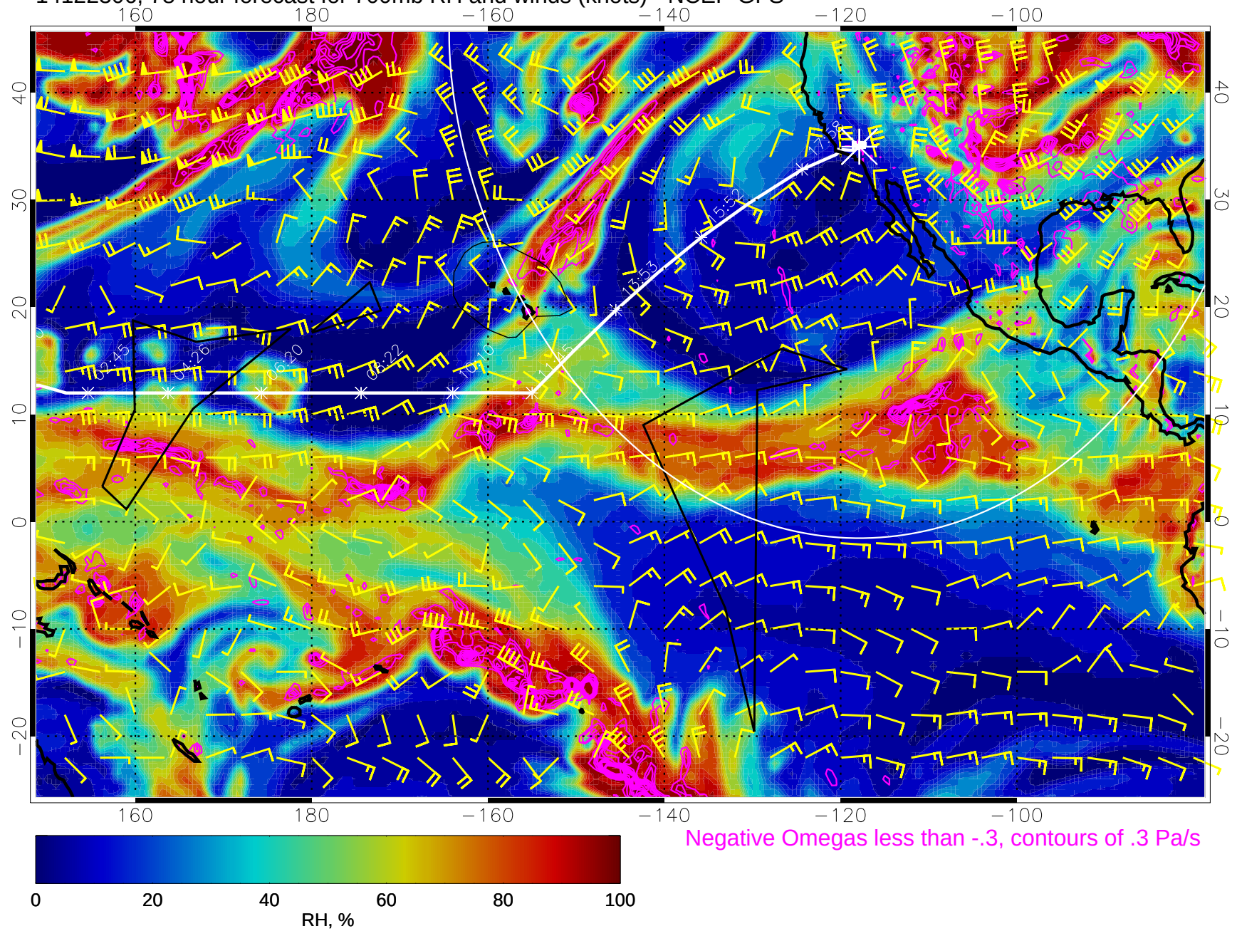
14122306, 78 hour forecast for 700mb RH and winds (knots) - NCEP GFS
