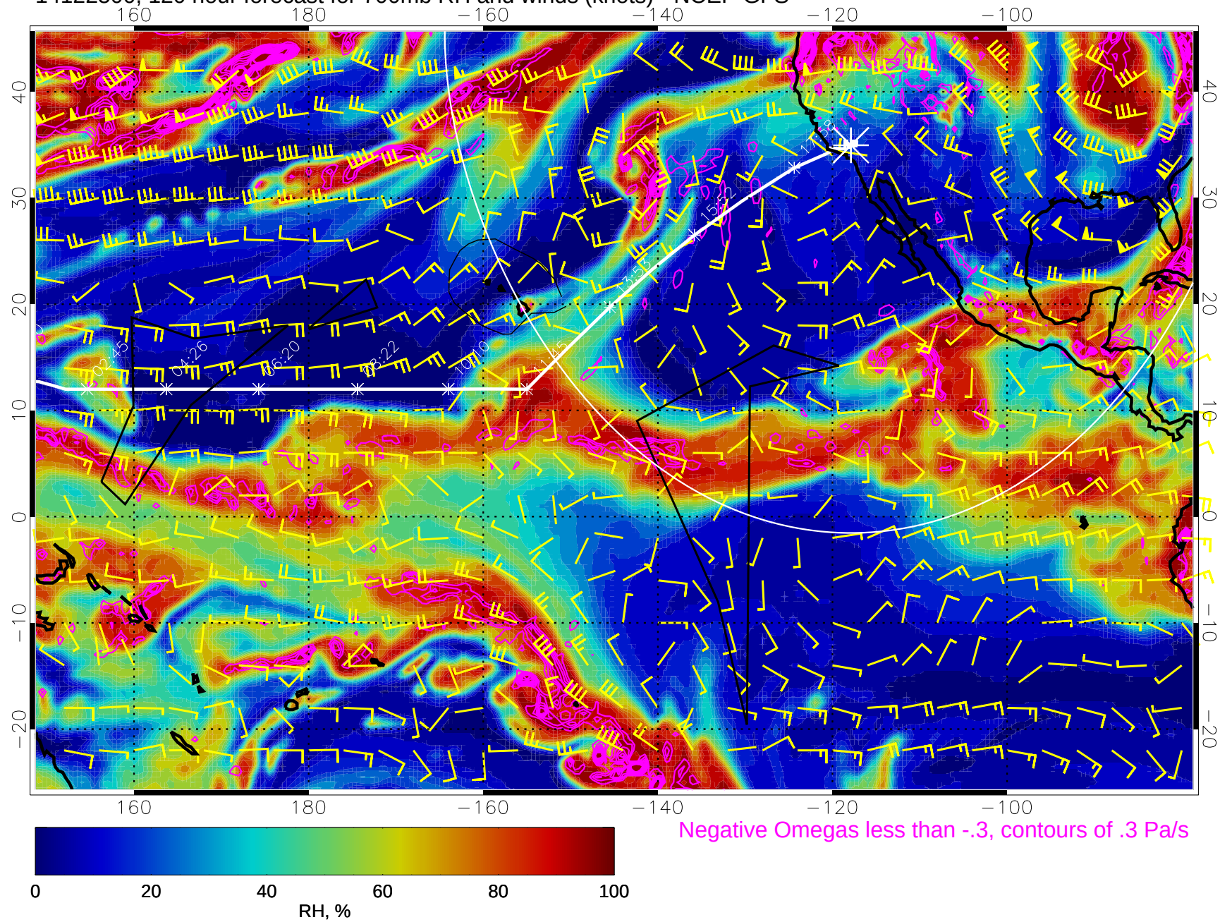
14122500, 120 hour forecast for 700mb RH and winds (knots) - NCEP GFS
