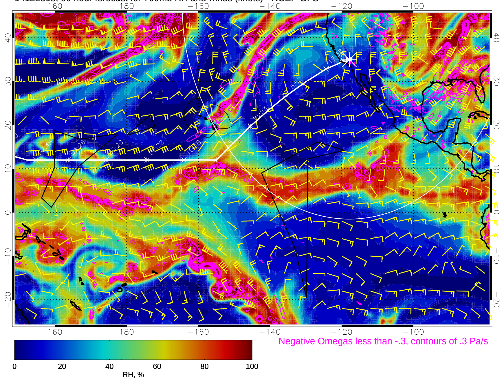
14122318, 90 hour forecast for 700mb RH and winds (knots) - NCEP GFS
