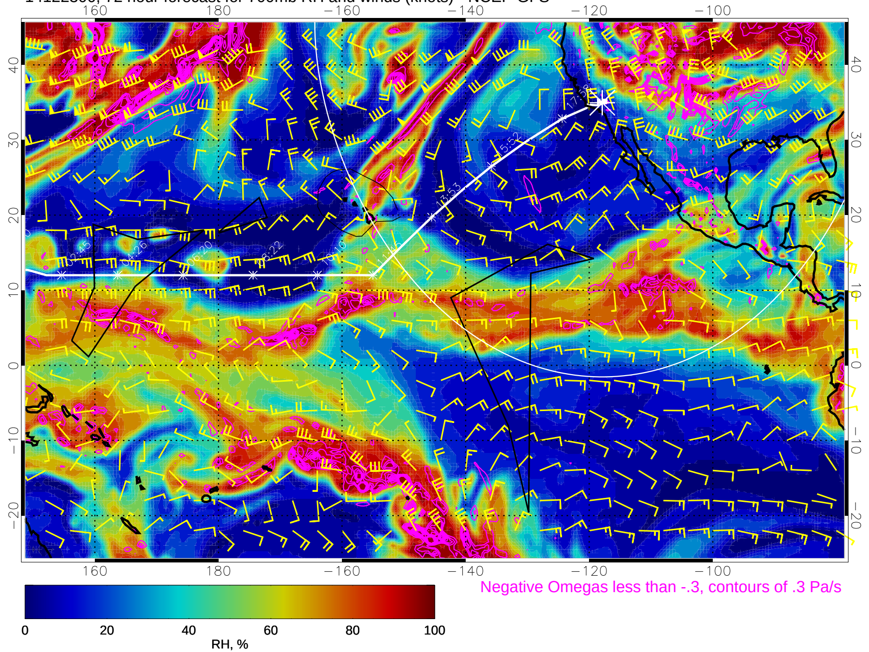
14122300, 72 hour forecast for 700mb RH and winds (knots) - NCEP GFS
