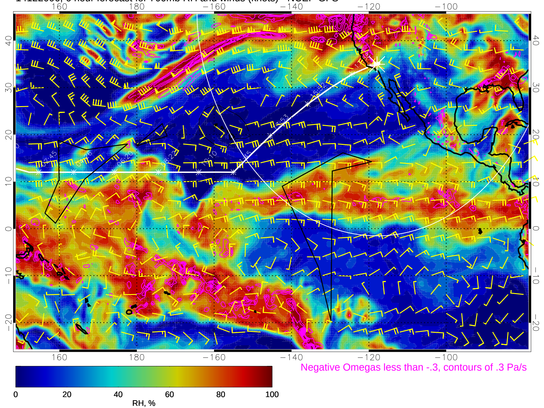
14122006, 6 hour forecast for 700mb RH and winds (knots) - NCEP GFS
