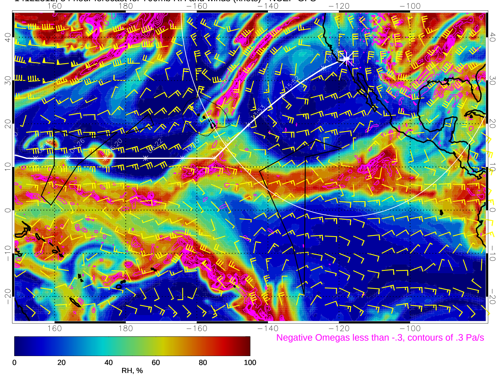
14122312, 84 hour forecast for 700mb RH and winds (knots) - NCEP GFS
