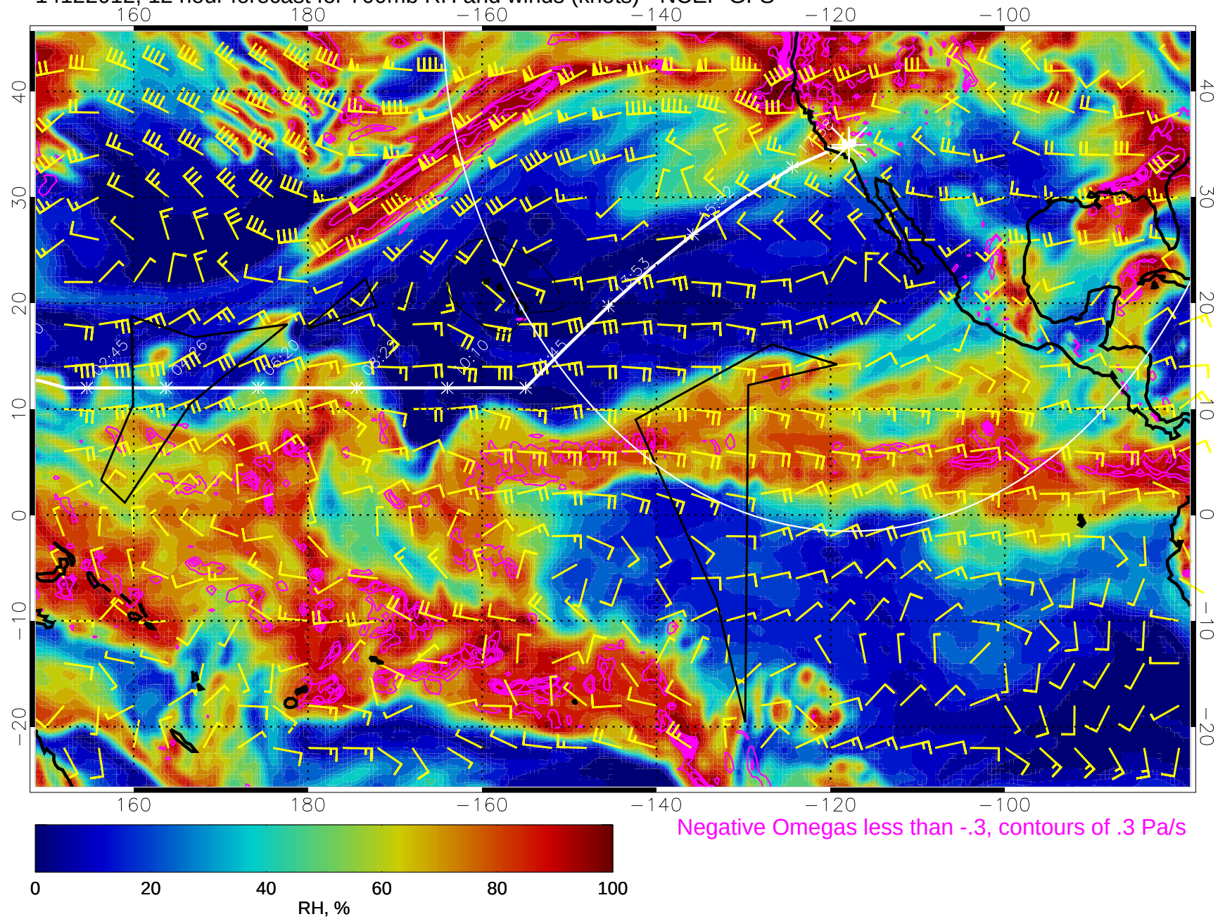
14122012, 12 hour forecast for 700mb RH and winds (knots) - NCEP GFS
