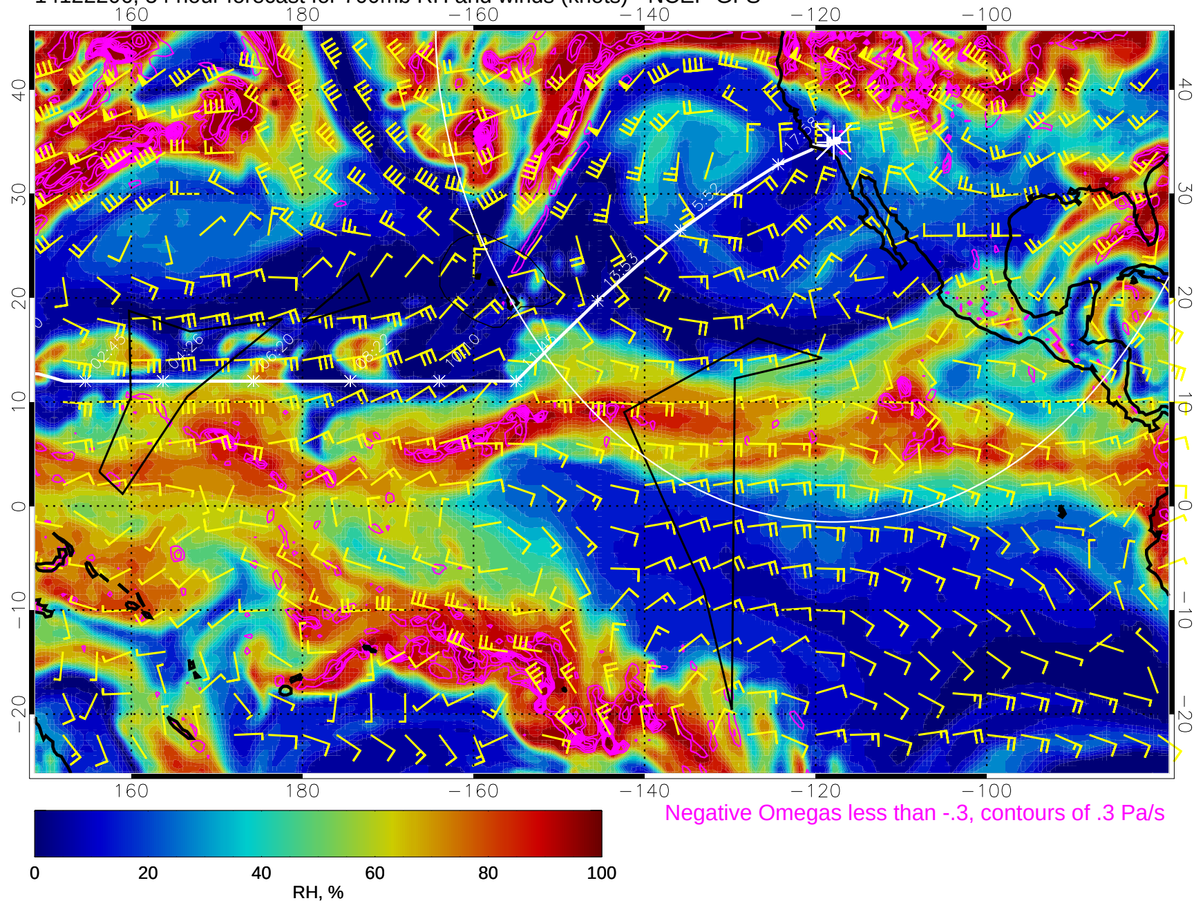
14122206, 54 hour forecast for 700mb RH and winds (knots) - NCEP GFS
