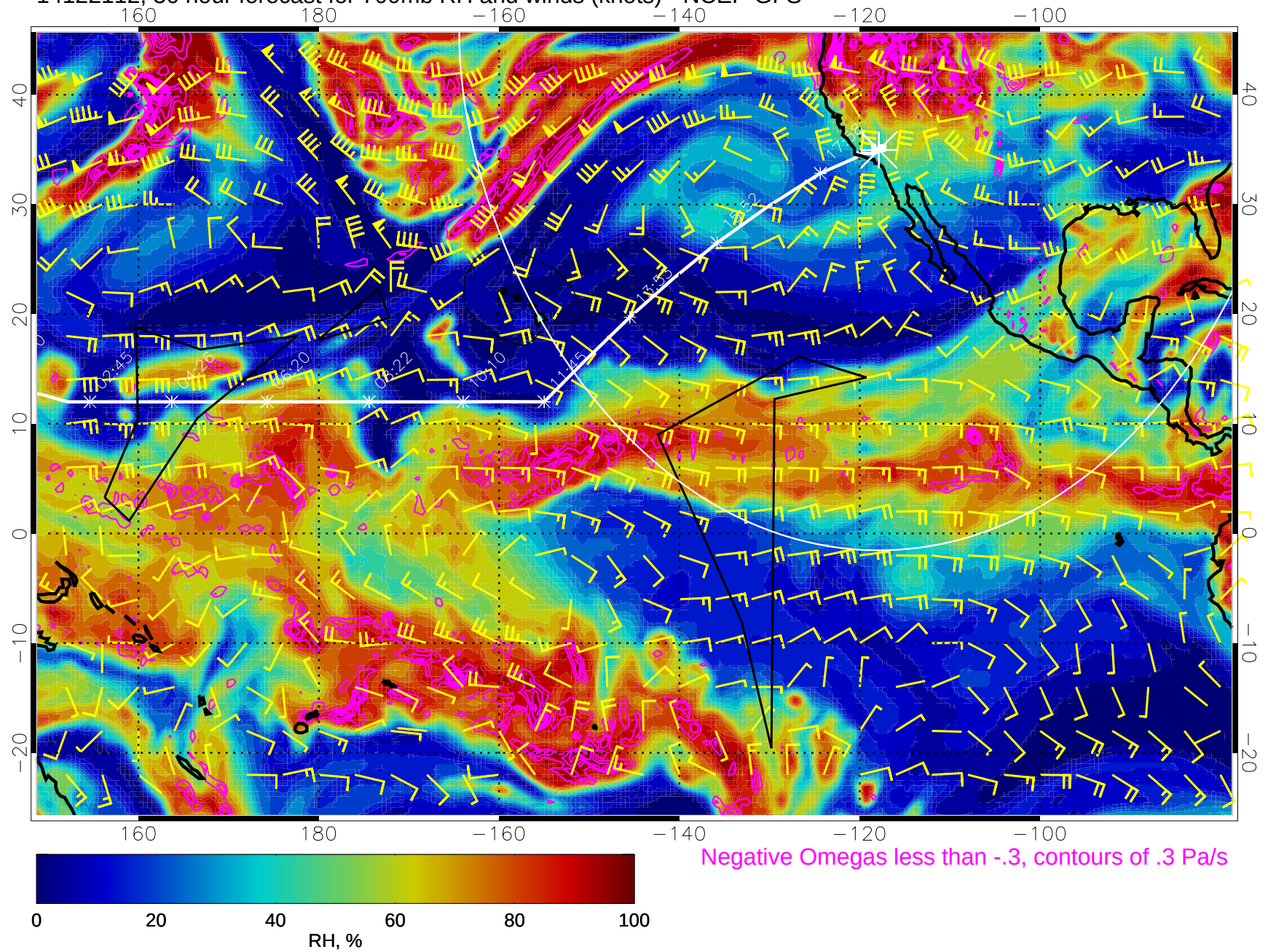
14122112, 36 hour forecast for 700mb RH and winds (knots) - NCEP GFS
