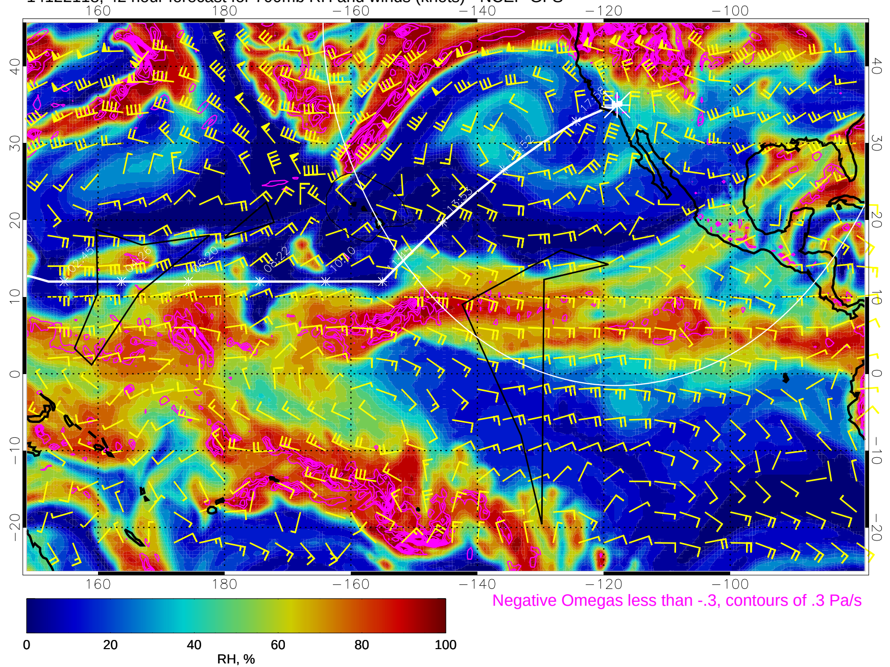
14122118, 42 hour forecast for 700mb RH and winds (knots) - NCEP GFS
