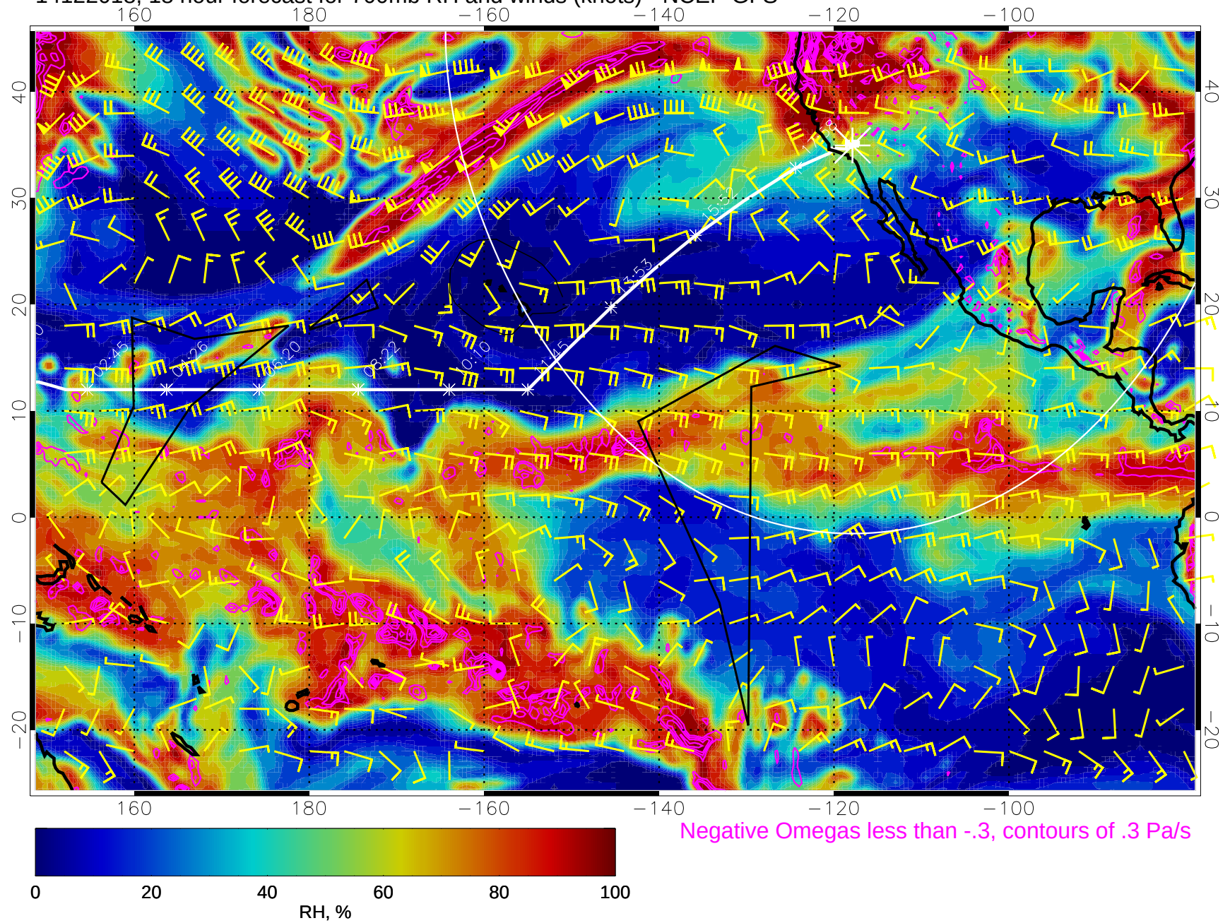
14122018, 18 hour forecast for 700mb RH and winds (knots) - NCEP GFS
