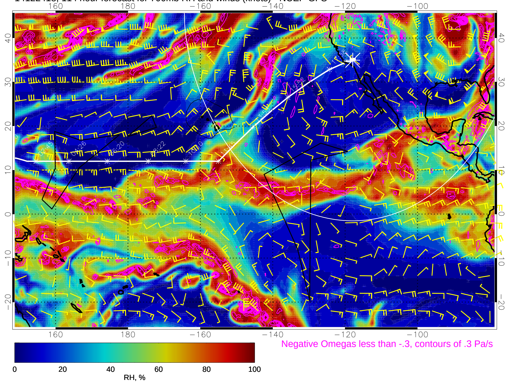
14122418, 114 hour forecast for 700mb RH and winds (knots) - NCEP GFS
