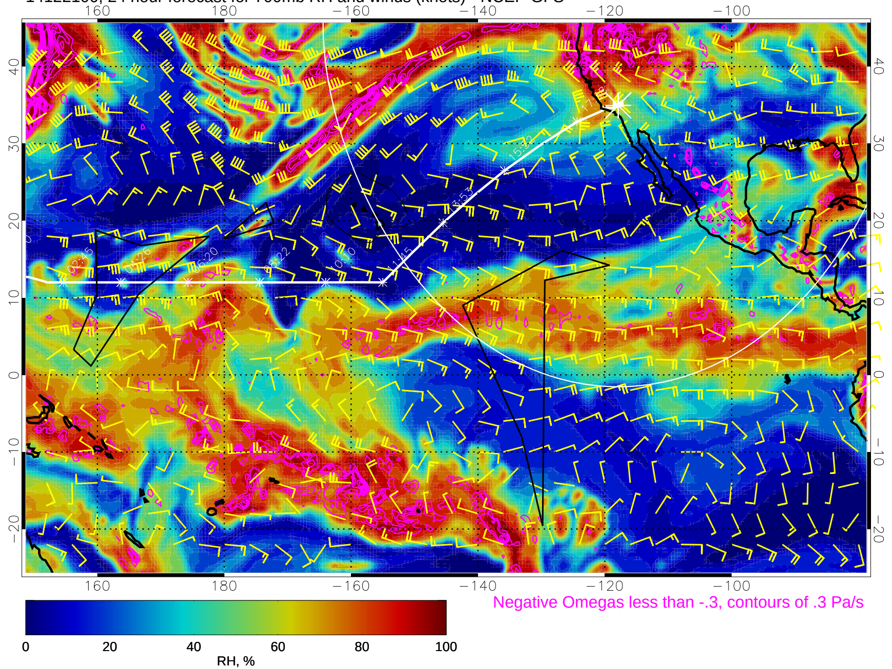
14122100, 24 hour forecast for 700mb RH and winds (knots) - NCEP GFS
