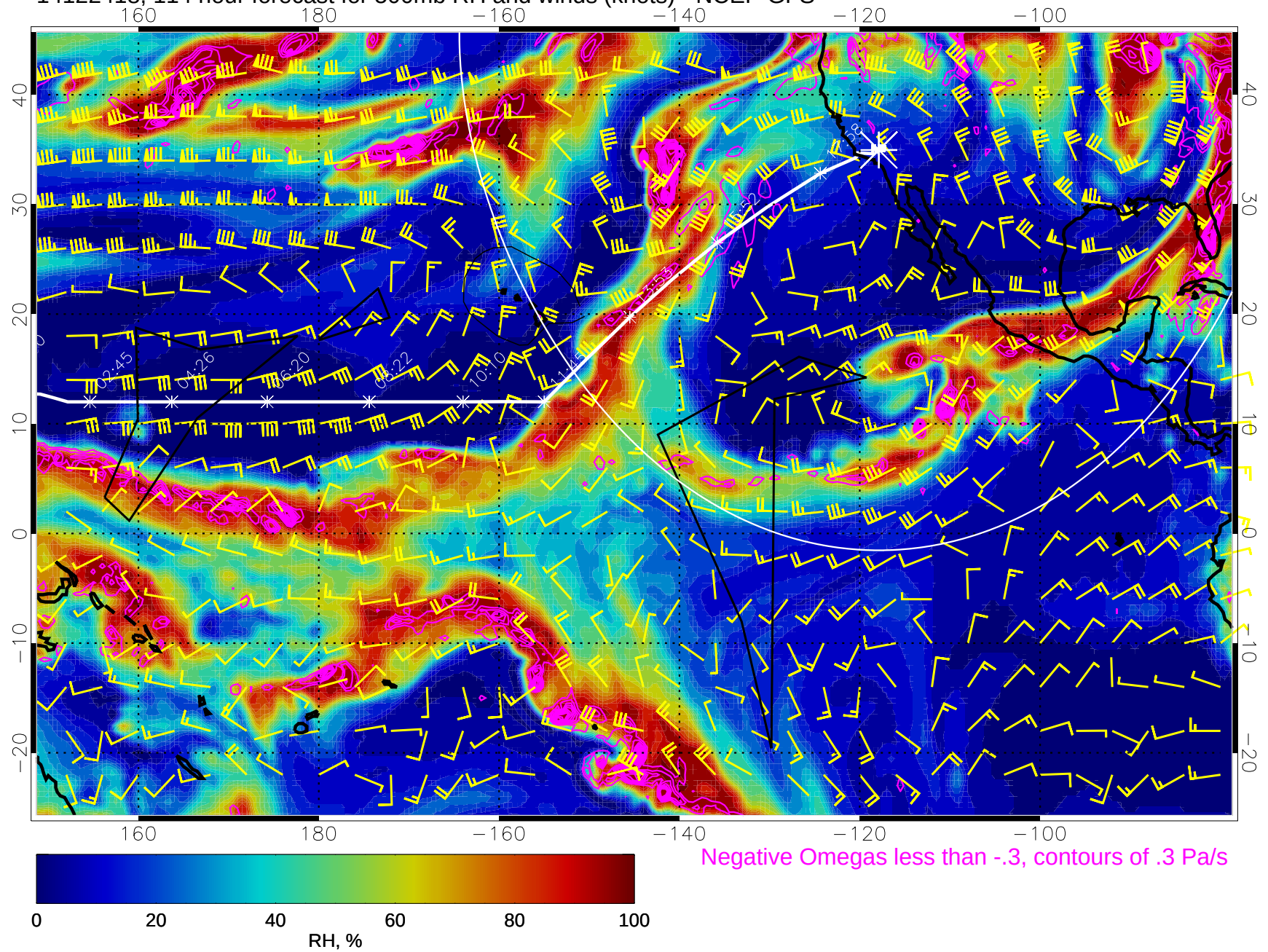
14122418, 114 hour forecast for 500mb RH and winds (knots) - NCEP GFS
