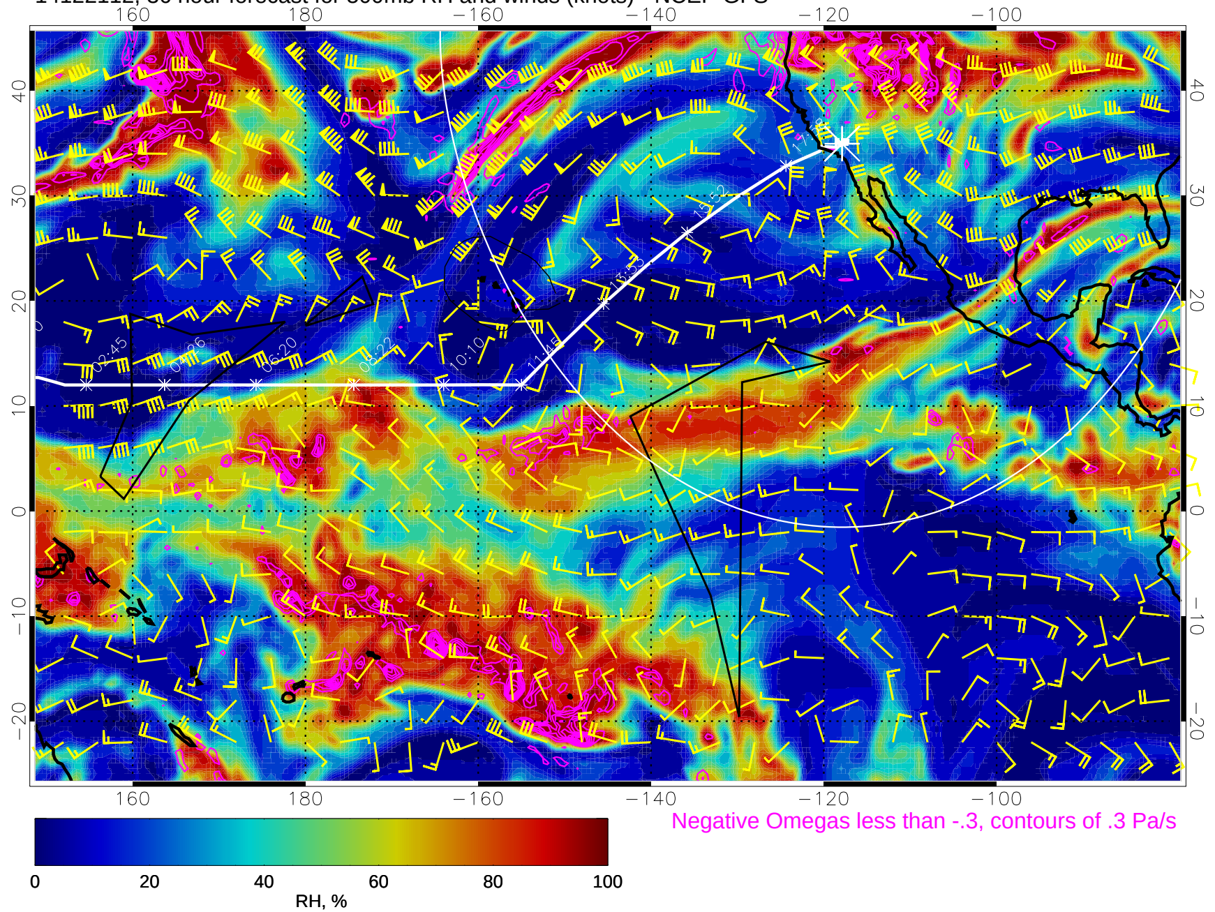
14122112, 36 hour forecast for 500mb RH and winds (knots) - NCEP GFS
