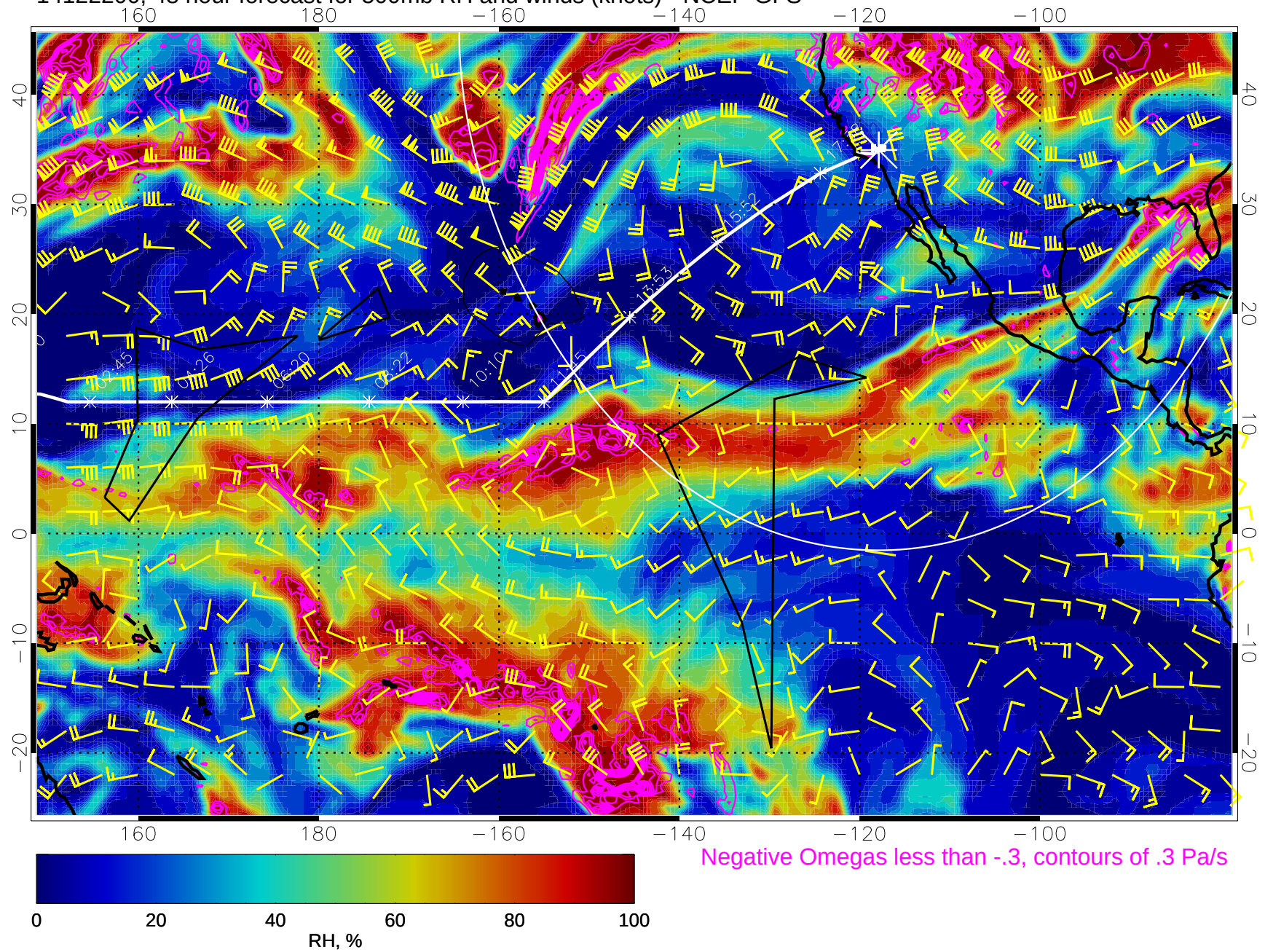
14122200, 48 hour forecast for 500mb RH and winds (knots) - NCEP GFS
