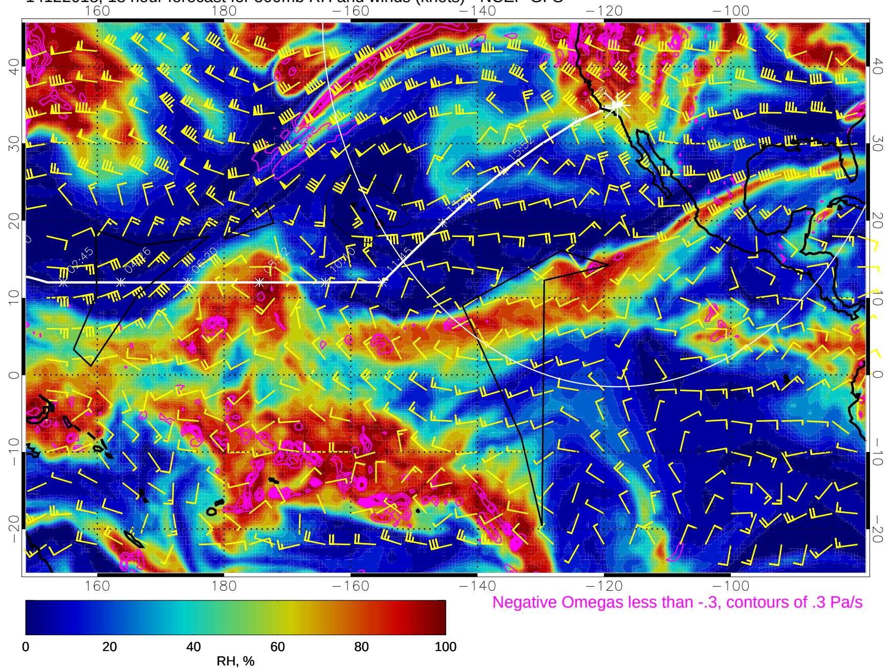
14122018, 18 hour forecast for 500mb RH and winds (knots) - NCEP GFS
