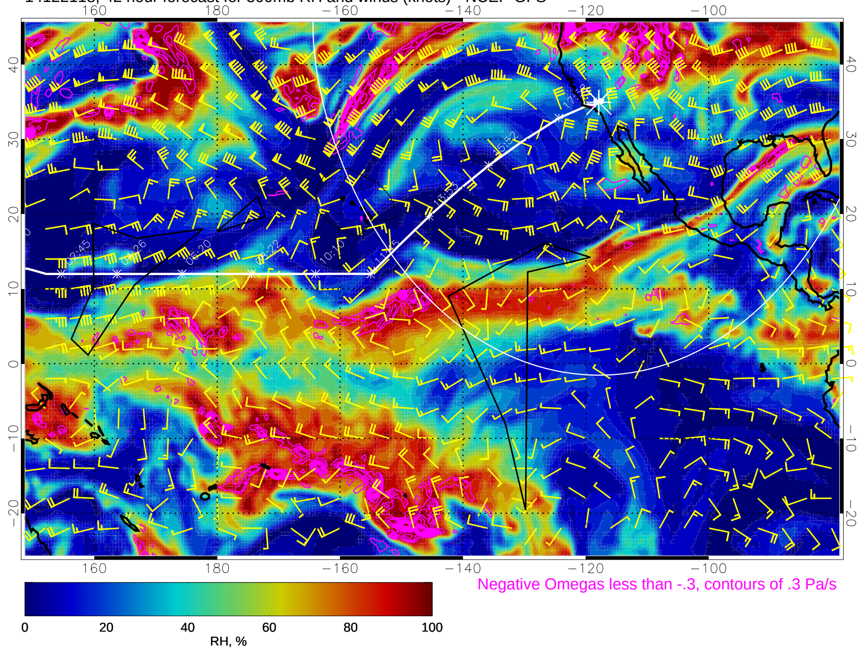
14122118, 42 hour forecast for 500mb RH and winds (knots) - NCEP GFS
