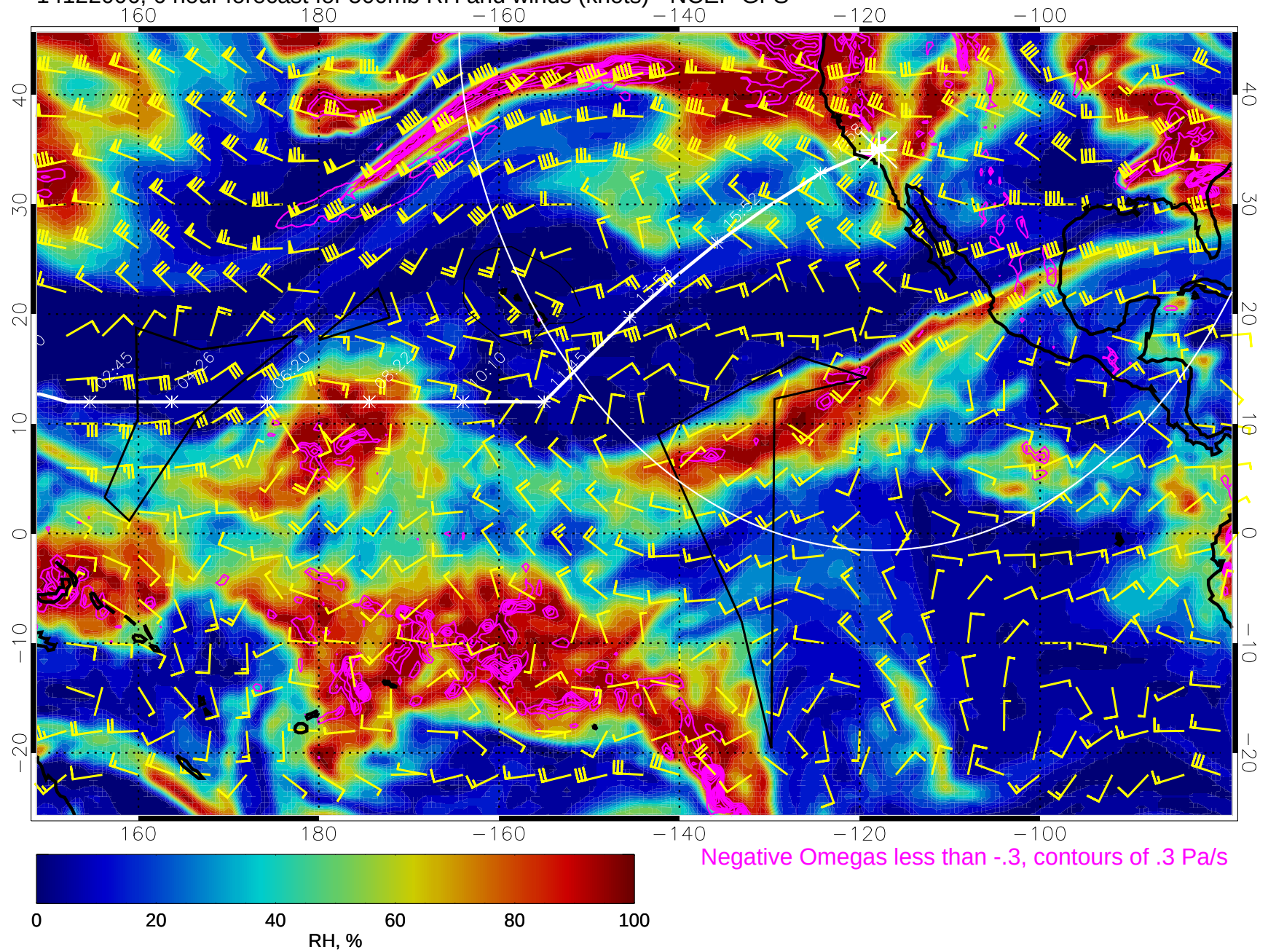
14122006, 6 hour forecast for 500mb RH and winds (knots) - NCEP GFS
