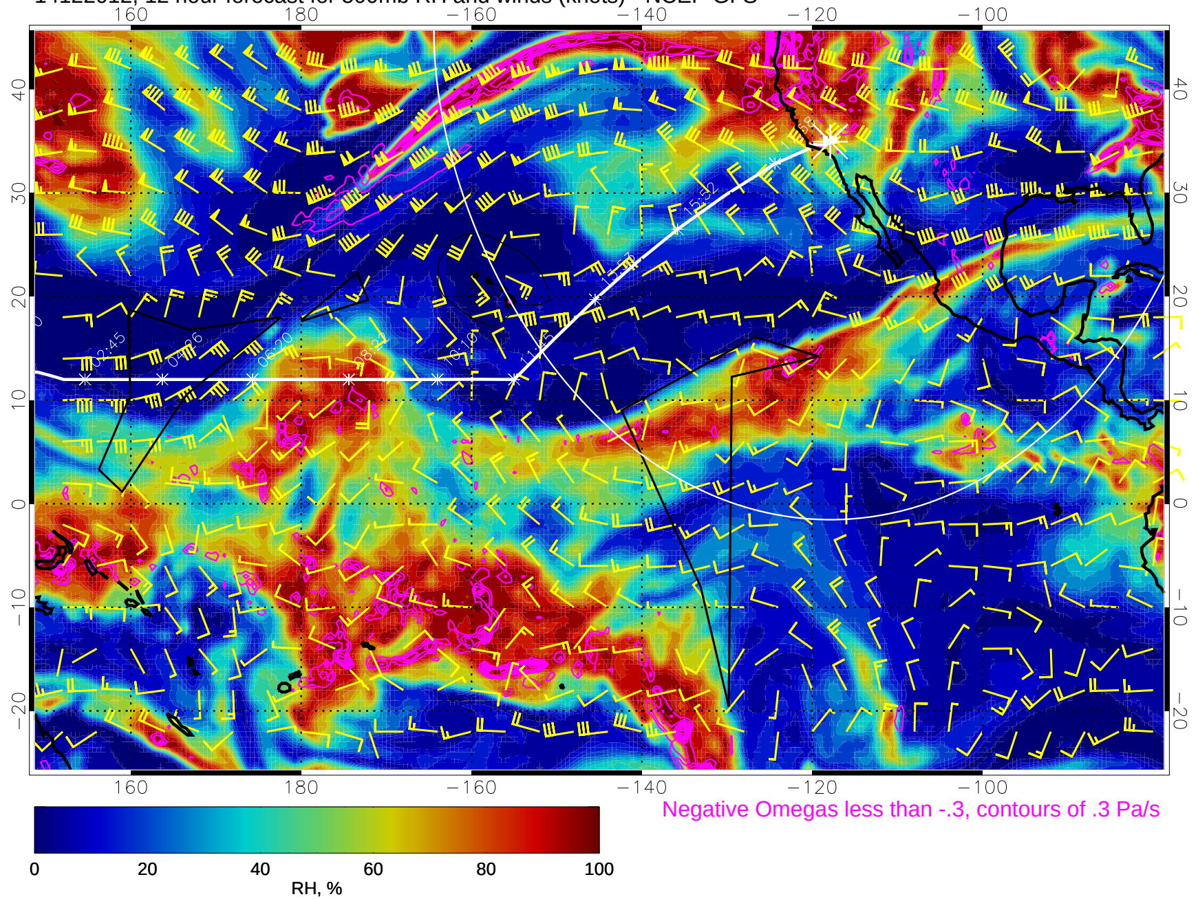
14122012, 12 hour forecast for 500mb RH and winds (knots) - NCEP GFS
