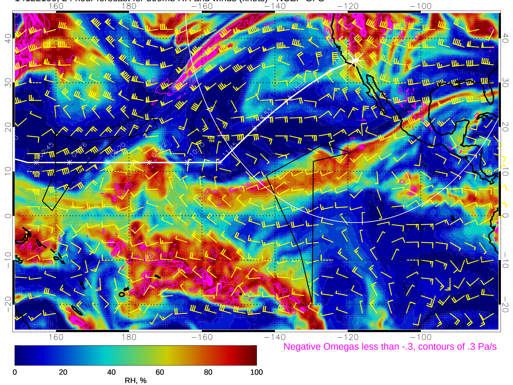
14122100, 24 hour forecast for 500mb RH and winds (knots) - NCEP GFS
