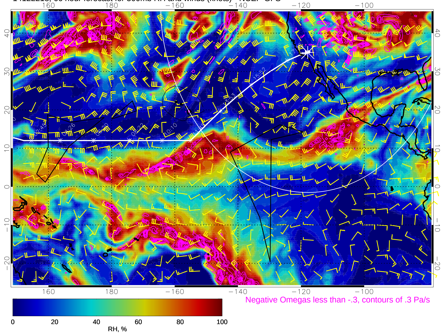
14122218, 66 hour forecast for 500mb RH and winds (knots) - NCEP GFS
