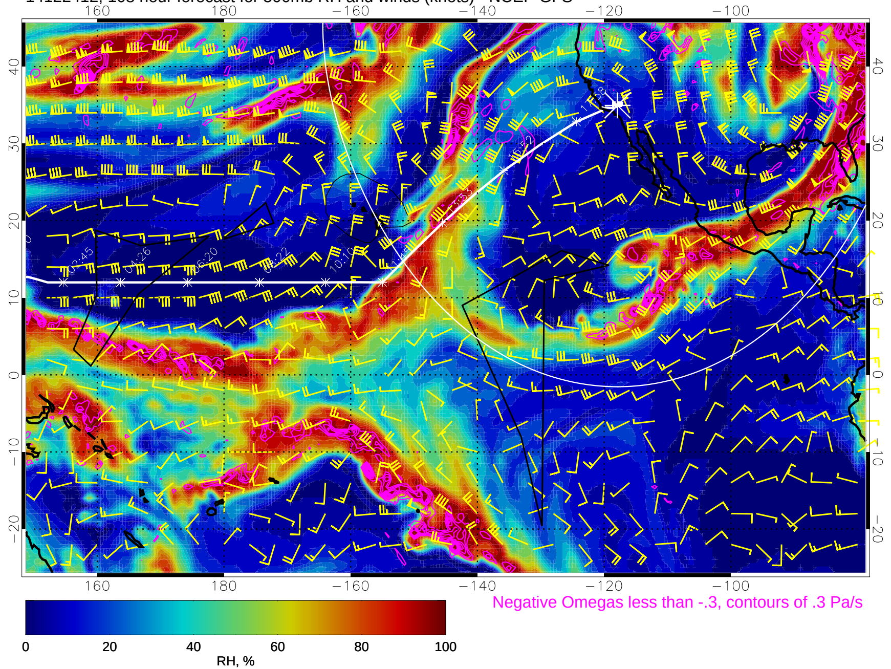
14122412, 108 hour forecast for 500mb RH and winds (knots) - NCEP GFS
