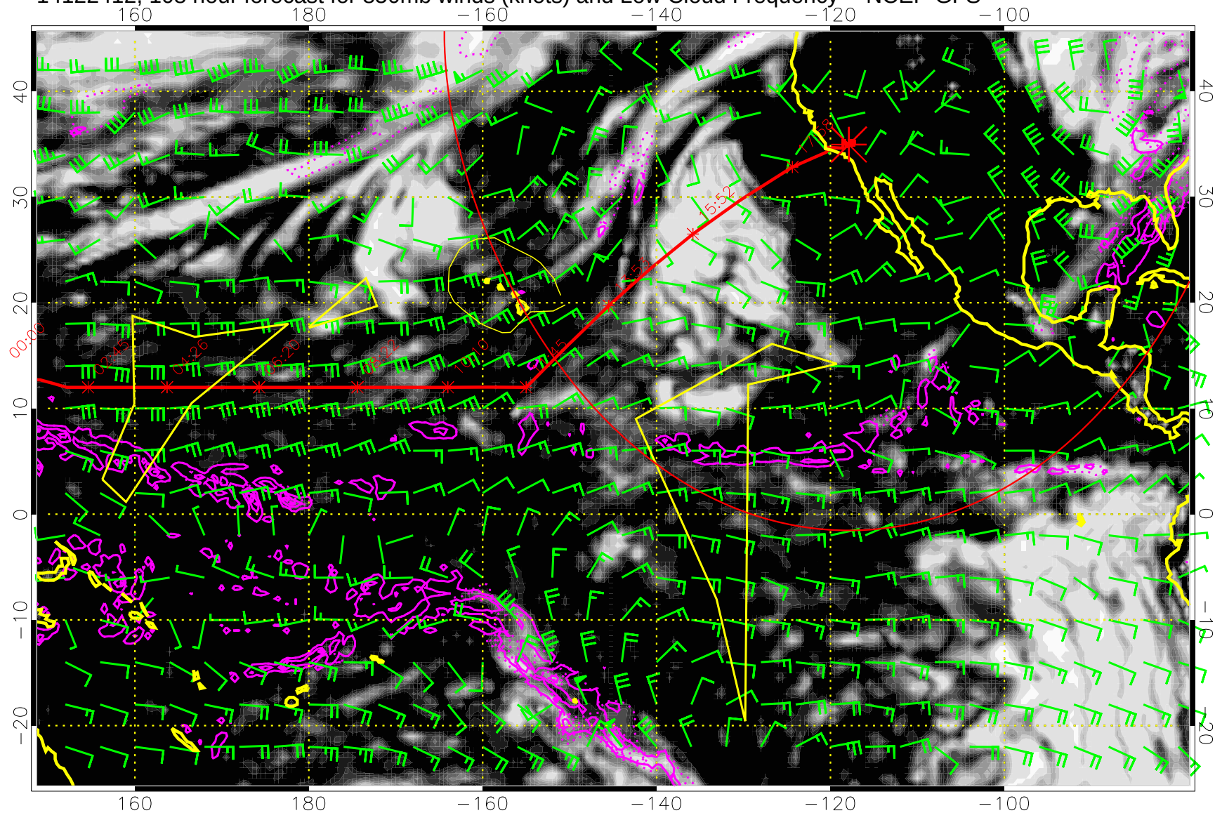
14122412, 108 hour forecast for 850mb winds (knots) and Low Cloud Frequency -- NCEP GFS
