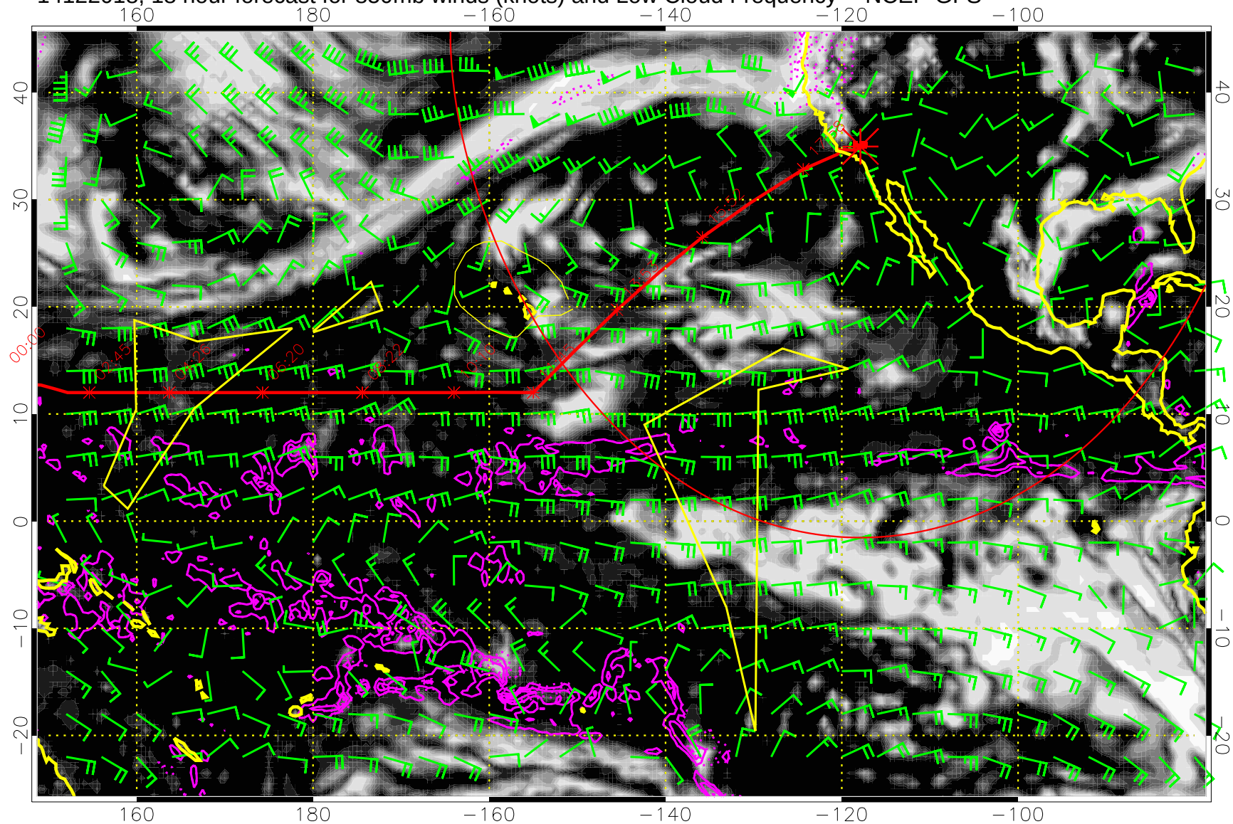
14122018, 18 hour forecast for 850mb winds (knots) and Low Cloud Frequency -- NCEP GFS
