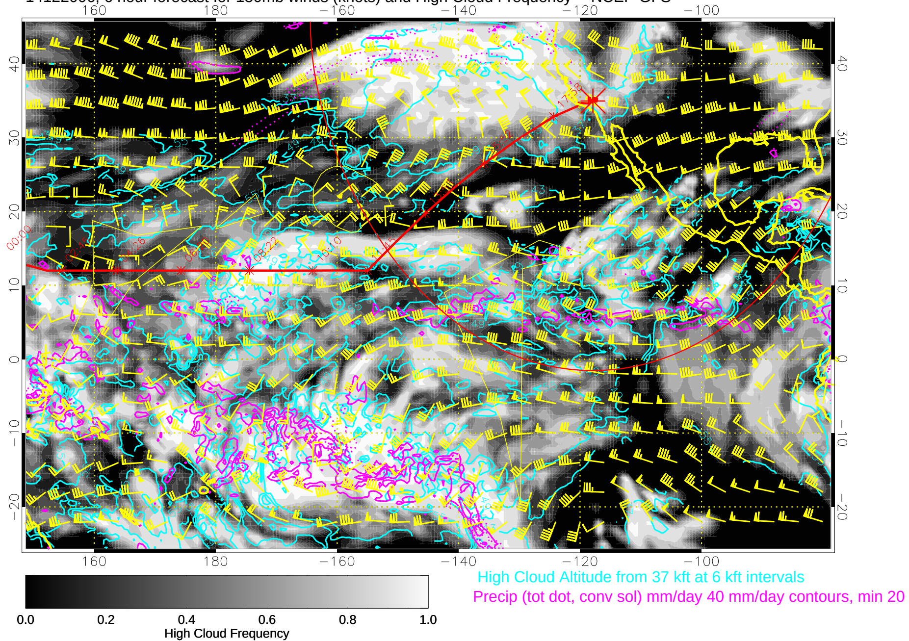
14122006, 6 hour forecast for 150mb winds (knots) and High Cloud Frequency -- NCEP GFS
