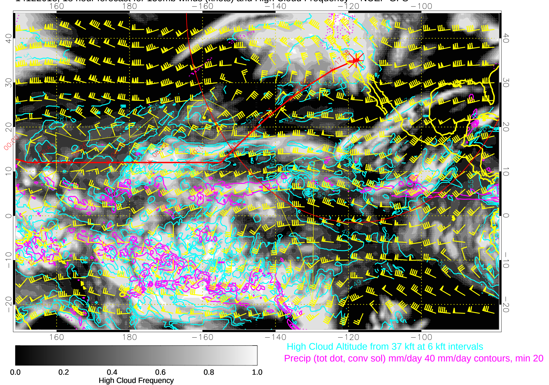
14122018, 18 hour forecast for 150mb winds (knots) and High Cloud Frequency -- NCEP GFS
