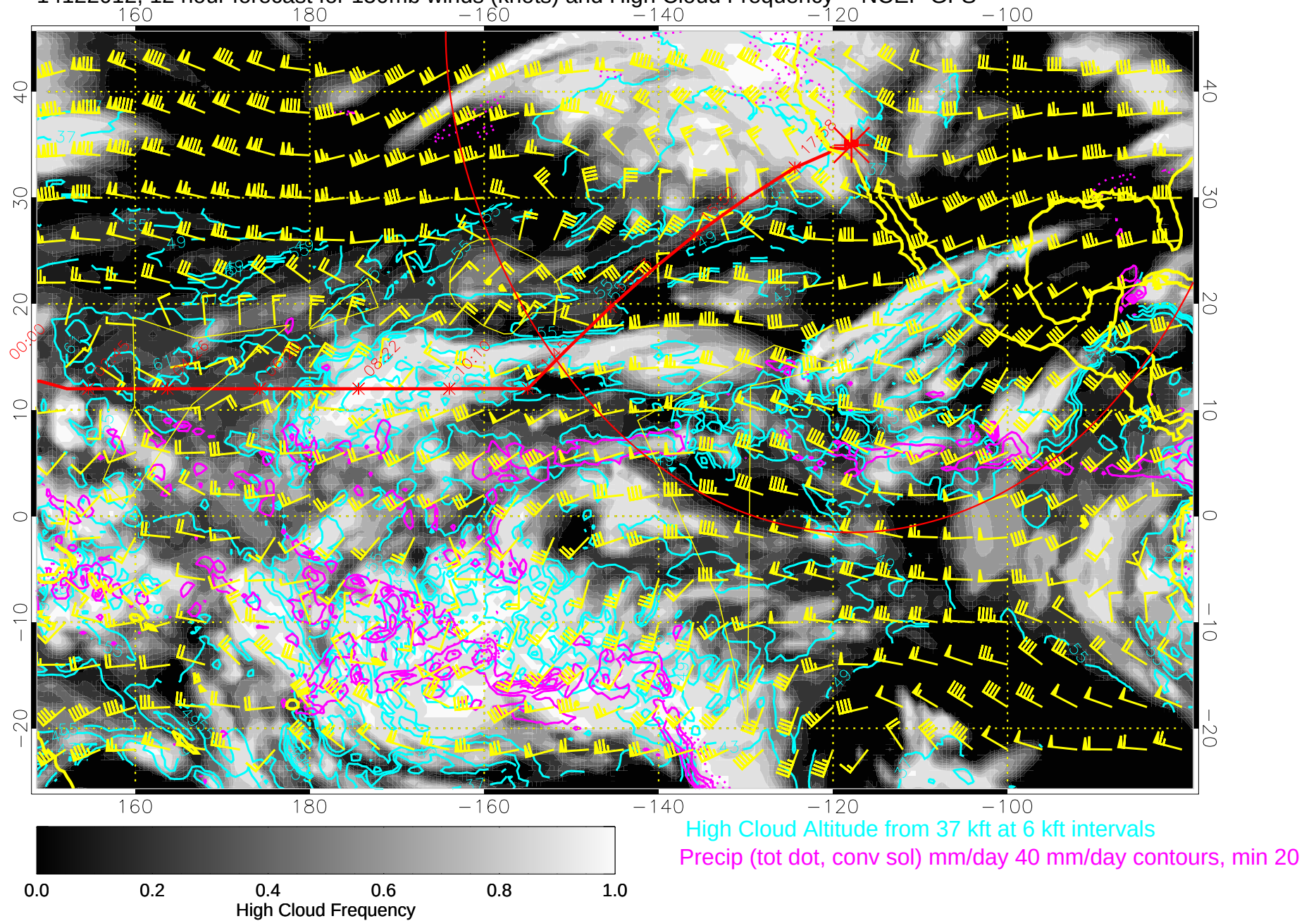
14122012, 12 hour forecast for 150mb winds (knots) and High Cloud Frequency -- NCEP GFS
